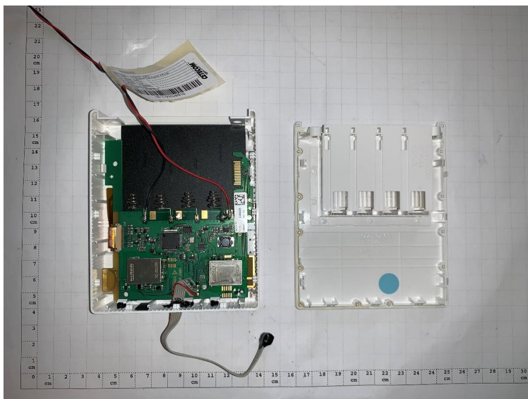
Photograph 18: EUT D, bottom view, opened
