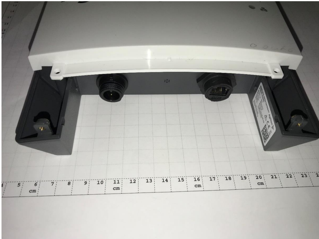
Photograph 21: AE 3, rear view
