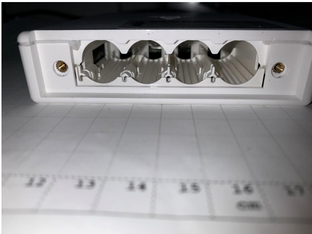
Photograph 15: EUT C, left side, cover open
