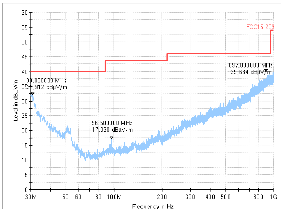
Diagram 7: Channel 11 (3.03_Ch11_PWR0_laying)
