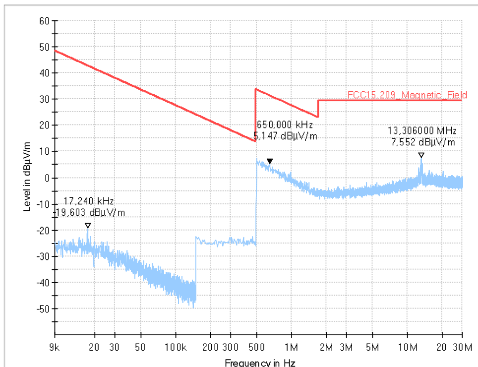
Diagram 3: Channel 18 (2.07_MgF_Ch18_PWR0_standing)
