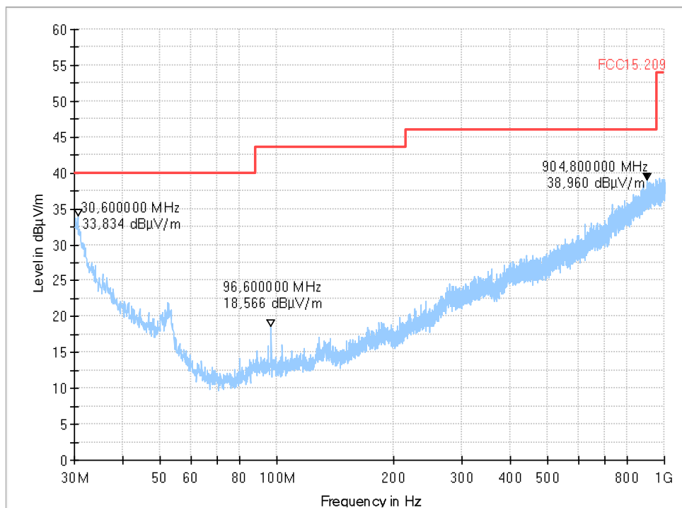
Diagram 8: Channel 11 (3.06_Ch11_PWR0_standing)
