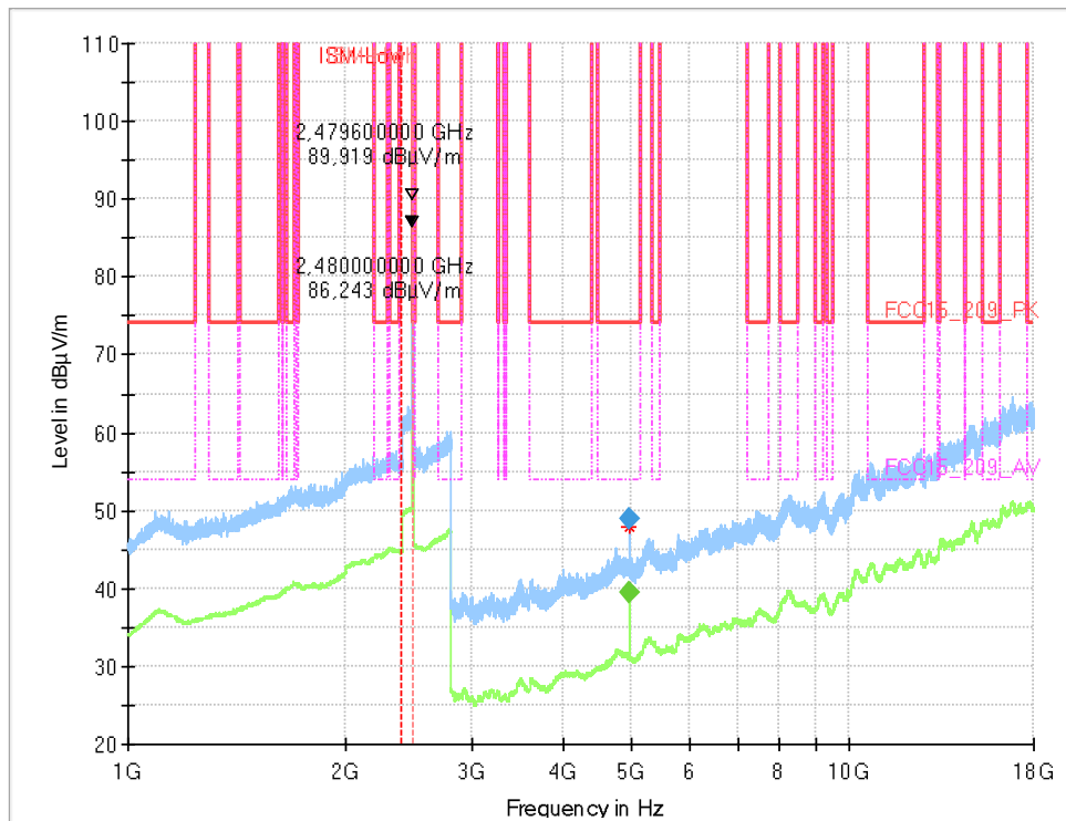
Diagram 15: Channel 26 (4.06_Ch26_PWR4)
