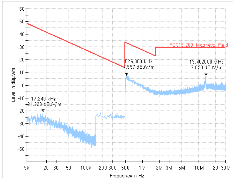
Diagram 1: Channel 11 (2.05_MgF_Ch11_PWR0_laying)
