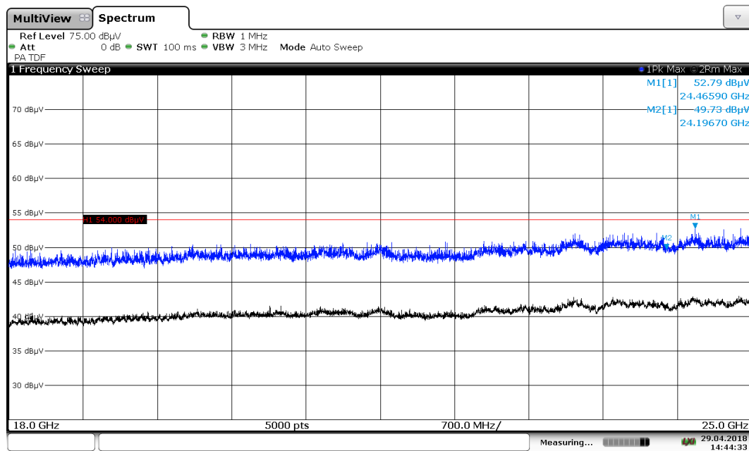
Diagram 18: 4.15_Ch26_PWR4
