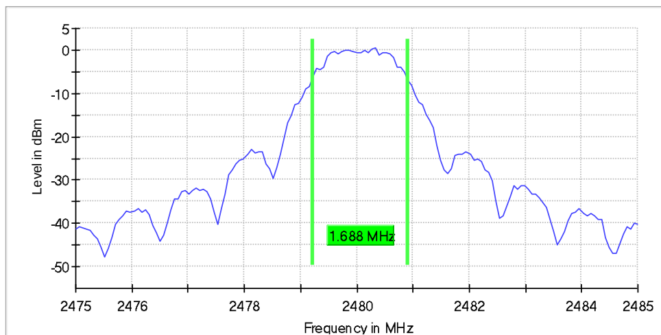
Diagram 29: Channel 26
