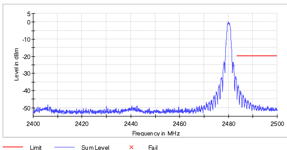
Diagram 20: Channel 26 – Band –Edge high (Ch26=2480MHz), PWR -4
