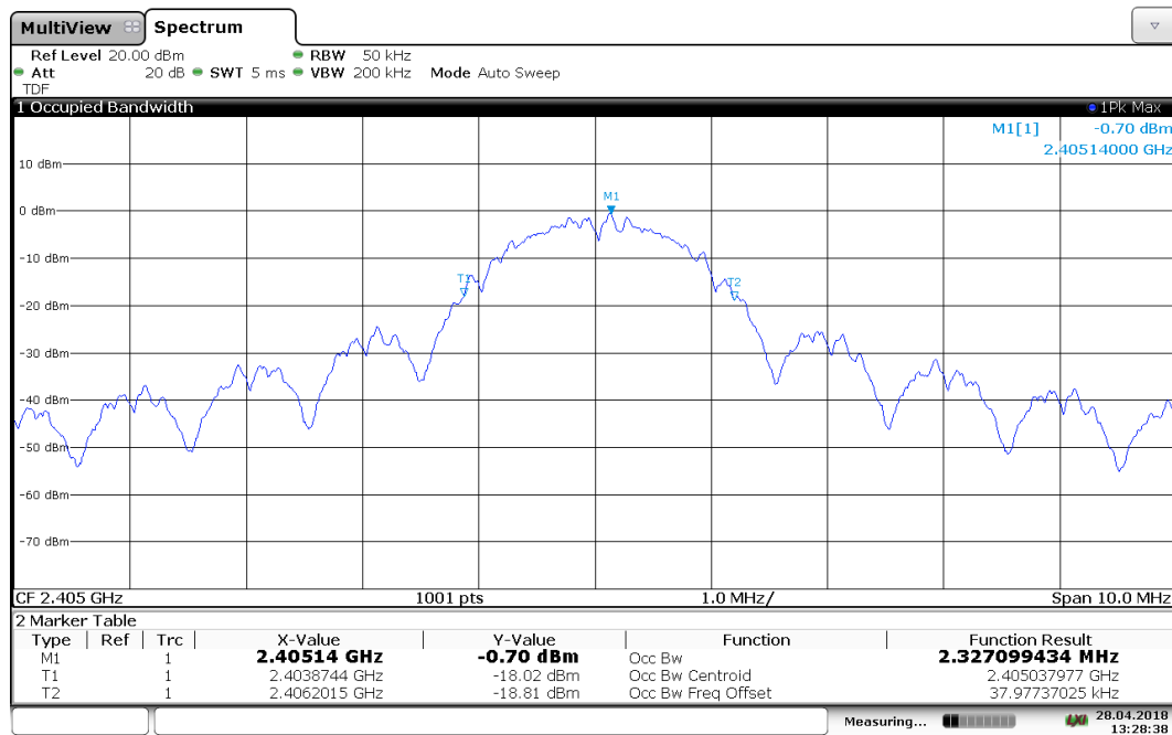
Diagram 30: OBW 99% - channel 11
