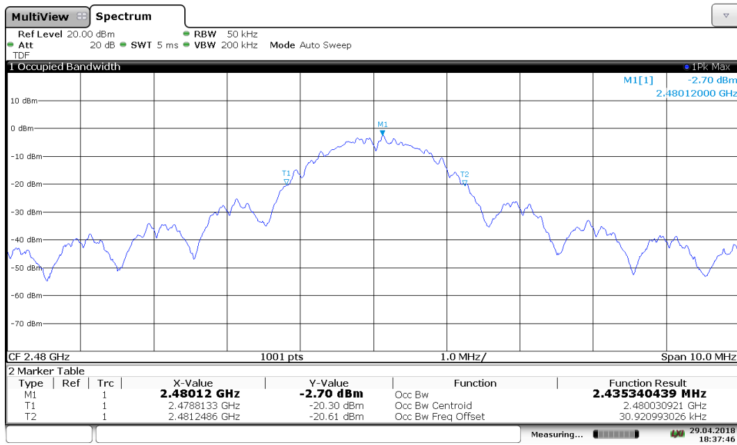
Diagram 32: OBW 99% - channel 26
