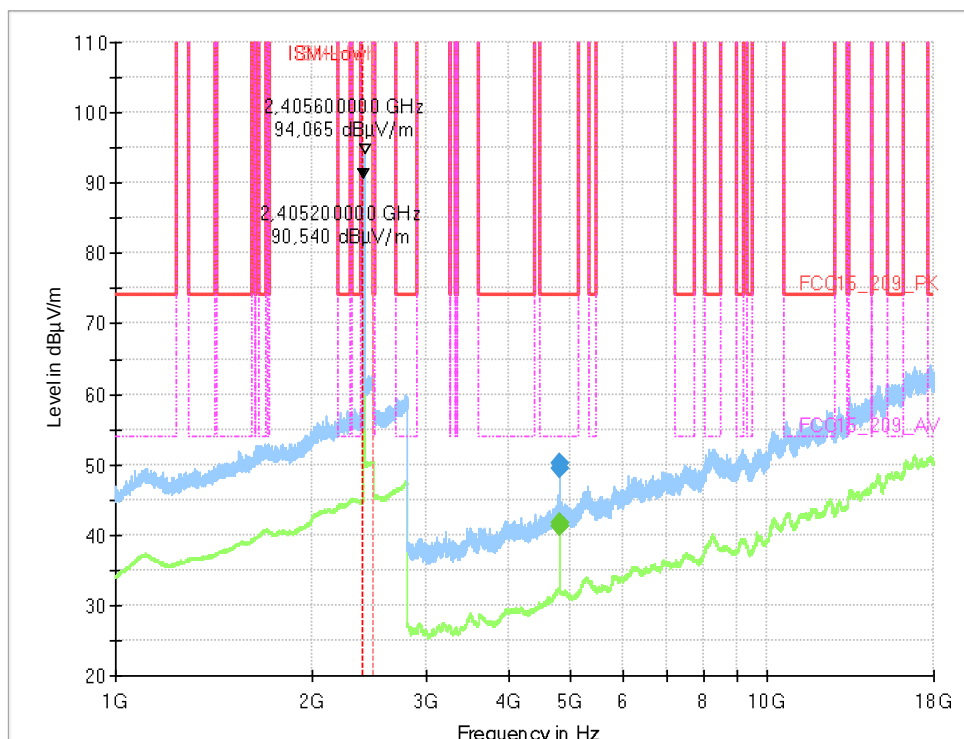
Diagram 13: Channel 11 (4.04_Ch11_PWR0)
