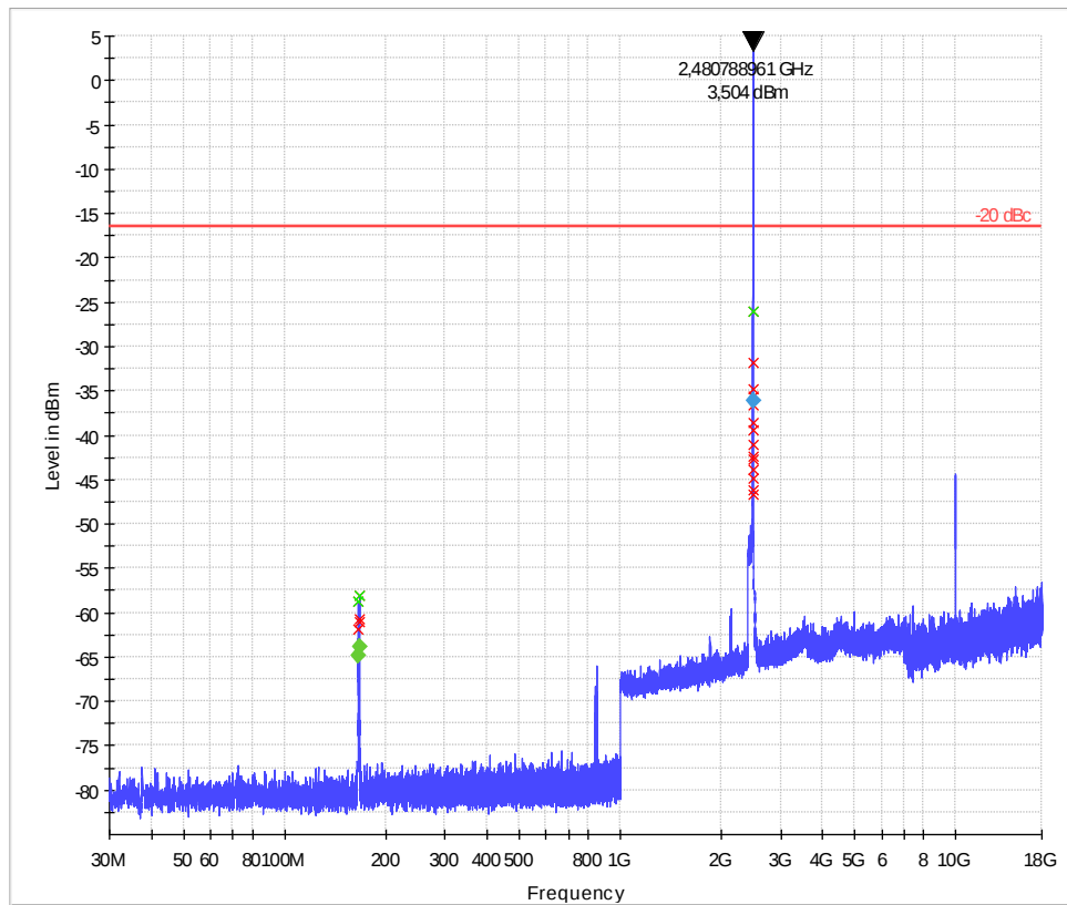
Diagram 38: 20dBc emissions on channel 26 -> Pass
