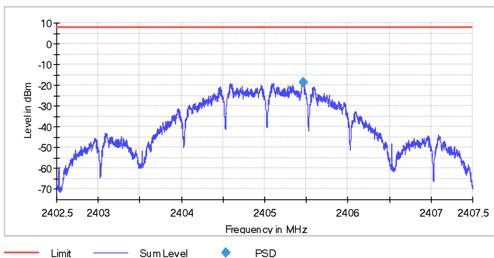
Diagram 33: Power Spectrum density (channel 11)
