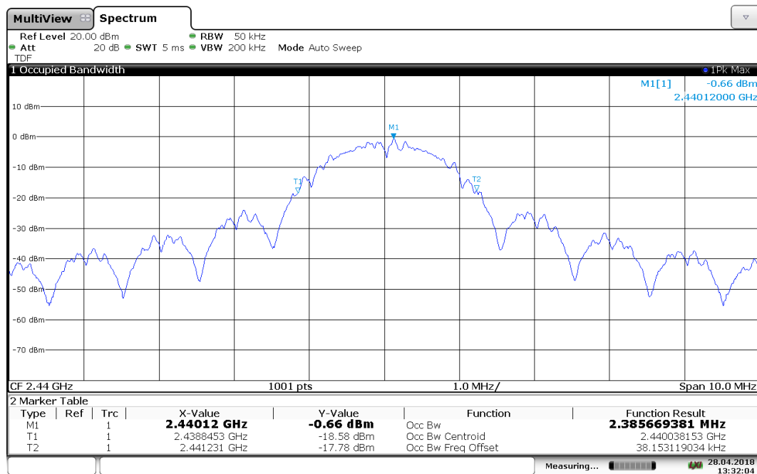
Diagram 31: OBW 99% - channel 18
