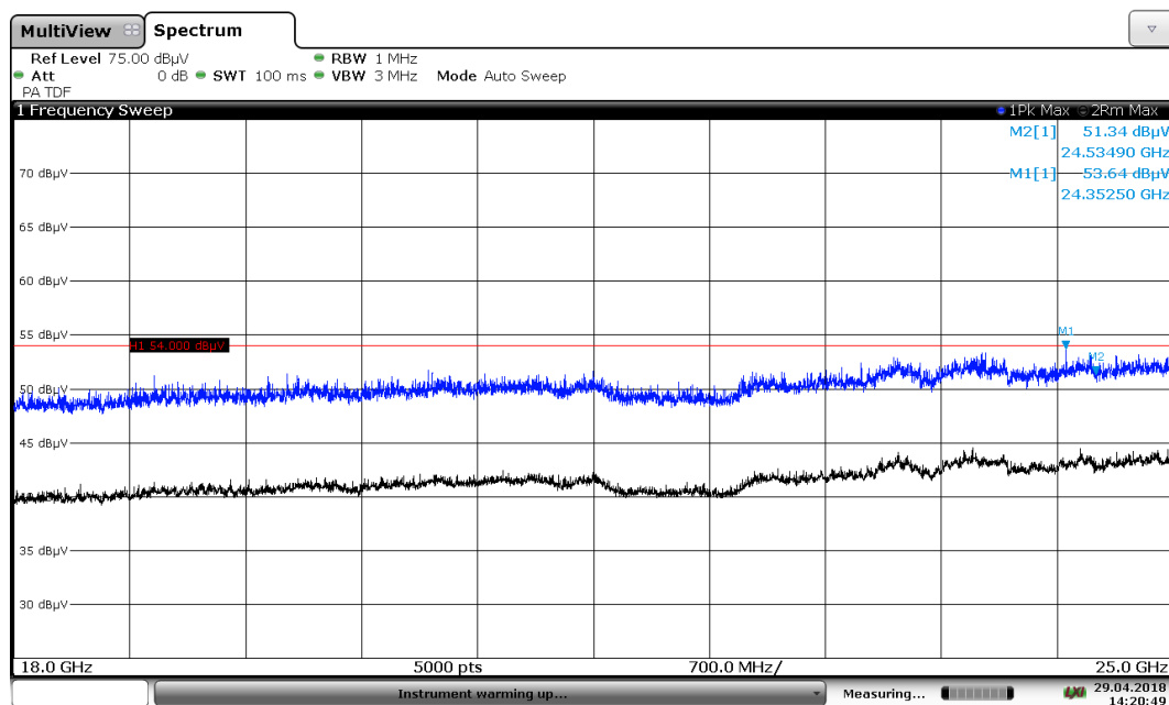
Diagram 16: 4.13_Ch11_PWR0
