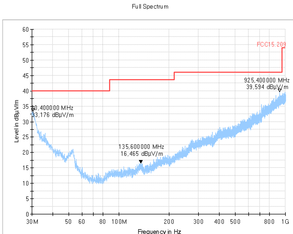
Diagram 11: Channel 26 (3.01_Ch26_PWR4_laying)
