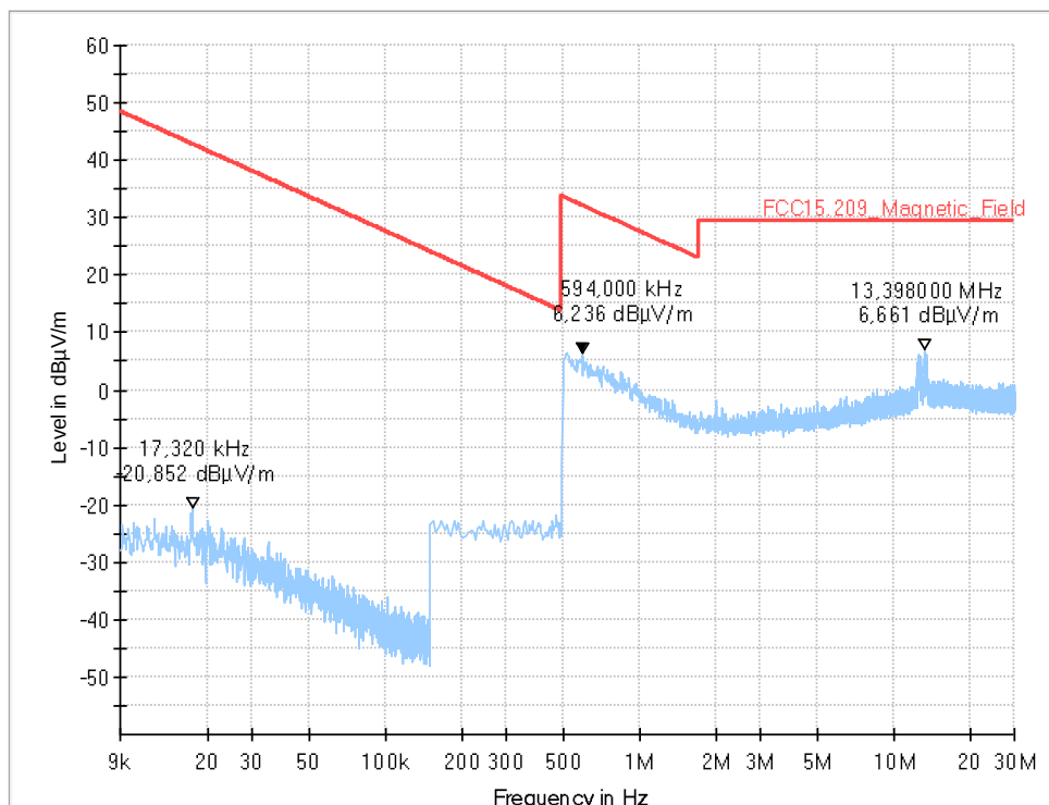
Diagram 4: Channel 18 (2.08_MgF_Ch18_PWR0_laying)
