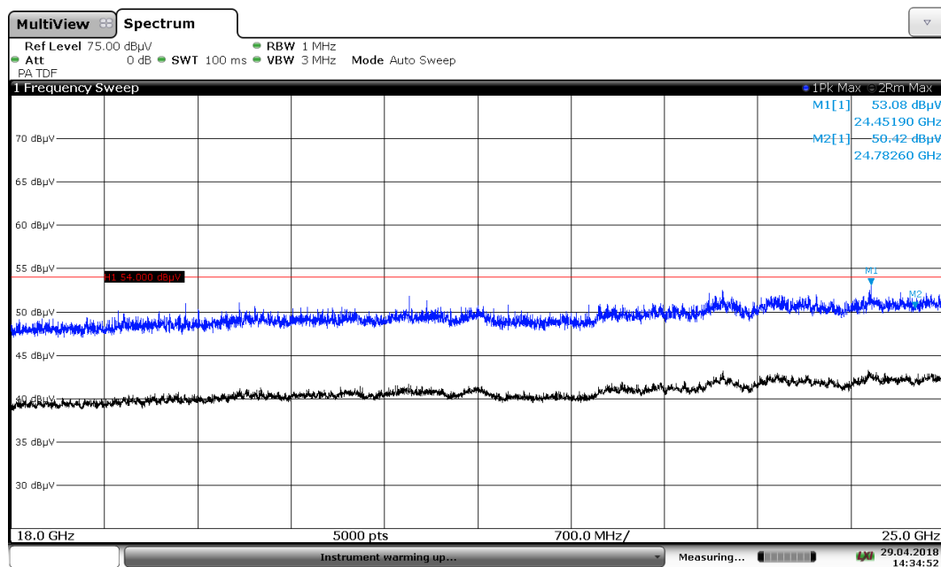
Diagram 17: 4.14_Ch18_PWR0
