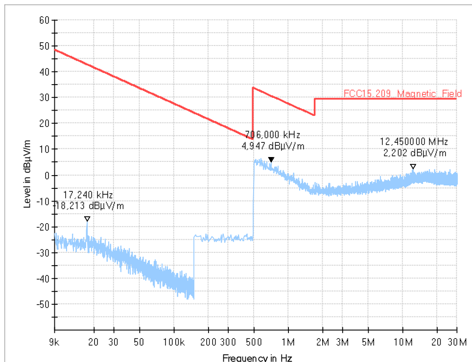
Diagram 2: Channel 11 (2.06_MgF_Ch11_PWR0_standing)
