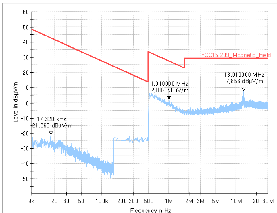
Diagram 6: Channel 26 (2.10_MgF_Ch26_PWR4_standing)
