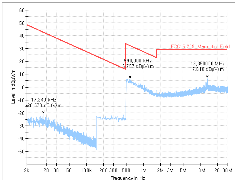
Diagram 5: Channel 26 (2.09_MgF_Ch26_PWR4_laying)
