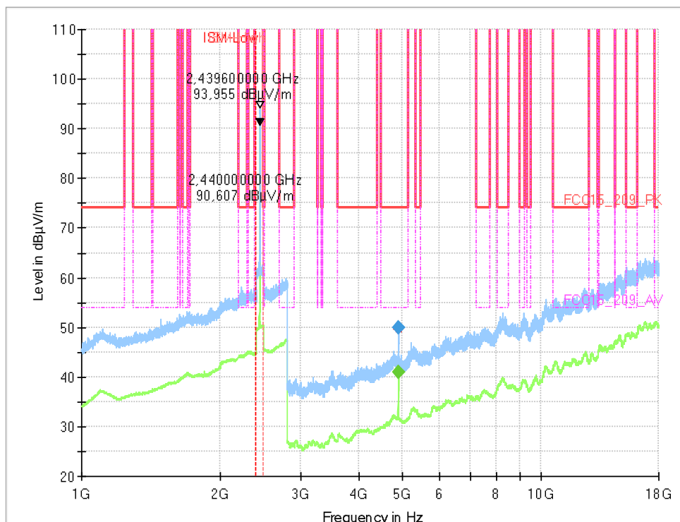
Diagram 14: Channel 18 (4.05_Ch18_PWR0)
