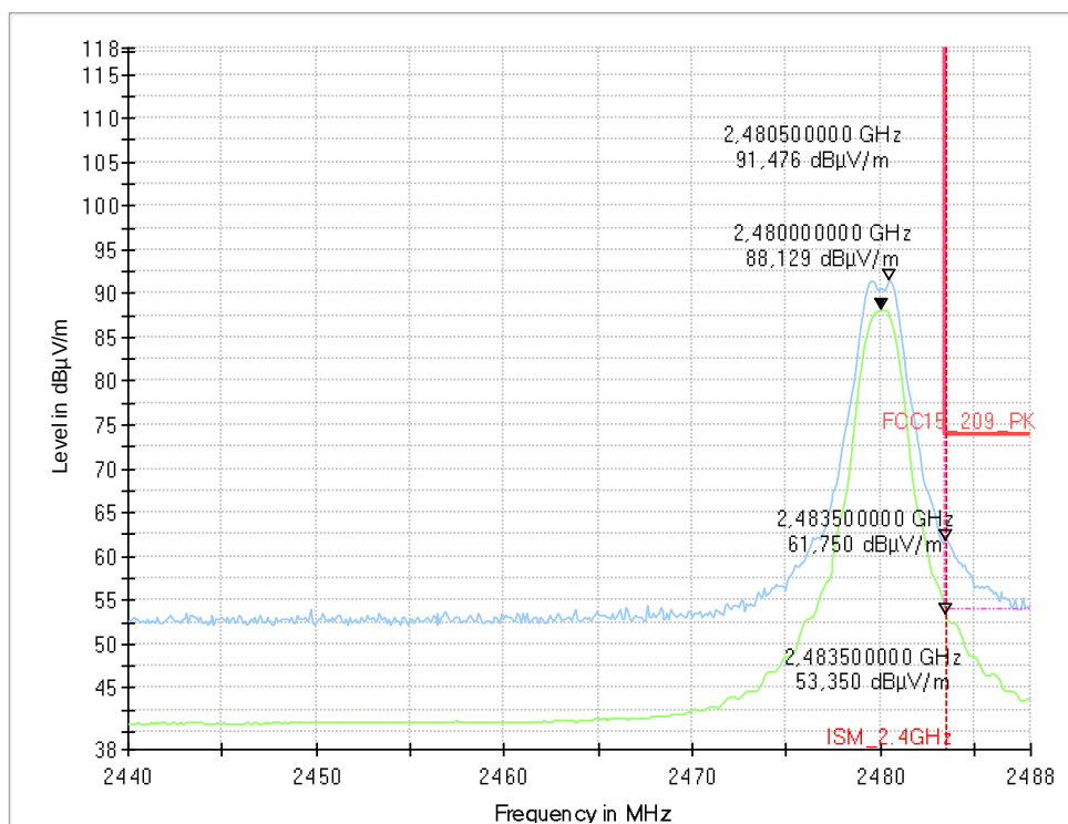
Diagram 21: Channel 26 – Band –Edge high (Ch26=2480MHz), PWR -4
