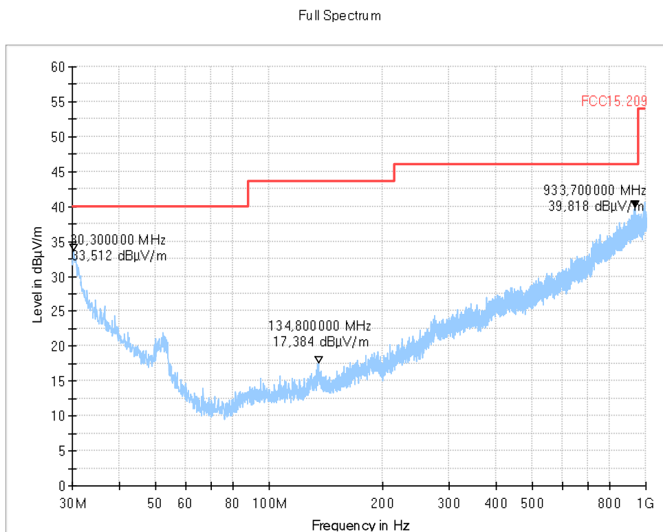
Diagram 12: Channel 26 (3.04_Ch26_PWR4_standing)
