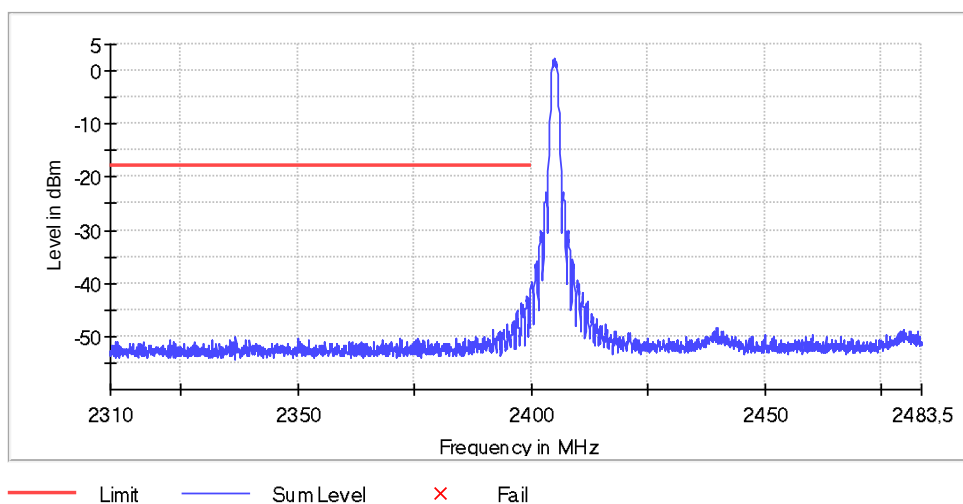
Diagram 19: Channel 11 – Band –Edge low (Ch11=2405MHz), PWR 0
