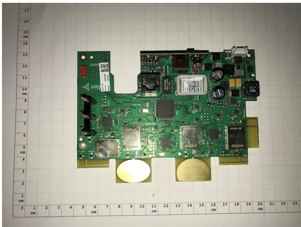
Photograph 2: EUT A, PCB, top view
