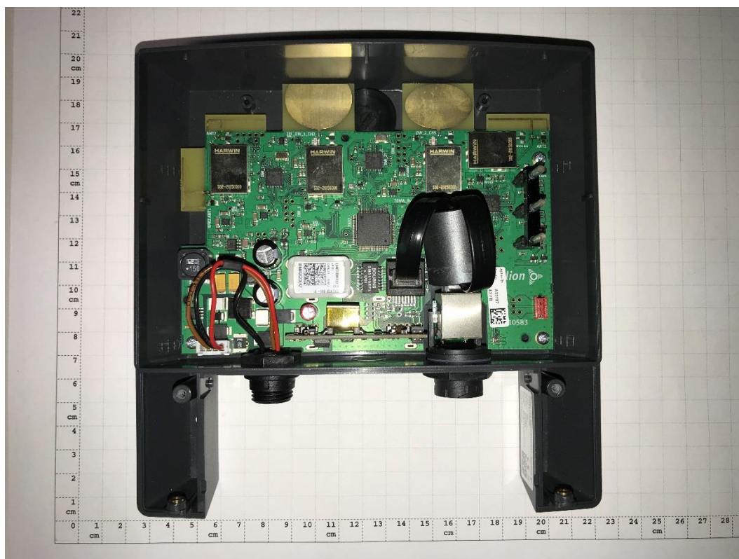
Photograph 1: EUT A, PCB + case, top view
