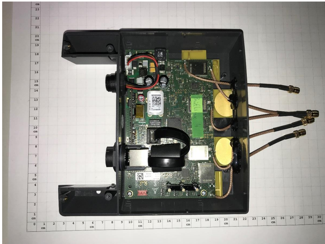
Photograph 6: EUT B, PCB + case
