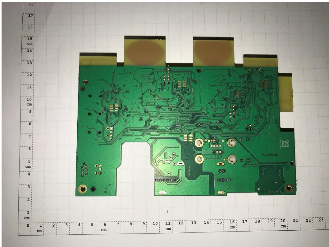
Photograph 3: EUT A, PCB, bottom view
