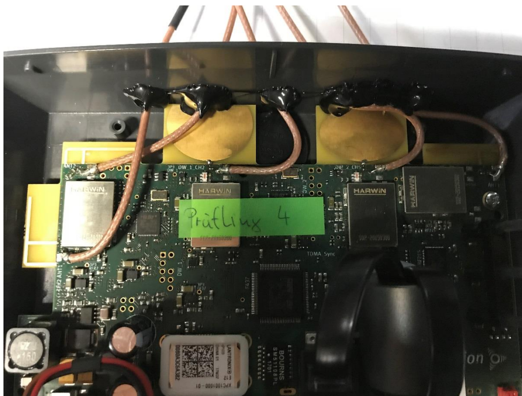
Photograph 7: EUT B, antennas/antenna connectors close view, from left to right: Ant 1, RFR 2 Ant 2, DW Ch 2, DW Ch 5, RF 215
