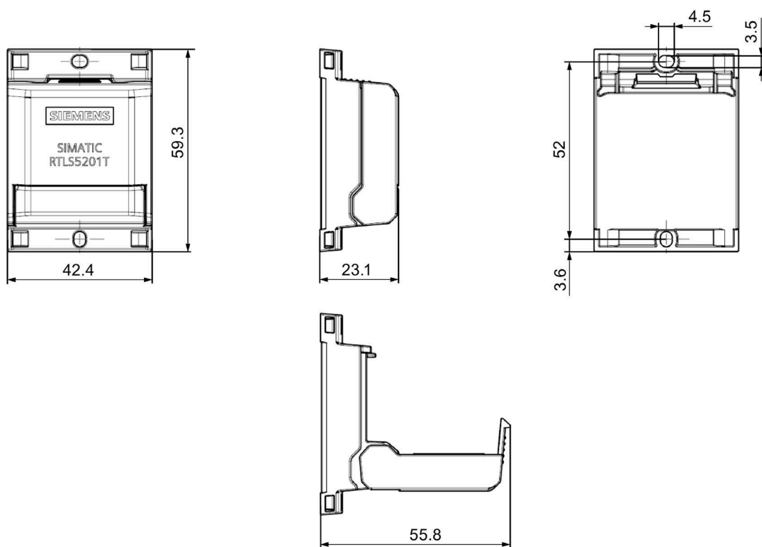
Figure 2-1 Dimension drawing SIMATIC RTL55201T - All dimensions are specified in millimeters
