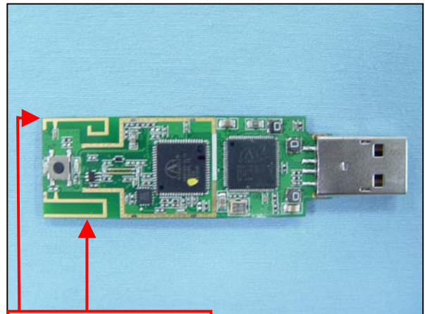
PCB Antenna
