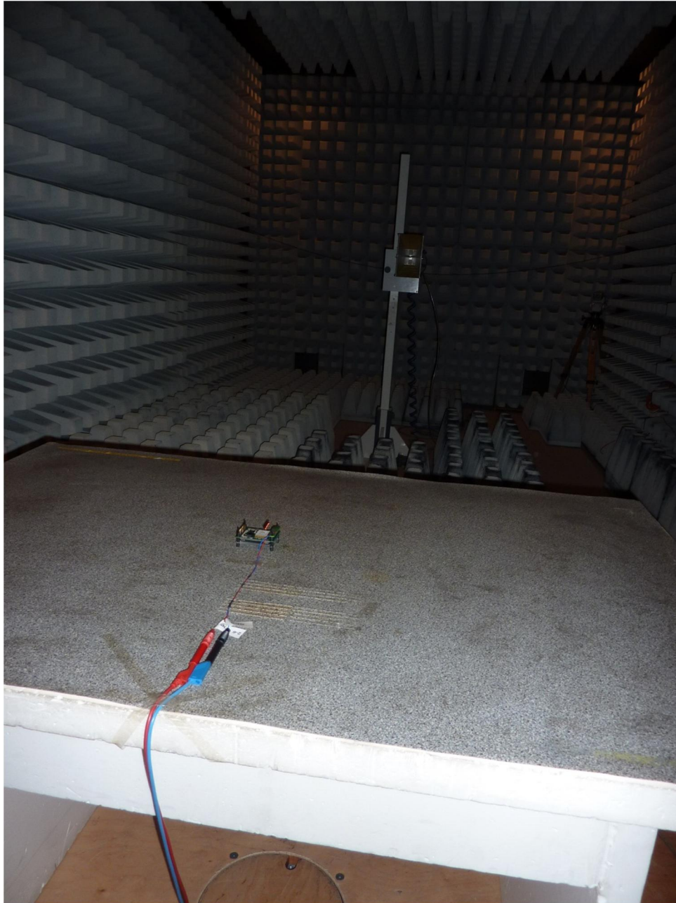
130413_6.JPG: Test setup fully anechoic chamber
