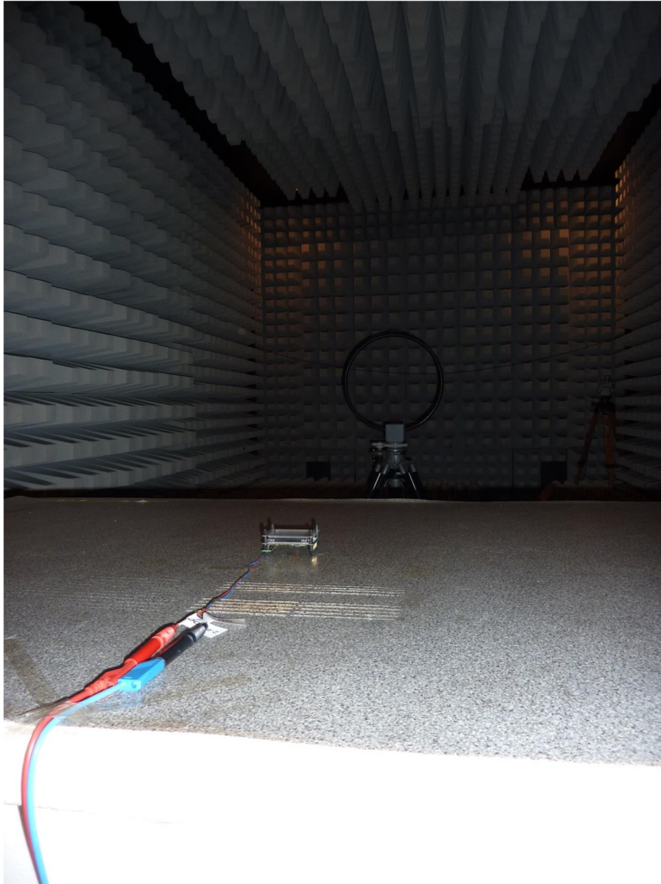
130413_4.JPG: Test setup fully anechoic chamber
