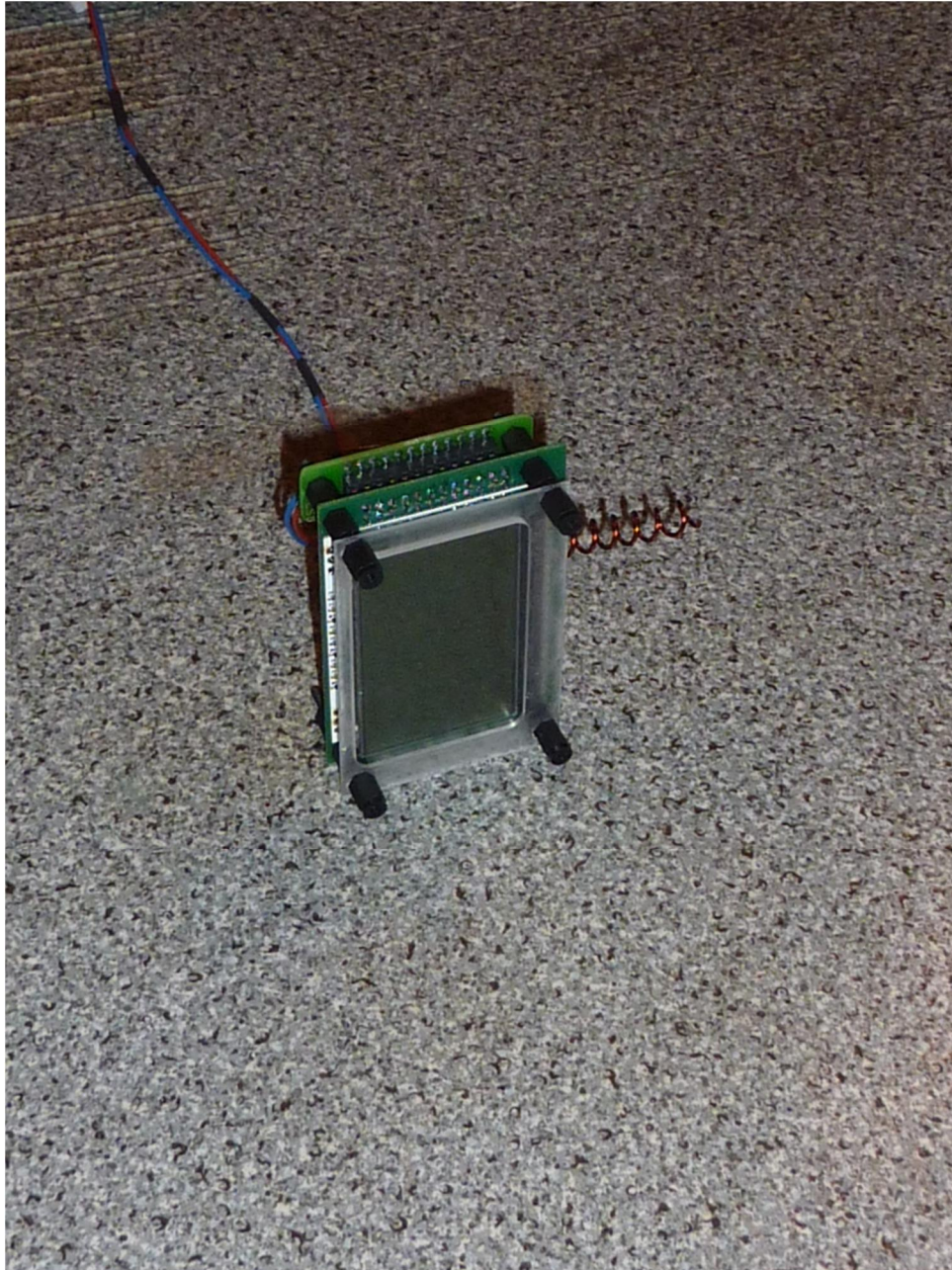
130413_2.JPG: Test setup fully anechoic chamber (Position 2)
