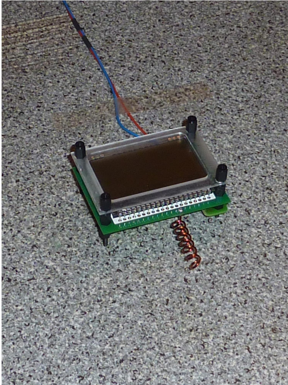
130413_3.JPG: Test setup fully anechoic chamber (Position 3)
