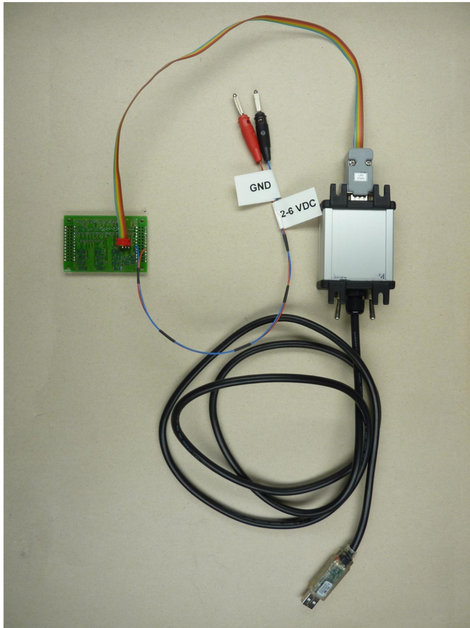
130413_14.JPG: Ancillary programmer (connected to programming PCB)
