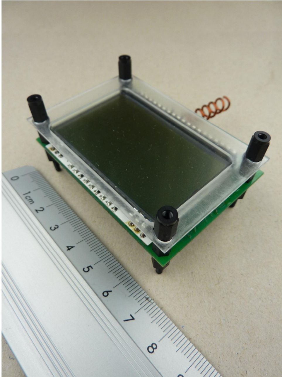
130413_10.JPG: H153V2, 3D view 1
