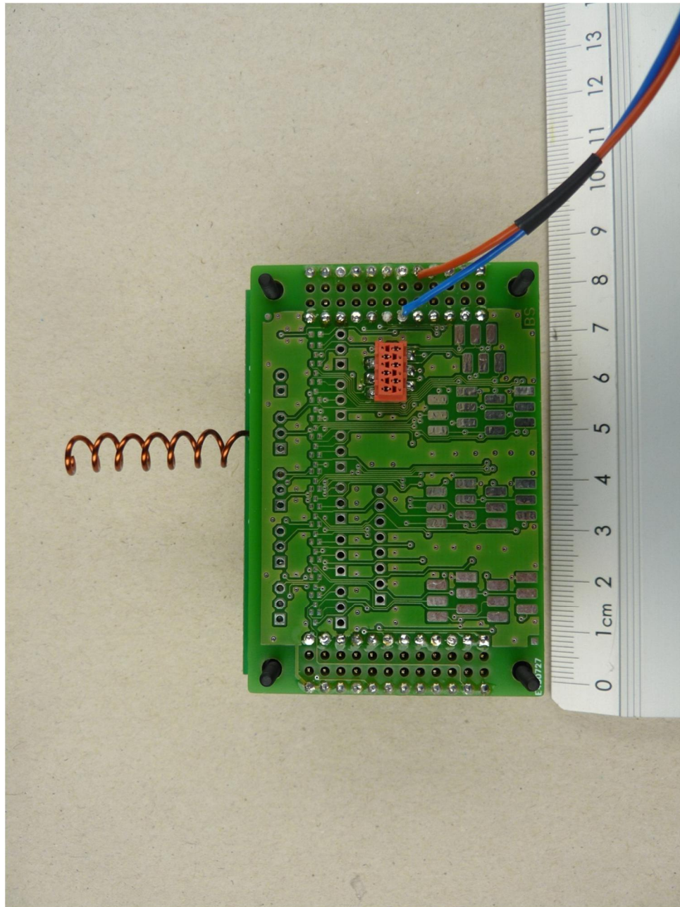
130413_13.JPG: Supply and programming PCB connected to H153V2, bottom view
