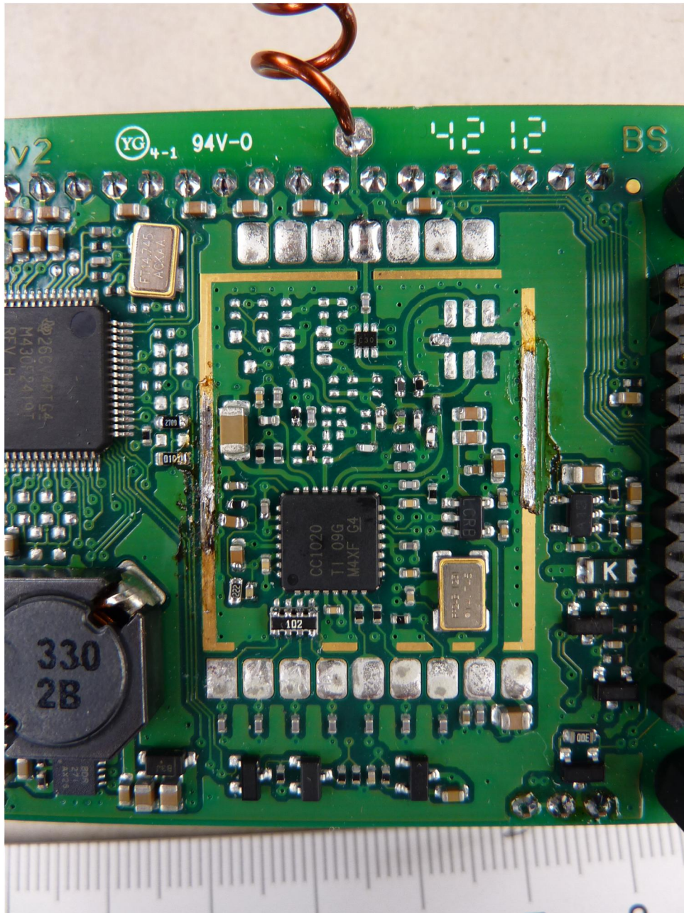
130413_15.JPG: shielding removed
