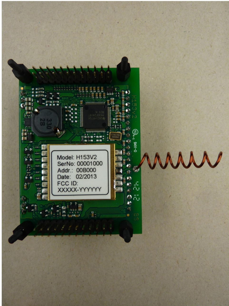
130413_12.JPG: H153V2, PCB bottom and type plate view
