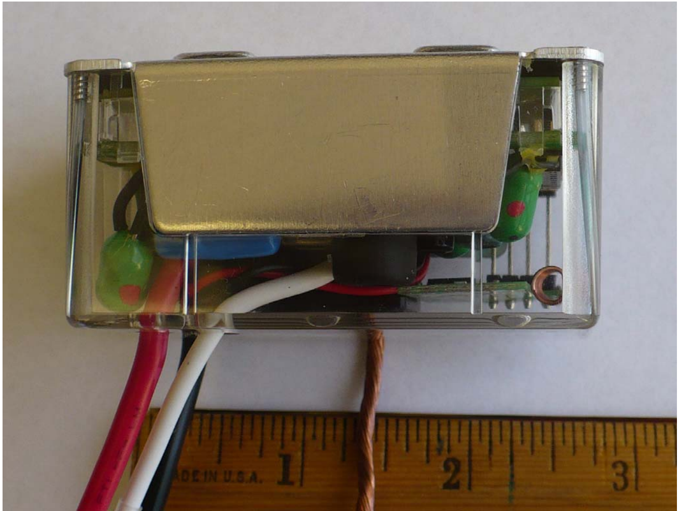
Right-Side View
