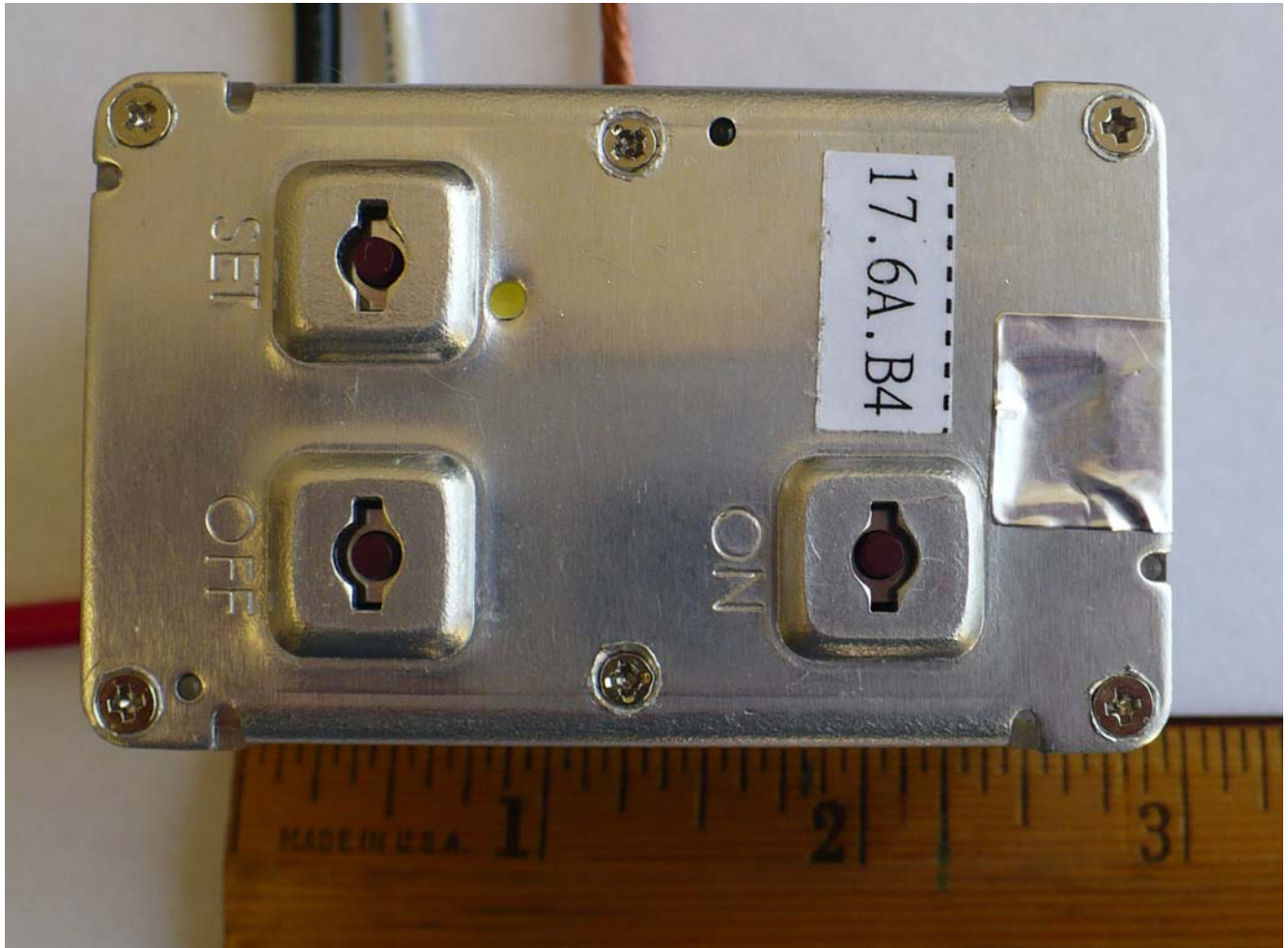
Front View
