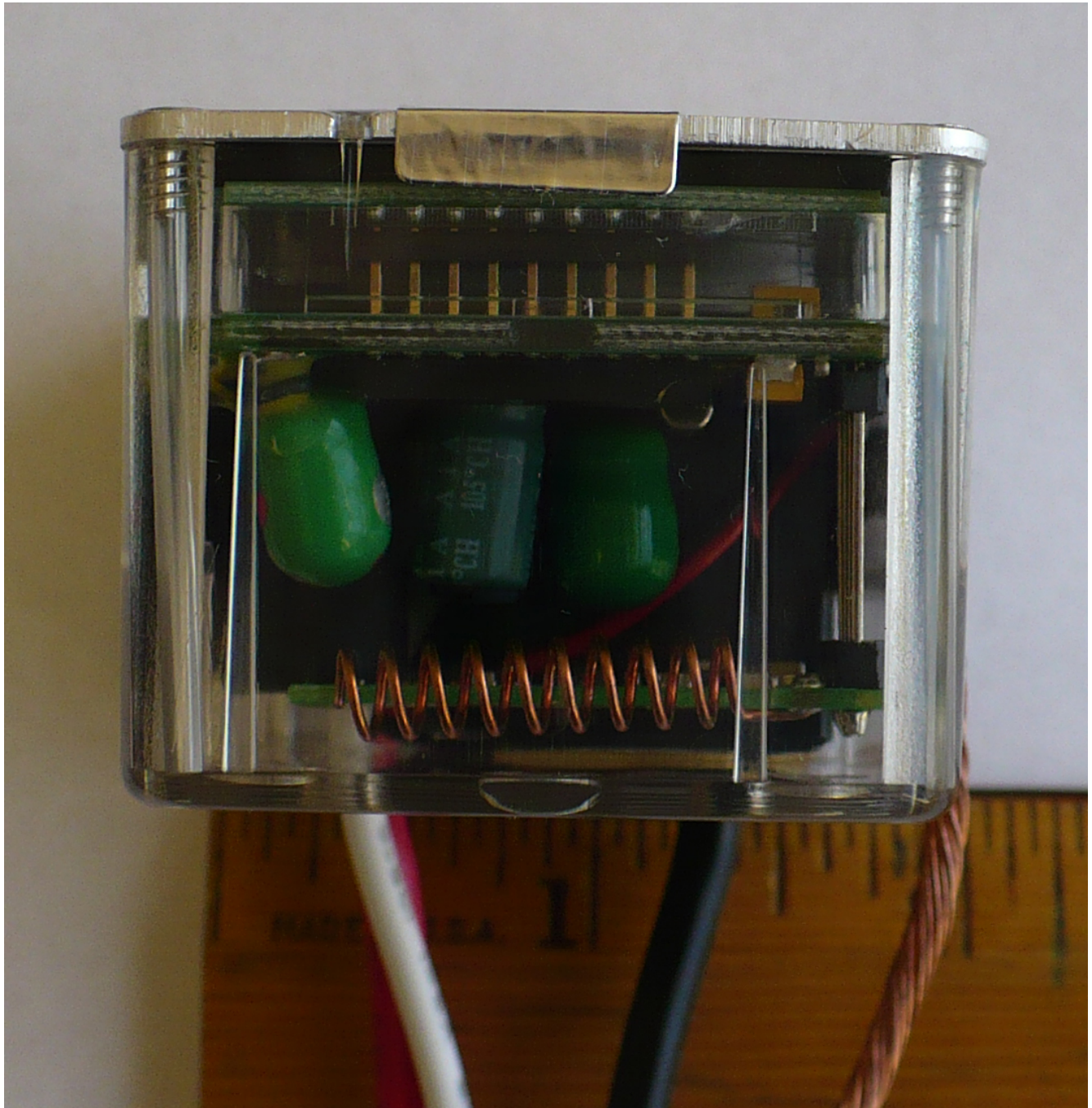
Top-End View
