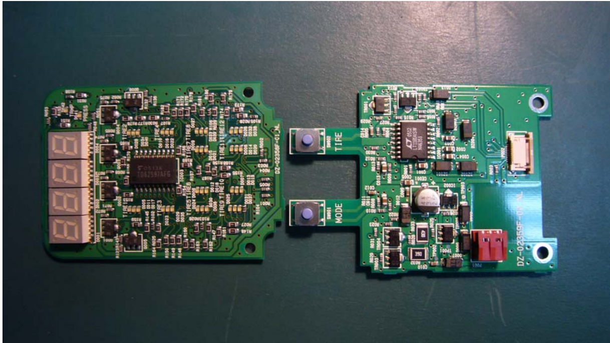
TOP View
