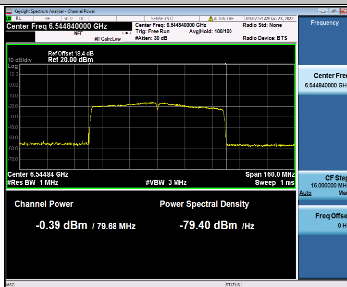
11AC80SISO_Ant2_6545
