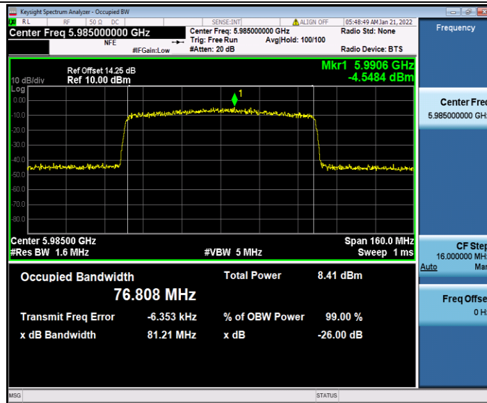
11AX80ISO_Ant2_5985
