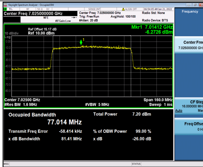
11AX80SISO_Ant2_7025
