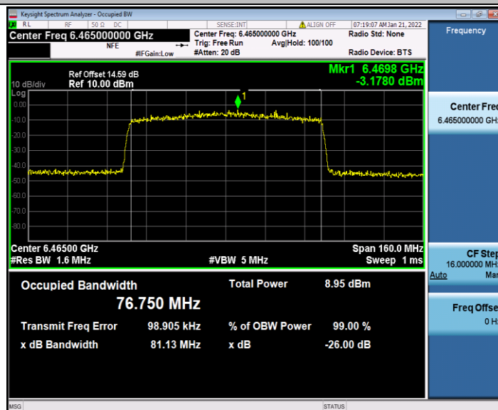
11AX80SISO_Ant2_6465
