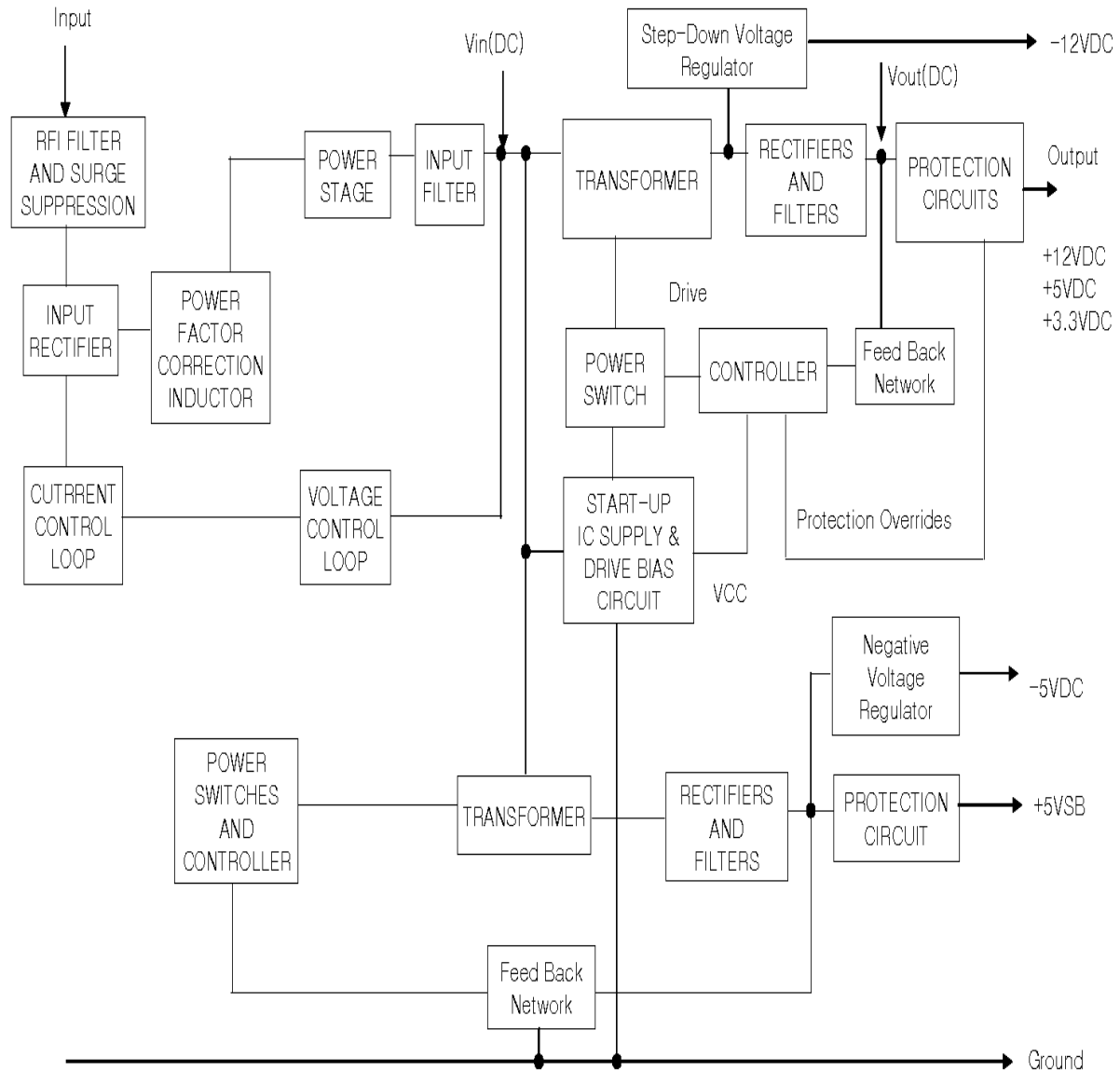
Block Diagram TNN400APF-V2
