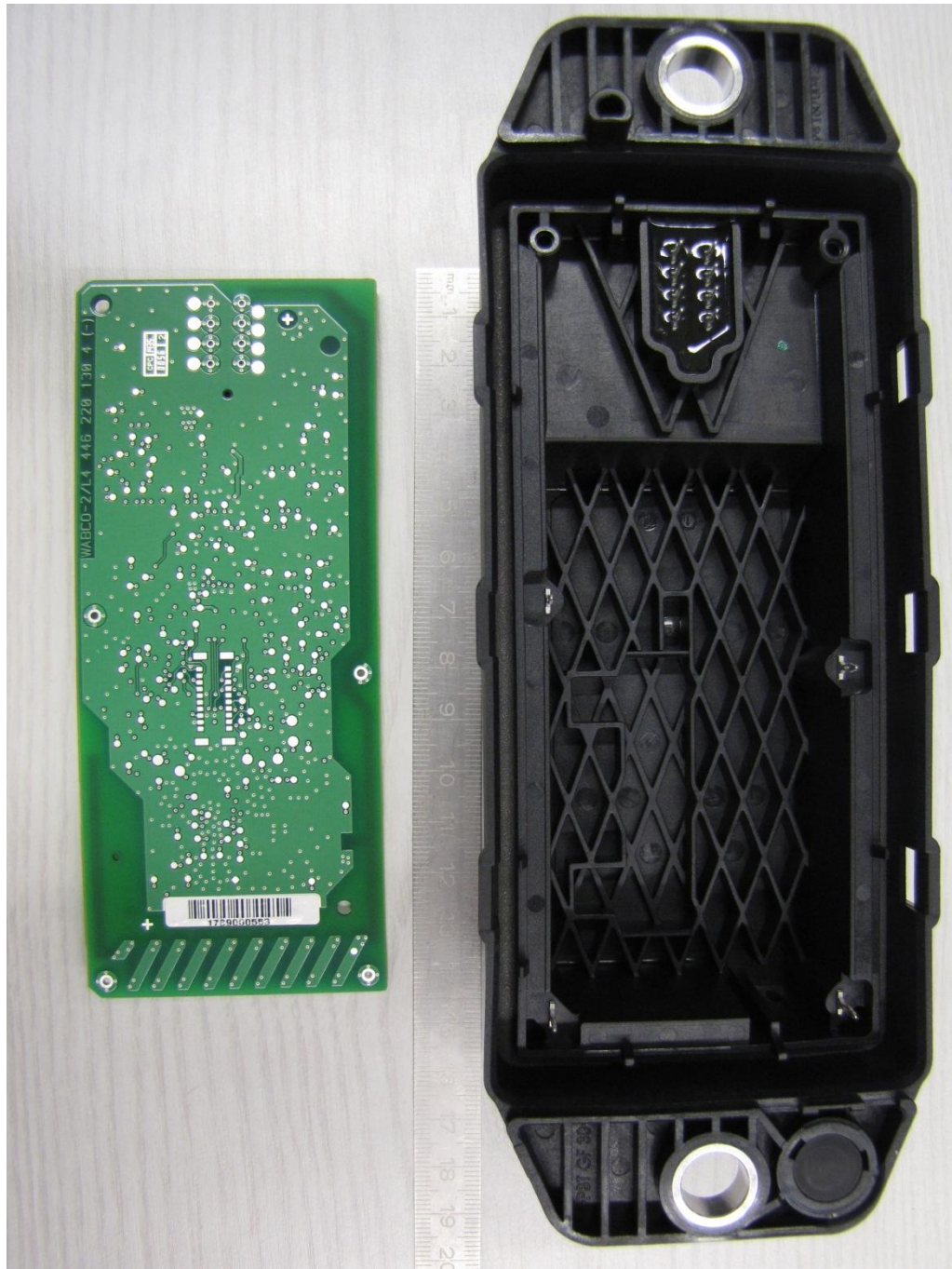
150998_10.JPG: OptiTire ECU, internal view
