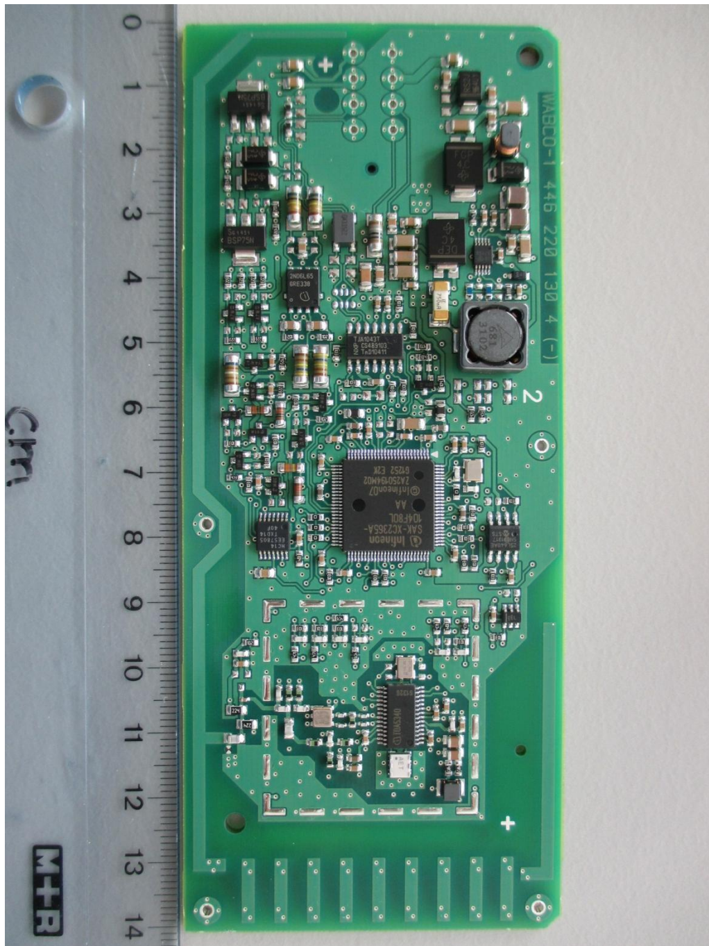
150998_3.JPG: OptiTire ECU, PCB, top view
