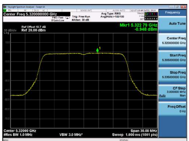
PSD-802.11a-5320M-chain4
