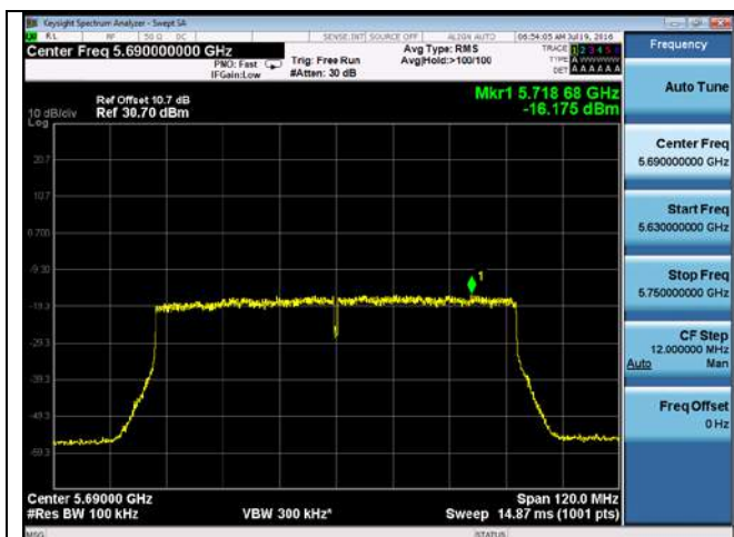
PSD-802.11ac-CROSS-5690M-chain1
