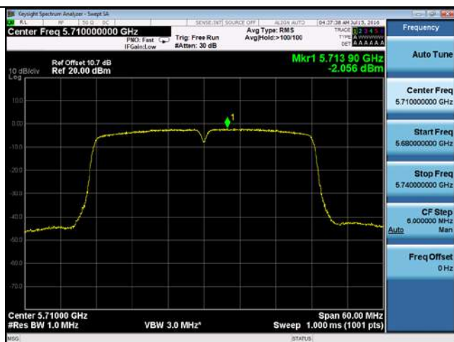
PSD-802.11n-40M-CROSS-5710M-chain1
