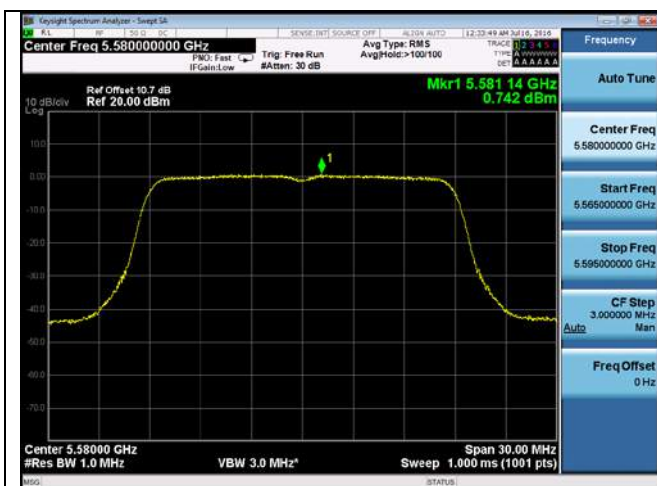
PSD-802.11n-20M-5580M-chain3
