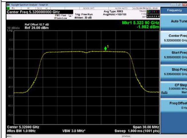
PSD-802.11n-20M-5320M-chain1
