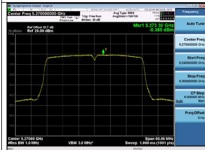
PSD-802.11n-40M-5270M-chain3
