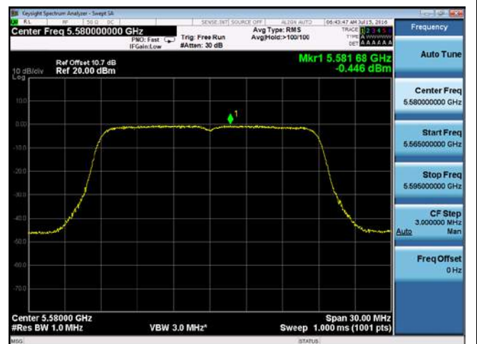
PSD-802.11n-20M-5580M-chain2
