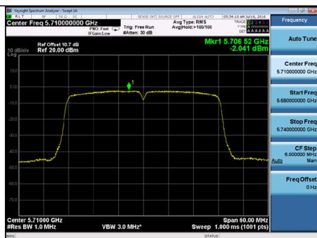
PSD-802.11n-40M-CROSS-5710M-chain4
