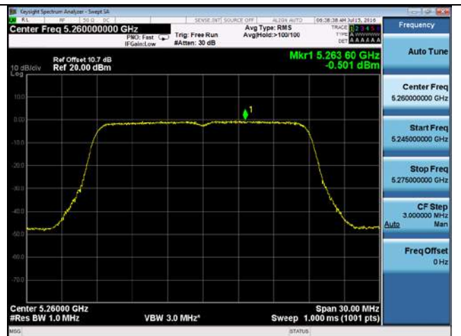
PSD-802.11n-20M-5260M-chain2
