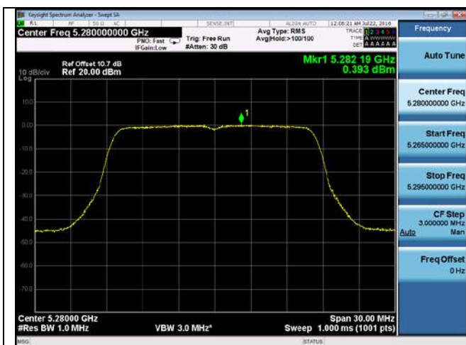
PSD-802.11a-5280M-chain3
