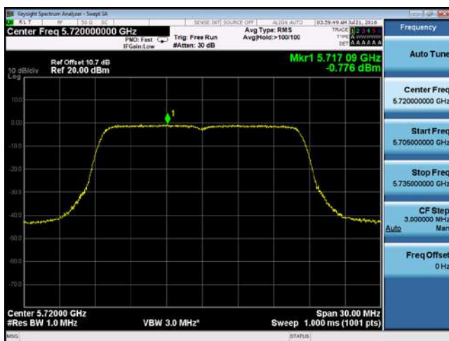
PSD-802.11a-CROSS-5720M-chain3
