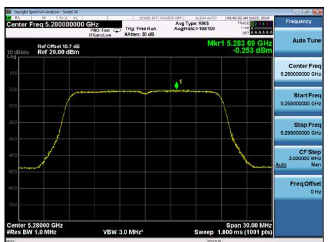
PSD-802.11n-20M-5280M-chain2
