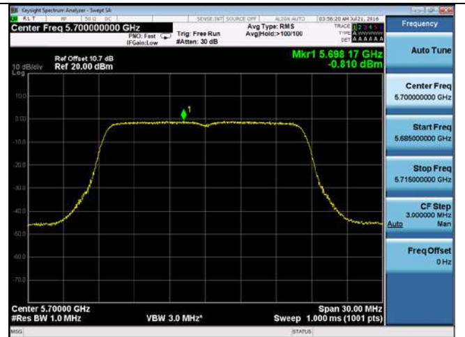
PSD-802.11a-5700M-chain2
