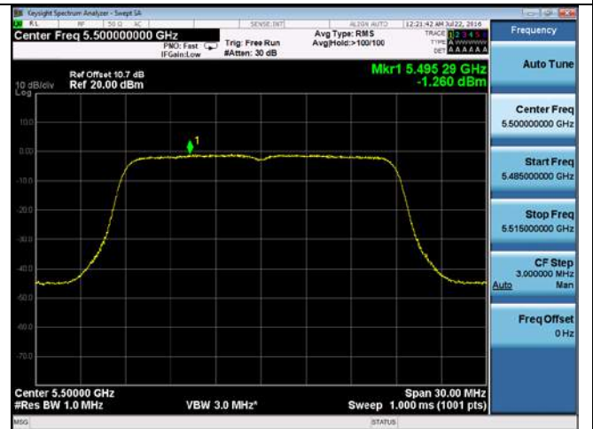
PSD-802.11n-20M-5500M-chain4
