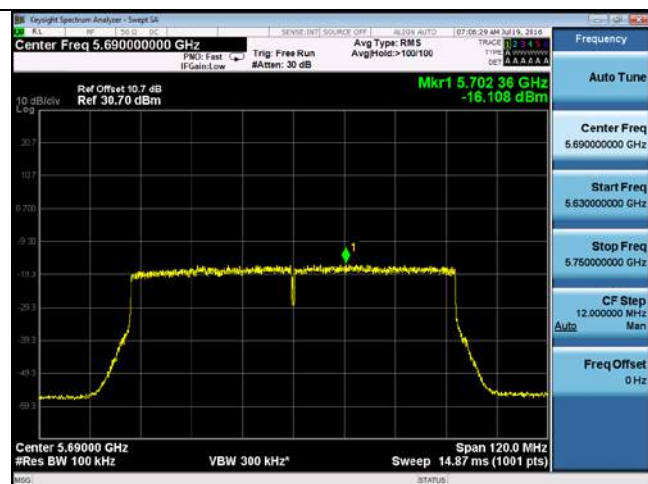
PSD-802.11ac-CROSS-5690M-chain4
