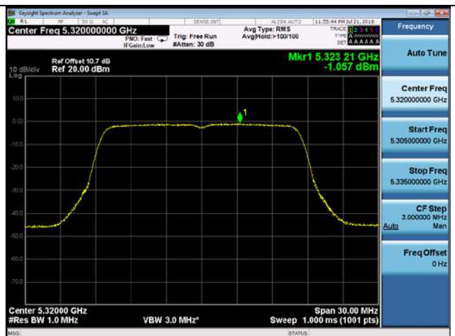
PSD-802.11a-5320M-chain2
