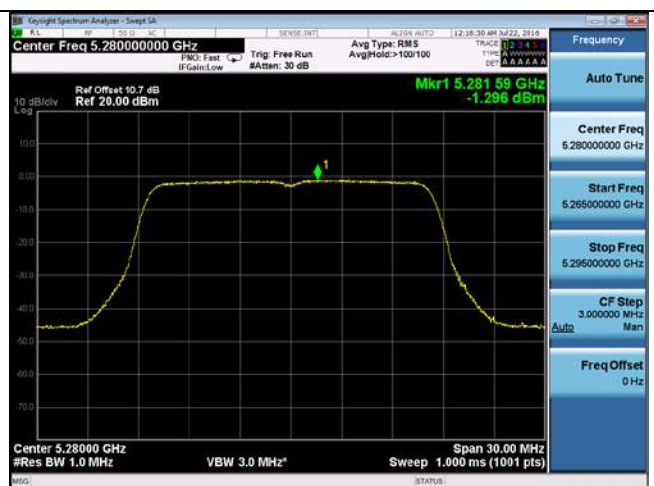
PSD-802.11a-5280M-chain4
