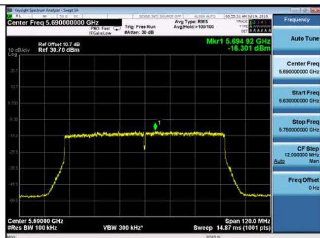
PSD-802.11ac-CROSS-5690M-chain2
