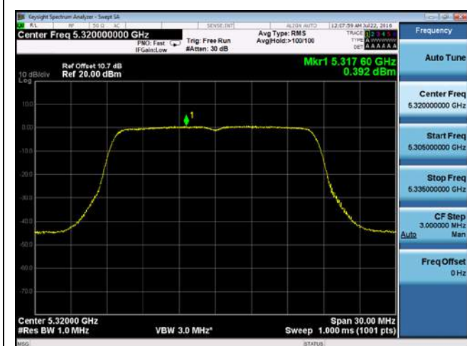
PSD-802.11a-5320M-chain3
