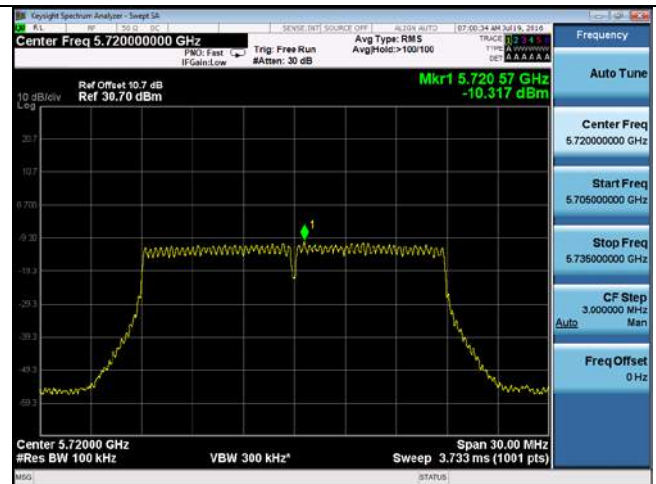
PSD-802.11n-20M-CROSS-5720M-chain2
