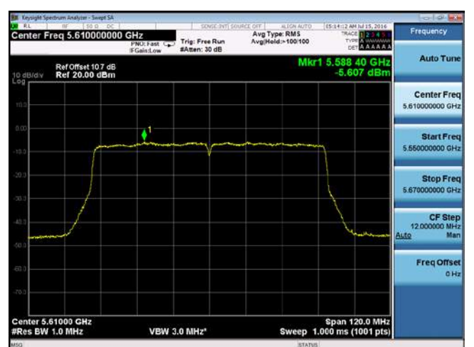
PSD-802.11ac-80M-5610M-chain2
