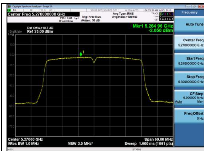
PSD-802.11n-40M-5270M-chain1
