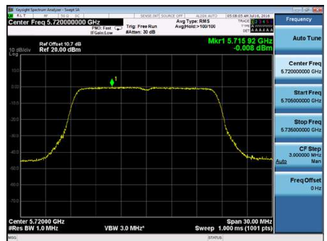
PSD-802.11a-CROSS-5720M-chain4
