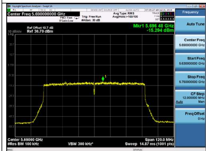
PSD-802.11ac-CROSS-5690M-chain3
