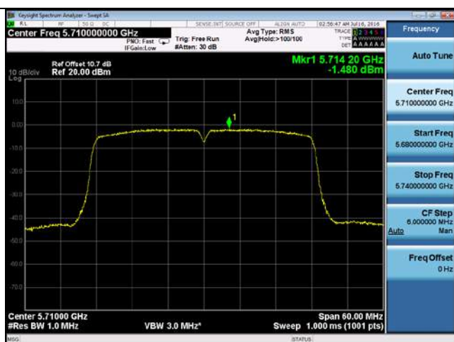
PSD-802.11n-40M-CROSS-5710M-chain3
