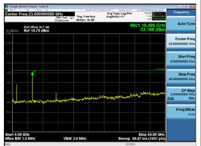
CUE-802.11n-20-5240M-chain 1(6GHz-40GHz)
