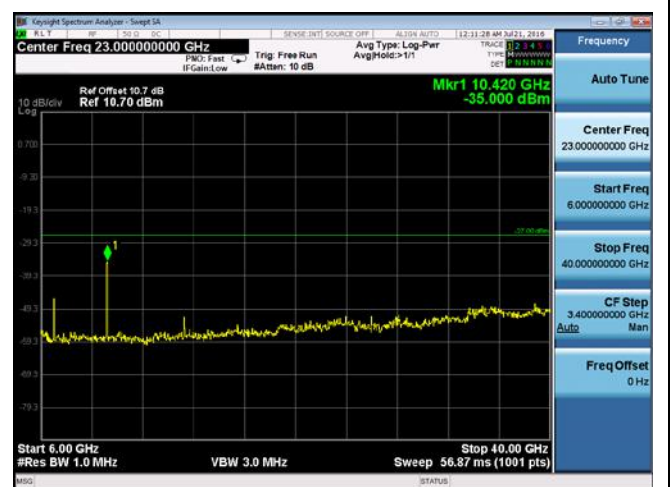
CUE-802.11a-5200M-chain2(6GHz-40GHz)
