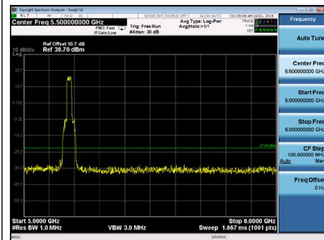
CUE-802.11n-20-5180M-chain3(5GHz-6GHz)
