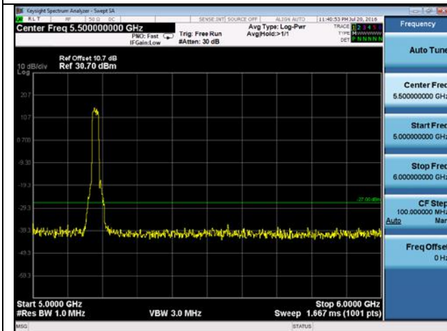
CUE-802.11n-20-5180M-chain1(5GHz-6GHz)
