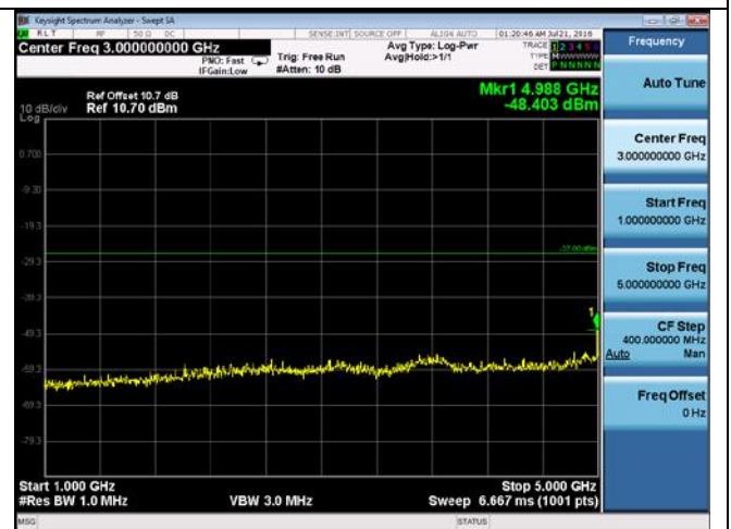
CUE-802.11n-40-5190M -chain3(1GHz-5GHz)
