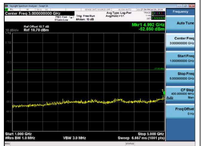
CUE-802.11a-5200M-chain1(1GHz-5GHz)
