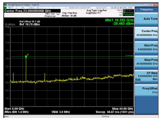
CUE-802.11n-20-5180M-chain3(6GHz-40GHz)
