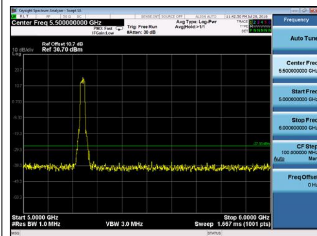
CUE-802.11n-20-5240M-chain 1(5GHz-6GHz)
