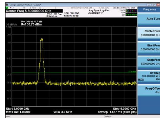
CUE-802.11n-20-5240M-chain 4(5GHz-6GHz)
