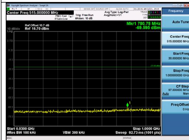
CUE-802.11n-40-5190M -chain3(30MHz-1GHz)
