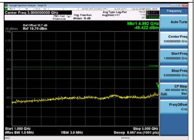
CUE-802.11a-5200M-chain2(1GHz-5GHz)
