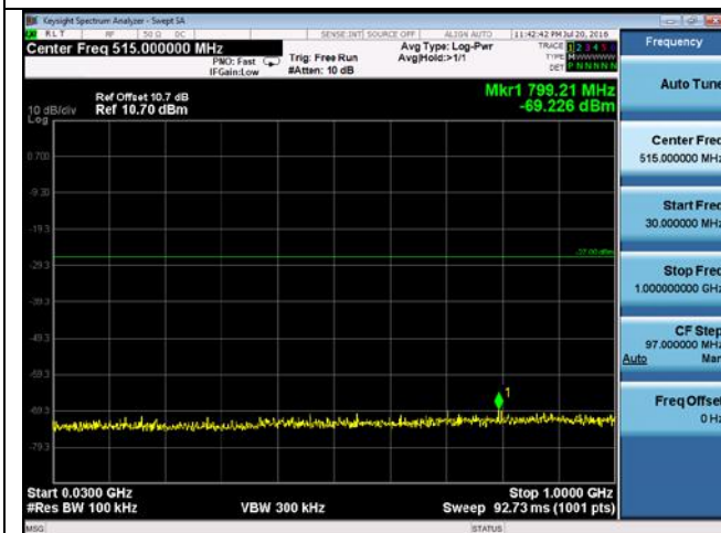
CUE-802.11n-20-5240M-chain 1(30MHz-1GHz)
