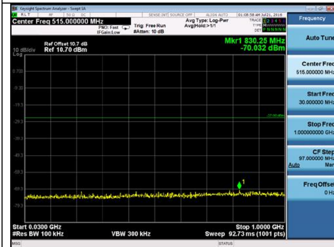
CUE-802.11n-20-5180M-chain3(30MHz-1GHz)
