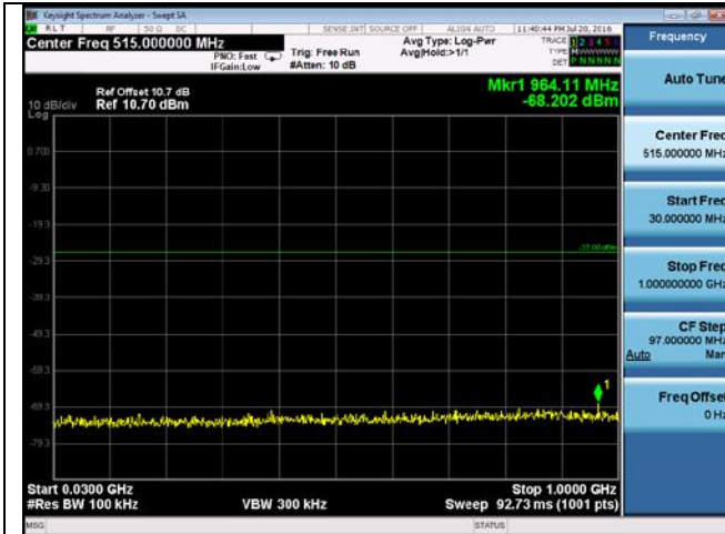
CUE-802.11n-20-5180M-chain1(30MHz-1GHz)
