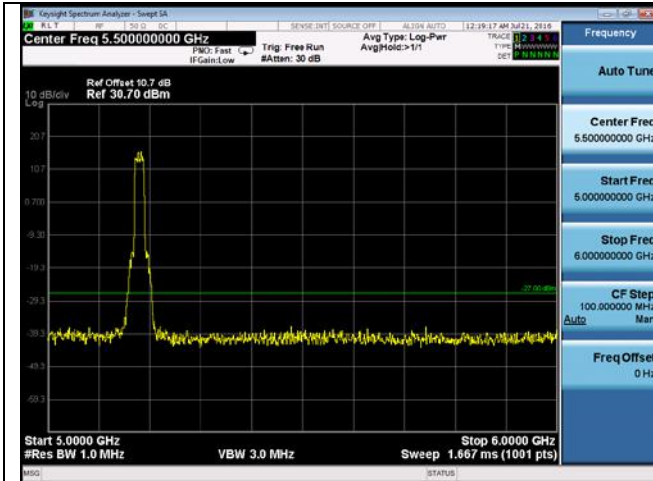
CUE-802.11n-20-5180M-chain2(5GHz-6GHz)
