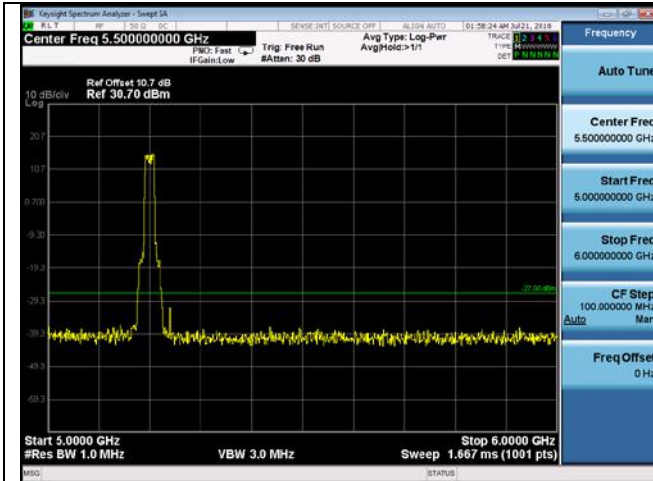
CUE-802.11n-20-5200M-chain 4(5GHz-6GHz)
