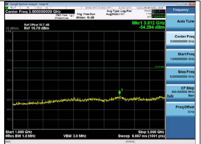
CUE-802.11a-5240M-chain 2(1GHz-5GHz)
