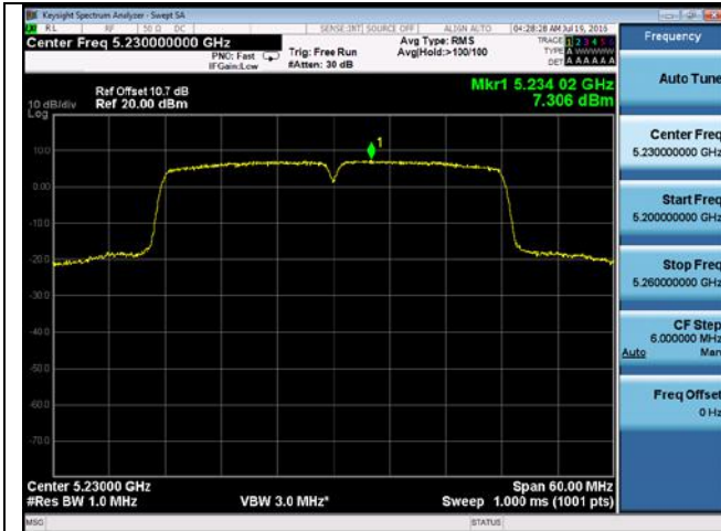
PSD-802.11n-40M-5230M-chain3
