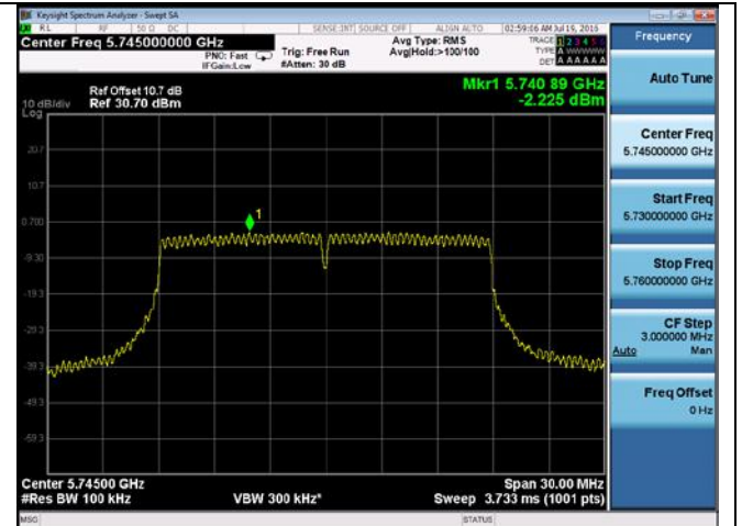
PSD-802.11n-20M-5745M-chain2
