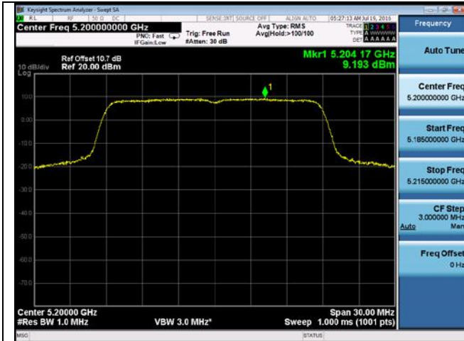
PSD-802.11n-20M-5200M-chain3
