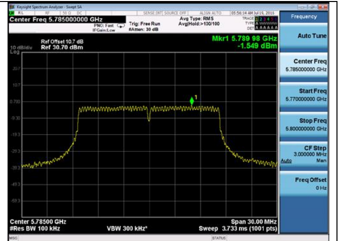
PSD-802.11a-5785M-chain4
