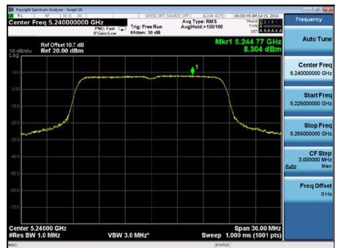
PSD-802.11a-5240M-chain4
