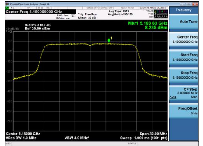
PSD-802.11n-20M-5180M-chain2
