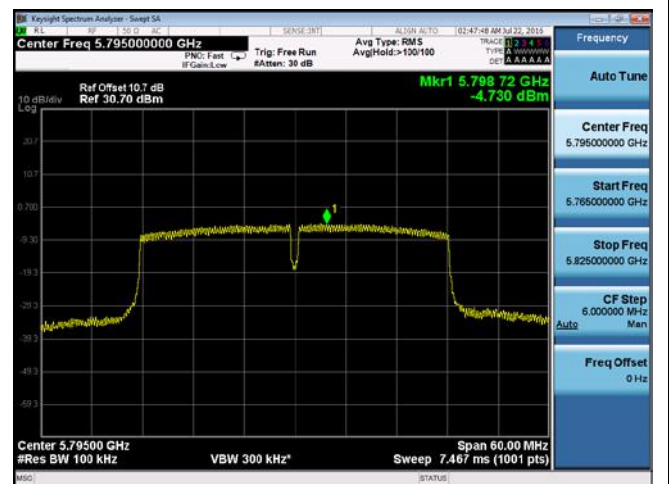
PSD-802.11n-40M-5795M-chain2
