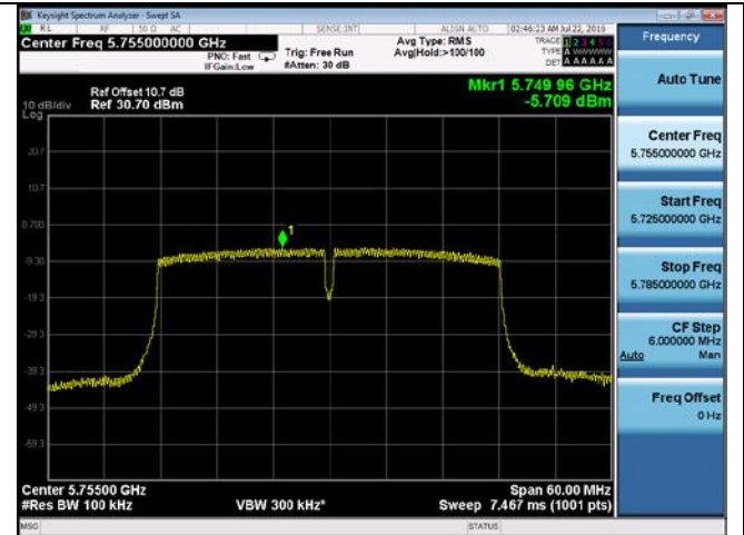
PSD-802.11n-40M-5755M-chain2
