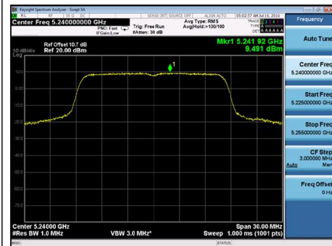
PSD-802.11a-5240M-chain3
