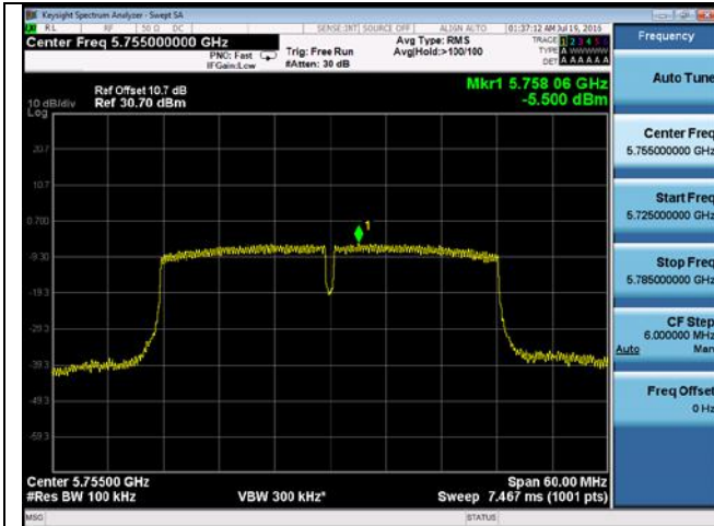
PSD-802.11n-40M-5755M-chain1
