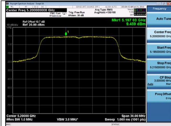
PSD-802.11a-5200M-chain3
