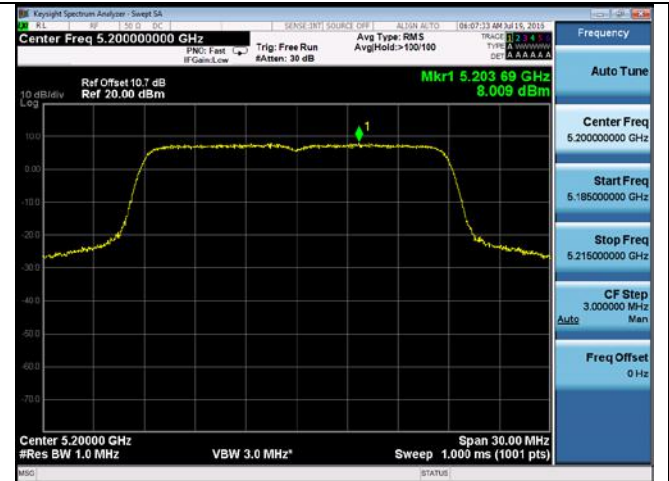
PSD-802.11n-20M-5200M-chain4
