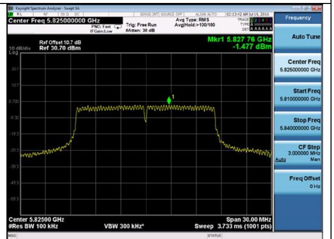
PSD-802.11a-5825M-chain2
