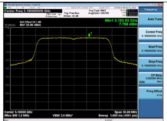
PSD-802.11a-5180M-chain4
