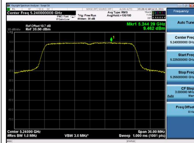
PSD-802.11n-20M-5240M-chain3
