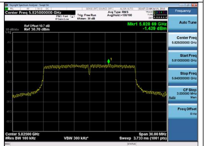
PSD-802.11n-20M-5825M-chain2
