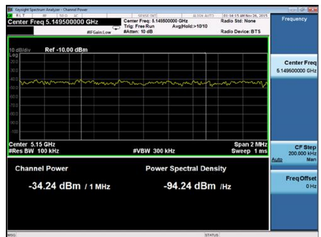
Band Edge -802.11ac-80M-5210M-chain4(Left)
