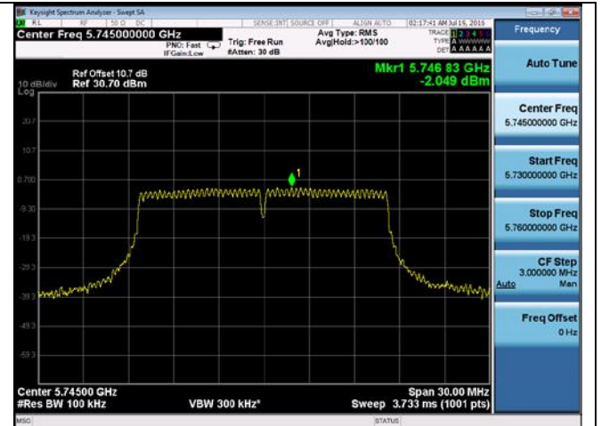
PSD-802.11a-5745M-chain2
