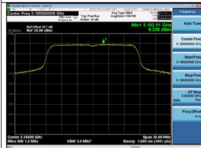
PSD-802.11a-5180M-chain3
