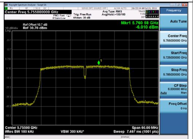
PSD-802.11n-40M-5755M-chain4
