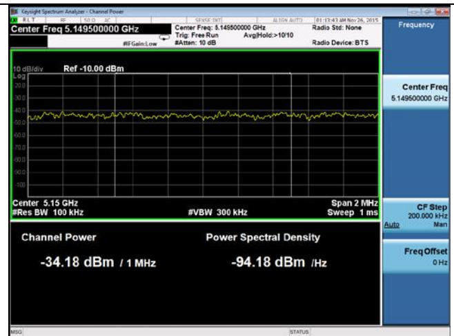
Band Edge -802.11ac-80M-5210M-chain2(Left)
