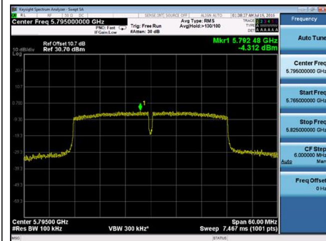
PSD-802.11n-40M-5795M-chain1
