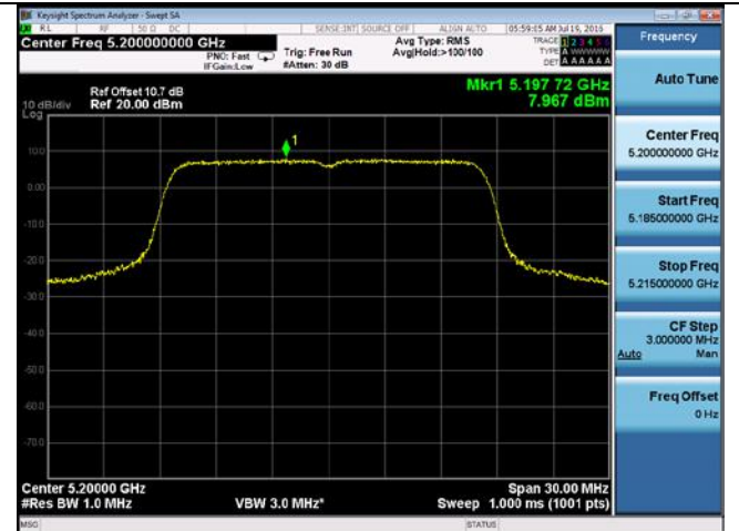
PSD-802.11a-5200M-chain4
