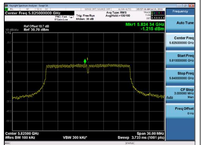
PSD-802.11a-5825M-chain4
