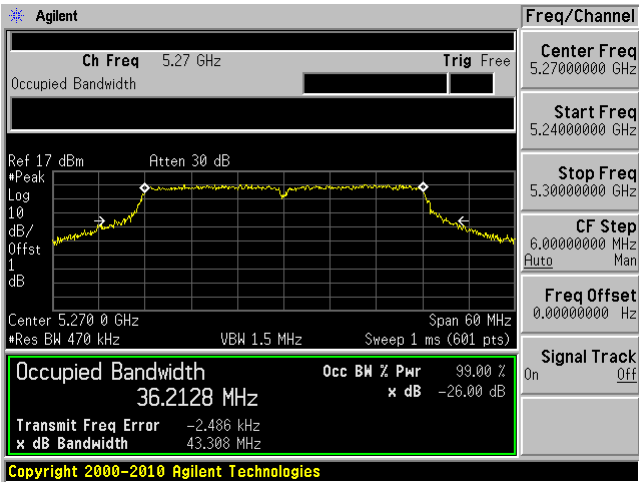
Low channel: 5270 MHz Chain 1
