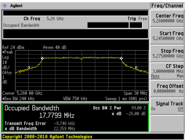
Low channel: 5260 MHz Chain 1
