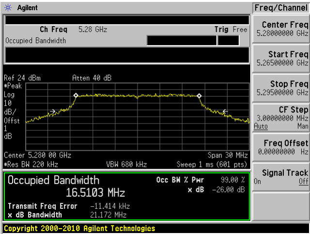
Middle channel: 5280 MHz Chain 1
