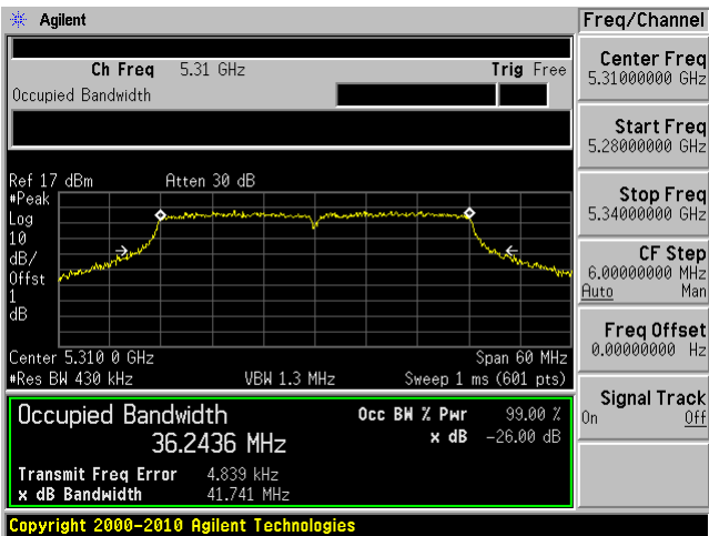
High channel: 5310 MHz Chain 1
