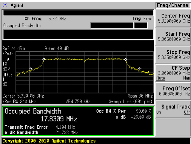
High channel: 5320 MHz Chain 1
