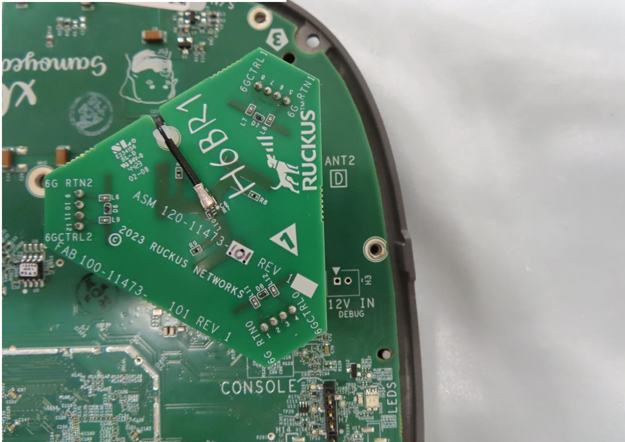
Antenna 2_WLAN 2.4GHz, 5GHz and 6GHz
