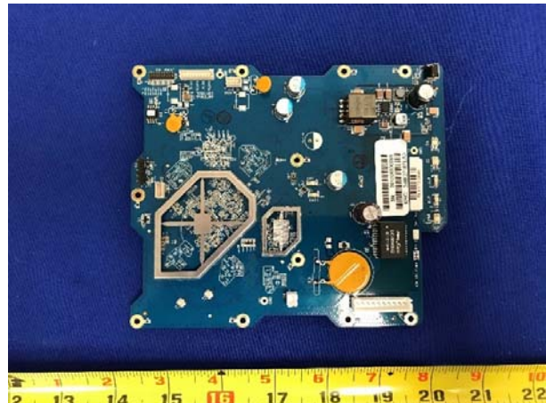
Modem Board Top View without shielding
