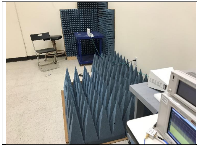
DFS setup View
