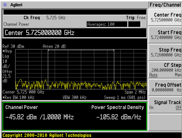
802.11 n 20, Chain 0 High Band Edge
