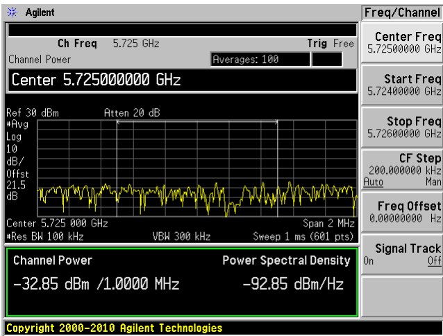
802.11 n 40, Chain 1 High Band Edge
