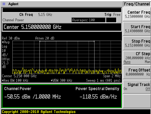
802.11 n 40, Chain 0 Low Band Edge
