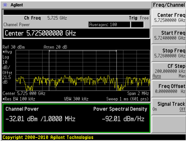
802.11 n 40, Chain 0 High Band Edge
