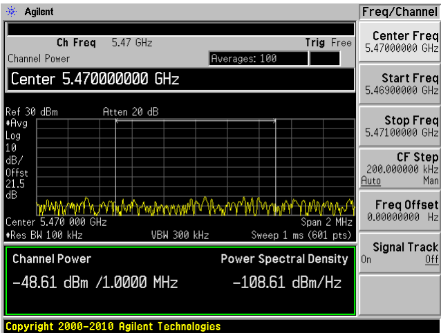
802.11 n 20, Chain 0 Low Band Edge
