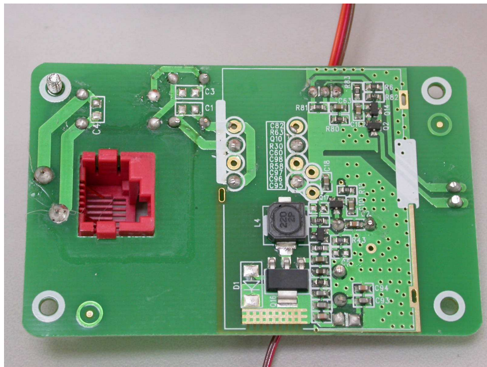
11. Rear view of PCB1
