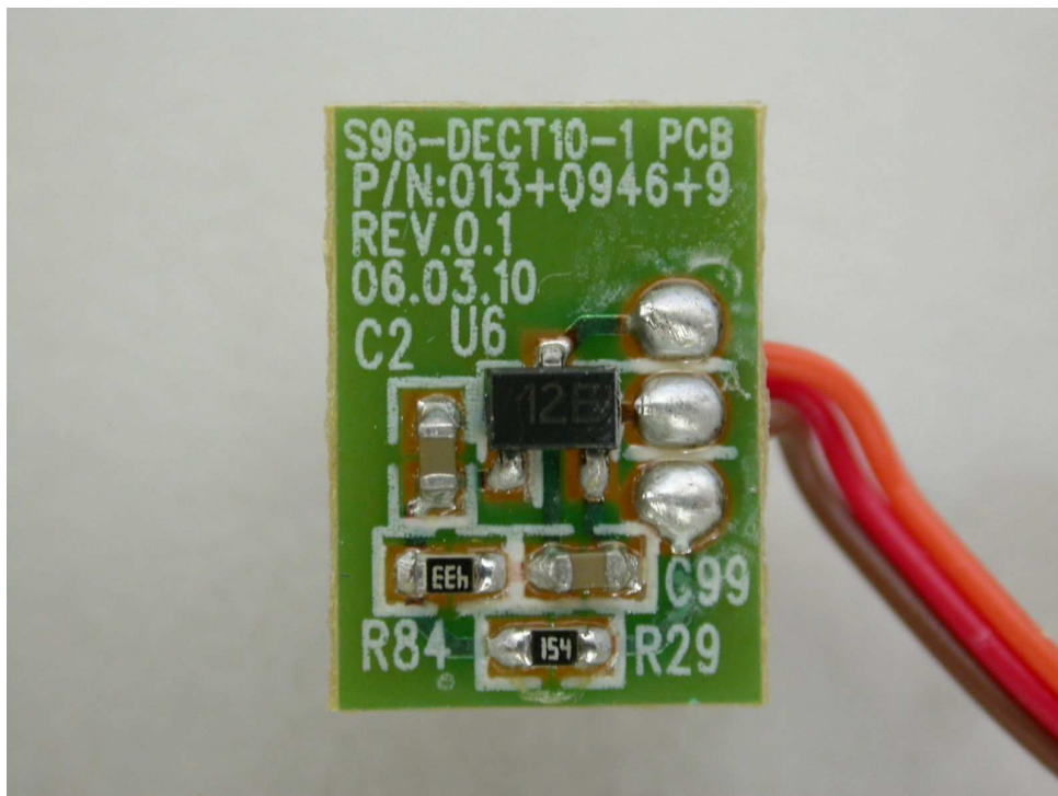
15. Rear view of PCB3
