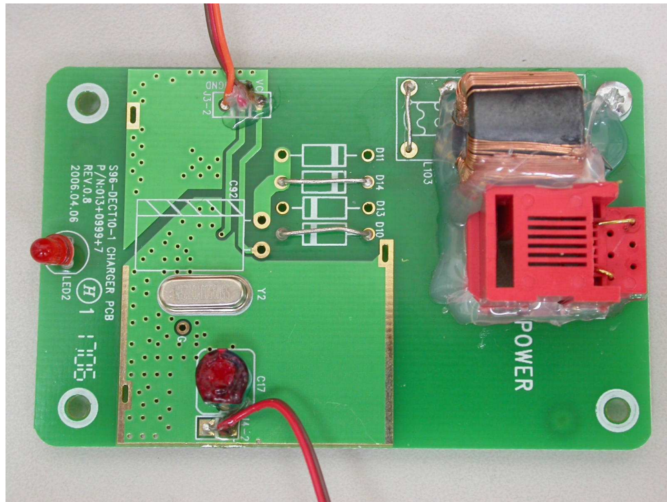
10. Front view of PCB1
