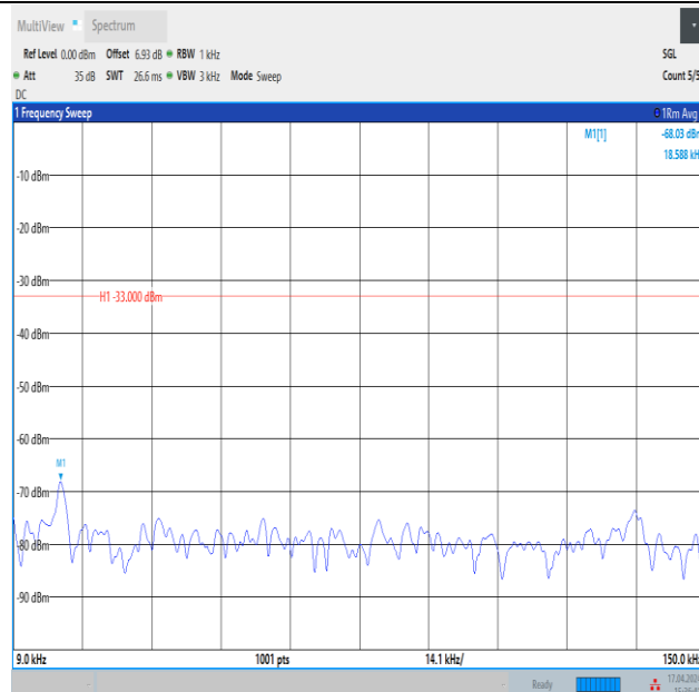
Band12_10MHz_16QAM_23095_1RB#0_0.009~0.15_0.009~0.15
