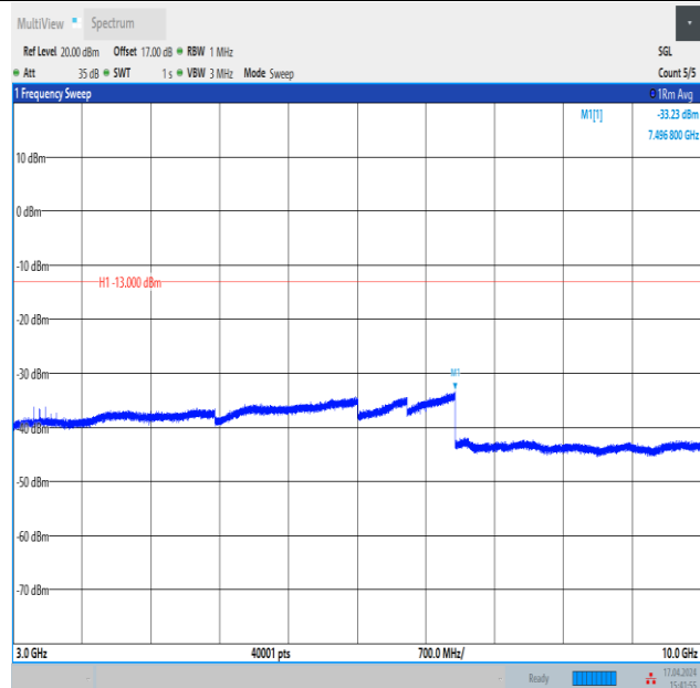
Band12_10MHz_QPSK_23130_1RB#49_3000~10000_3000~10000
