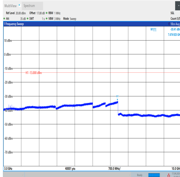
Band12_3MHz_QPSK_23165_1RB#0_3000~10000_3000~10000
