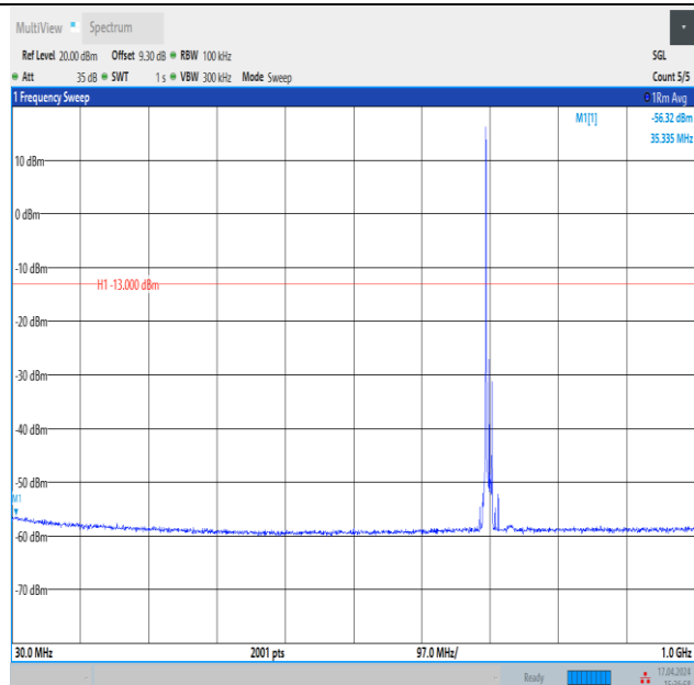
Band12_10MHz_16QAM_23095_1RB#0_30~1000_30~1000
