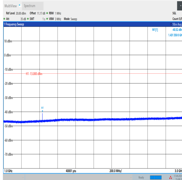
Band12_3MHz_16QAM_23165_1RB#14_1000~3000_1000~3000
