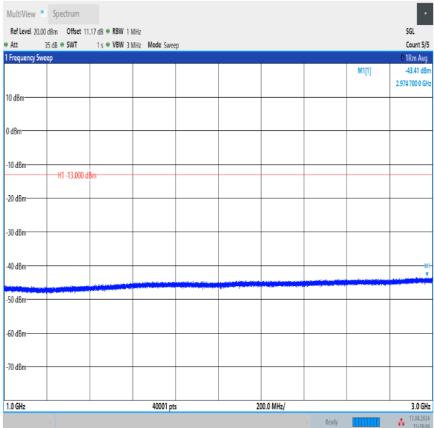
Band12_10MHz_QPSK_23095_1RB#49_1000~3000_1000~3000
