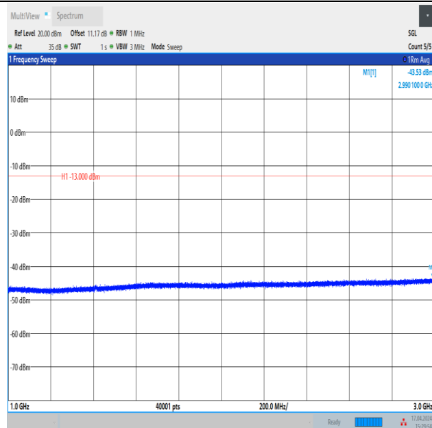
Band12_10MHz_QPSK_23060_50RB#0_1000~3000_1000~3000
