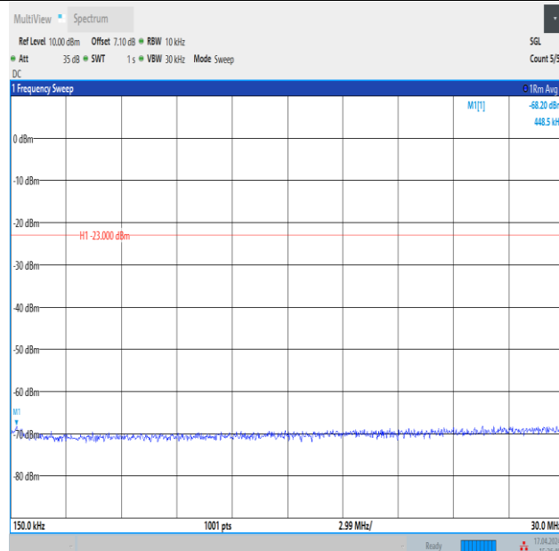
Band12_10MHz_16QAM_23095_1RB#0_0.15~30_0.15~30
