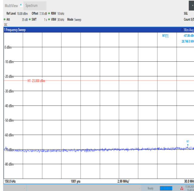
Band12_10MHz_16QAM_23130_1RB#49_0.15~30_0.15~30
