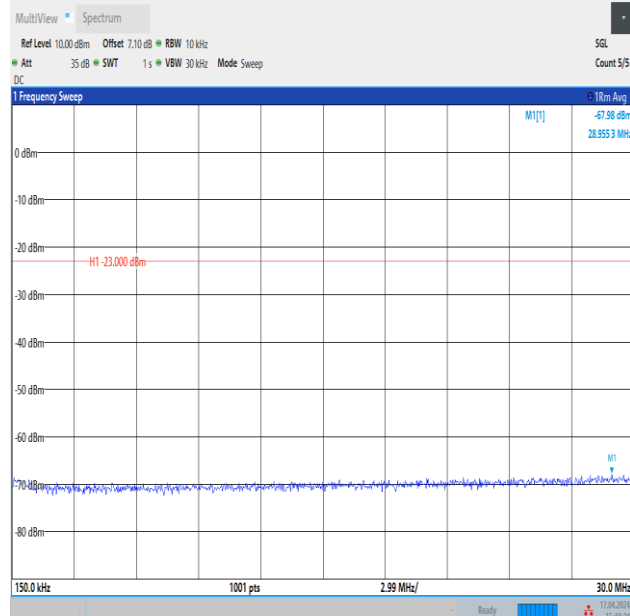
Band12_10MHz_16QAM_23130_1RB#0_0.15~30_0.15~30
