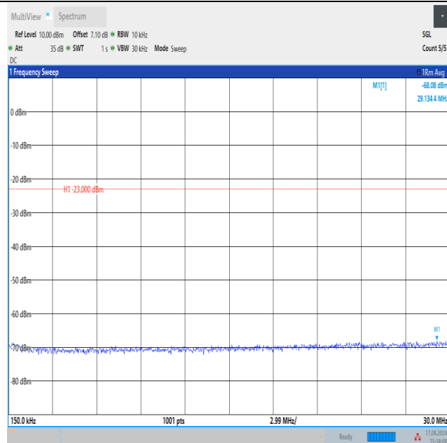
Band12_10MHz_QPSK_23060_1RB#49_0.15~30_0.15~30
