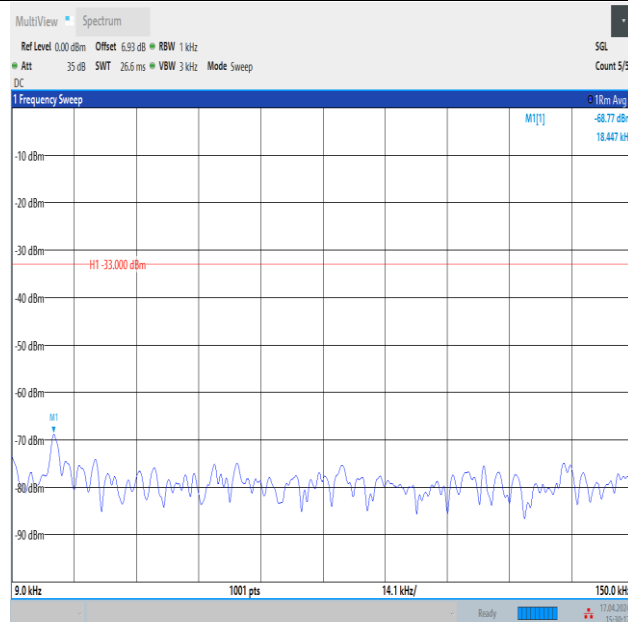
Band12_10MHz_QPSK_23095_50RB#0_0.009~0.15_0.009~0.15
