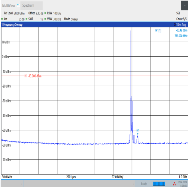
Band12_10MHz_QPSK_23095_1RB#0_30~1000_30~1000
