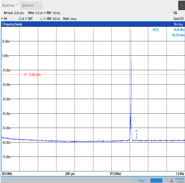
Band12_3MHz_16QAM_23165_1RB#14_30~1000_30~1000
