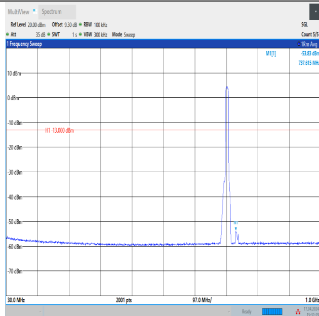
Band12_10MHz_QPSK_23130_50RB#0_30~1000_30~1000
