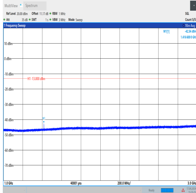
Band12_10MHz_16QAM_23060_1RB#49_1000~3000_1000~3000
