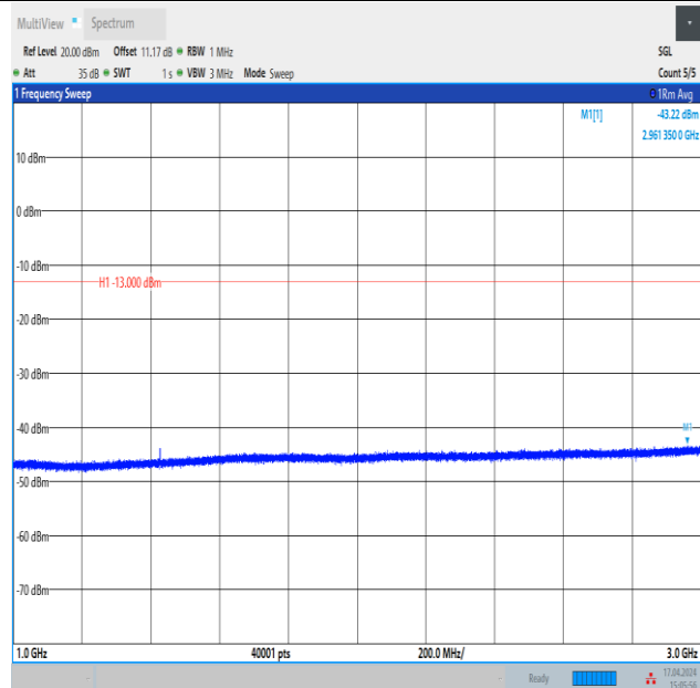
Band12_3MHz_QPSK_23165_1RB#0_1000~3000_1000~3000
