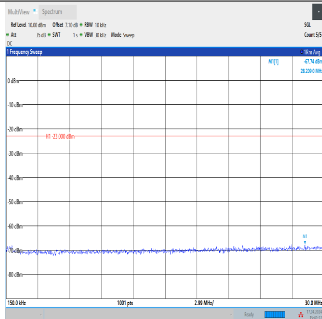
Band12_10MHz_QPSK_23130_1RB#49_0.15~30_0.15~30
