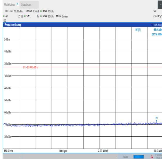
Band12_3MHz_QPSK_23165_1RB#0_0.15~30_0.15~30
