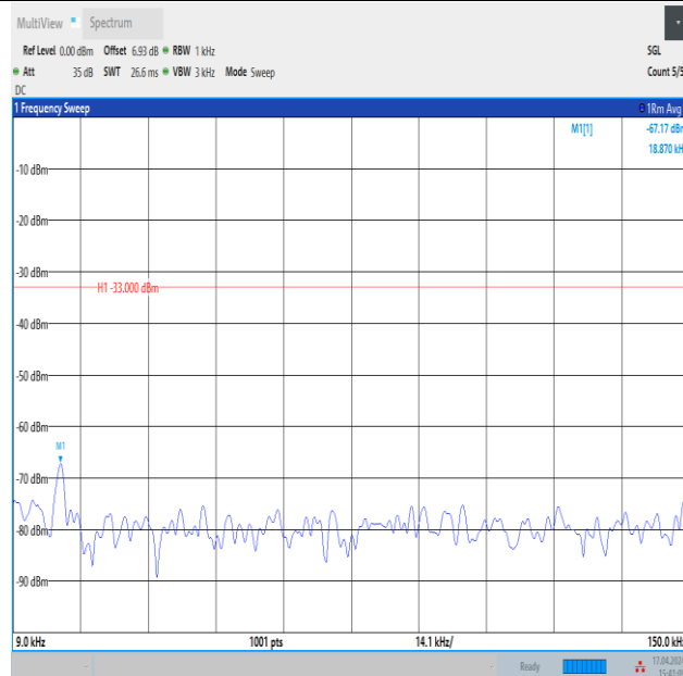
Band12_10MHz_QPSK_23130_1RB#49_0.009~0.15_0.009~0.15
