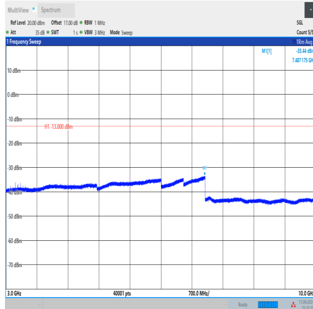
Band12_10MHz_QPSK_23130_50RB#0_3000~10000_3000~10000
