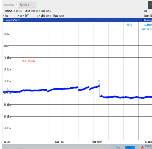
Band12_10MHz_16QAM_23130_1RB#0_3000~10000_3000~10000
