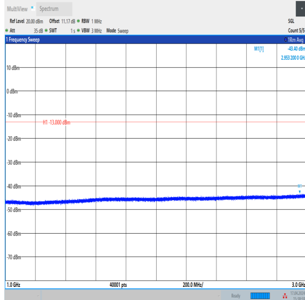
Band12_10MHz_16QAM_23095_1RB#49_1000~3000_1000~3000
