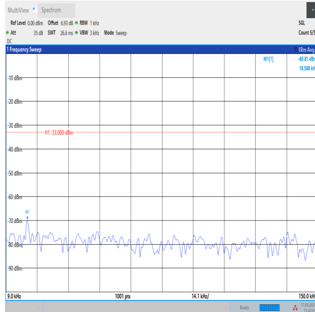
Band12_10MHz_16QAM_23130_1RB#49_0.009~0.15_0.009~0.15
