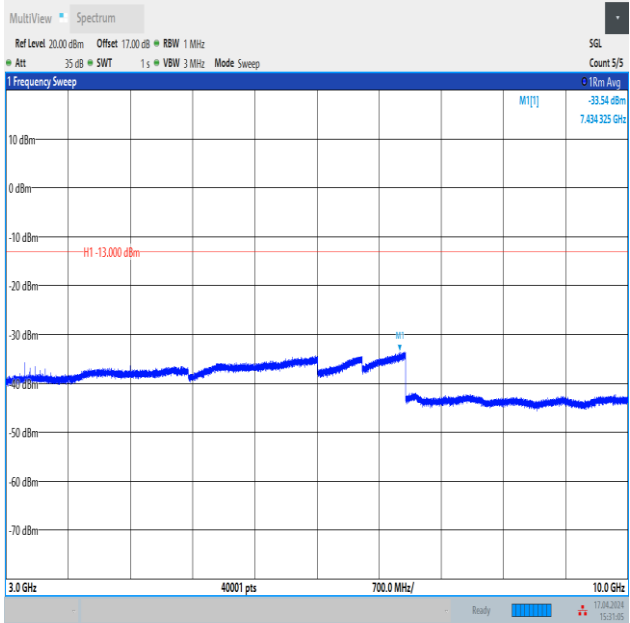
Band12_10MHz_QPSK_23095_50RB#0_3000~10000_3000~10000
