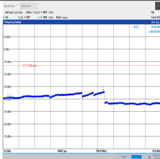
Band12_3MHz_QPSK_23165_15RB#0_3000~10000_3000~10000
