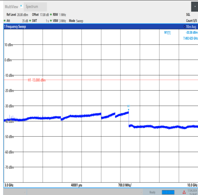
Band12_10MHz_QPSK_23060_1RB#49_3000~10000_3000~10000
