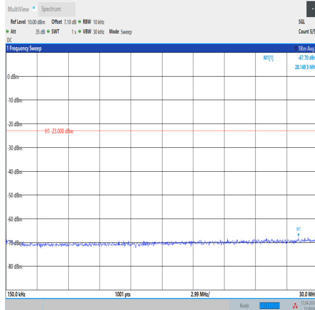
Band12_3MHz_QPSK_23165_15RB#0_0.15~30_0.15~30
