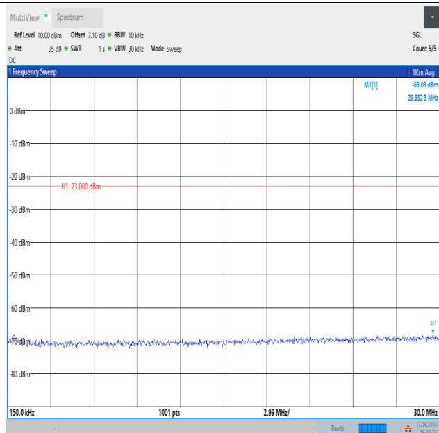
Band12_10MHz_QPSK_23095_50RB#0_0.15~30_0.15~30
