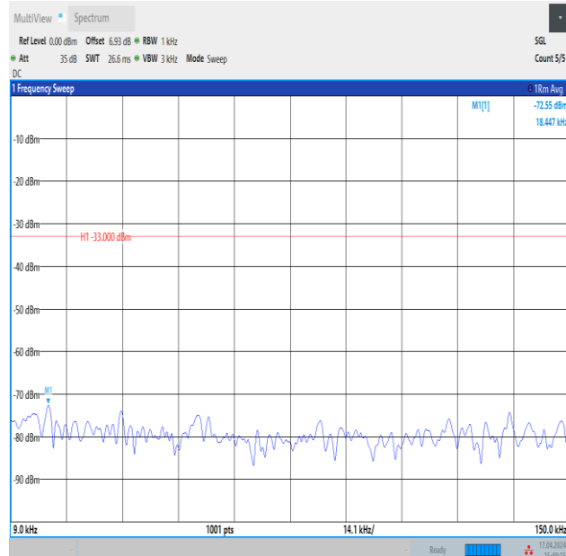
Band12_10MHz_16QAM_23130_1RB#0_0.009~0.15_0.009~0.15
