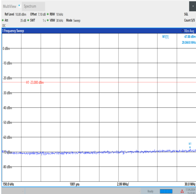
Band12_10MHz_QPSK_23095_1RB#49_0.15~30_0.15~30
