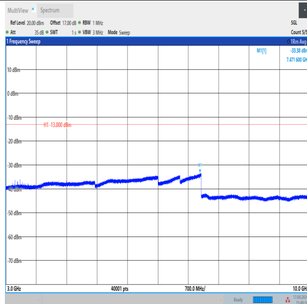
Band12_10MHz_QPSK_23130_1RB#0_3000~10000_3000~10000
