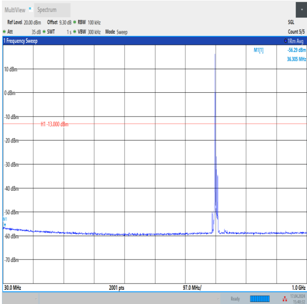
Band12_10MHz_16QAM_23130_1RB#0_30~1000_30~1000
