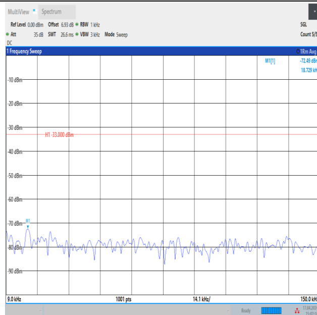
Band12_3MHz_QPSK_23165_1RB#14_0.009~0.15_0.009~0.15
