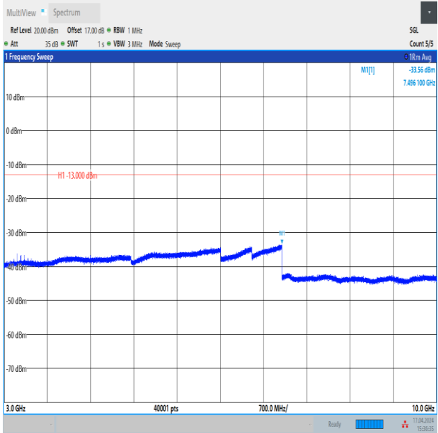
Band12_10MHz_QPSK_23095_1RB#0_3000~10000_3000~10000
