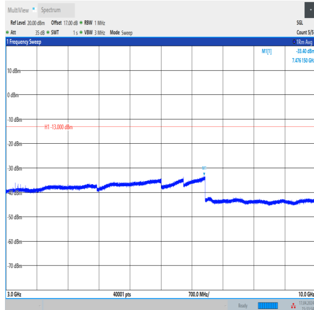
Band12_10MHz_16QAM_23060_1RB#0_3000~10000_3000~10000
