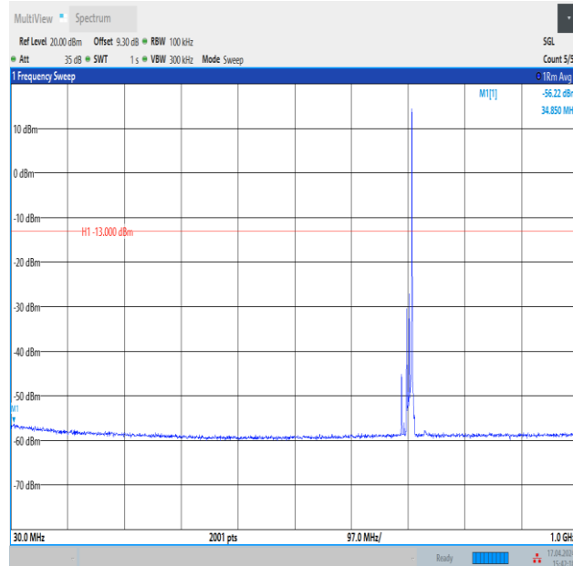
Band12_10MHz_16QAM_23130_1RB#49_30~1000_30~1000
