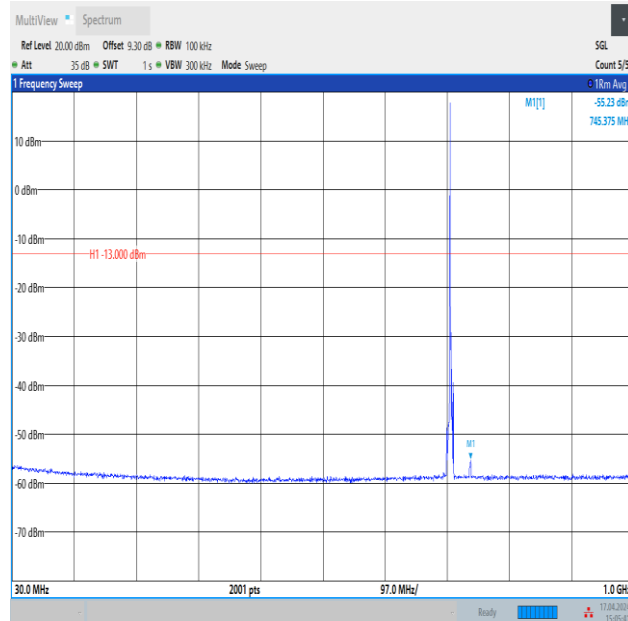
Band12_3MHz_QPSK_23165_1RB#0_30~1000_30~1000
