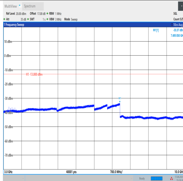
Band12_3MHz_16QAM_23165_15RB#0_3000~10000_3000~10000
