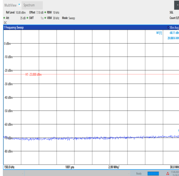
Band12_10MHz_QPSK_23060_50RB#0_0.15~30_0.15~30
