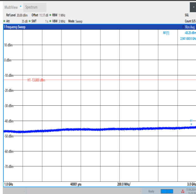
Band12_10MHz_16QAM_23060_1RB#0_1000~3000_1000~3000
