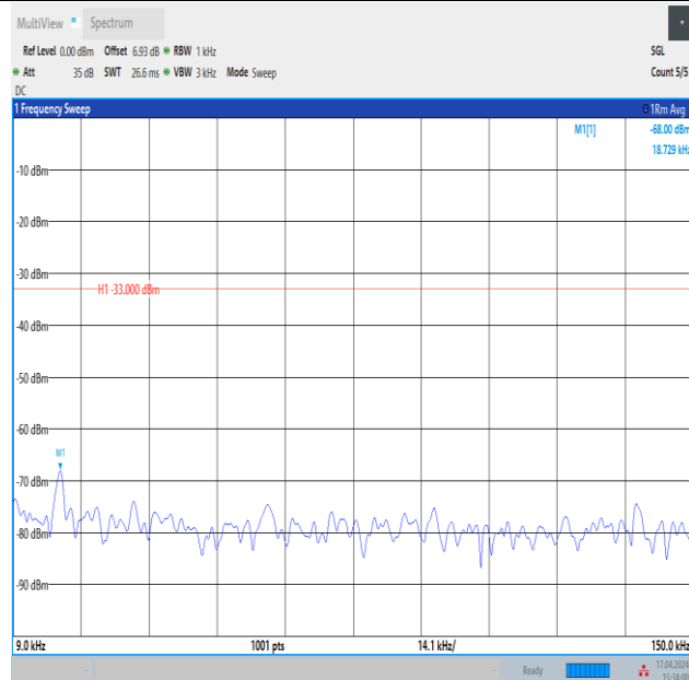
Band12_10MHz_QPSK_23060_1RB#49_0.009~0.15_0.009~0.15
