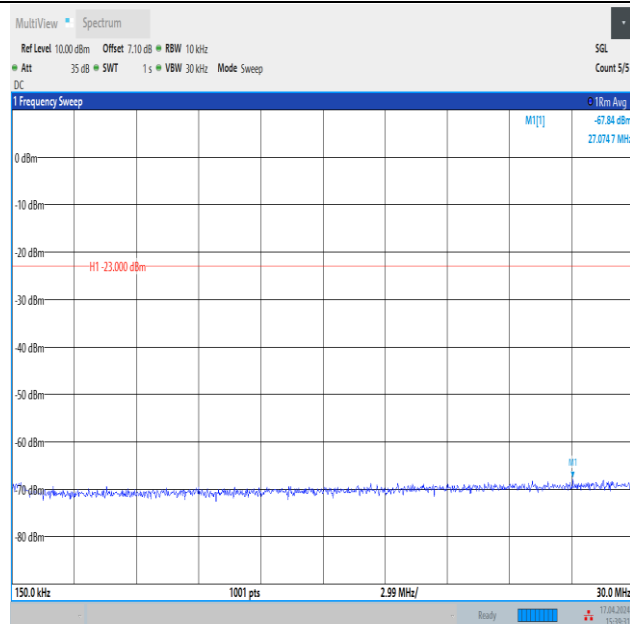
Band12_10MHz_QPSK_23130_1RB#0_0.15~30_0.15~30
