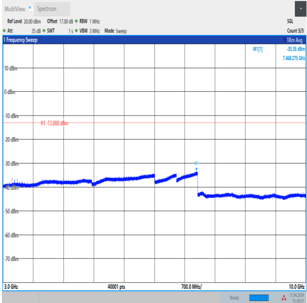
Band12_10MHz_QPSK_23095_1RB#49_3000~10000_3000~10000
