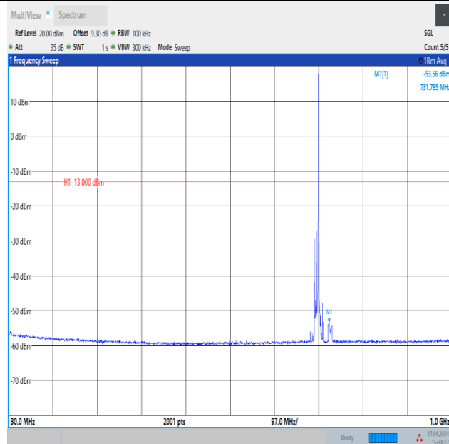
Band12_10MHz_QPSK_23060_1RB#49_30~1000_30~1000
