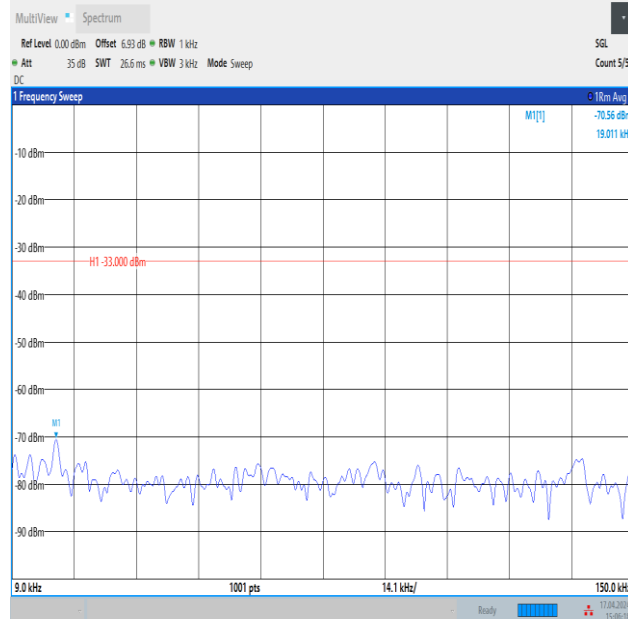
Band12_3MHz_16QAM_23165_1RB#0_0.009~0.15_0.009~0.15
