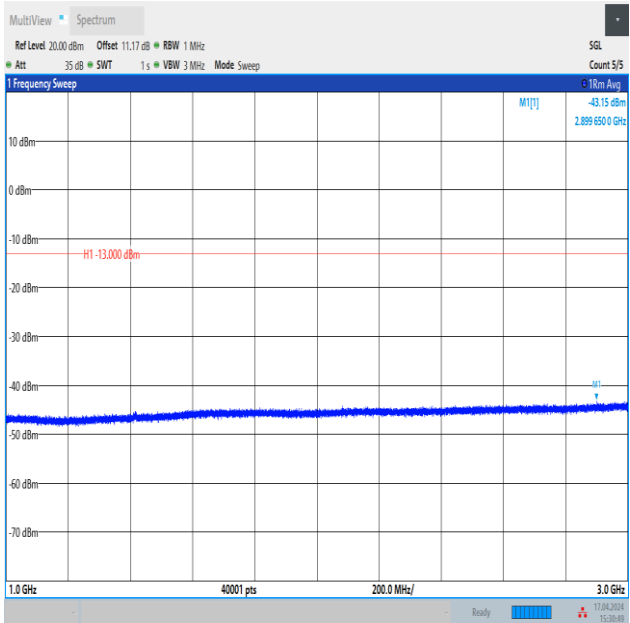
Band12_10MHz_QPSK_23095_50RB#0_1000~3000_1000~3000
