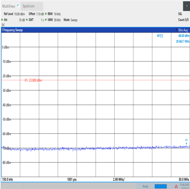
Band12_10MHz_QPSK_23060_1RB#0_0.15~30_0.15~30
