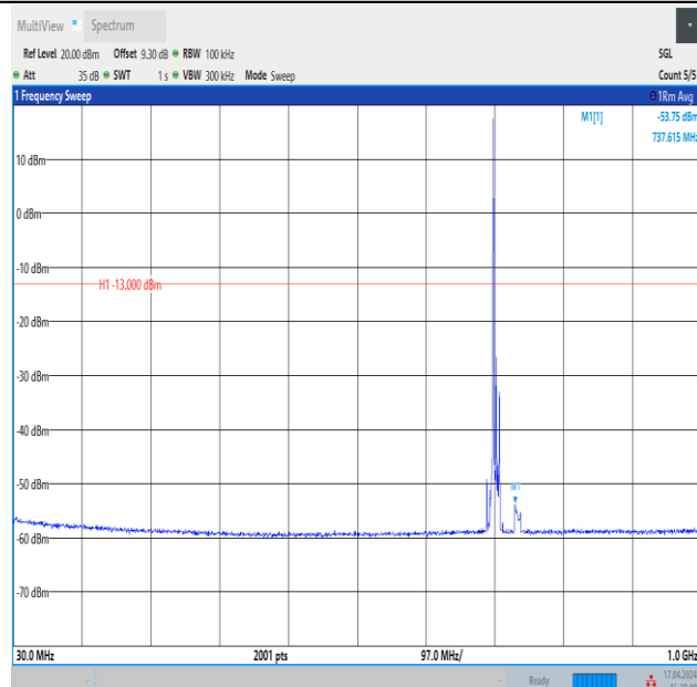
Band12_10MHz_QPSK_23130_1RB#0_30~1000_30~1000
