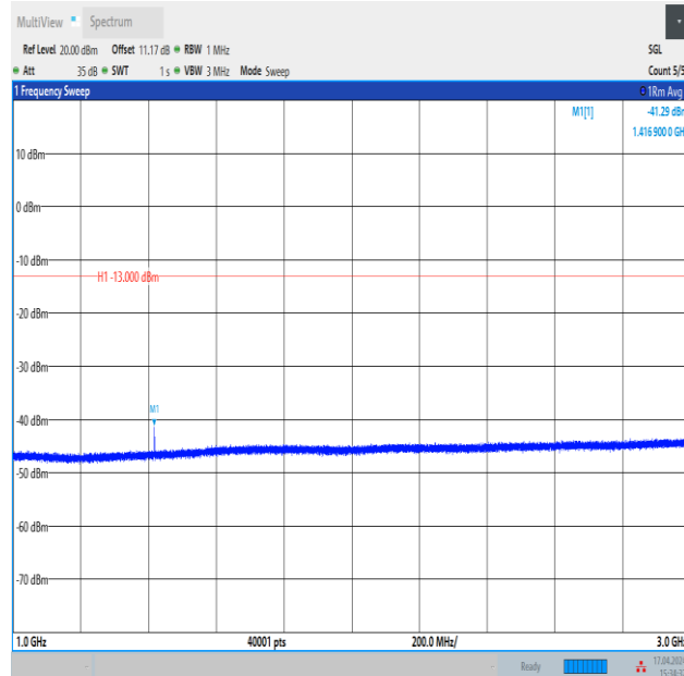
Band12_10MHz_QPSK_23060_1RB#49_1000~3000_1000~3000
