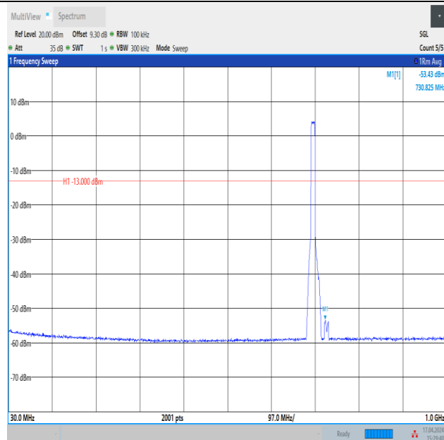
Band12_10MHz_QPSK_23060_50RB#0_30~1000_30~1000
