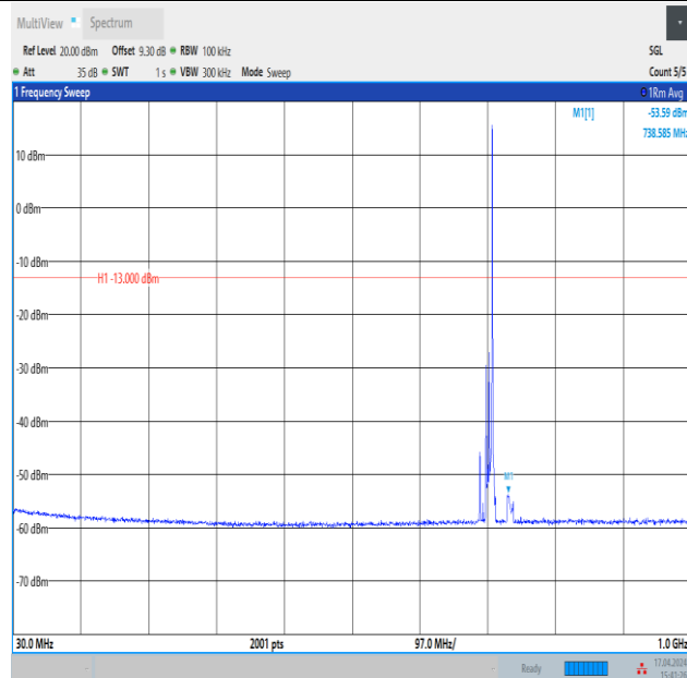
Band12_10MHz_QPSK_23130_1RB#49_30~1000_30~1000
