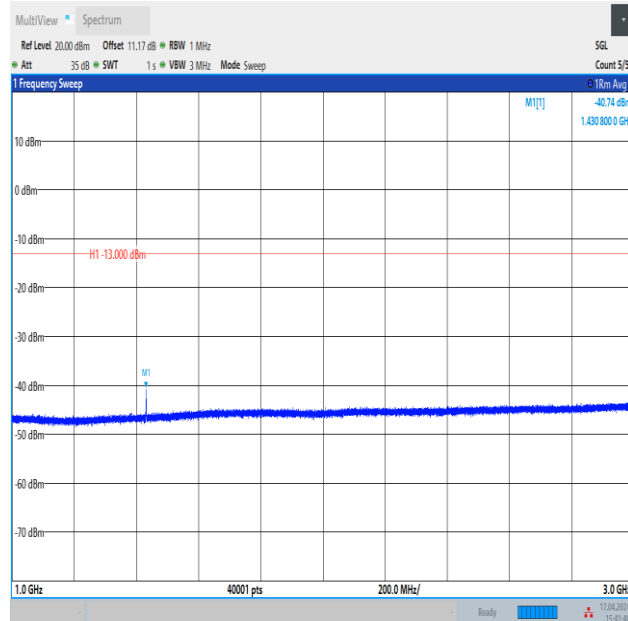
Band12_10MHz_QPSK_23130_1RB#49_1000~3000_1000~3000
