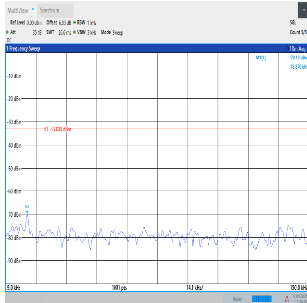
Band12_3MHz_16QAM_23165_15RB#0_0.009~0.15_0.009~0.15
