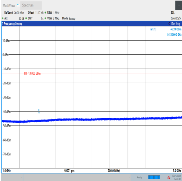
Band12_10MHz_16QAM_23130_1RB#0_1000~3000_1000~3000
