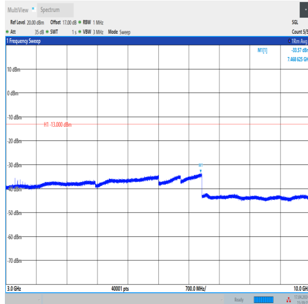
Band12_10MHz_16QAM_23095_1RB#49_3000~10000_3000~10000
