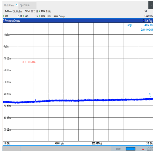
Band12_3MHz_QPSK_23165_15RB#0_1000~3000_1000~3000
