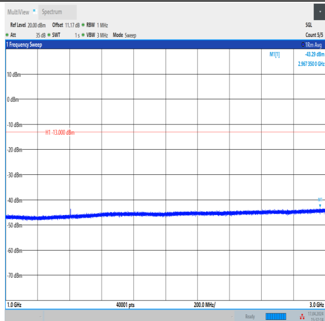
Band12_10MHz_16QAM_23095_1RB#0_1000~3000_1000~3000
