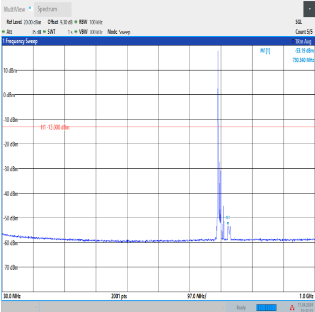
Band12_10MHz_QPSK_23060_1RB#0_30~1000_30~1000
