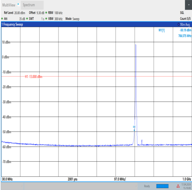
Band12_3MHz_16QAM_23165_15RB#0_30~1000_30~1000
