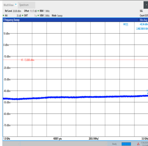
Band12_10MHz_QPSK_23130_50RB#0_1000~3000_1000~3000
