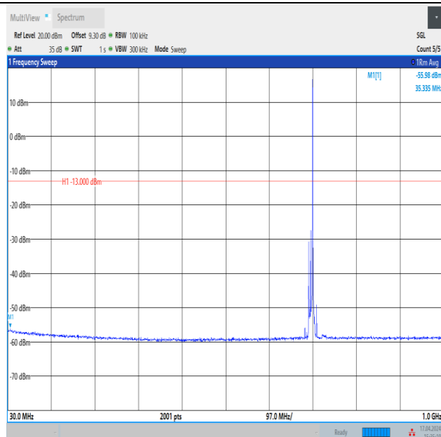
Band12_10MHz_16QAM_23060_1RB#49_30~1000_30~1000
