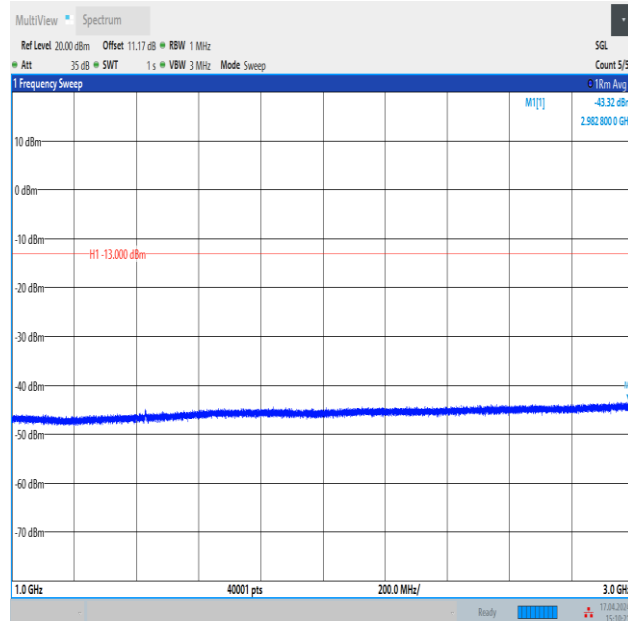
Band12_3MHz_16QAM_23165_15RB#0_1000~3000_1000~3000
