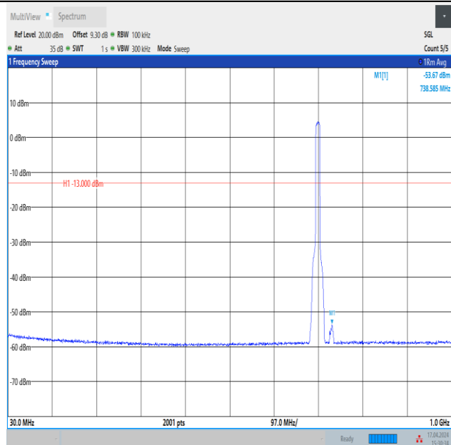
Band12_10MHz_QPSK_23095_50RB#0_30~1000_30~1000
