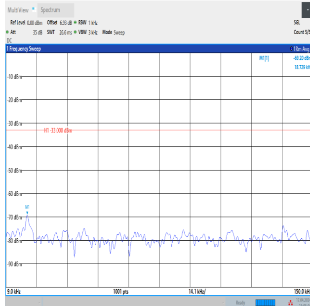
Band12_3MHz_QPSK_23165_1RB#0_0.009~0.15_0.009~0.15
