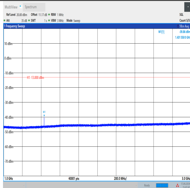
Band12_3MHz_QPSK_23165_1RB#14_1000~3000_1000~3000
