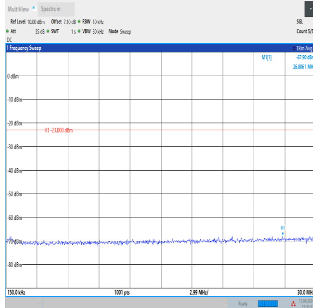
Band12_10MHz_QPSK_23130_50RB#0_0.15~30_0.15~30
