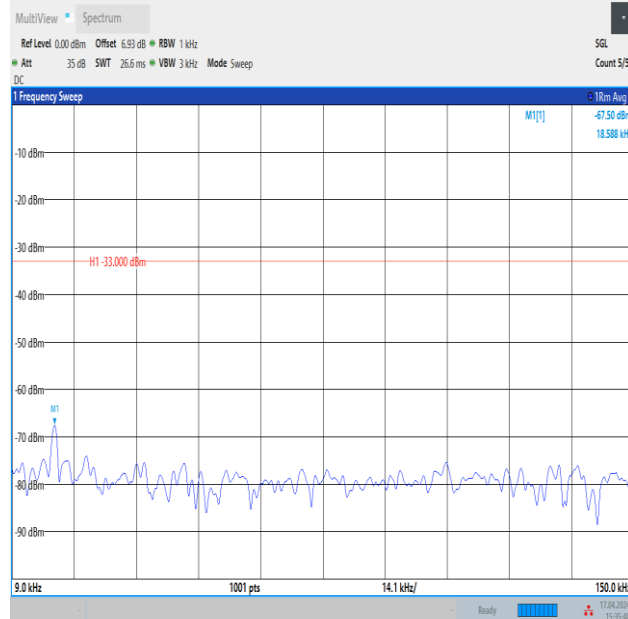
Band12_10MHz_QPSK_23095_1RB#0_0.009~0.15_0.009~0.15
