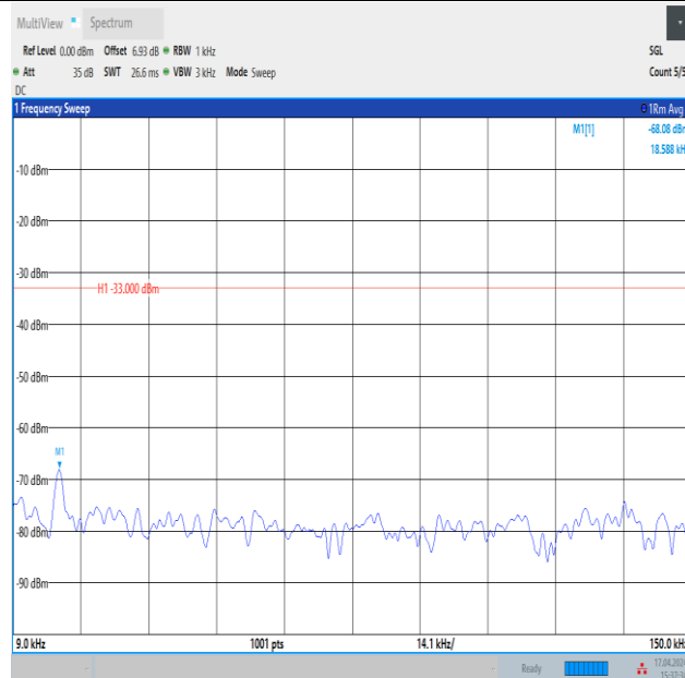
Band12_10MHz_QPSK_23095_1RB#49_0.009~0.15_0.009~0.15
