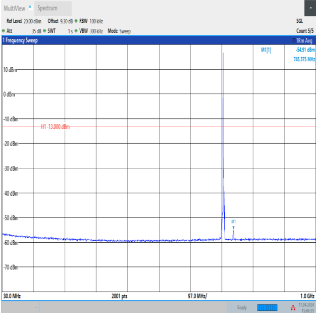
Band12_3MHz_16QAM_23165_1RB#0_30~1000_30~1000
