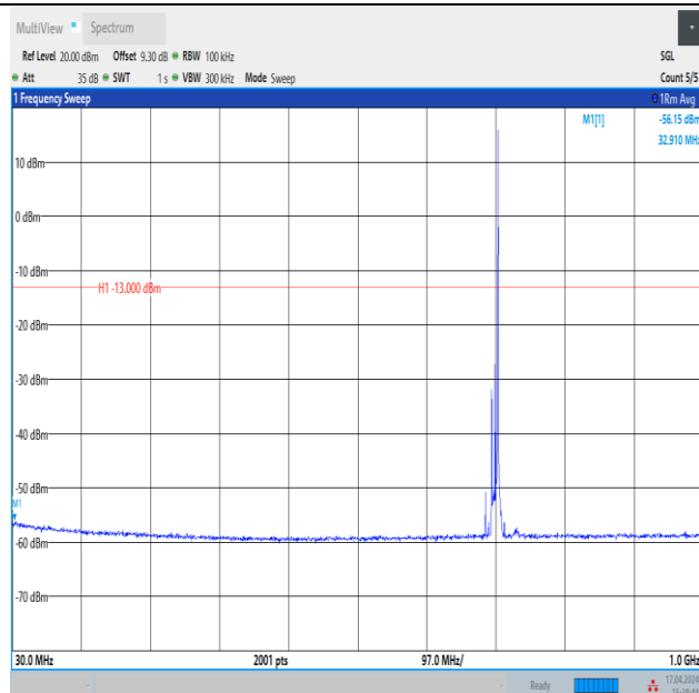
Band12_10MHz_16QAM_23095_1RB#49_30~1000_30~1000
