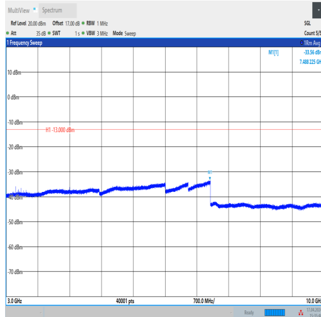
Band12_10MHz_16QAM_23060_1RB#49_3000~10000_3000~10000
