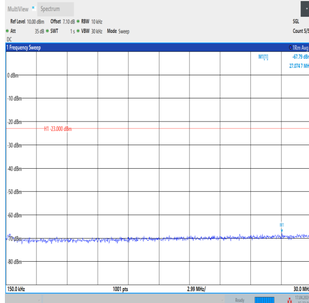
Band12_10MHz_16QAM_23060_1RB#0_0.15~30_0.15~30
