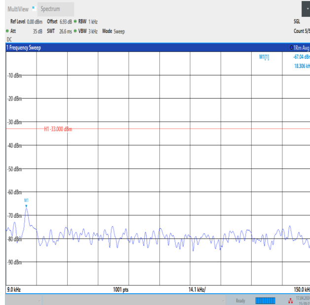
Band12_10MHz_QPSK_23130_1RB#0_0.009~0.15_0.009~0.15
