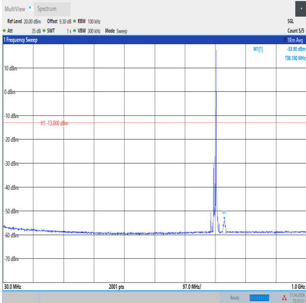
Band12_10MHz_QPSK_23095_1RB#49_30~1000_30~1000
