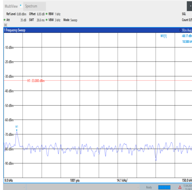
Band12_10MHz_16QAM_23060_1RB#49_0.009~0.15_0.009~0.15
