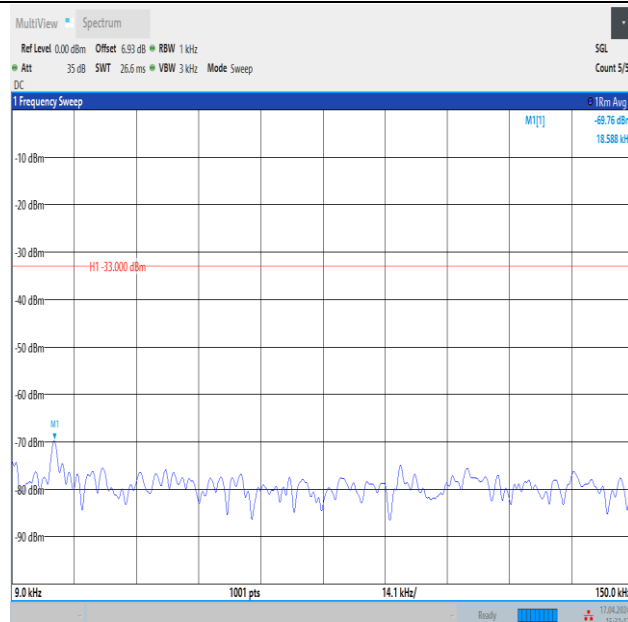
Band12_10MHz_QPSK_23130_50RB#0_0.009~0.15_0.009~0.15
