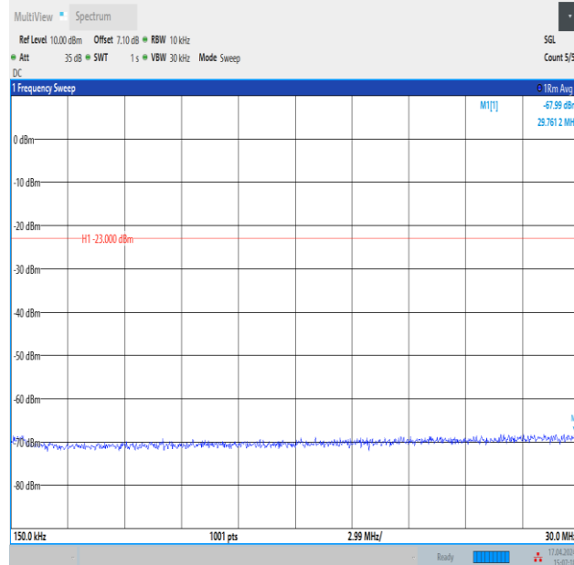
Band12_3MHz_QPSK_23165_1RB#14_0.15~30_0.15~30
