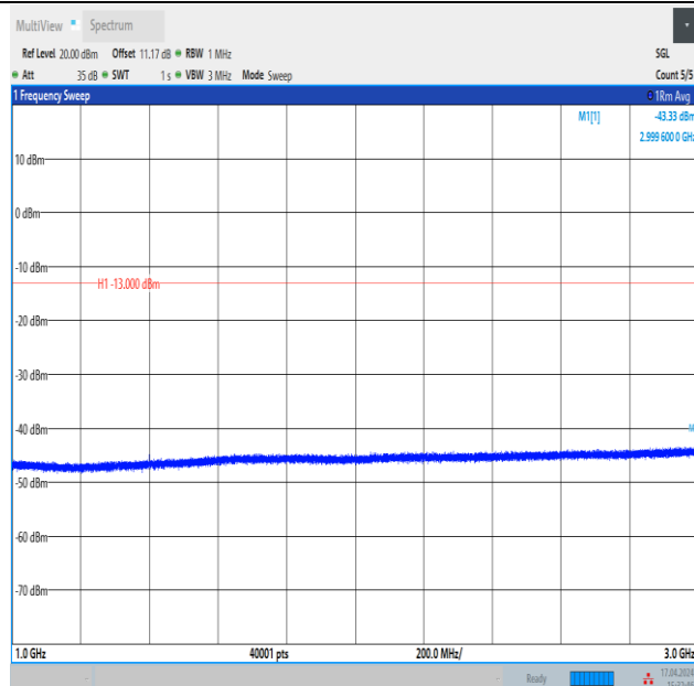
Band12_10MHz_QPSK_23060_1RB#0_1000~3000_1000~3000
