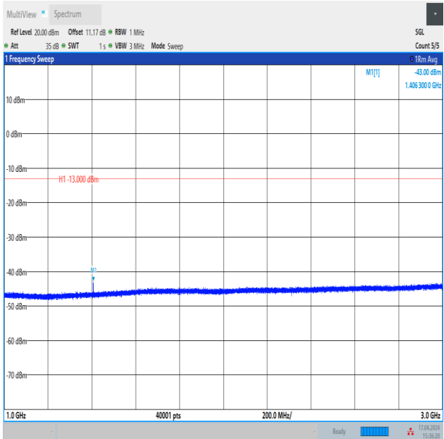
Band12_10MHz_QPSK_23095_1RB#0_1000~3000_1000~3000
