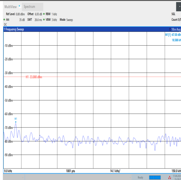
Band12_10MHz_QPSK_23060_50RB#0_0.009~0.15_0.009~0.15
