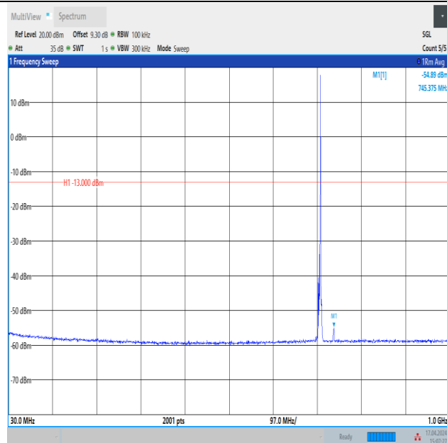
Band12_3MHz_QPSK_23165_1RB#14_30~1000_30~1000
