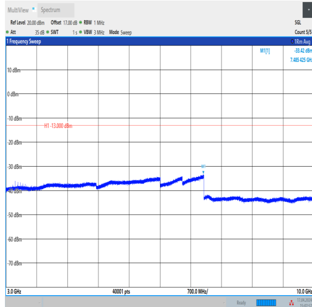
Band12_3MHz_QPSK_23165_1RB#14_3000~10000_3000~10000
