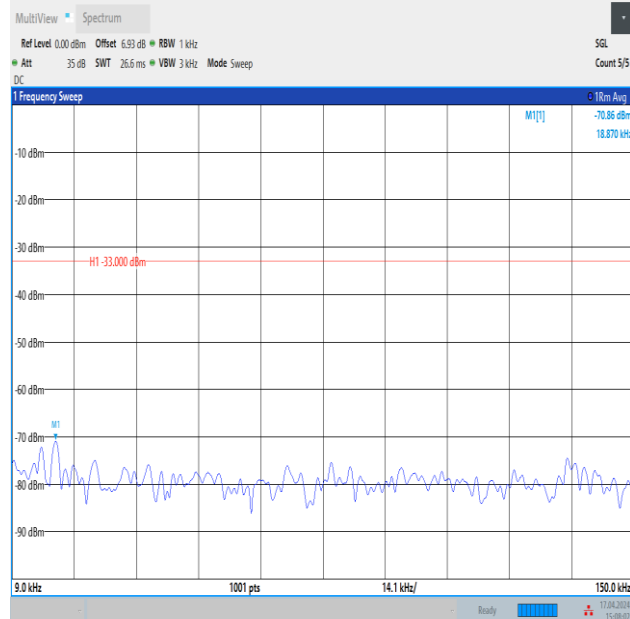
Band12_3MHz_16QAM_23165_1RB#14_0.009~0.15_0.009~0.15
