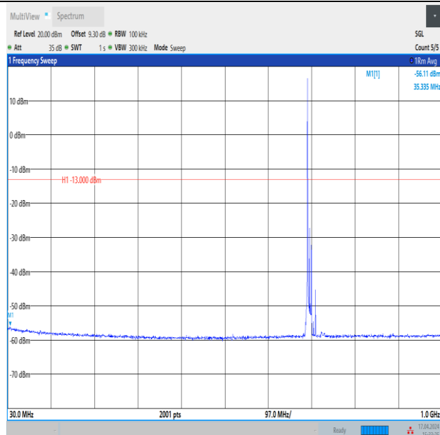
Band12_10MHz_16QAM_23060_1RB#0_30~1000_30~1000
