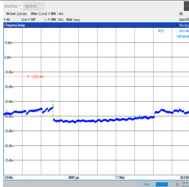
Band4_3MHz_16QAM_20175_1RB#14_3000~20000_3000~20000
