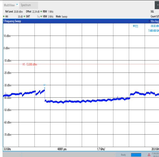
Band4_3MHz_16QAM_20385_1RB#14_3000~20000_3000~20000
