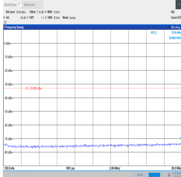
Band4_3MHz_16QAM_19965_1RB#14_0.15~30_0.15~30
