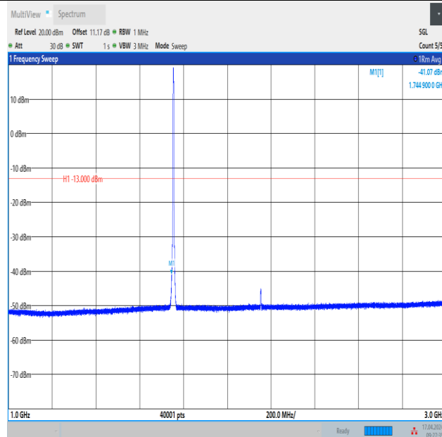
Band4_3MHz_QPSK_20385_15RB#0_1000~3000_1000~3000
