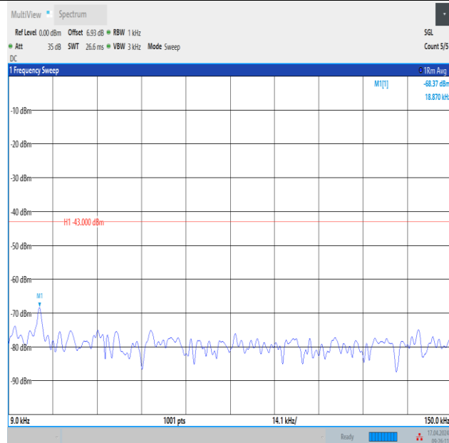
Band4_3MHz_16QAM_20385_1RB#14_0.009~0.15_0.009~0.15
