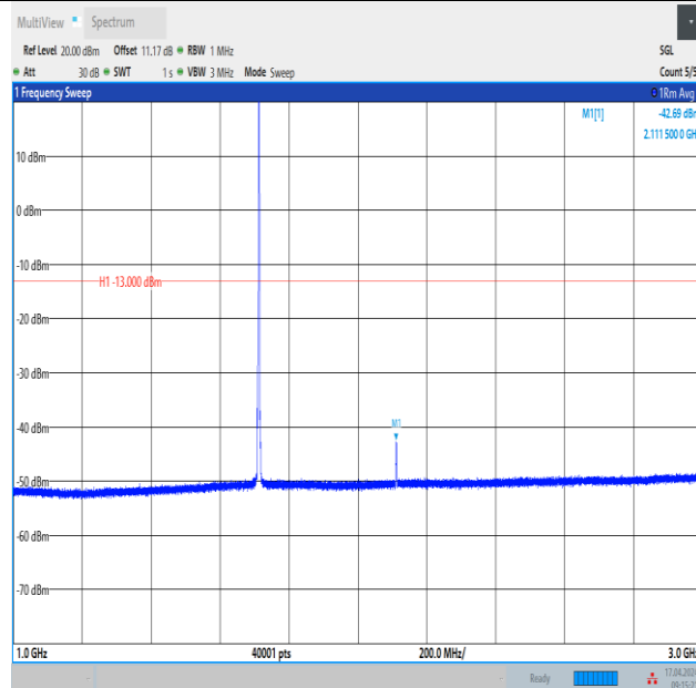
Band4_3MHz_QPSK_19965_1RB#14_1000~3000_1000~3000
