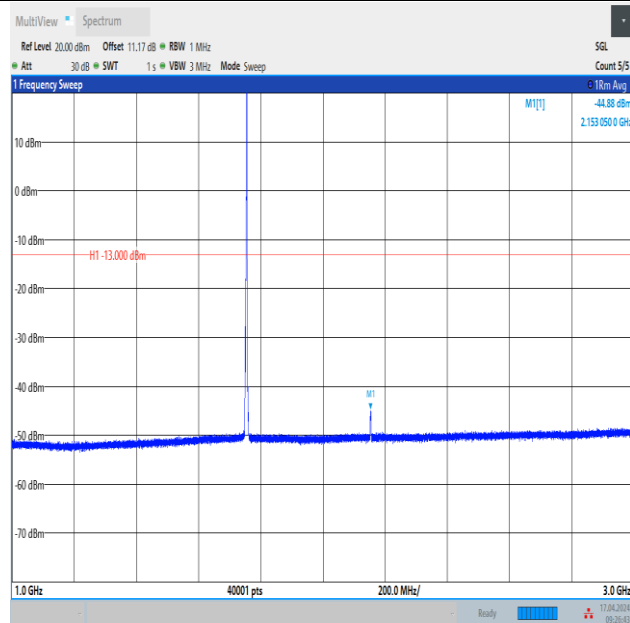
Band4_3MHz_16QAM_20385_1RB#14_1000~3000_1000~3000
