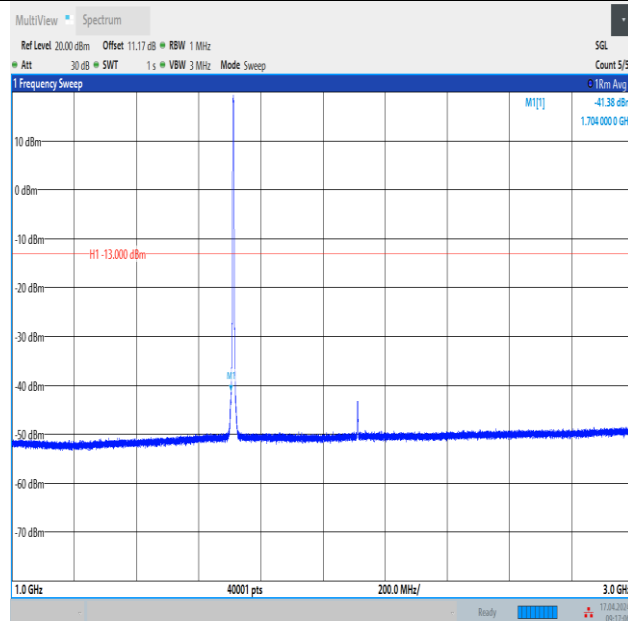
Band4_3MHz_QPSK_19965_15RB#0_1000~3000_1000~3000
