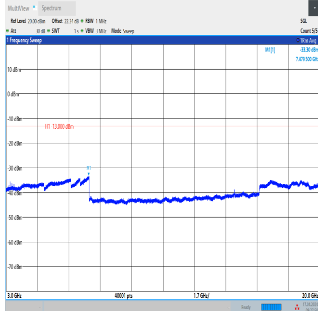
Band4_3MHz_QPSK_20385_15RB#0_3000~20000_3000~20000
