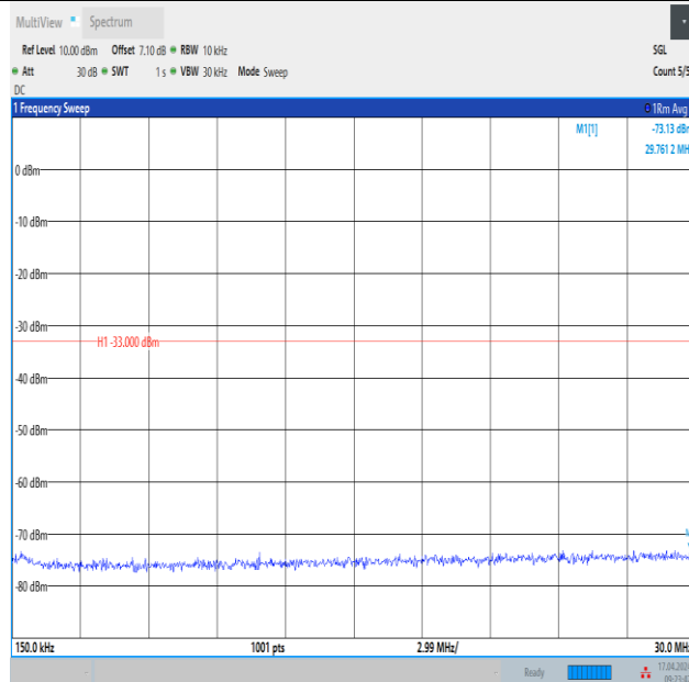
Band4_3MHz_QPSK_20385_1RB#0_0.15~30_0.15~30
