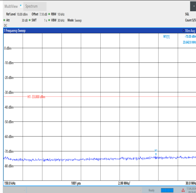
Band4_3MHz_QPSK_19965_15RB#0_0.15~30_0.15~30
