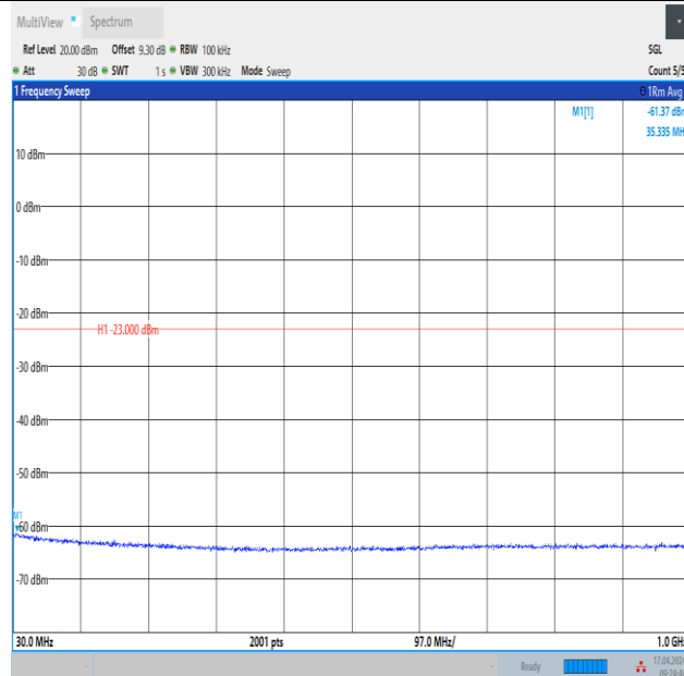
Band4_3MHz_16QAM_20385_1RB#0_30~1000_30~1000
