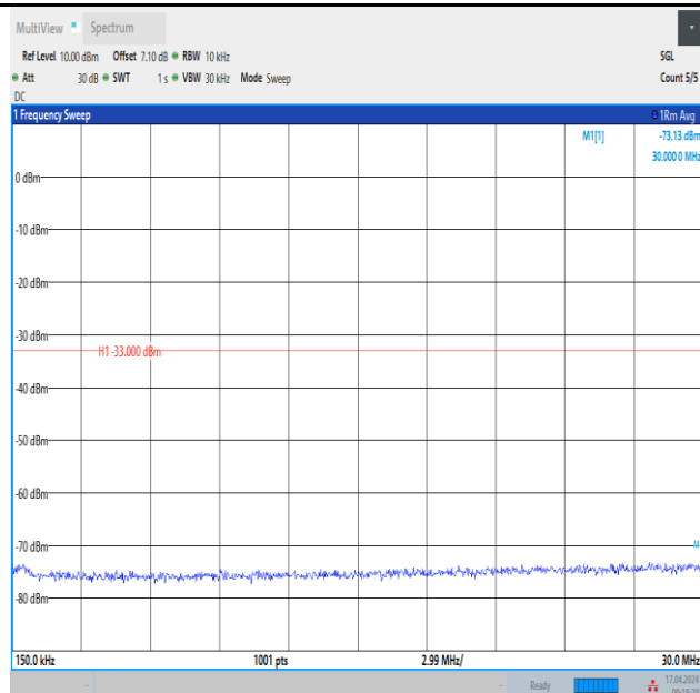
Band4_3MHz_QPSK_20175_1RB#0_0.15~30_0.15~30
