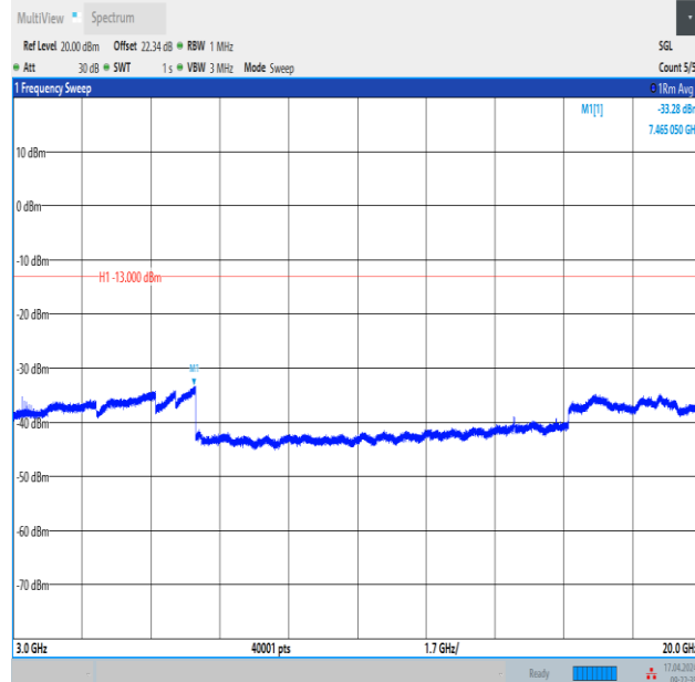
Band4_3MHz_QPSK_20175_15RB#0_3000~20000_3000~20000
