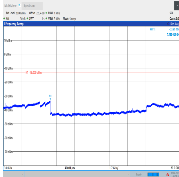
Band4_3MHz_16QAM_20175_1RB#0_3000~20000_3000~20000
