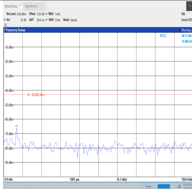
Band4_3MHz_16QAM_20175_1RB#0_0.009~0.15_0.009~0.15
