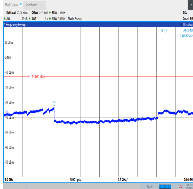
Band4_3MHz_QPSK_19965_1RB#14_3000~20000_3000~20000
