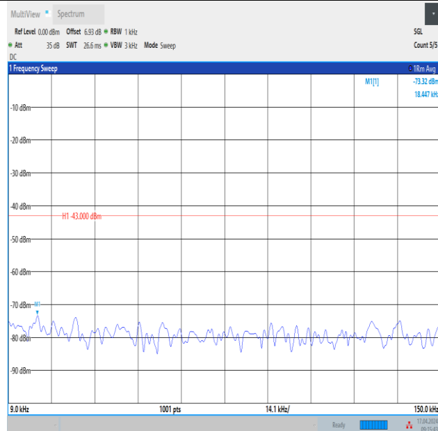
Band4_3MHz_16QAM_19965_1RB#14_0.009~0.15_0.009~0.15
