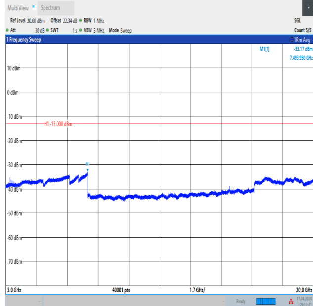
Band4_3MHz_QPSK_19965_15RB#0_3000~20000_3000~20000
