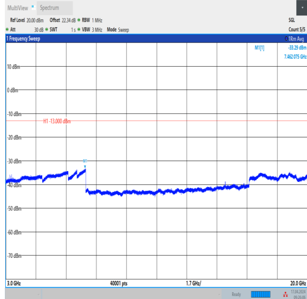
Band4_3MHz_QPSK_20385_1RB#14_3000~20000_3000~20000
