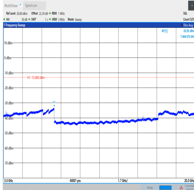
Band4_3MHz_QPSK_20175_1RB#14_3000~20000_3000~20000
