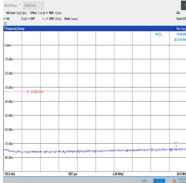
Band4_3MHz_16QAM_20175_15RB#0_0.15~30_0.15~30
