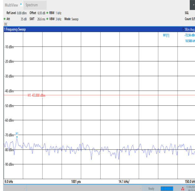
Band4_3MHz_QPSK_20385_1RB#0_0.009~0.15_0.009~0.15
