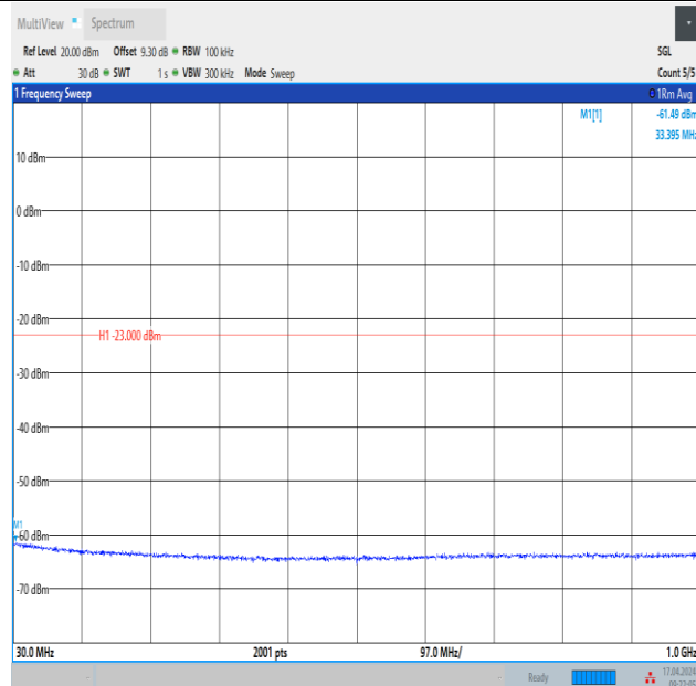
Band4_3MHz_QPSK_20175_15RB#0_30~1000_30~1000
