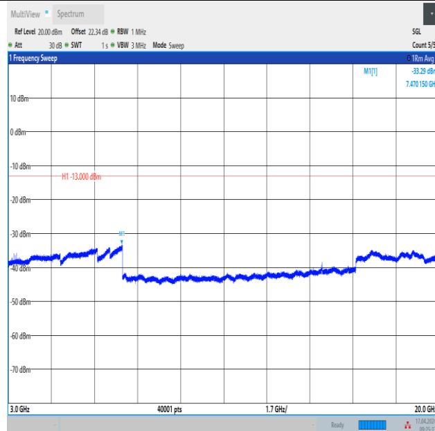
Band4_3MHz_16QAM_20385_1RB#0_3000~20000_3000~20000
