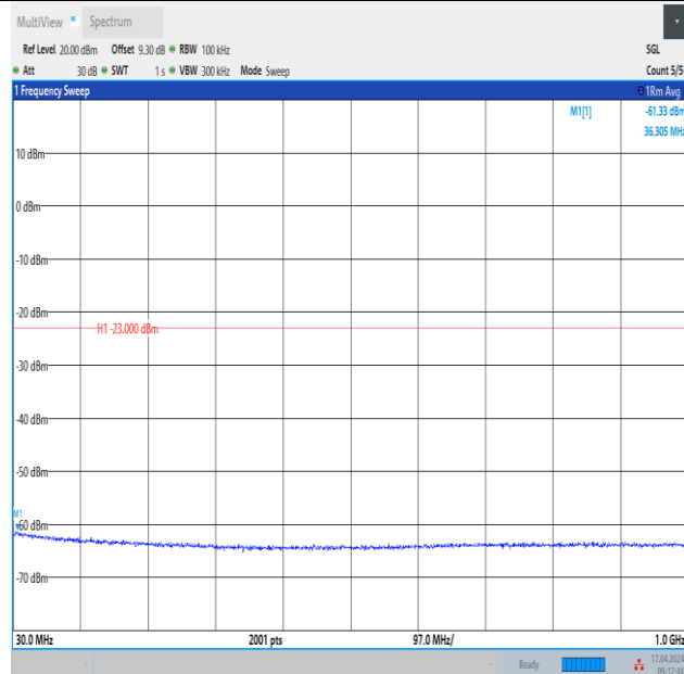
Band4_3MHz_16QAM_19965_15RB#0_30~1000_30~1000
