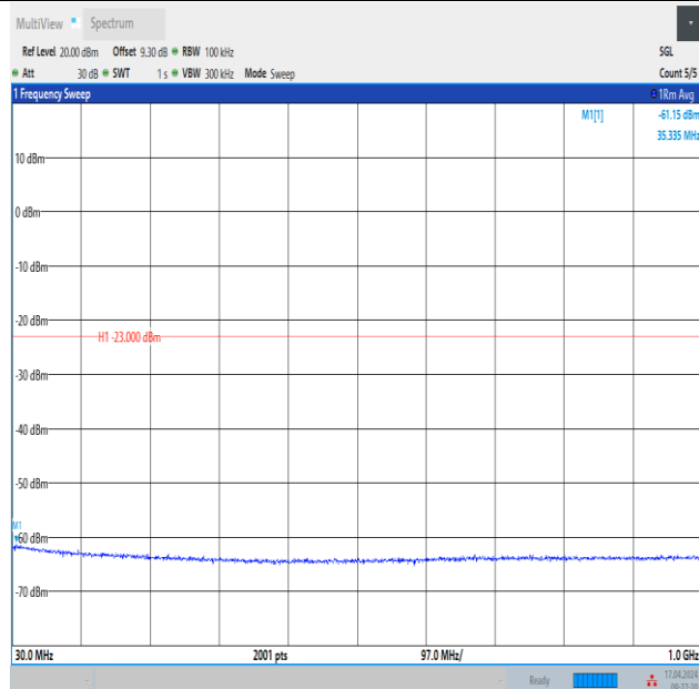
Band4_3MHz_QPSK_20385_15RB#0_30~1000_30~1000
