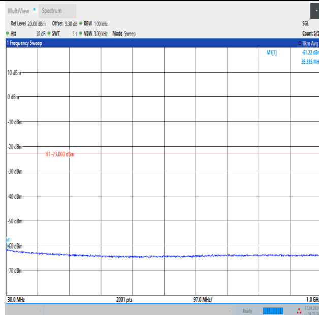
Band4_3MHz_QPSK_20385_1RB#14_30~1000_30~1000
