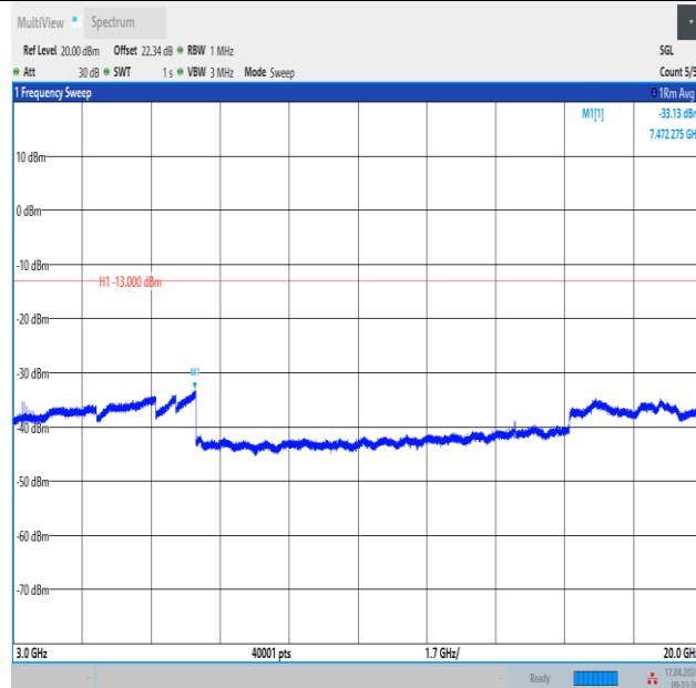
Band4_3MHz_16QAM_20175_15RB#0_3000~20000_3000~20000
