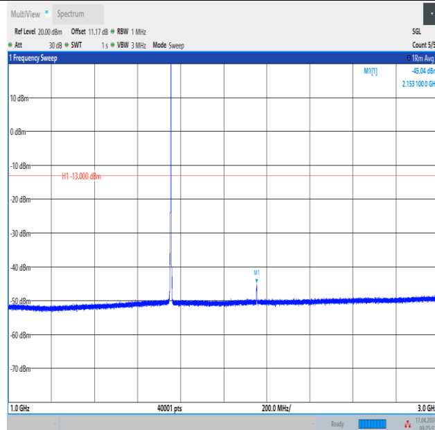
Band4_3MHz_QPSK_20385_1RB#14_1000~3000_1000~3000
