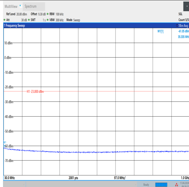
Band4_3MHz_QPSK_20175_1RB#14_30~1000_30~1000
