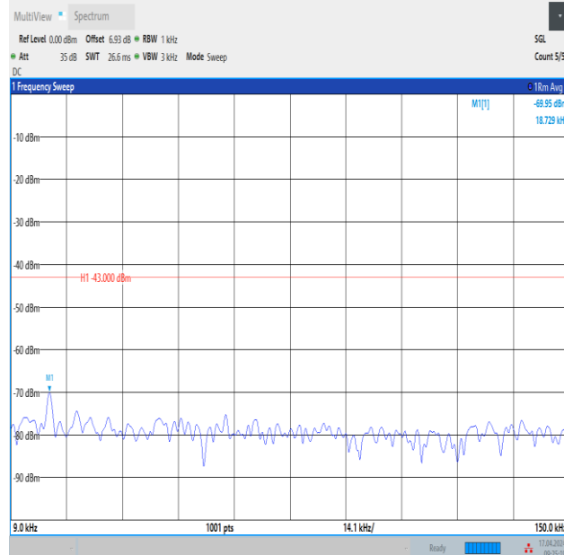
Band4_3MHz_QPSK_20385_1RB#14_0.009~0.15_0.009~0.15
