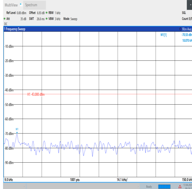
Band4_3MHz_QPSK_20175_1RB#0_0.009~0.15_0.009~0.15
