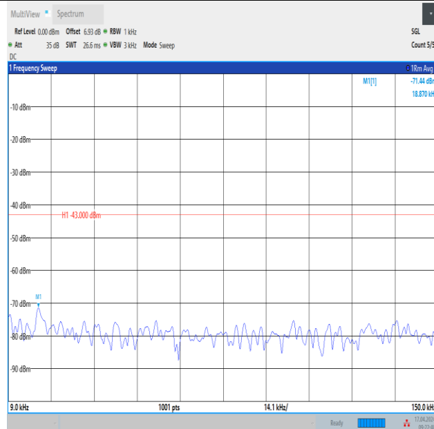
Band4_3MHz_16QAM_20175_15RB#0_0.009~0.15_0.009~0.15
