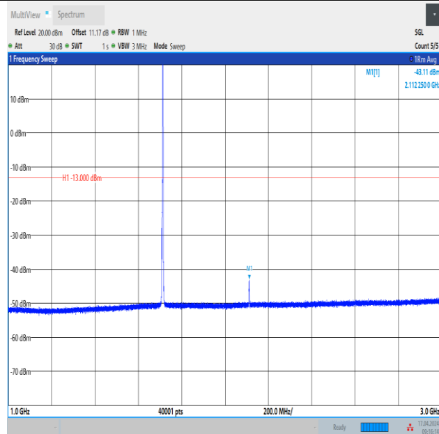
Band4_3MHz_16QAM_19965_1RB#14_1000~3000_1000~3000
