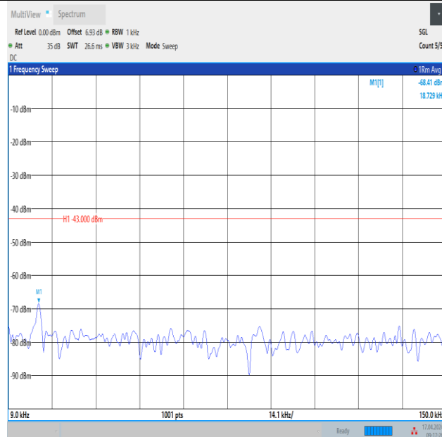
Band4_3MHz_16QAM_19965_15RB#0_0.009~0.15_0.009~0.15
