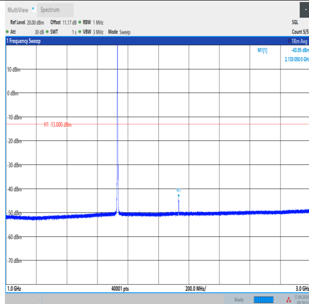
Band4_3MHz_QPSK_20175_1RB#0_1000~3000_1000~3000
