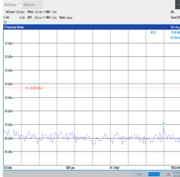
Band4_3MHz_QPSK_20175_15RB#0_0.009~0.15_0.009~0.15
