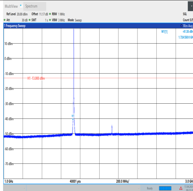
Band4_3MHz_QPSK_20175_15RB#0_1000~3000_1000~3000
