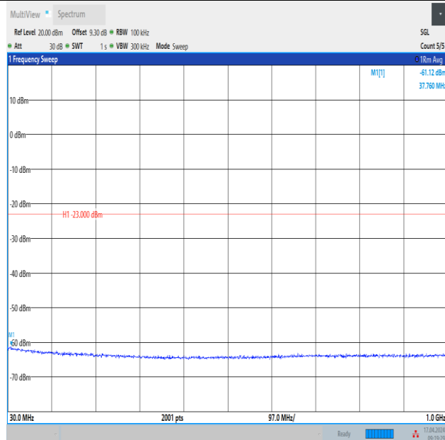
Band4_3MHz_16QAM_20175_1RB#0_30~1000_30~1000
