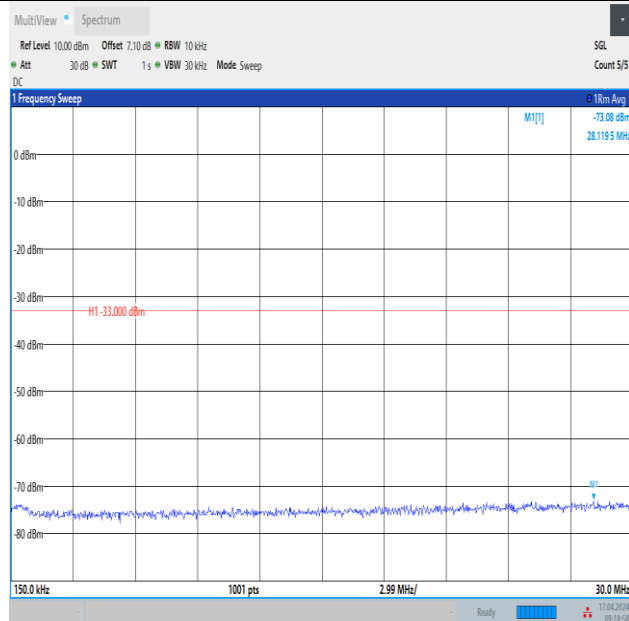
Band4_3MHz_QPSK_19965_1RB#14_0.15~30_0.15~30
