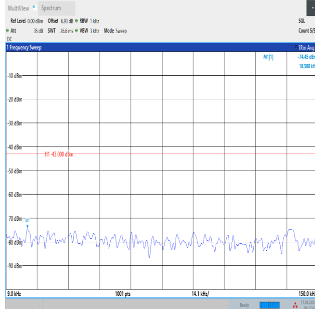
Band4_3MHz_QPSK_20385_15RB#0_0.009~0.15_0.009~0.15
