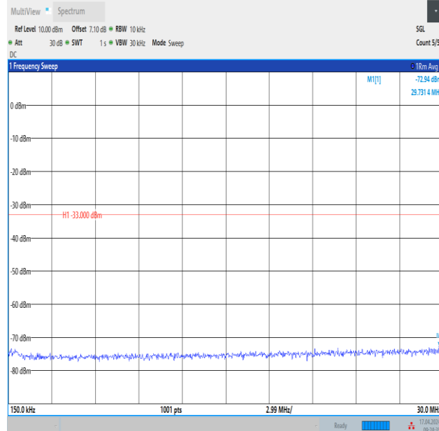
Band4_3MHz_16QAM_20385_1RB#0_0.15~30_0.15~30
