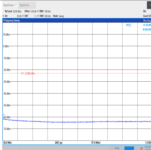
Band4_3MHz_QPSK_20385_1RB#0_30~1000_30~1000
