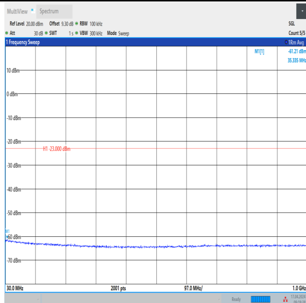
Band4_3MHz_QPSK_20175_1RB#0_30~1000_30~1000
