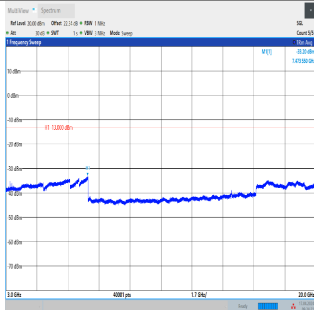
Band4_3MHz_QPSK_20385_1RB#0_3000~20000_3000~20000
