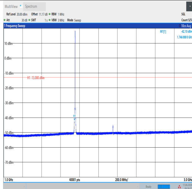
Band4_3MHz_16QAM_20385_15RB#0_1000~3000_1000~3000
