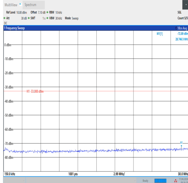
Band4_3MHz_16QAM_20385_1RB#14_0.15~30_0.15~30
