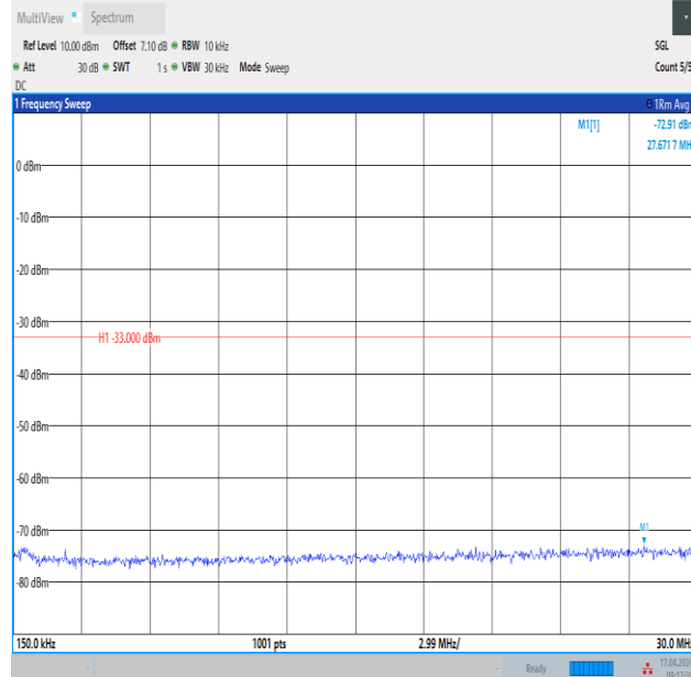
Band4_3MHz_16QAM_19965_15RB#0_0.15~30_0.15~30
