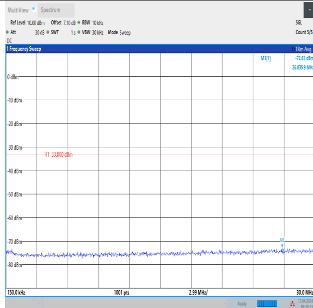
Band4_3MHz_QPSK_20175_1RB#14_0.15~30_0.15~30
