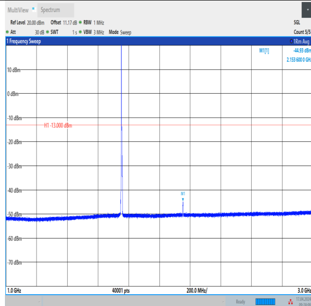
Band4_3MHz_QPSK_20385_1RB#0_1000~3000_1000~3000
