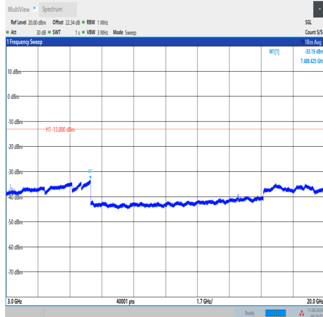
Band4_3MHz_QPSK_20175_1RB#0_3000~20000_3000~20000
