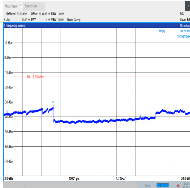
Band4_3MHz_16QAM_19965_1RB#14_3000~20000_3000~20000
