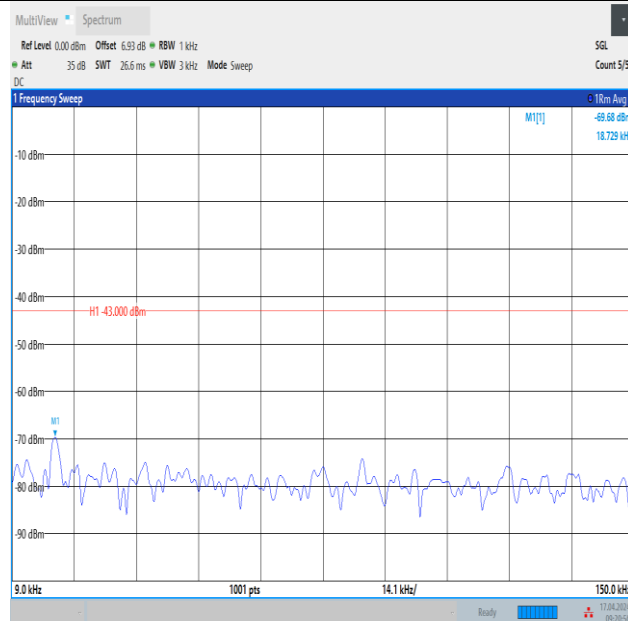
Band4_3MHz_16QAM_20175_1RB#14_0.009~0.15_0.009~0.15
