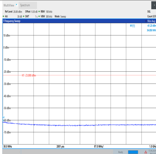
Band4_3MHz_QPSK_19965_1RB#14_30~1000_30~1000
