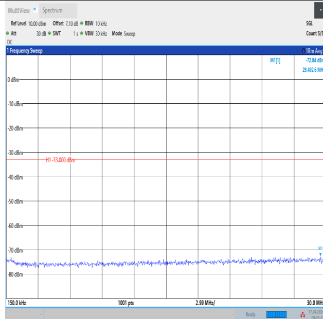
Band4_3MHz_QPSK_20385_1RB#14_0.15~30_0.15~30
