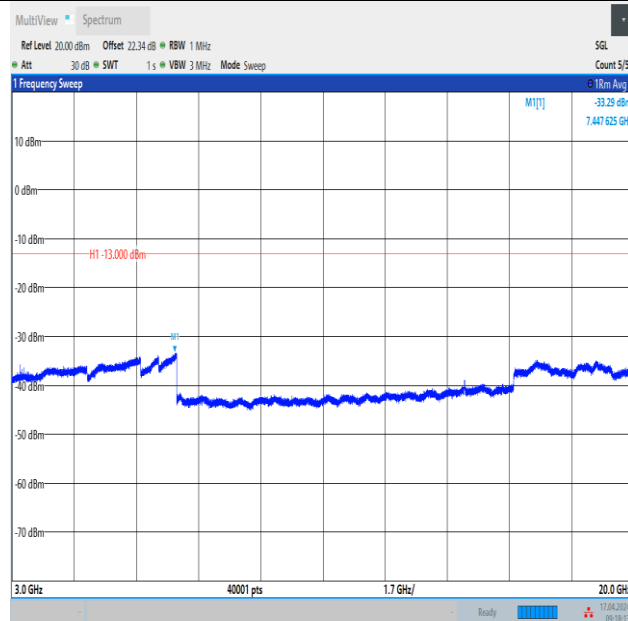
Band4_3MHz_16QAM_19965_15RB#0_3000~20000_3000~20000
