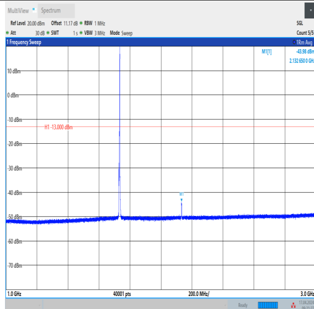
Band4_3MHz_16QAM_20175_1RB#14_1000~3000_1000~3000
