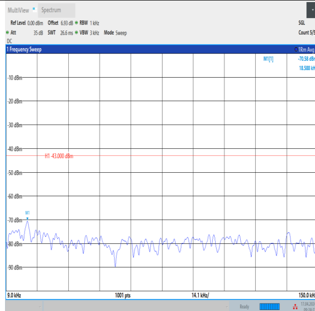
Band4_3MHz_16QAM_20385_1RB#0_0.009~0.15_0.009~0.15
