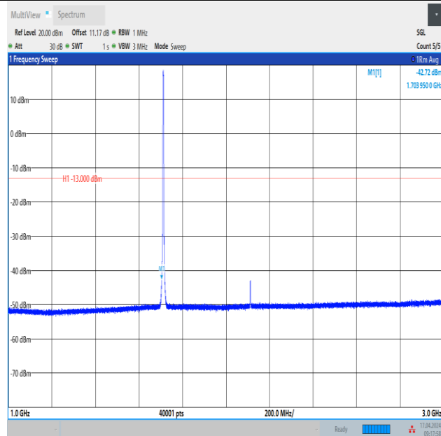
Band4_3MHz_16QAM_19965_15RB#0_1000~3000_1000~3000
