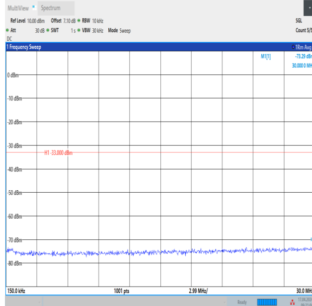
Band4_3MHz_16QAM_20175_1RB#14_0.15~30_0.15~30
