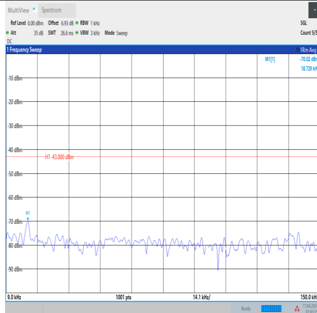
Band2_15MHz_16QAM_18900_1RB#74_0.009~0.15_0.009~0.15
