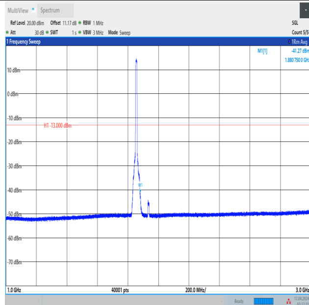
Band2_10MHz_QPSK_18650_50RB#0_1000~3000_1000~3000
