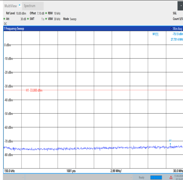
Band2_10MHz_16QAM_19150_1RB#49_0.15~30_0.15~30
