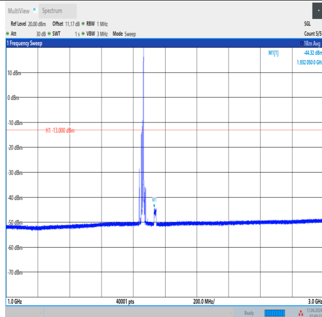
Band2_15MHz_16QAM_18675_1RB#74_1000~3000_1000~3000
