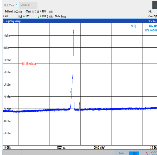
Band2_10MHz_QPSK_19150_50RB#0_1000~3000_1000~3000
