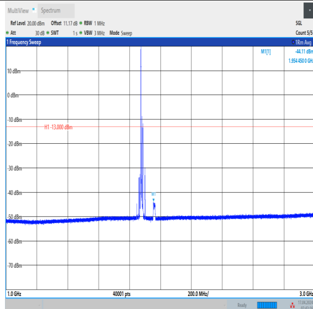
Band2_15MHz_16QAM_18900_1RB#0_1000~3000_1000~3000
