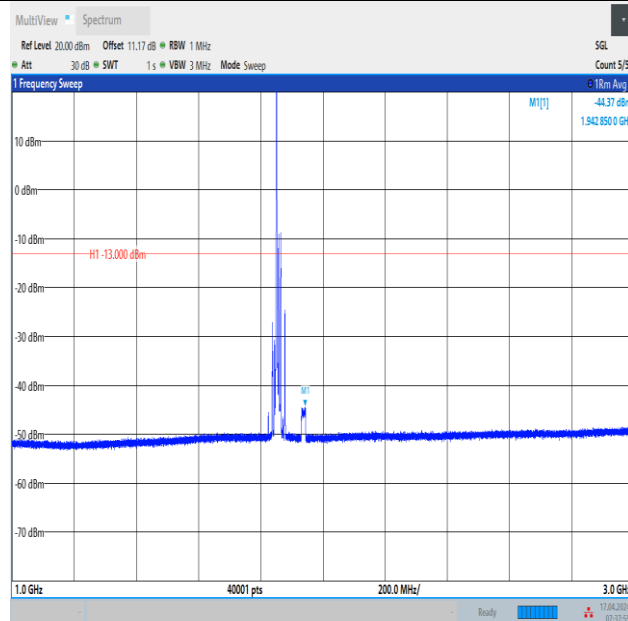
Band2_15MHz_QPSK_18675_1RB#0_1000~3000_1000~3000
