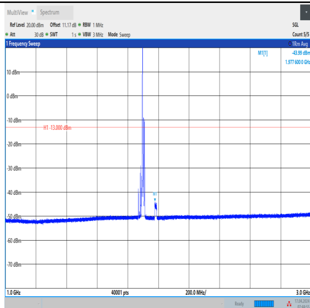
Band2_15MHz_QPSK_19125_1RB#0_1000~3000_1000~3000
