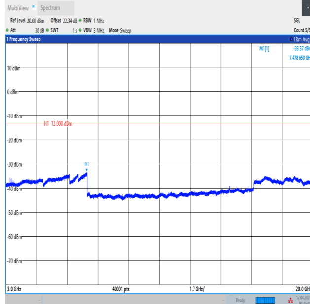
Band2_10MHz_16QAM_19150_1RB#0_3000~20000_3000~20000
