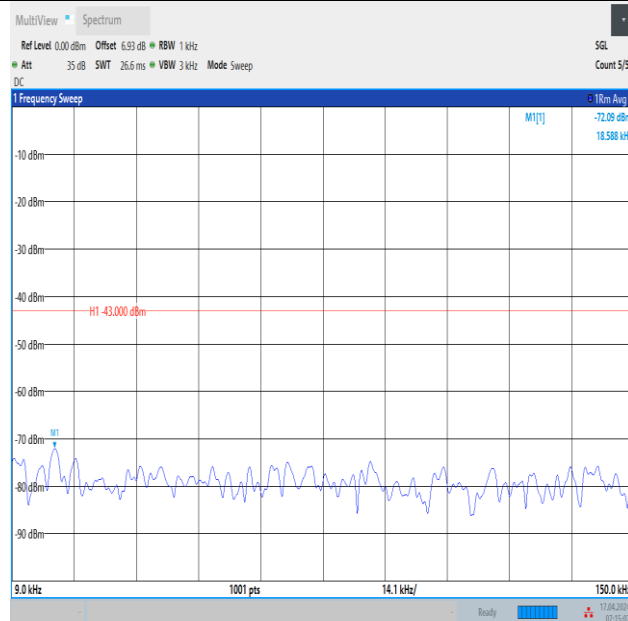
Band2_10MHz_QPSK_19150_1RB#49_0.009~0.15_0.009~0.15
