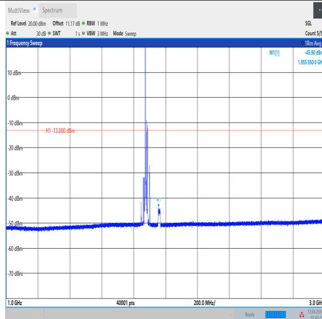
Band2_15MHz_QPSK_18900_1RB#0_1000~3000_1000~3000
