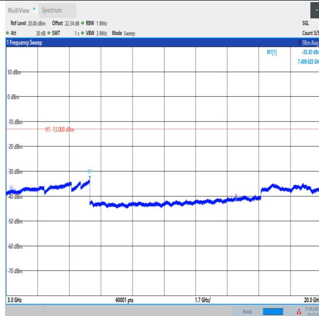
Band2_10MHz_QPSK_19150_1RB#49_3000~20000_3000~20000
