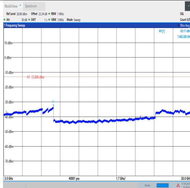
Band2_15MHz_QPSK_18900_75RB#0_3000~20000_3000~20000
