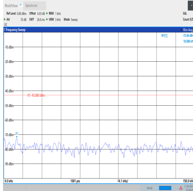
Band2_15MHz_QPSK_19125_1RB#0_0.009~0.15_0.009~0.15
