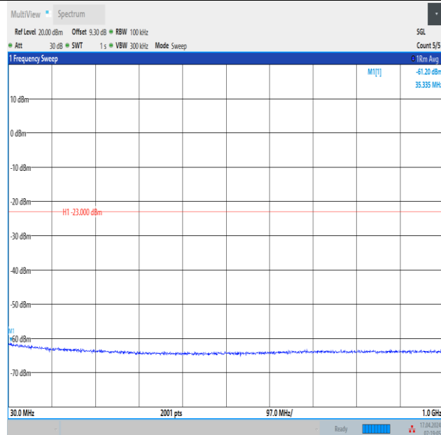
Band2_10MHz_QPSK_19150_50RB#0_30~1000_30~1000
