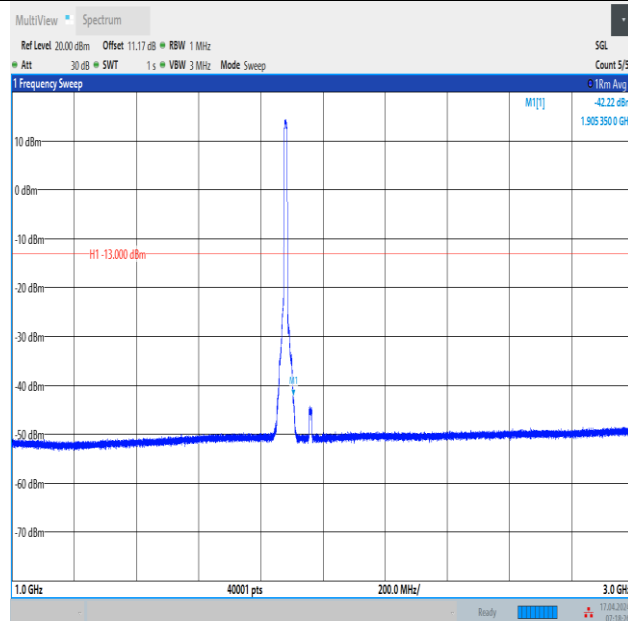
Band2_10MHz_QPSK_18900_50RB#0_1000~3000_1000~3000
