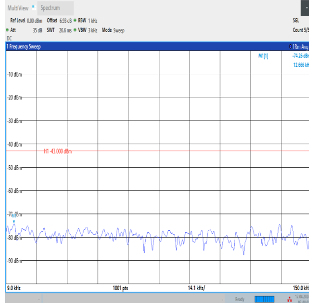
Band2_15MHz_QPSK_18675_75RB#0_0.009~0.15_0.009~0.15
