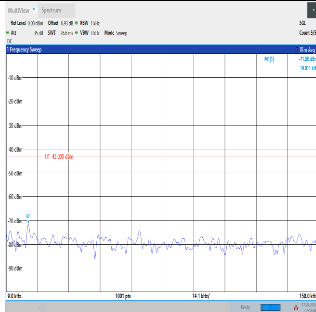
Band2_10MHz_QPSK_19150_50RB#0_0.009~0.15_0.009~0.15
