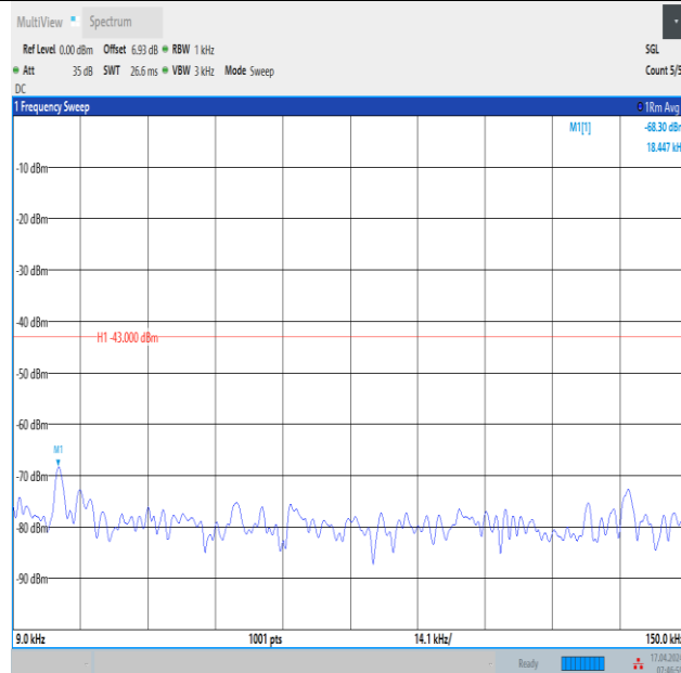
Band2_15MHz_16QAM_19125_1RB#74_0.009~0.15_0.009~0.15
