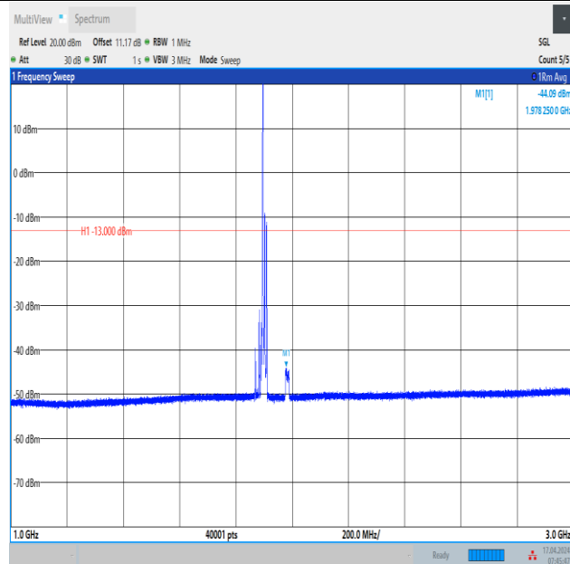
Band2_15MHz_16QAM_19125_1RB#0_1000~3000_1000~3000
