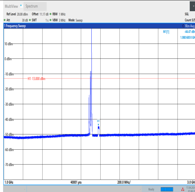
Band2_15MHz_QPSK_19125_1RB#74_1000~3000_1000~3000
