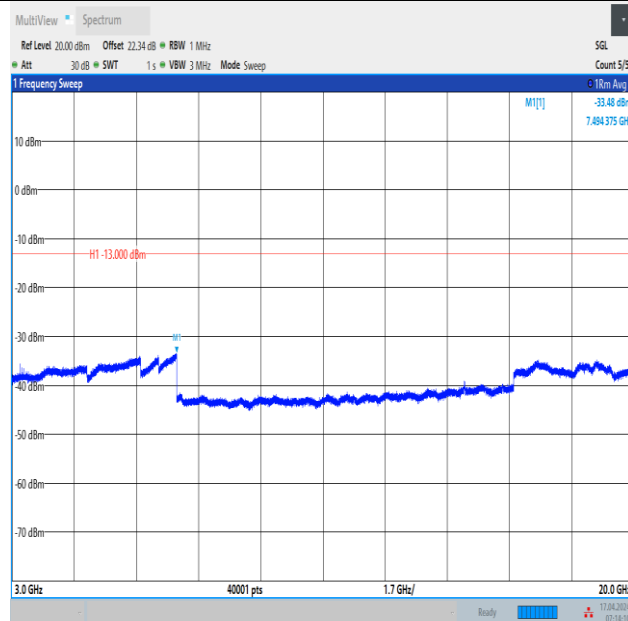
Band2_10MHz_QPSK_19150_1RB#0_3000~20000_3000~20000
