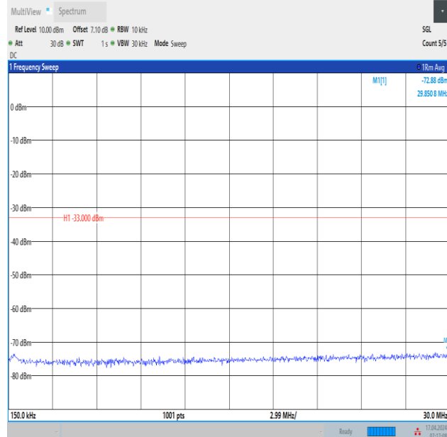
Band2_10MHz_QPSK_18650_50RB#0_0.15~30_0.15~30
