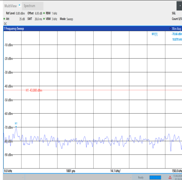
Band2_15MHz_16QAM_18675_1RB#74_0.009~0.15_0.009~0.15
