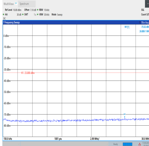
Band2_10MHz_QPSK_19150_50RB#0_0.15~30_0.15~30
