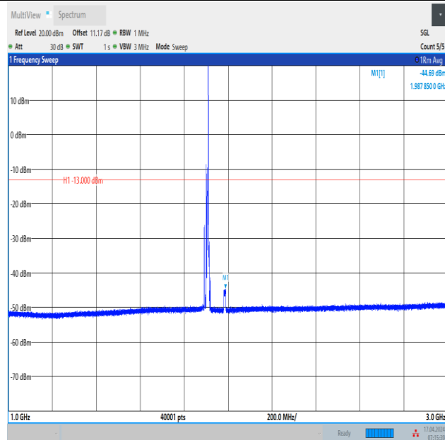
Band2_10MHz_QPSK_19150_1RB#49_1000~3000_1000~3000
