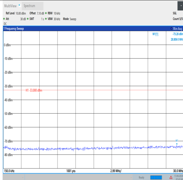
Band2_15MHz_QPSK_18900_1RB#74_0.15~30_0.15~30
