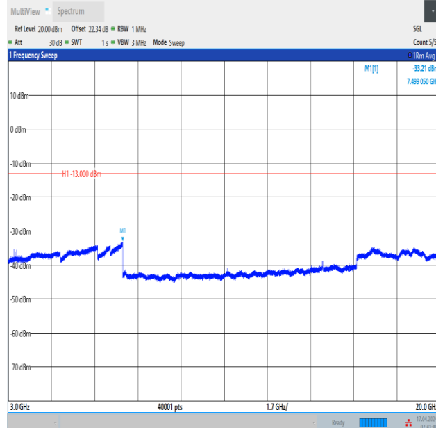
Band2_15MHz_QPSK_18900_1RB#0_3000~20000_3000~20000
