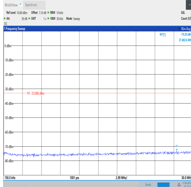
Band2_10MHz_QPSK_19150_1RB#49_0.15~30_0.15~30
