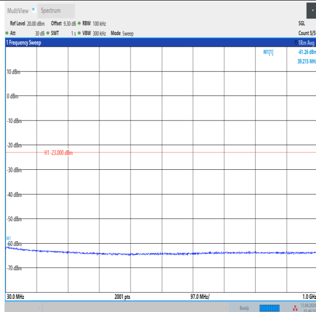
Band2_15MHz_QPSK_19125_1RB#74_30~1000_30~1000
