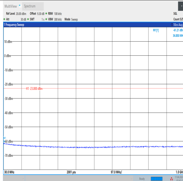
Band2_15MHz_QPSK_18900_1RB#0_30~1000_30~1000
