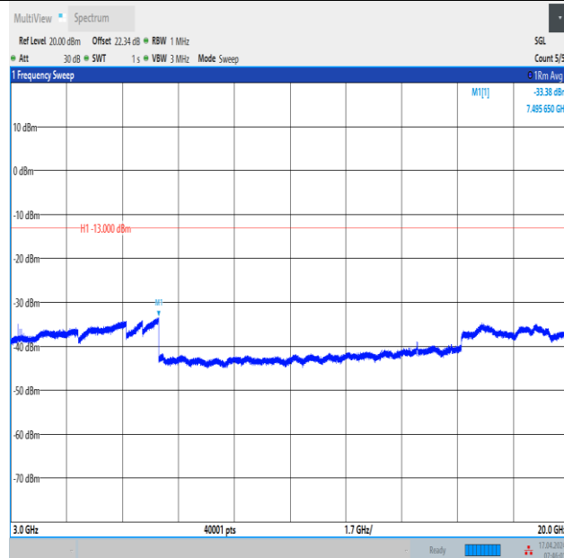
Band2_15MHz_16QAM_19125_1RB#0_3000~20000_3000~20000
