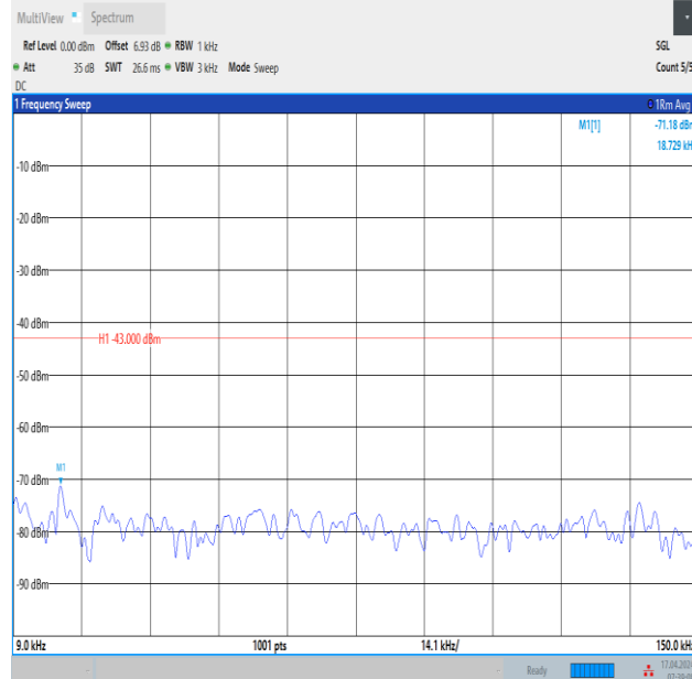
Band2_15MHz_QPSK_18675_1RB#74_0.009~0.15_0.009~0.15
