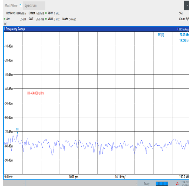
Band2_10MHz_16QAM_19150_1RB#49_0.009~0.15_0.009~0.15
