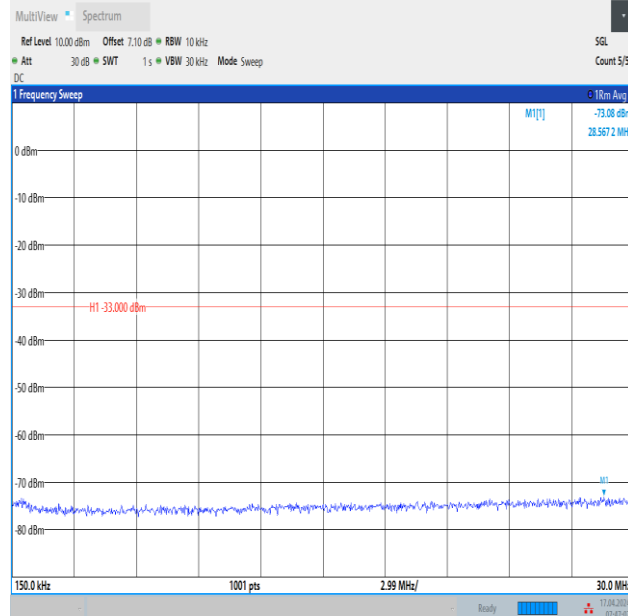
Band2_15MHz_16QAM_19125_1RB#74_0.15~30_0.15~30
