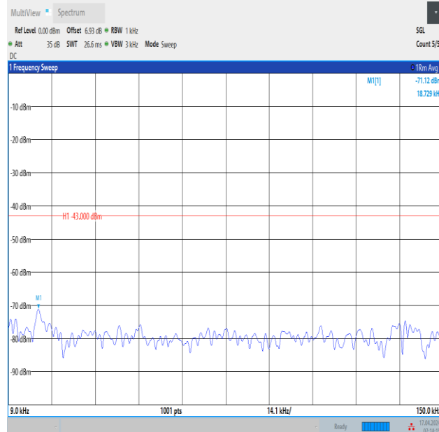
Band2_10MHz_16QAM_19150_1RB#0_0.009~0.15_0.009~0.15
