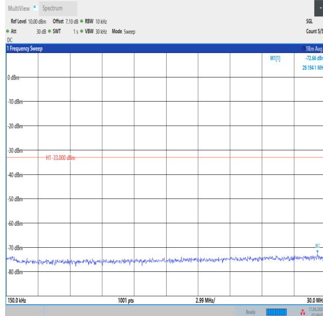
Band2_15MHz_QPSK_18900_75RB#0_0.15~30_0.15~30
