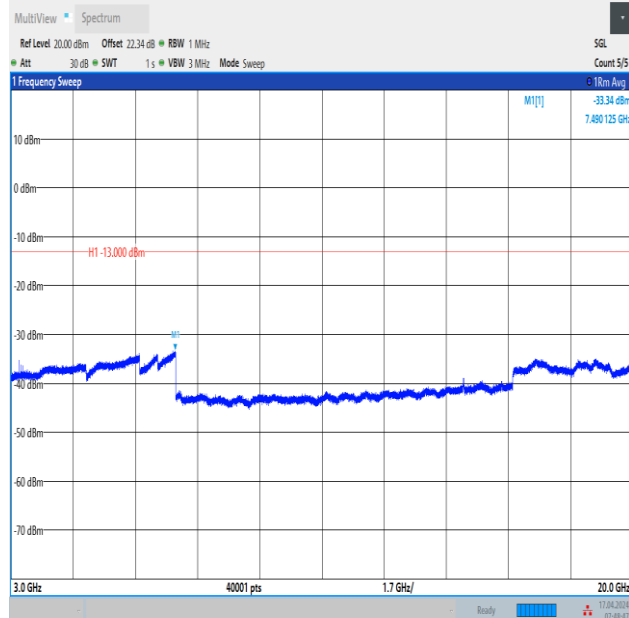
Band2_15MHz_QPSK_18675_75RB#0_3000~20000_3000~20000
