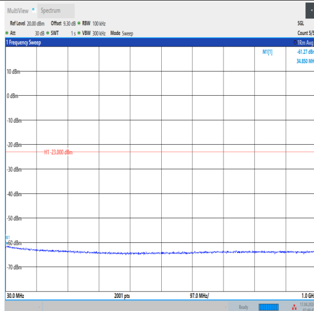
Band2_15MHz_QPSK_19125_1RB#0_30~1000_30~1000
