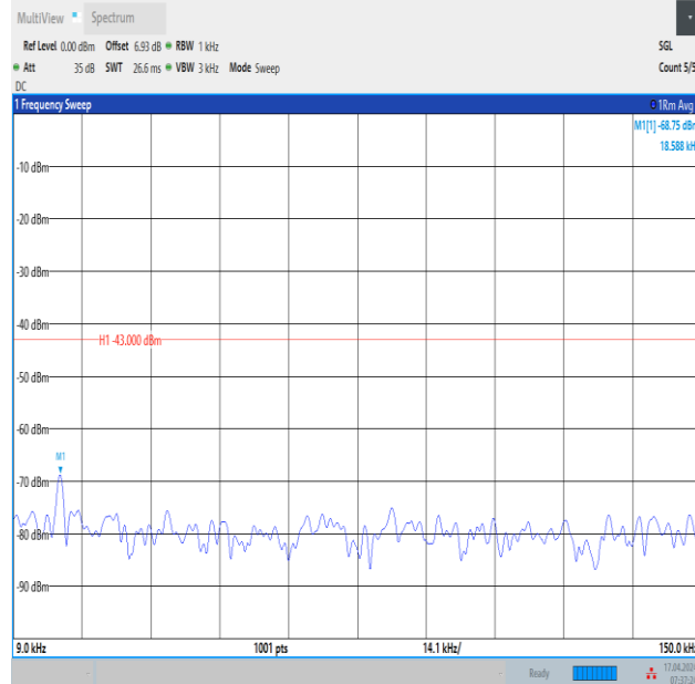
Band2_15MHz_QPSK_18675_1RB#0_0.009~0.15_0.009~0.15
