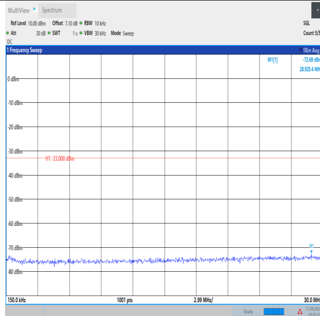
Band2_15MHz_QPSK_18900_1RB#0_0.15~30_0.15~30
