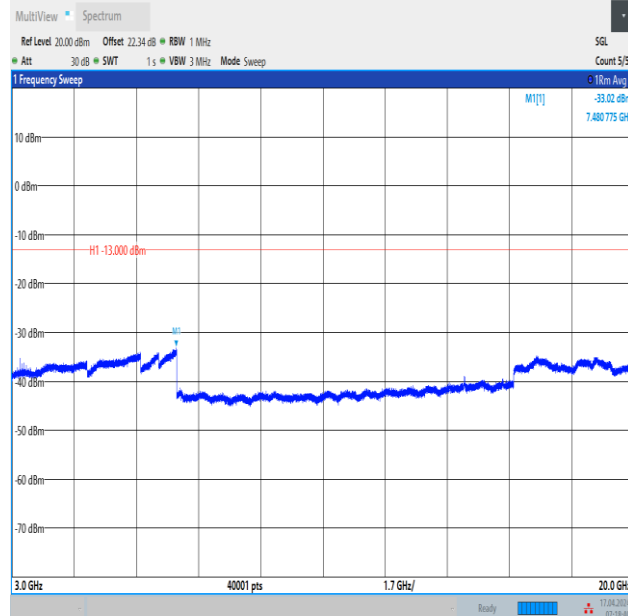
Band2_10MHz_QPSK_18900_50RB#0_3000~20000_3000~20000
