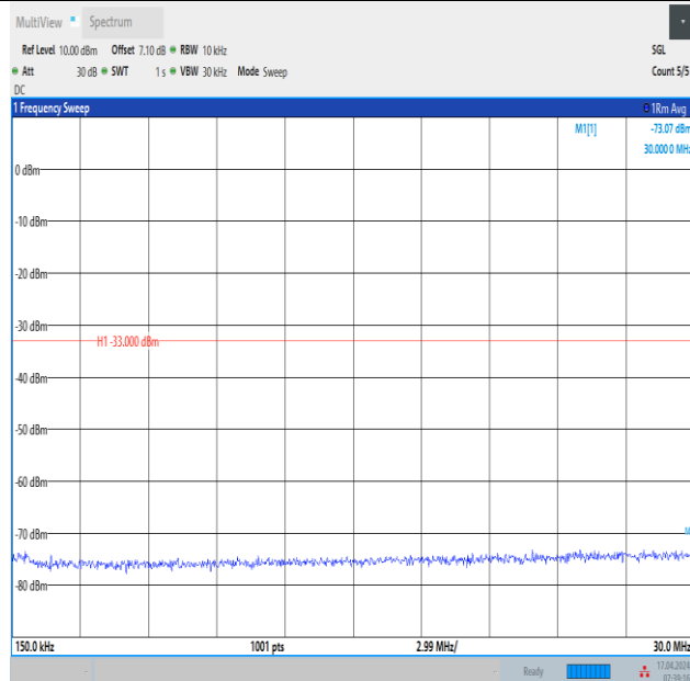
Band2_15MHz_QPSK_18675_1RB#74_0.15~30_0.15~30
