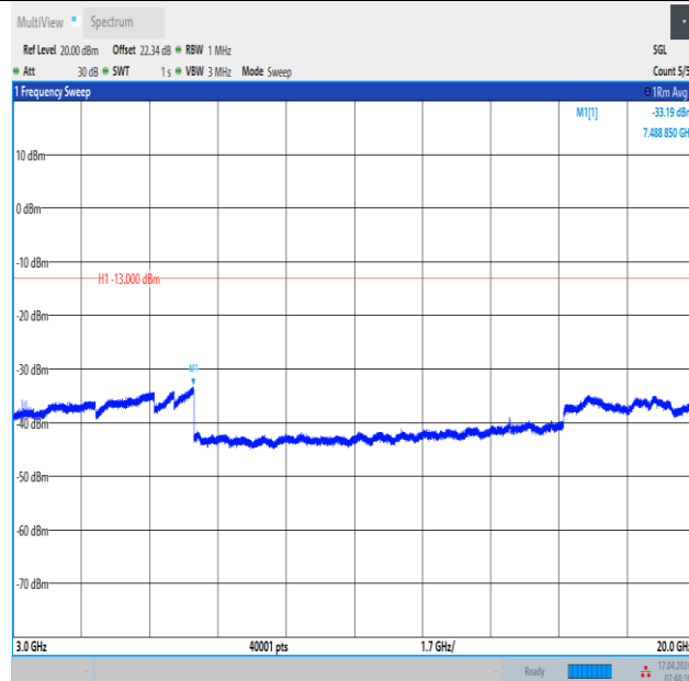
Band2_15MHz_16QAM_18900_1RB#74_3000~20000_3000~20000
