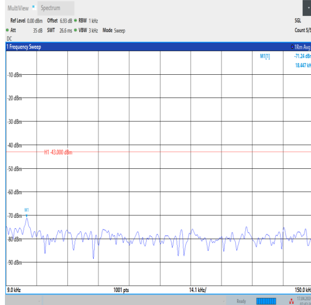
Band2_15MHz_QPSK_18900_1RB#74_0.009~0.15_0.009~0.15
