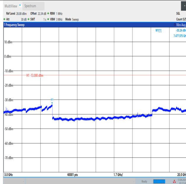
Band2_10MHz_QPSK_18650_50RB#0_3000~20000_3000~20000
