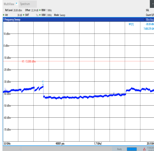
Band2_15MHz_QPSK_18900_1RB#74_3000~20000_3000~20000
