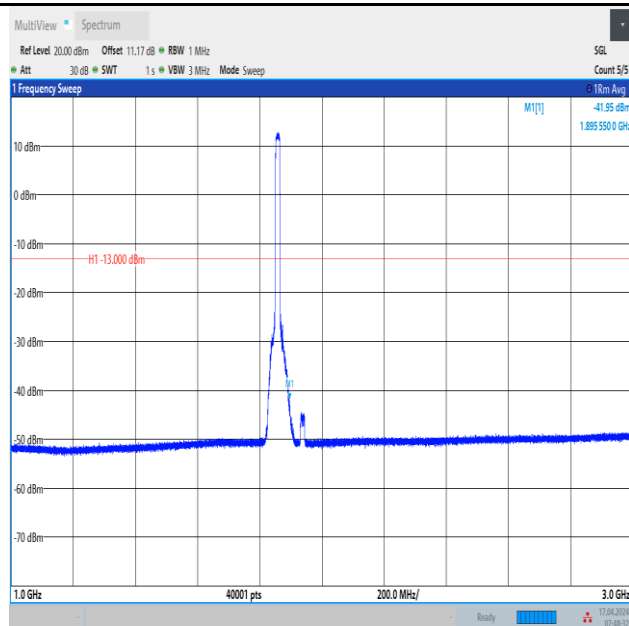
Band2_15MHz_QPSK_18675_75RB#0_1000~3000_1000~3000
