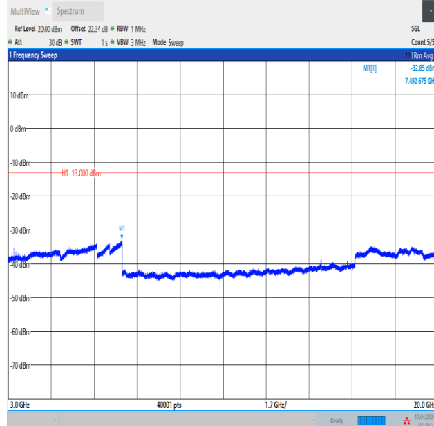
Band2_15MHz_QPSK_18675_1RB#74_3000~20000_3000~20000
