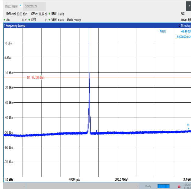
Band2_10MHz_16QAM_19150_1RB#0_1000~3000_1000~3000
