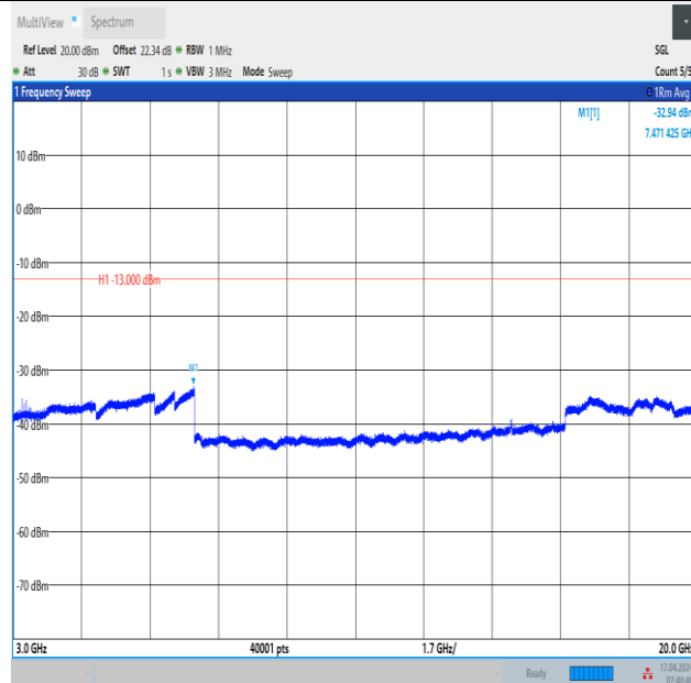
Band2_15MHz_16QAM_18675_1RB#74_3000~20000_3000~20000
