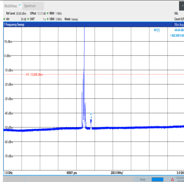
Band2_15MHz_QPSK_18900_1RB#74_1000~3000_1000~3000
