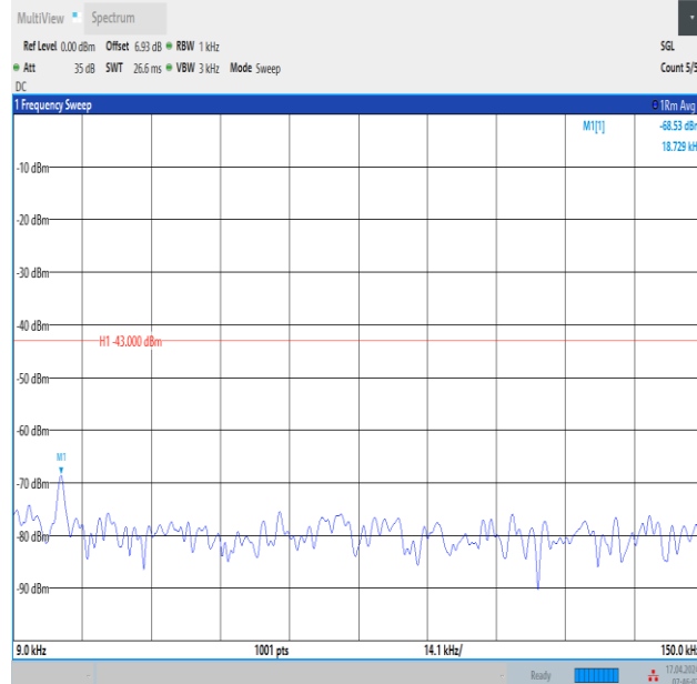
Band2_15MHz_QPSK_19125_1RB#74_0.009~0.15_0.009~0.15
