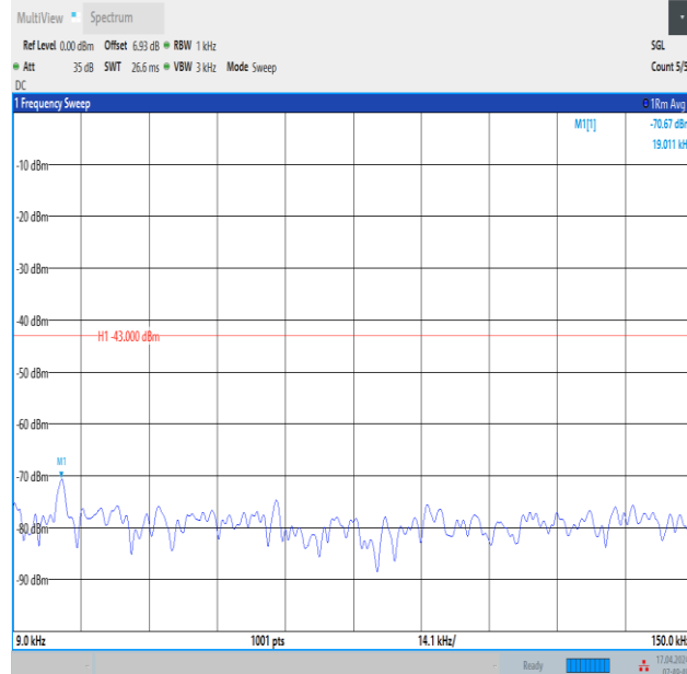
Band2_15MHz_QPSK_19125_75RB#0_0.009~0.15_0.009~0.15
