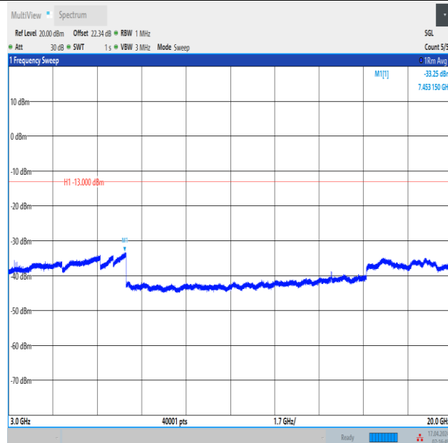
Band2_10MHz_16QAM_19150_1RB#49_3000~20000_3000~20000
