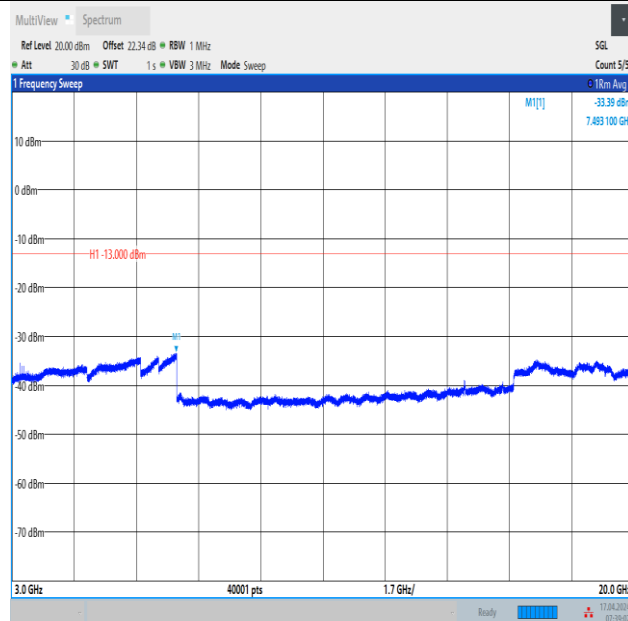
Band2_15MHz_16QAM_18675_1RB#0_3000~20000_3000~20000
