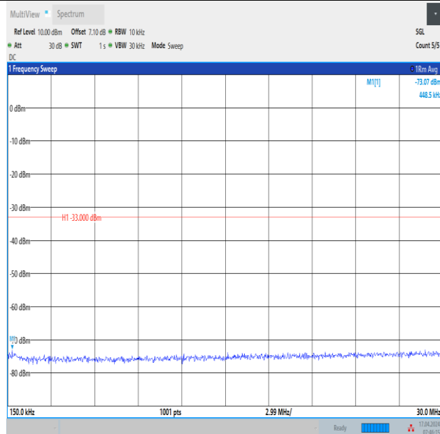
Band2_15MHz_QPSK_19125_1RB#74_0.15~30_0.15~30
