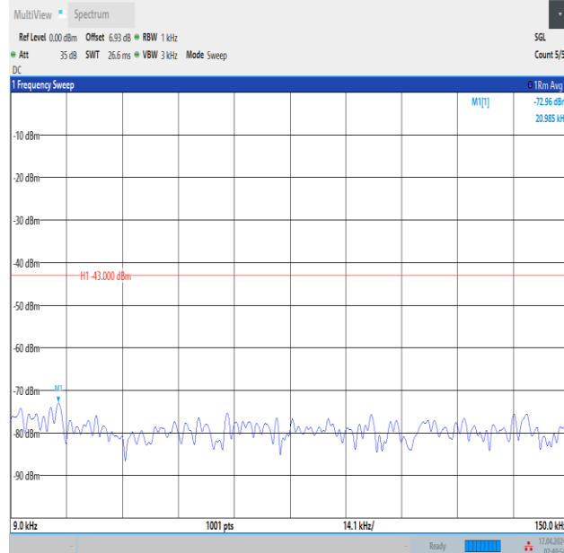
Band2_15MHz_QPSK_18900_1RB#0_0.009~0.15_0.009~0.15
