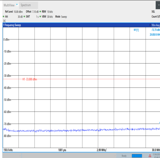
Band2_15MHz_QPSK_19125_1RB#0_0.15~30_0.15~30
