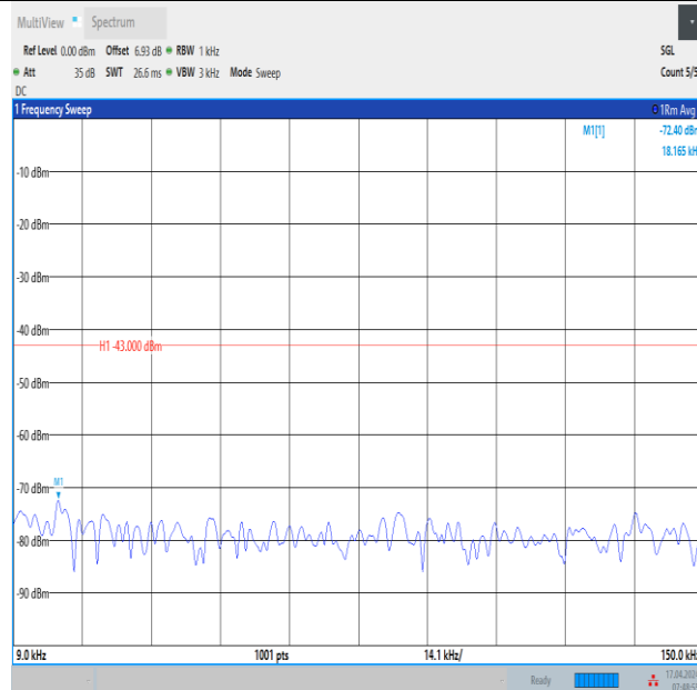
Band2_15MHz_QPSK_18900_75RB#0_0.009~0.15_0.009~0.15
