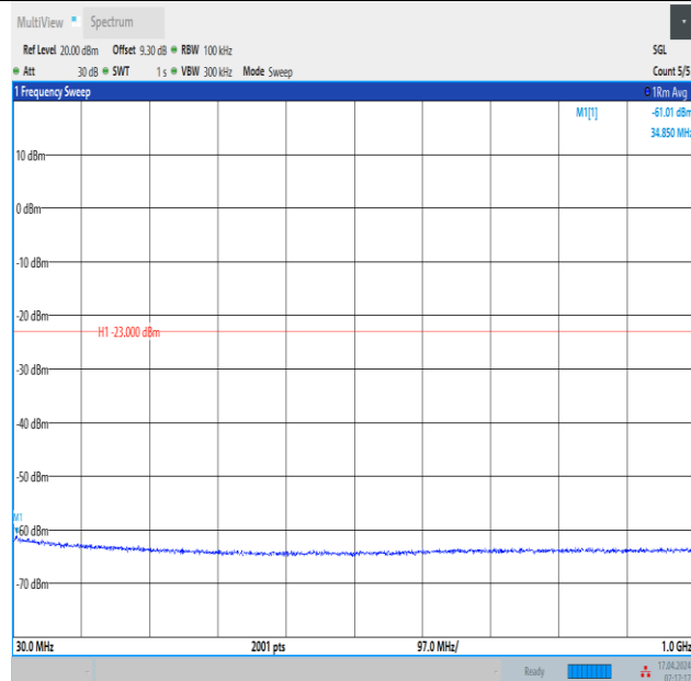
Band2_10MHz_QPSK_18650_50RB#0_30~1000_30~1000
