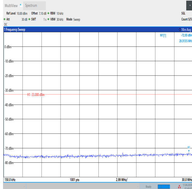
Band2_15MHz_16QAM_18675_1RB#74_0.15~30_0.15~30
