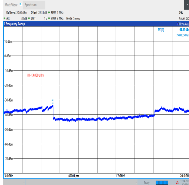
Band2_15MHz_QPSK_19125_1RB#74_3000~20000_3000~20000
