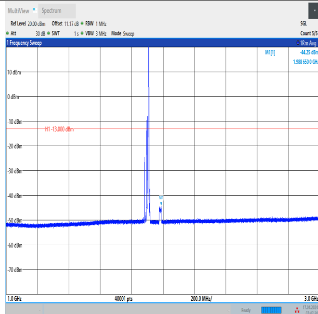
Band2_15MHz_16QAM_19125_1RB#74_1000~3000_1000~3000
