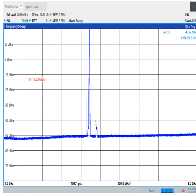
Band2_15MHz_16QAM_18900_1RB#74_1000~3000_1000~3000
