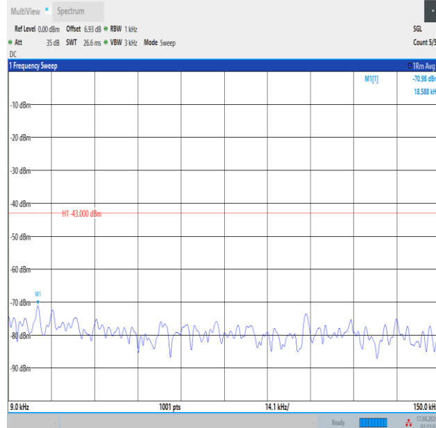
Band2_10MHz_QPSK_18900_50RB#0_0.009~0.15_0.009~0.15
