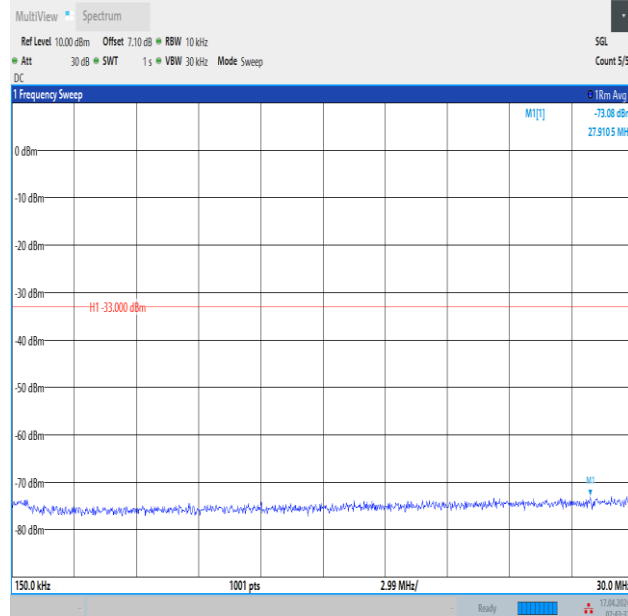
Band2_15MHz_16QAM_18900_1RB#74_0.15~30_0.15~30
