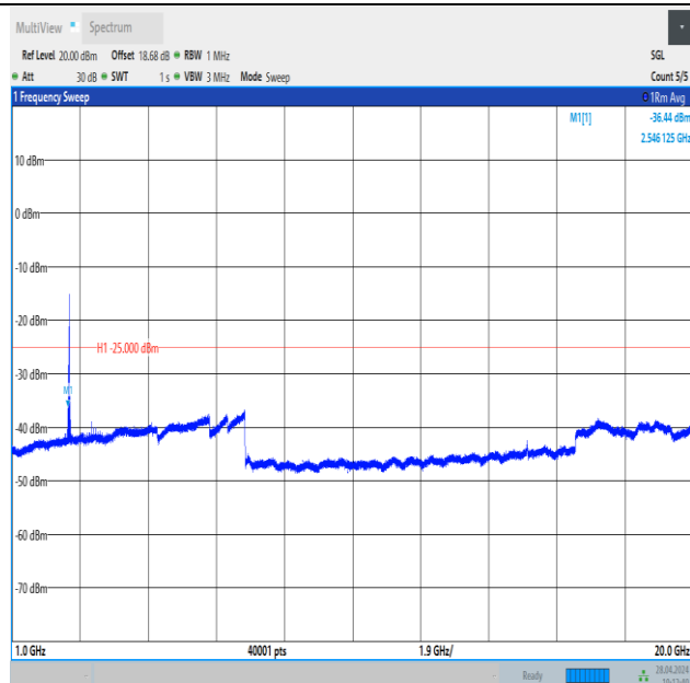
Band41_15MHz_16QAM_40620_1RB#0_1000~20000_1000~20000
