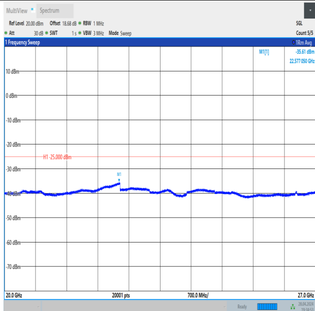
Band41_10MHz_QPSK_41540_1RB#49_20000~27000_20000~27000
