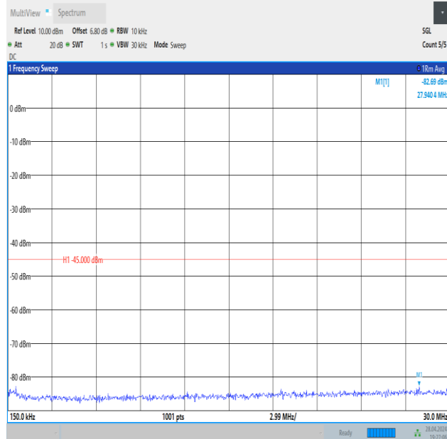
Band41_10MHz_16QAM_39700_1RB#0_0.15~30_0.15~30
