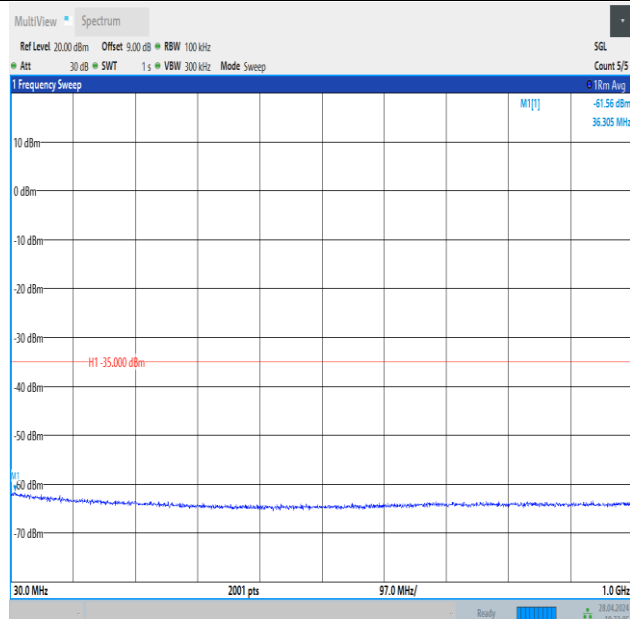
Band41_10MHz_QPSK_40620_50RB#0_30~1000_30~1000
