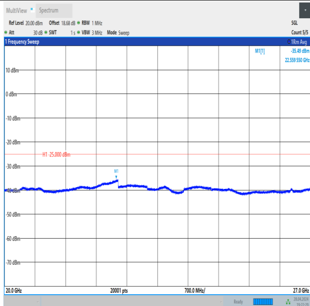
Band41_10MHz_QPSK_40620_50RB#0_20000~27000_20000~27000
