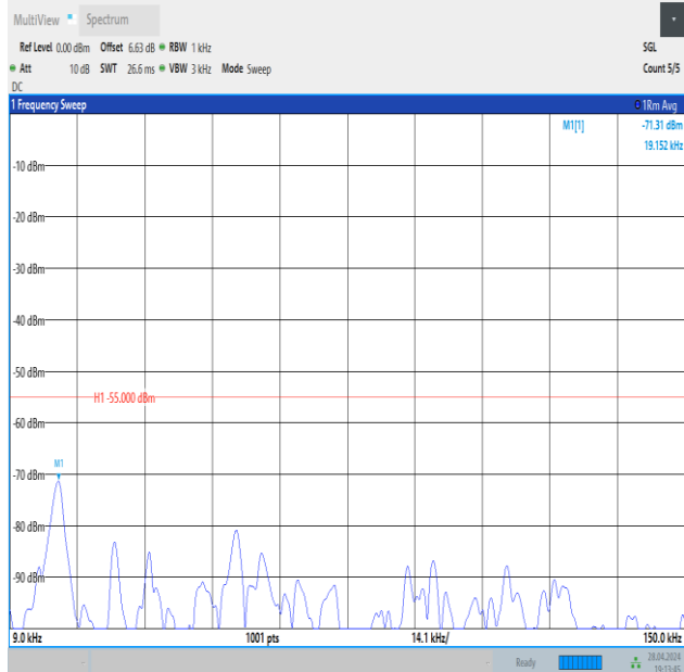
Band41_15MHz_16QAM_40620_1RB#74_0.009~0.15_0.009~0.15
