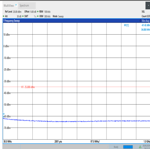
Band41_10MHz_QPSK_39700_50RB#0_30~1000_30~1000
