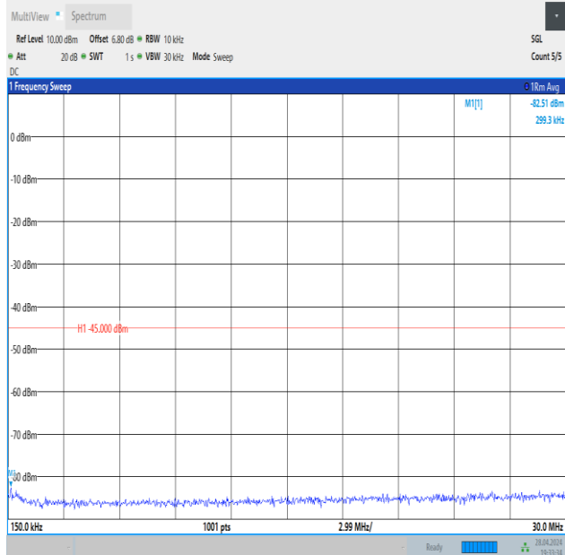
Band41_10MHz_16QAM_41540_1RB#0_0.15~30_0.15~30
