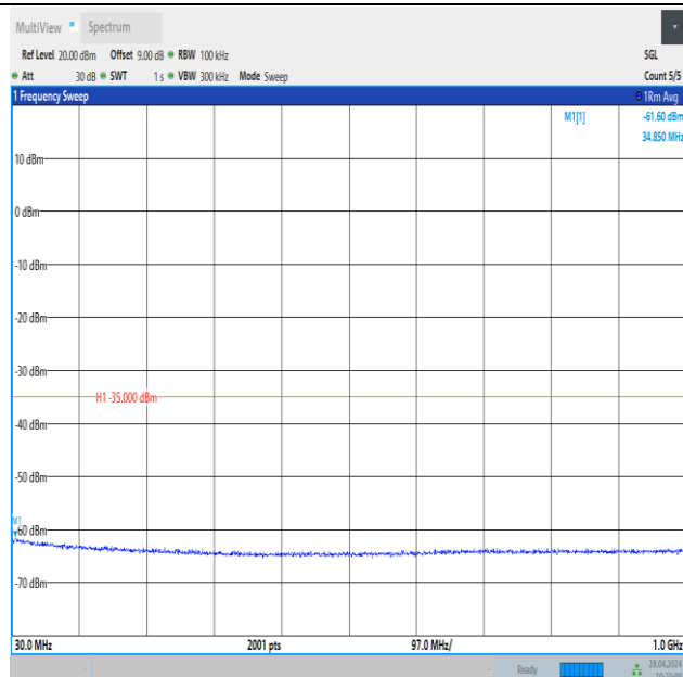
Band41_10MHz_QPSK_41540_50RB#0_30~1000_30~1000
