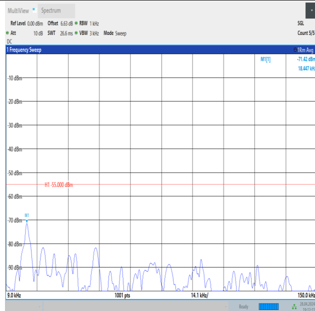
Band41_15MHz_16QAM_40620_1RB#0_0.009~0.15_0.009~0.15
