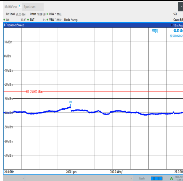
Band41_10MHz_QPSK_39700_50RB#0_20000~27000_20000~27000
