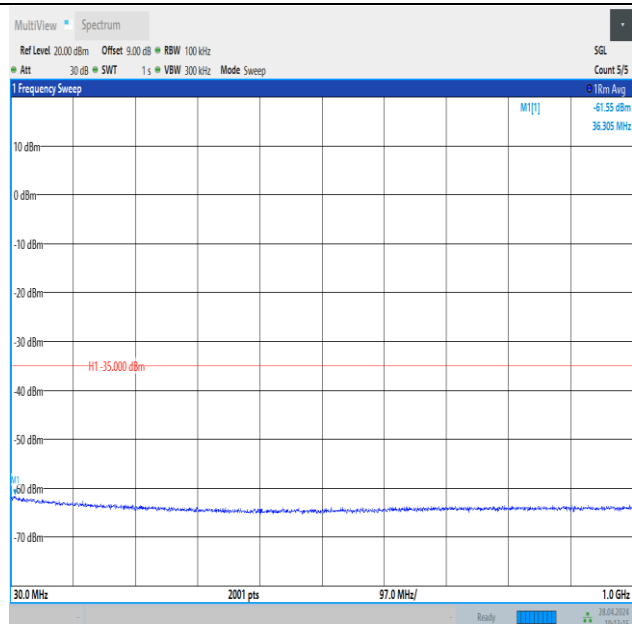
Band41_15MHz_QPSK_40620_1RB#74_30~1000_30~1000
