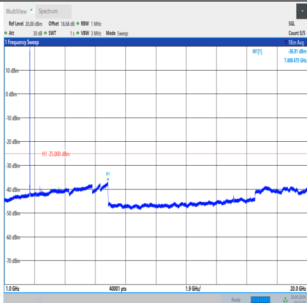
Band41_10MHz_QPSK_40620_50RB#0_1000~20000_1000~20000
