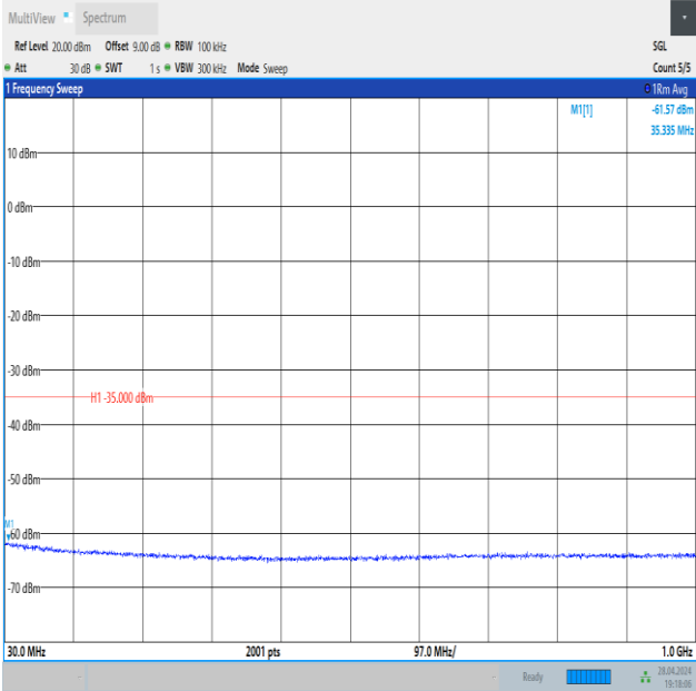
Band41_15MHz_16QAM_41515_1RB#0_30~1000_30~1000
