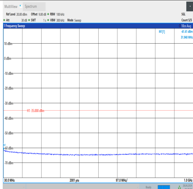
Band41_10MHz_QPSK_39700_1RB#49_30~1000_30~1000
