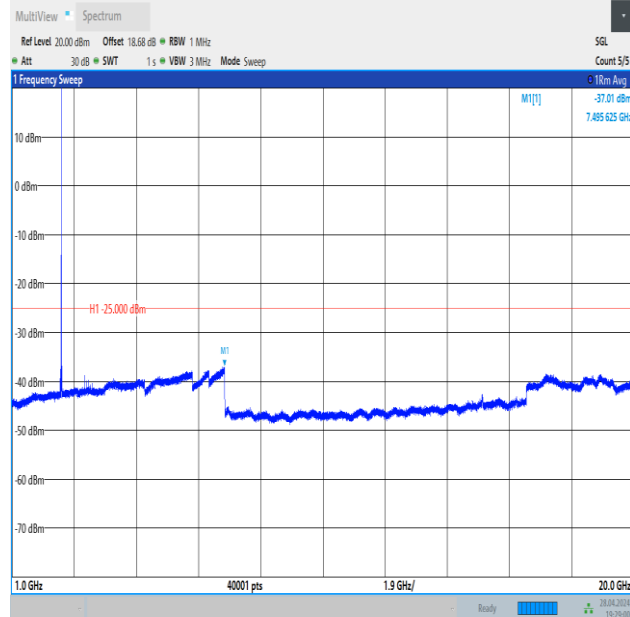
Band41_10MHz_16QAM_39700_1RB#49_1000~20000_1000~20000
