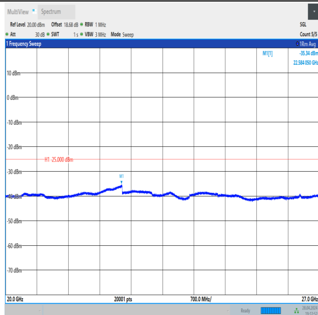
Band41_15MHz_16QAM_40620_1RB#0_20000~27000_20000~27000
