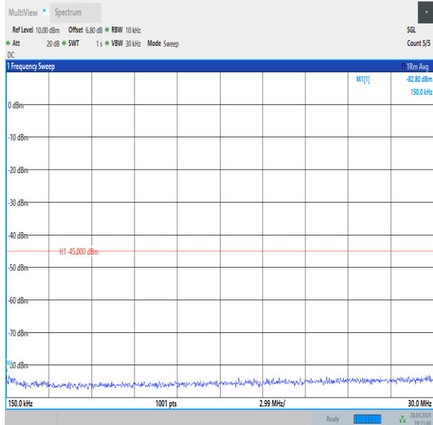
Band41_15MHz_QPSK_40620_1RB#74_0.15~30_0.15~30
