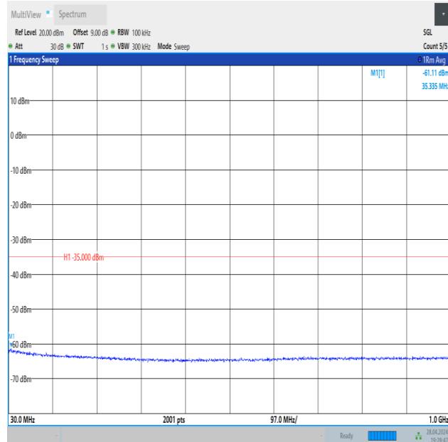
Band41_10MHz_16QAM_39700_1RB#49_30~1000_30~1000
