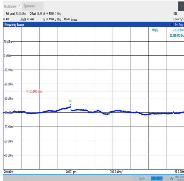
Band41_15MHz_16QAM_41515_1RB#74_20000~27000_20000~27000
