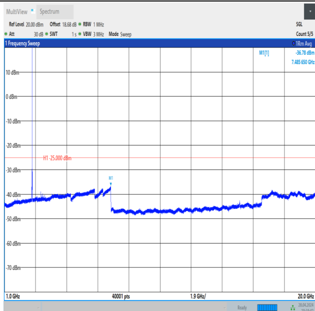
Band41_10MHz_QPSK_41540_1RB#49_1000~20000_1000~20000
