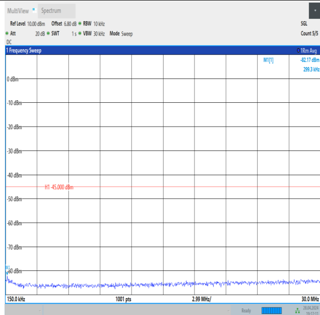
Band41_15MHz_QPSK_41515_1RB#0_0.15~30_0.15~30
