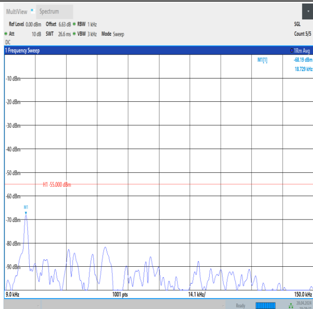
Band41_10MHz_16QAM_39700_1RB#49_0.009~0.15_0.009~0.15
