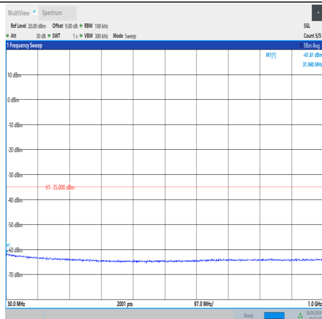
Band41_15MHz_QPSK_41515_1RB#0_30~1000_30~1000
