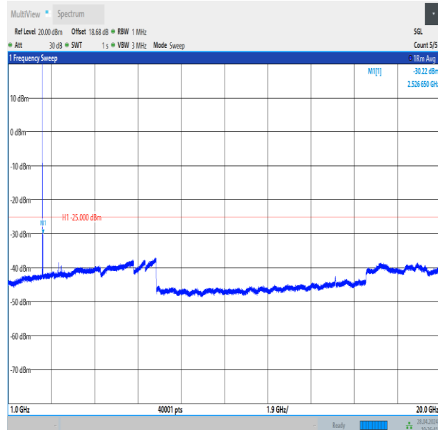
Band41_10MHz_QPSK_39700_1RB#0_1000~20000_1000~20000
