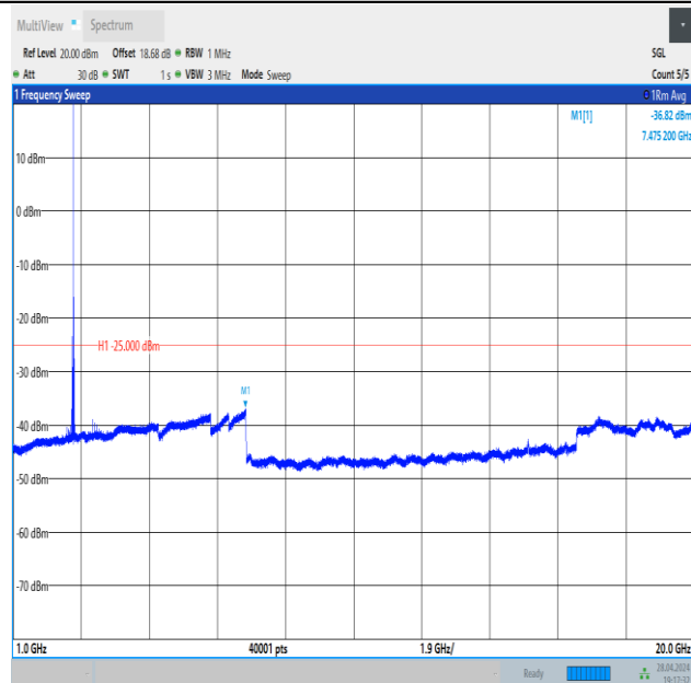
Band41_15MHz_QPSK_41515_1RB#0_1000~20000_1000~20000
