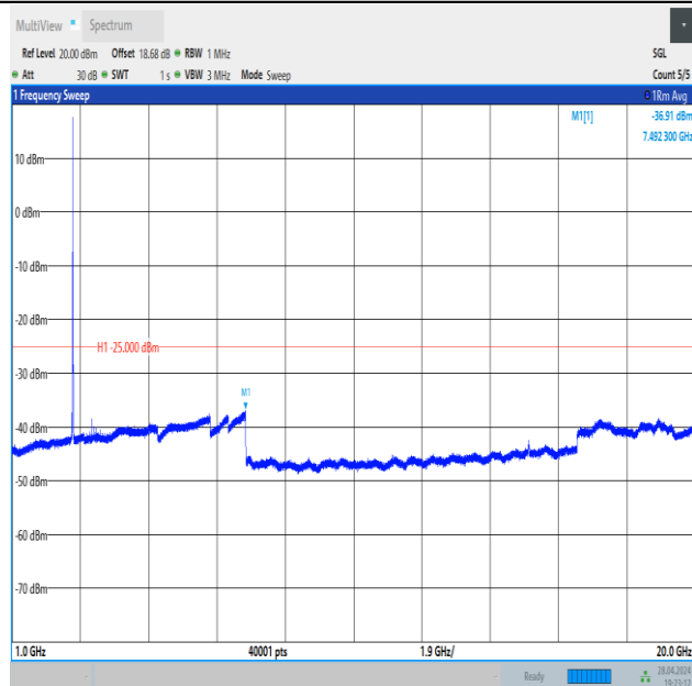
Band41_10MHz_QPSK_41540_50RB#0_1000~20000_1000~20000
