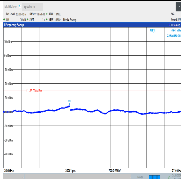
Band41_15MHz_QPSK_40620_1RB#0_20000~27000_20000~27000
