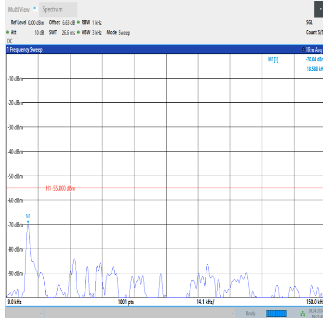
Band41_10MHz_QPSK_40620_50RB#0_0.009~0.15_0.009~0.15
