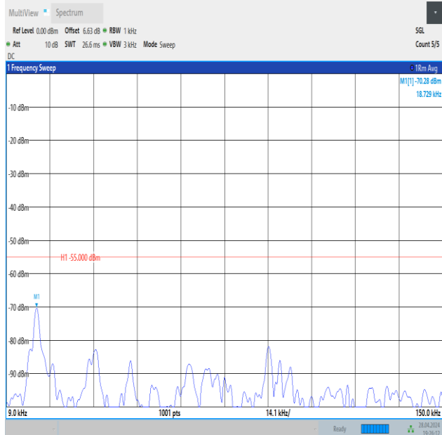
Band41_10MHz_QPSK_39700_1RB#0_0.009~0.15_0.009~0.15
