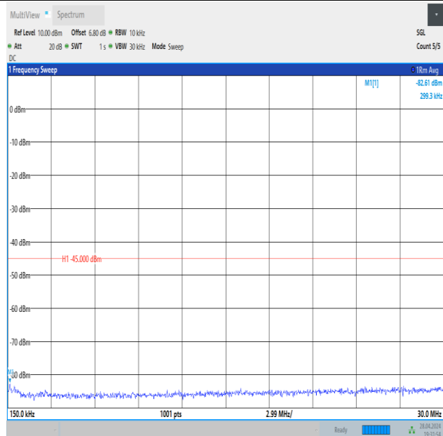
Band41_10MHz_16QAM_40620_1RB#49_0.15~30_0.15~30
