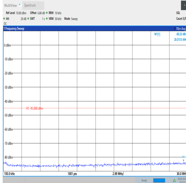
Band41_10MHz_QPSK_41540_50RB#0_0.15~30_0.15~30
