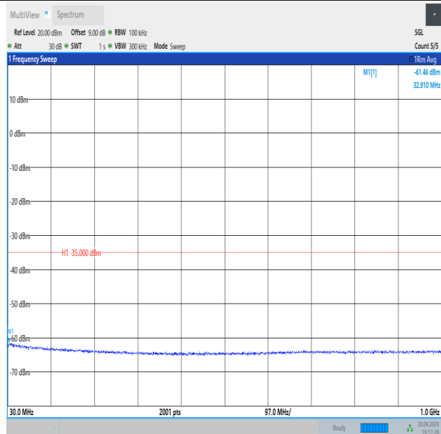
Band41_15MHz_16QAM_40620_1RB#0_30~1000_30~1000
