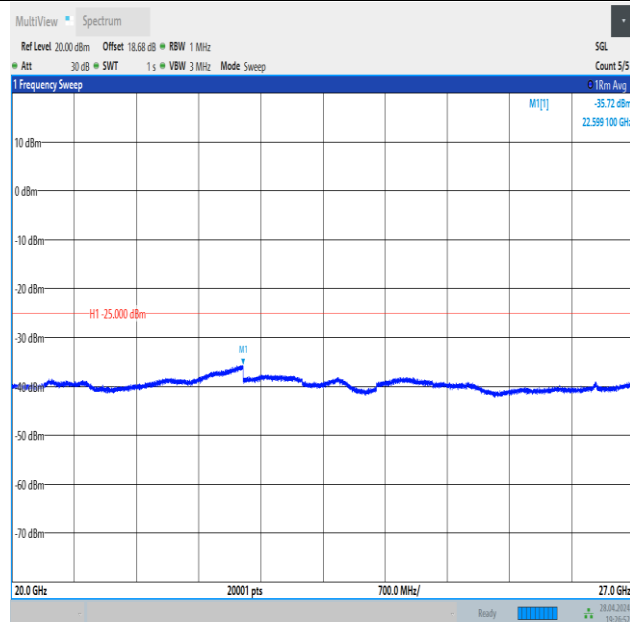
Band41_10MHz_QPSK_39700_1RB#0_20000~27000_20000~27000
