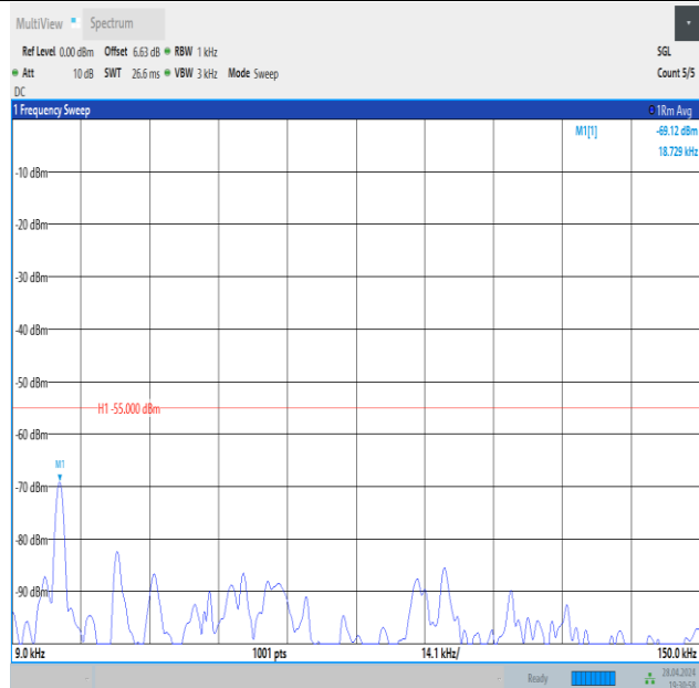
Band41_10MHz_QPSK_40620_1RB#49_0.009~0.15_0.009~0.15
