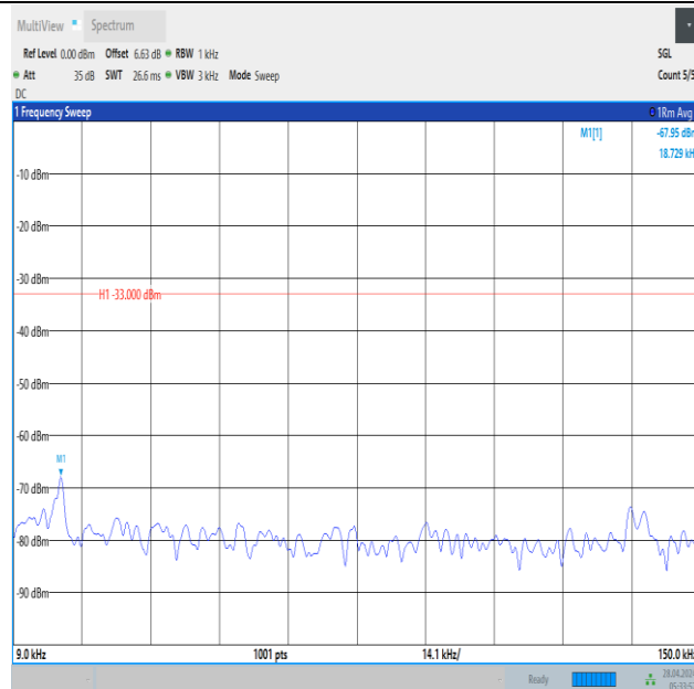
Band12_5MHz_QPSK_23035_1RB#24_0.009~0.15_0.009~0.15
