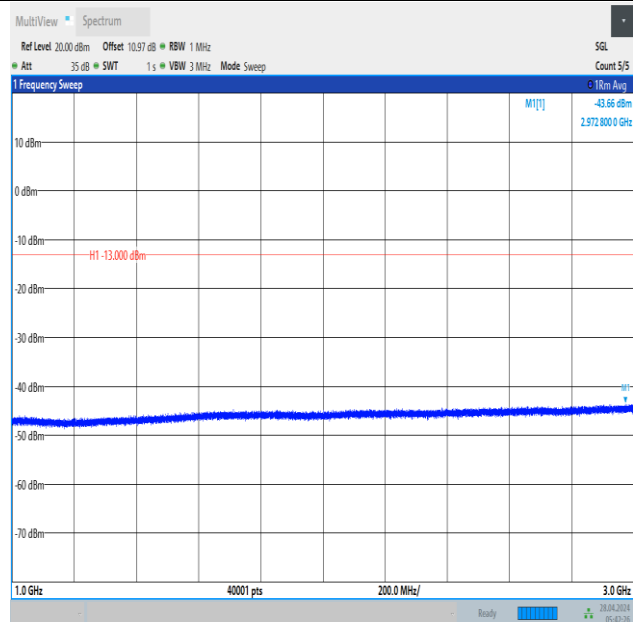
Band12_5MHz_QPSK_23155_1RB#0_1000~3000_1000~3000
