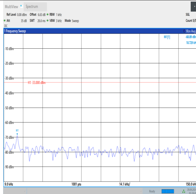
Band12_5MHz_16QAM_23035_1RB#24_0.009~0.15_0.009~0.15
