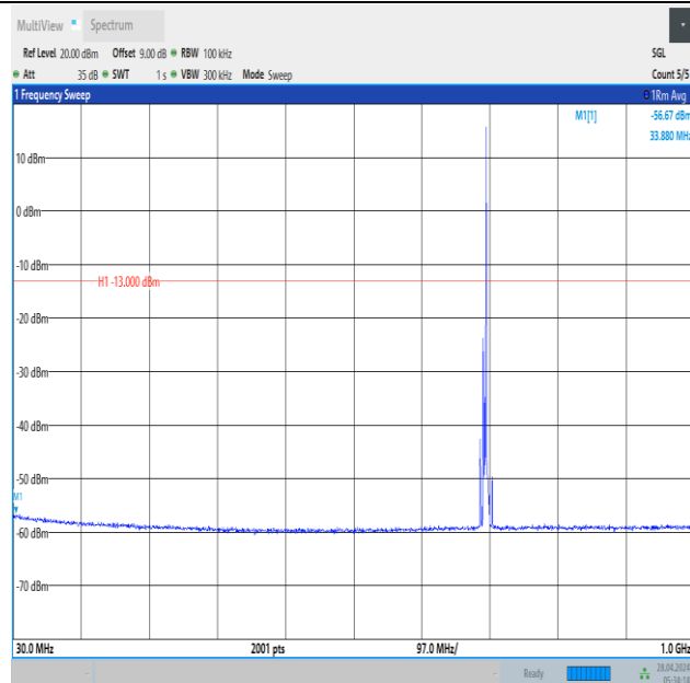
Band12_5MHz_QPSK_23035_1RB#24_30~1000_30~1000
