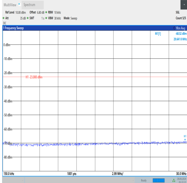
Band12_5MHz_QPSK_23035_1RB#0_0.15~30_0.15~30
