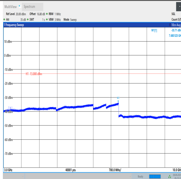
Band12_1.4MHz_QPSK_23173_1RB#0_3000~10000_3000~10000
