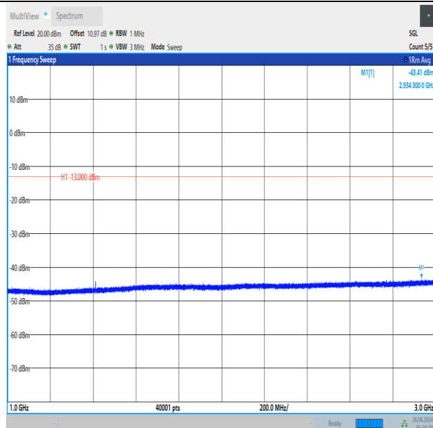
Band12_5MHz_16QAM_23095_1RB#0_1000~3000_1000~3000
