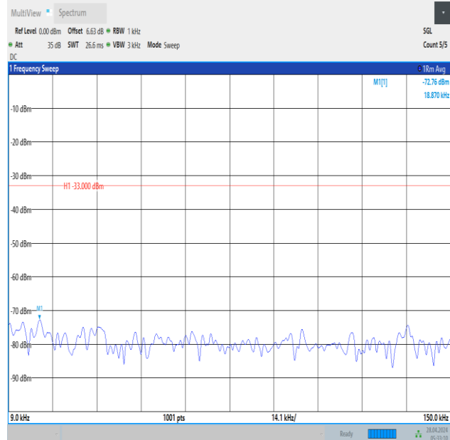
Band12_5MHz_16QAM_23035_1RB#0_0.009~0.15_0.009~0.15
