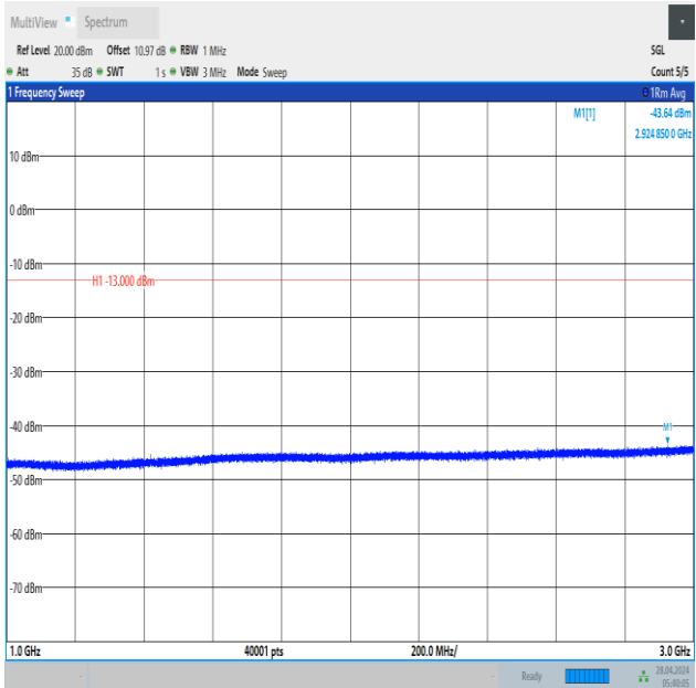
Band12_5MHz_16QAM_23095_1RB#24_1000~3000_1000~3000
