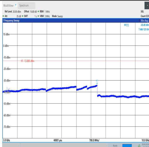
Band12_5MHz_16QAM_23095_1RB#0_3000~10000_3000~10000
