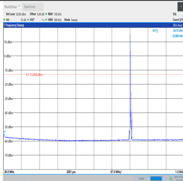
Band12_5MHz_16QAM_23155_1RB#0_30~1000_30~1000
