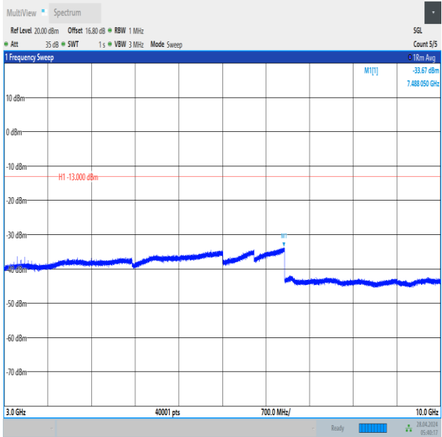
Band12_5MHz_16QAM_23095_1RB#24_3000~10000_3000~10000
