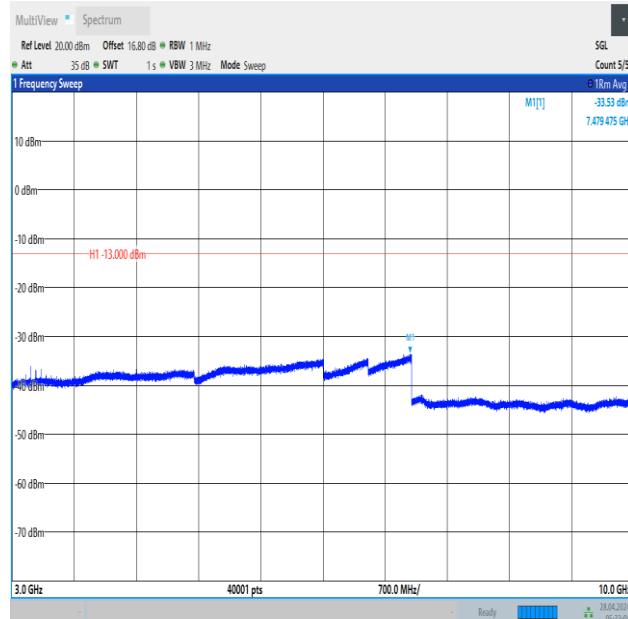
Band12_5MHz_QPSK_23035_1RB#0_3000~10000_3000~10000
