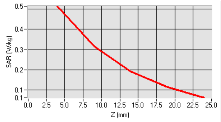
SAR, Z Axis Scan (X = 2, Y = 11)
