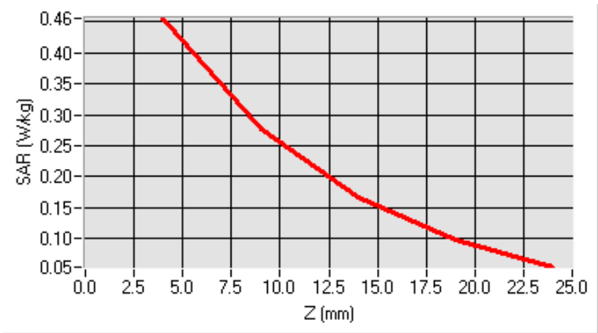
SAR, Z Axis Scan (X = -3, Y = 17)
