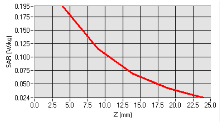
SAR, Z Axis Scan (X = -5, Y = 26)
