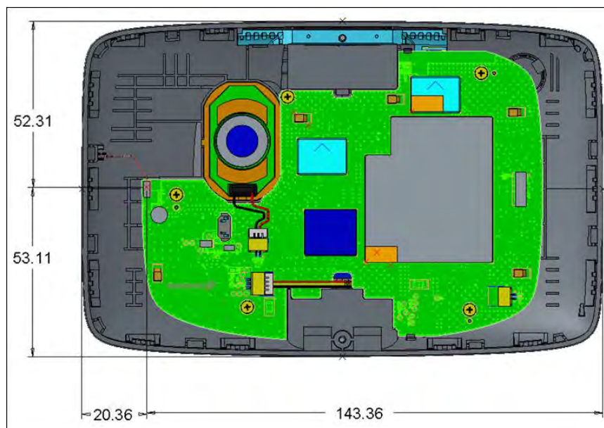
Fig.11 antenna location
