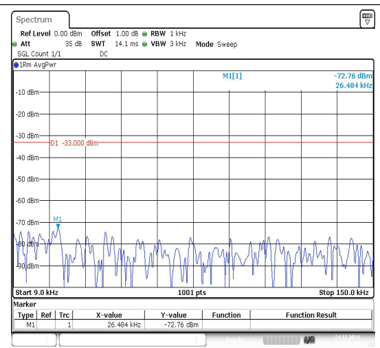
Band26_1.4MHz_16QAM_27033_1RB#0_0.009~0.15
