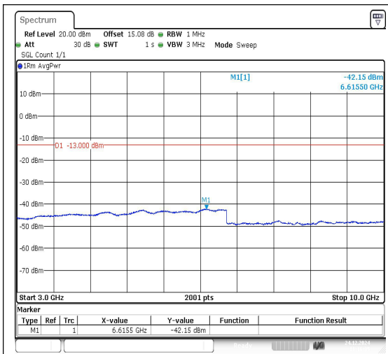
Band26_1.4MHz_QPSK_27033_1RB#0_3000~10000
