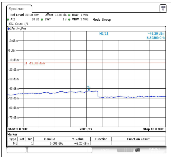
Band26_1.4MHz_QPSK_26915_1RB#0_3000~10000
