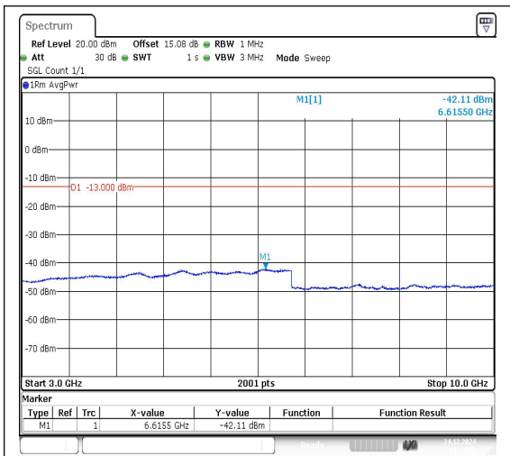
Band26_1.4MHz_QPSK_26797_1RB#0_3000~10000
