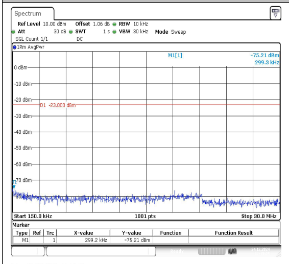
Band26_1.4MHz_16QAM_26915_1RB#0_0.15~30
