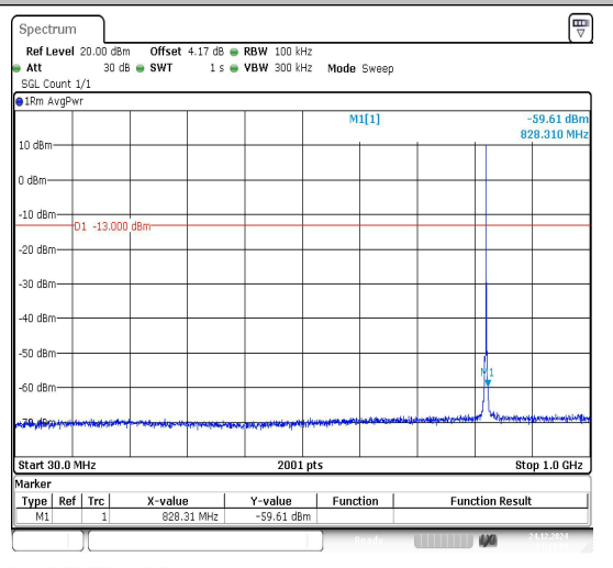
Band26_1.4MHz_16QAM_26797_1RB#0_30~100_0_30~1000
