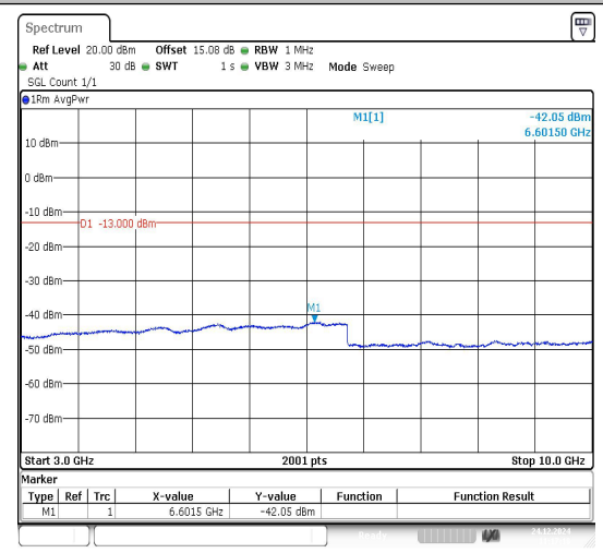
Band26_1.4MHz_16QAM_27033_1RB#0_30~100
