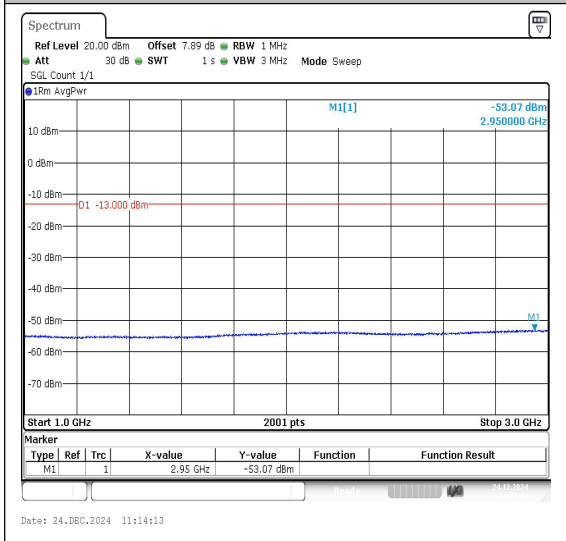
Band26_1.4MHz_16QAM_26797_1RB#0_0.15~3_0_0.15~30
