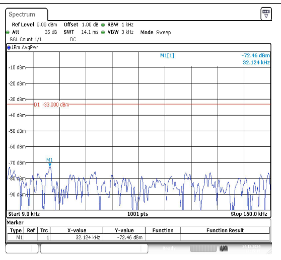
Band26_1.4MHz_16QAM_26915_1RB#0_0.009~0.15
