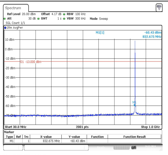
Band26_1.4MHz_16QAM_26915_1RB#0_30~100
