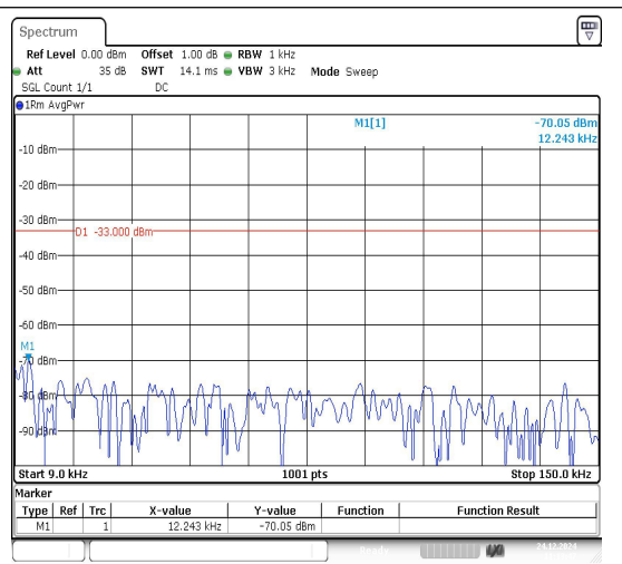
Band26_1.4MHz_16QAM_26797_1RB#0_0.009~0.15_0.009~0.15
