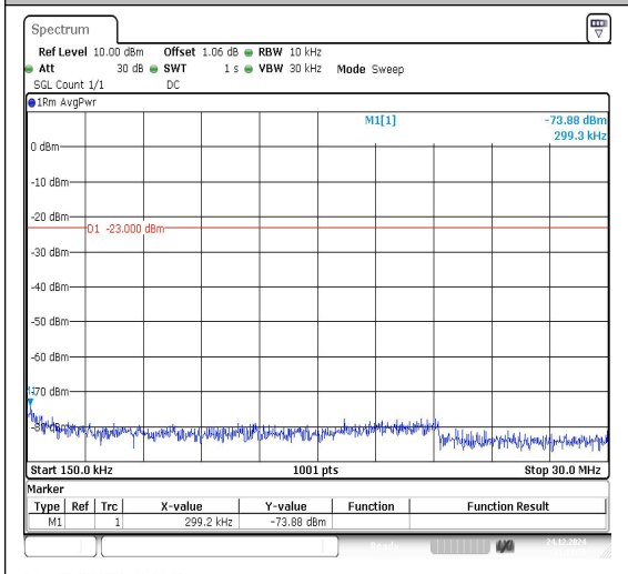
Band26_1.4MHz_16QAM_26797_1RB#0_0.15~3_0_0.15~30
