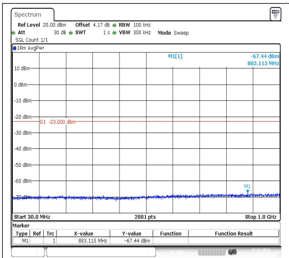
Band25_5MHz_QPSK_26065_1RB#0_30~1000 30~1000
