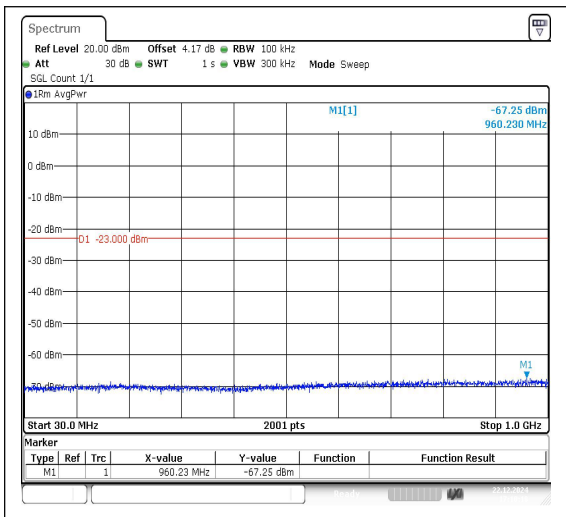
Band25_5MHz_QPSK_26665_1RB#0_30~1000 30~1000
