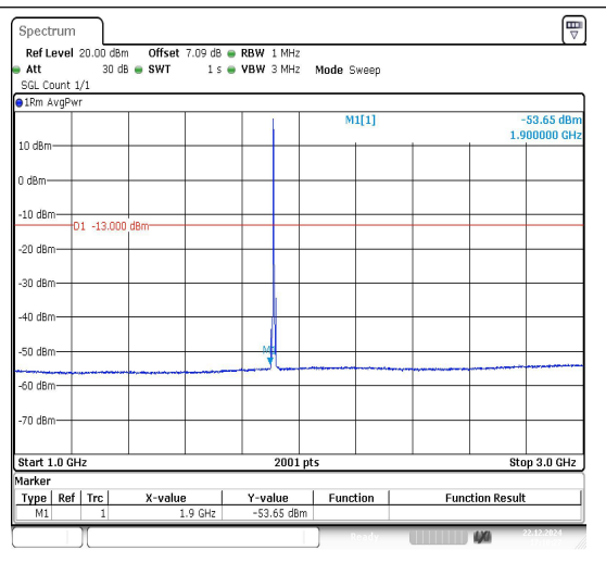
Band25_5MHz_QPSK_26665_1RB#0_1000~3000 1000~3000
