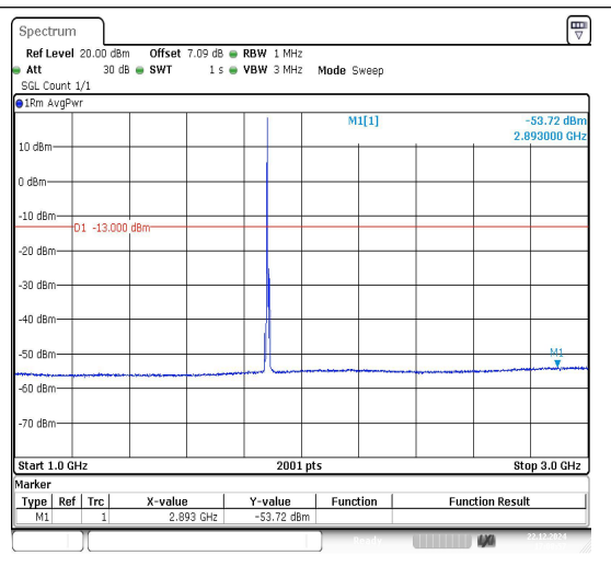
Band25_5MHz_QPSK_26365_1RB#0_1000~3000 _1000~3000
