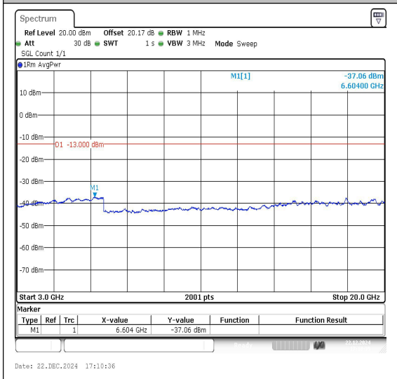
Band25_5MHz_QPSK_26665_1RB#0_3000~20000 00_3000~20000
