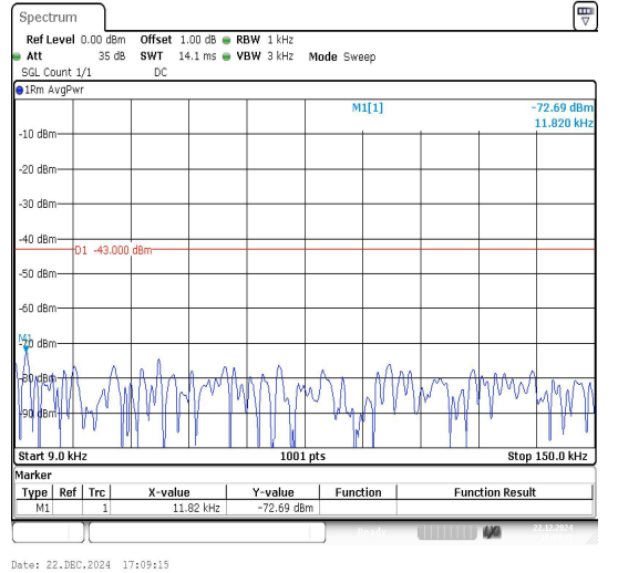
Band25_5MHz_16QAM_26365_1RB#0_0.009~0.15 5_0.009~0.15
