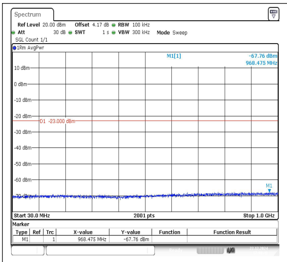
Band25_5MHz_QPSK_26365_1RB#0_30~1000 30~1000
