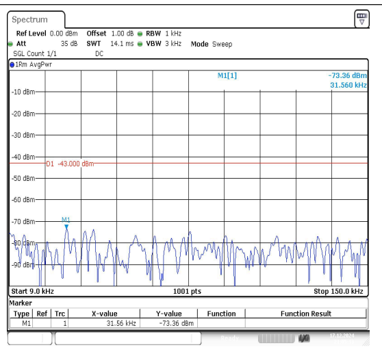
Band2_1.4MHz_16QAM_19193_1RB#0_0.009~0.15_0.009~0.15
