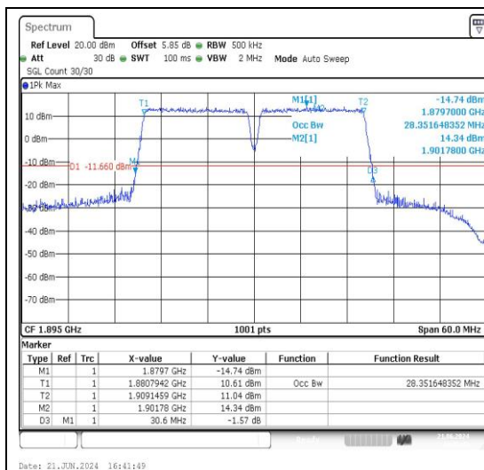
2-2-15MHz-15MHz-QPSK-QPSK-18975-19125-7 5RB#0-75RB#0-PASS
