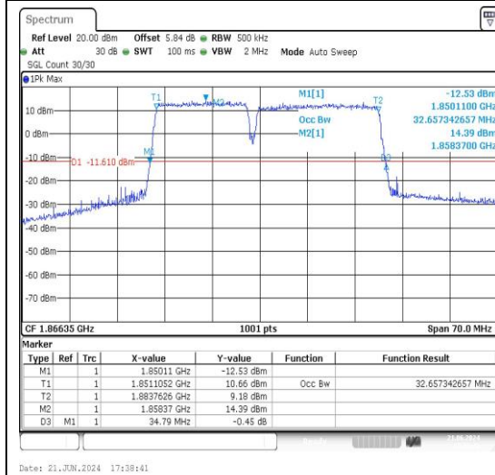
2-2-15MHz-20MHz-QPSK-QPSK-18678-18849-7 5RB#0-100RB#0-PASS
