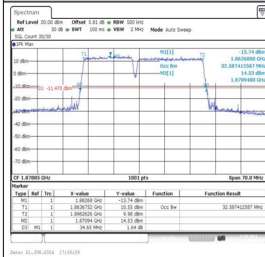
2-2-15MHz-20MHz-QPSK-QPSK-18678-18849-7 5RB#0-100RB#0-PASS
