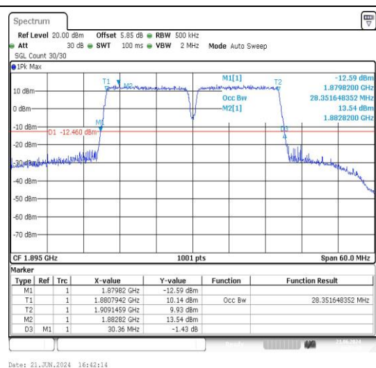
2-2-15MHz-15MHz-16QAM-16QAM-18975-19125- 75RB#0-75RB#0-PASS
