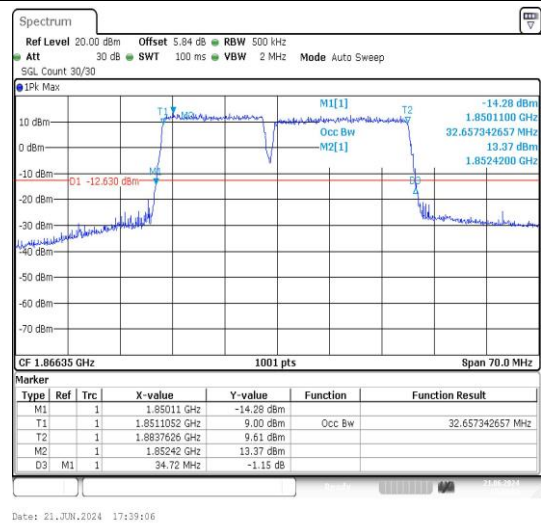
2-2-15MHz-20MHz-16QAM-16QAM-18678-18849- 75RB#0-100RB#0-PASS
