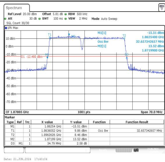
2-2-15MHz-20MHz-16QAM-16QAM-18678-18849- 75RB#0-100RB#0-PASS
