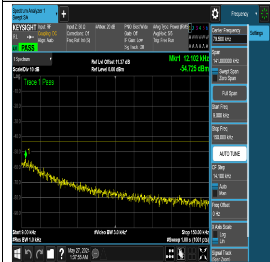
NTNV_DC_5A_n77A-3700-3980_PC2_30_5+70_ M+H_TID8_NS_01_0.009_0.15_#1
