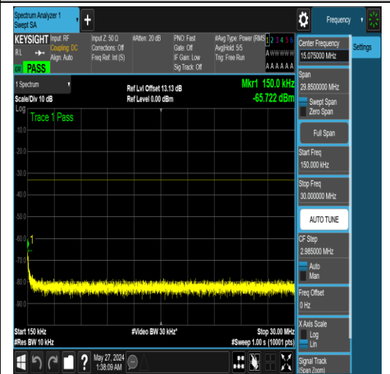
NTNV_DC_5A_n77A-3700-3980_PC2_30_5+70_ M+H_TID8_NS_01_0.15_30_#1
