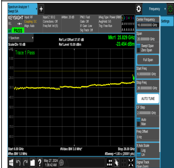
NTNV_DC_5A_n77A-3700-3980_PC2_30_5+70_ M+H_TID8_NS_01_0.009_0.15_#1
