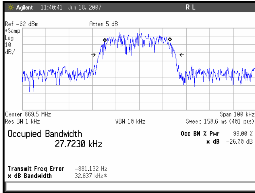
Plot 28. TDMA Downlink Low Channel Input
