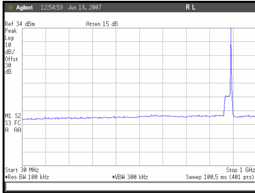
Plot 76. TDMA Downlink Conducted Emissions 30 MHz – 1GHz, High Channel
