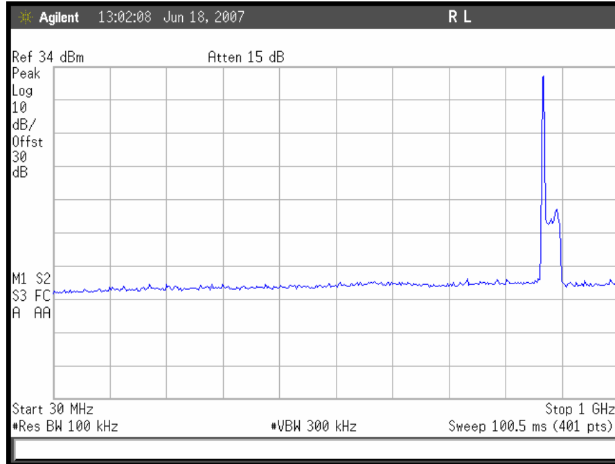
Plot 56. GSM Downlink Conducted Emissions 30 MHz – 1GHz, Low Channel
