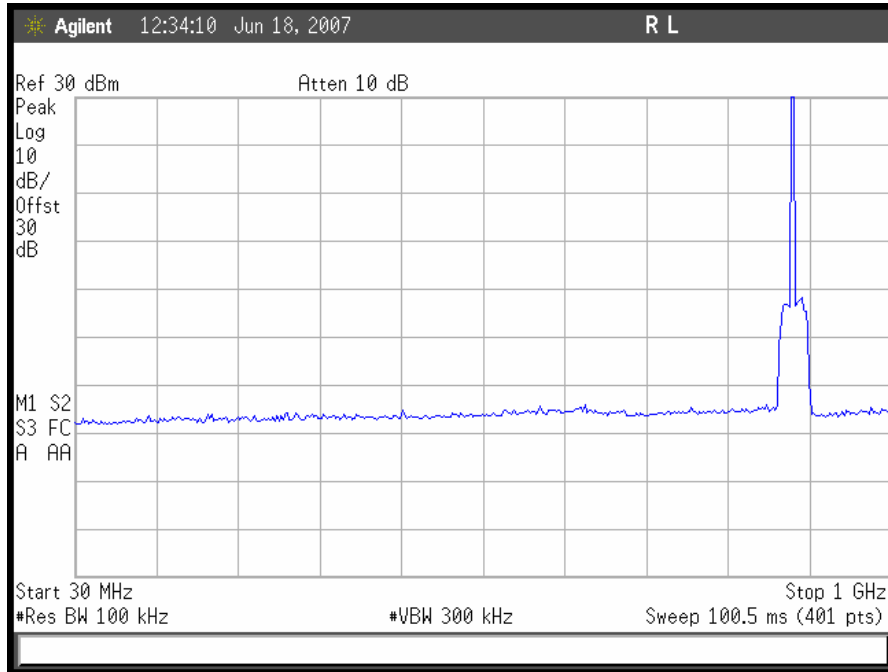
Plot 50. CDMA Uplink Conducted Emissions 30 MHz – 1GHz, Mid Channel
