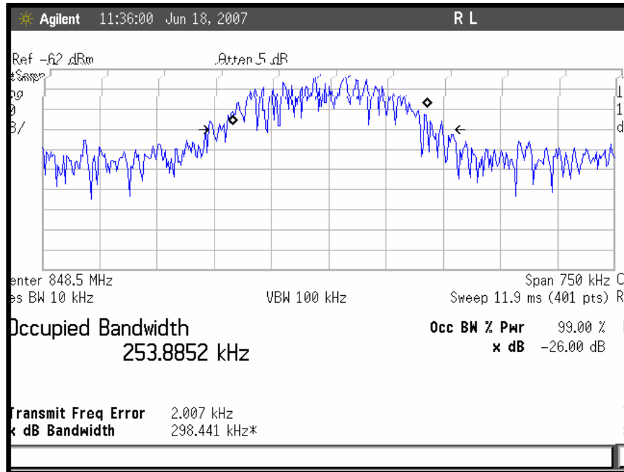
Plot 26. GSM Uplink High Channel Input
