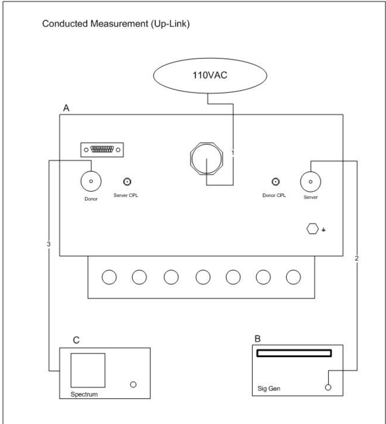
Figure 3. Block Diagram of Test Configuration (Conducted Measurement-Uplink)
