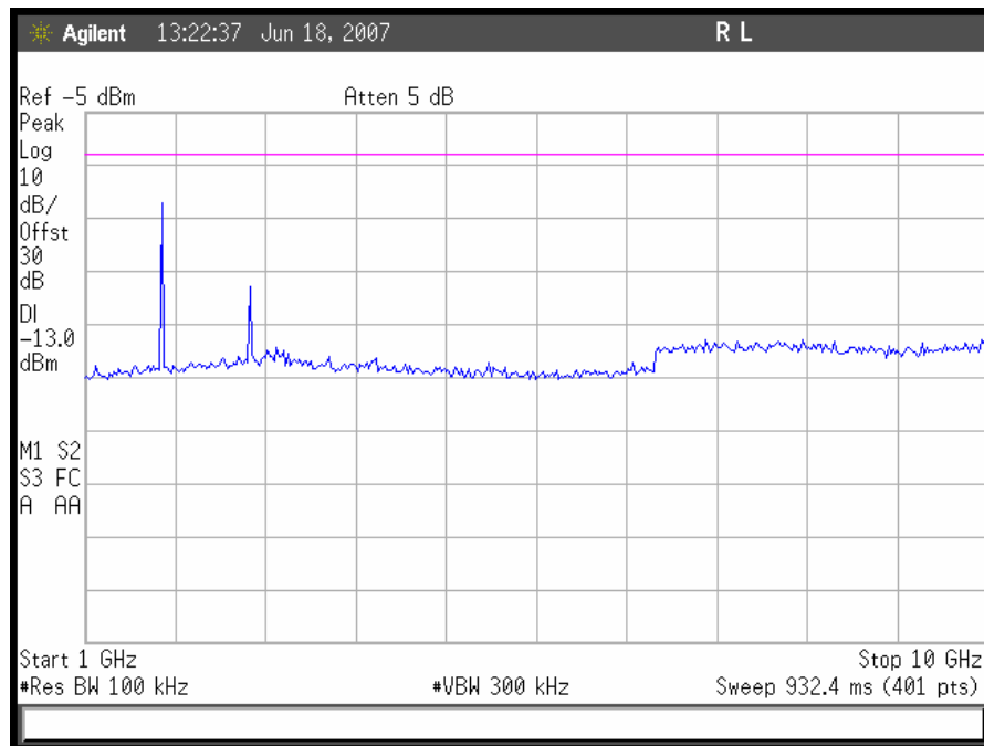
Plot 59. GSM Downlink Conducted Emissions 1 GHz – 10GHz, Mid Channel
