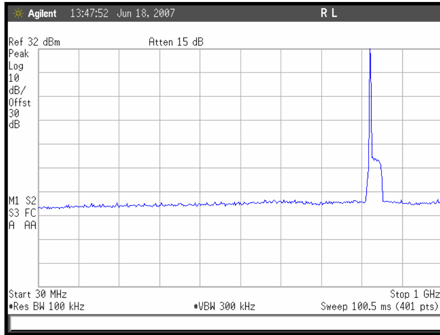
Plot 64. GSM Uplink Conducted Emissions 30 MHz – 1GHz, Low Channel
