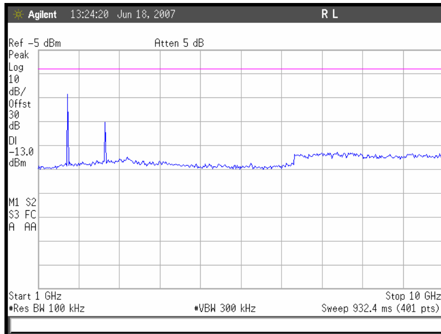
Plot 65. GSM Uplink Conducted Emissions 1 GHz – 10GHz, Low Channel
