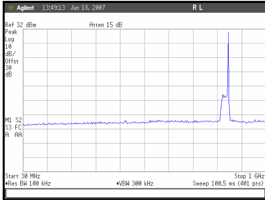
Plot 68. GSM Uplink Conducted Emissions 30 MHz - 1GHz, High Channel
