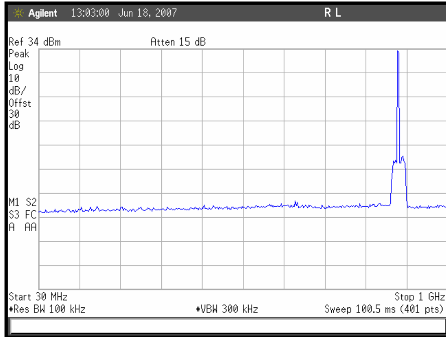
Plot 58. GSM Downlink Conducted Emissions 30 MHz – 1GHz, Mid Channel
