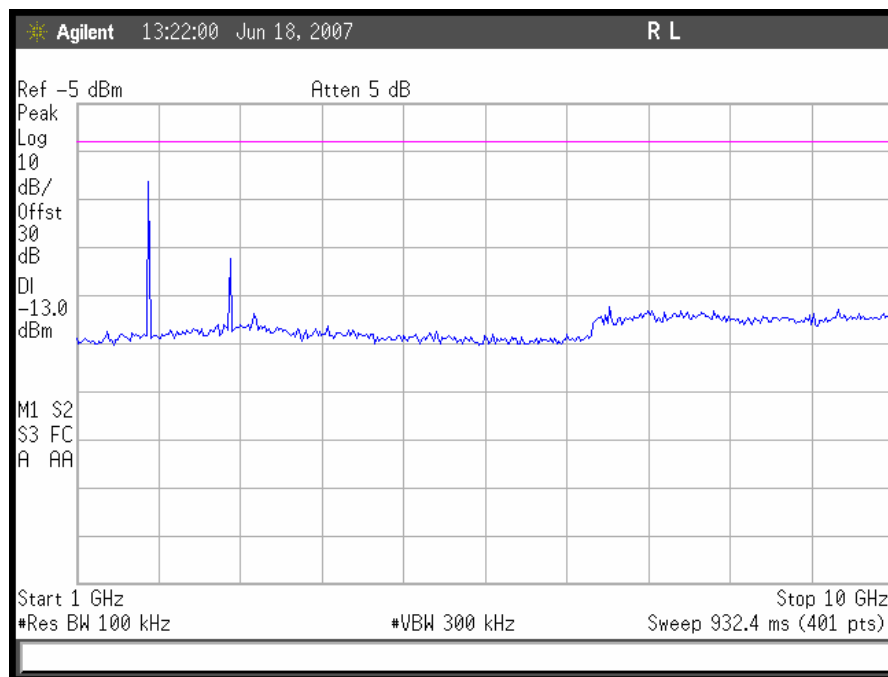
Plot 61. GSM Downlink Conducted Emissions 1 GHz – 10GHz, High Channel
