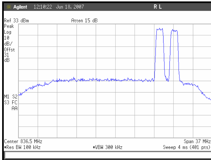
Plot 55. CDMA Intermodulation High End, Uplink
