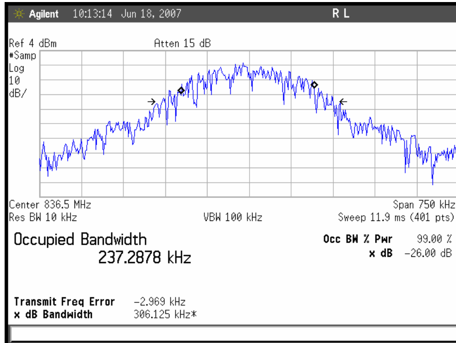
Plot 25. GSM Uplink Mid Channel Output
