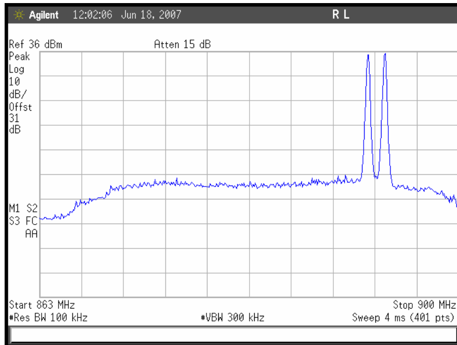
Plot 79. TDMA Intermodulation High End, Downlink
