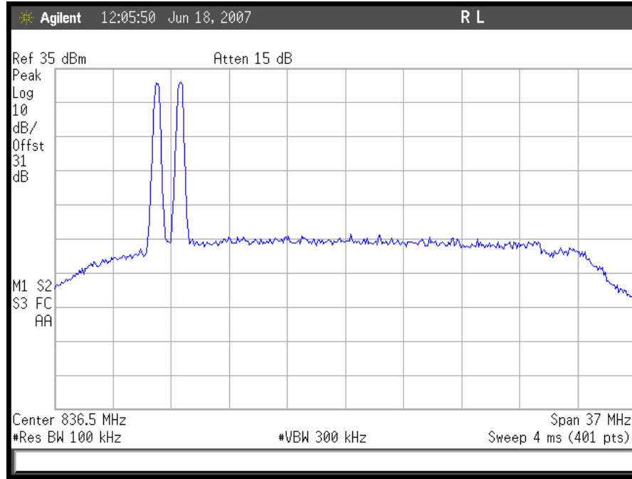
Plot 70. GSM Intermodulation Low End, Uplink
