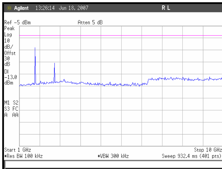
Plot 85. TDMA Uplink Conducted Emissions 1 GHz – 10GHz, High Channel
