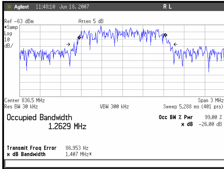
Plot 12. CDMA Uplink Mid Channel Input
