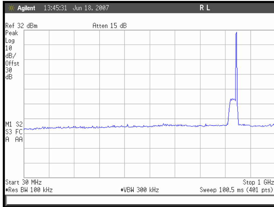
Plot 44. CDMA Downlink Conducted Emissions 30 MHz – 1GHz, High Channel
