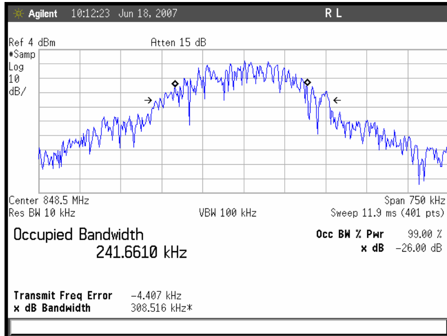
Plot 27. GSM Uplink High Channel Output
