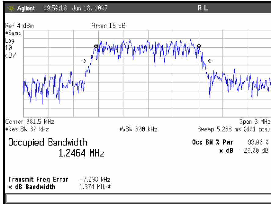
Plot 7. CDMA Downlink Mid Channel Output
