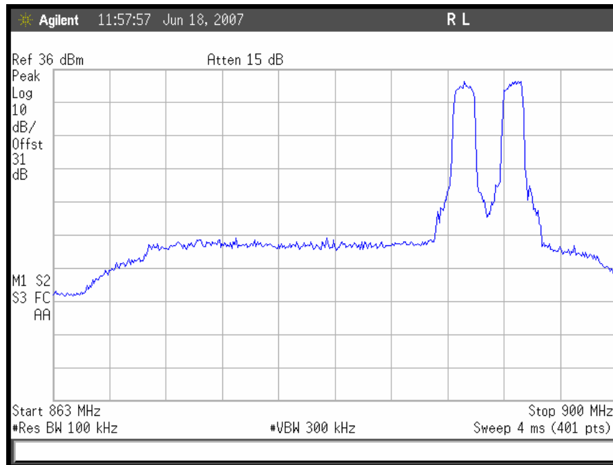
Plot 47. CDMA Intermodulation High End, Downlink
