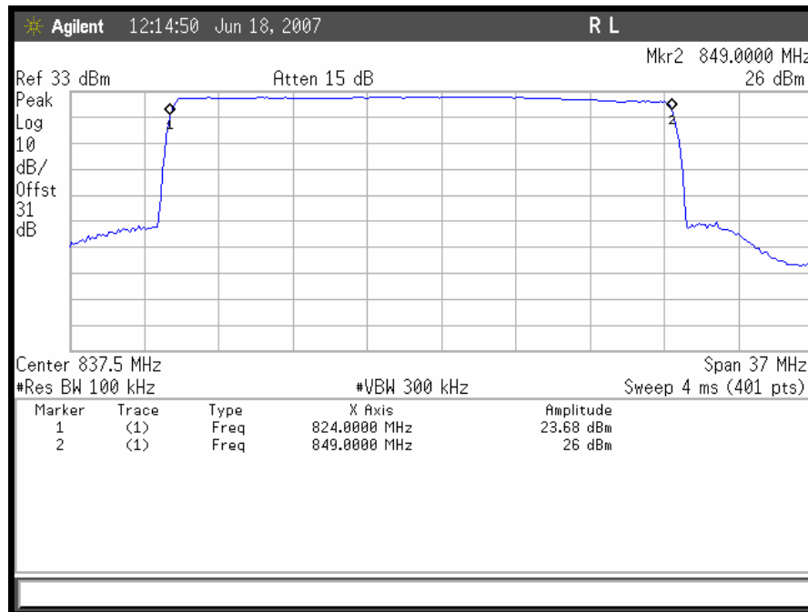
Plot 89. Out of Band Rejection - Uplink
