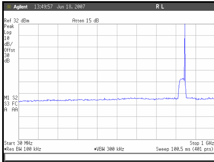
Plot 84. TDMA Uplink Conducted Emissions 30 MHz – 1GHz, High Channel
