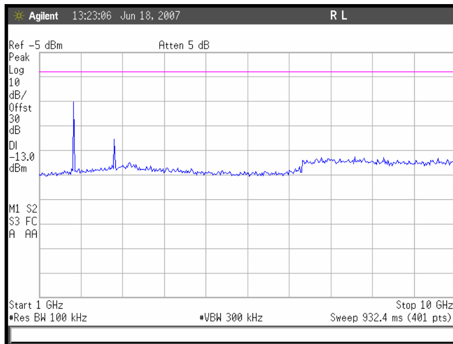
Plot 57. GSM Downlink Conducted Emissions 1 GHz – 10GHz, Low Channel
