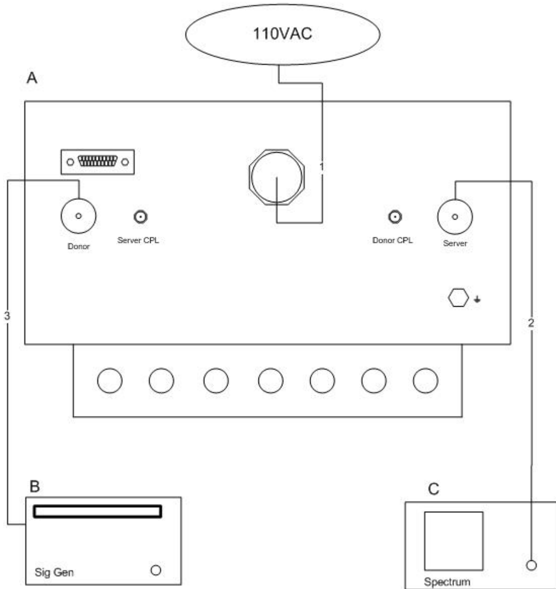
Figure 2. Block Diagram of Test Configuration (Conducted Measurement-Downlink)
