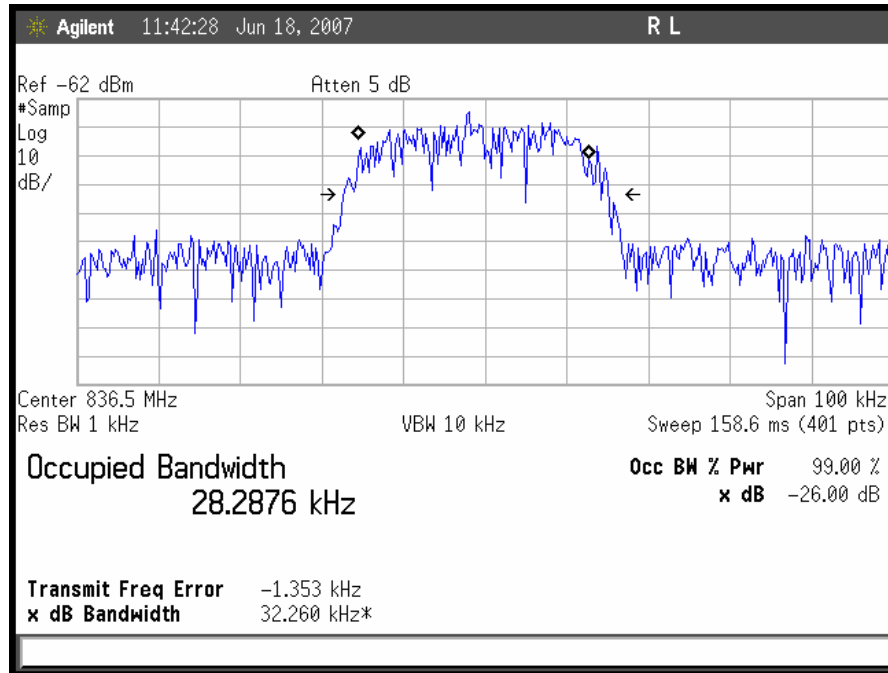
Plot 36. TDMA Uplink Mid Channel Input
