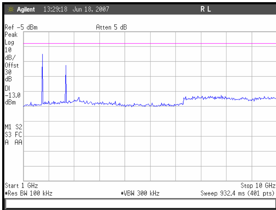
Plot 51. CDMA Uplink Conducted Emissions 1 GHz – 10GHz, Mid Channel
