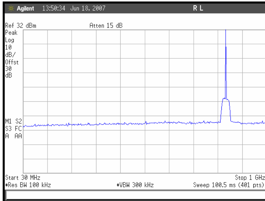
Plot 82. TDMA Uplink Conducted Emissions 30 MHz – 1GHz, Mid Channel
