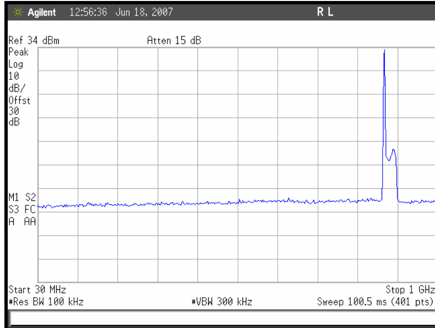
Plot 72. TDMA Downlink Conducted Emissions 30 MHz – 1GHz, Low Channel
