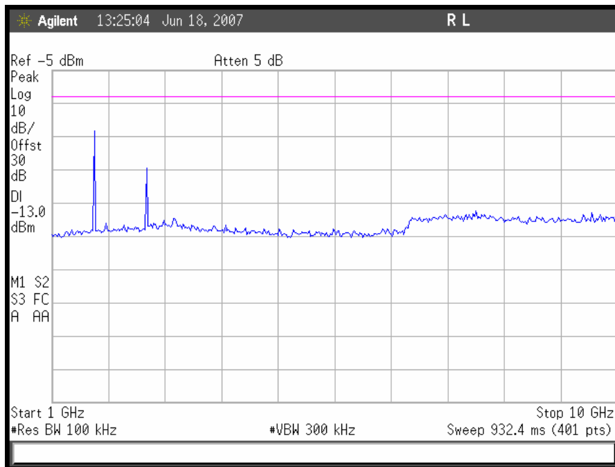
Plot 67. GSM Uplink Conducted Emissions 1 GHz – 10GHz, Mid Channel
