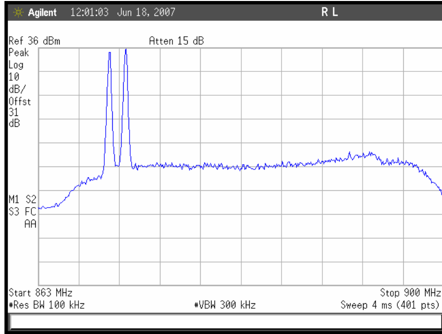
Plot 78. TDMA Intermodulation Low End, Downlink
