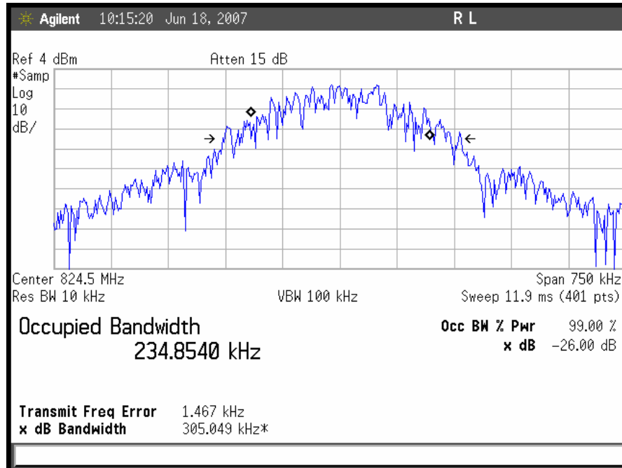
Plot 23. GSM Uplink Low Channel Output
