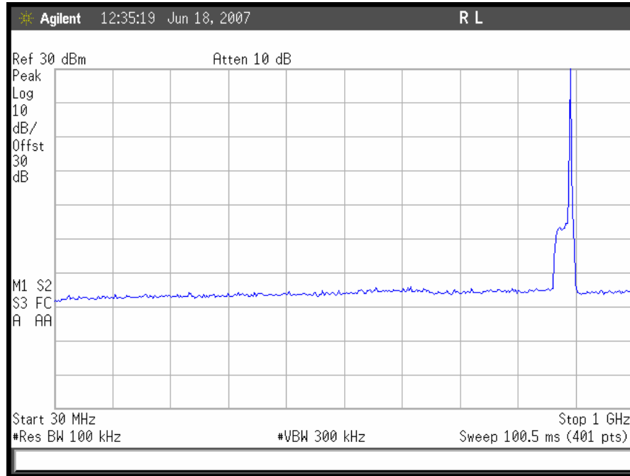
Plot 52. CDMA Uplink Conducted Emissions 30 MHz – 1GHz, High Channel
