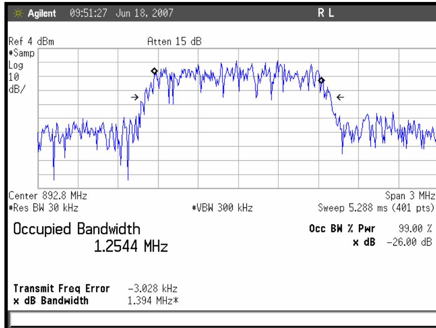
Plot 9. CDMA Downlink High Channel Output
