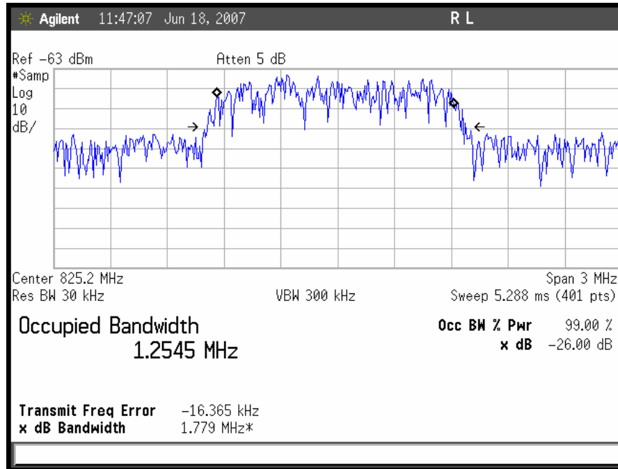
Plot 10. CDMA Uplink Low Channel Input
