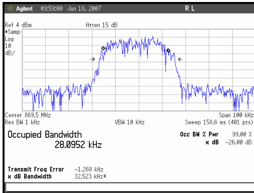
Plot 29. TDMA Downlink Low Channel Output
