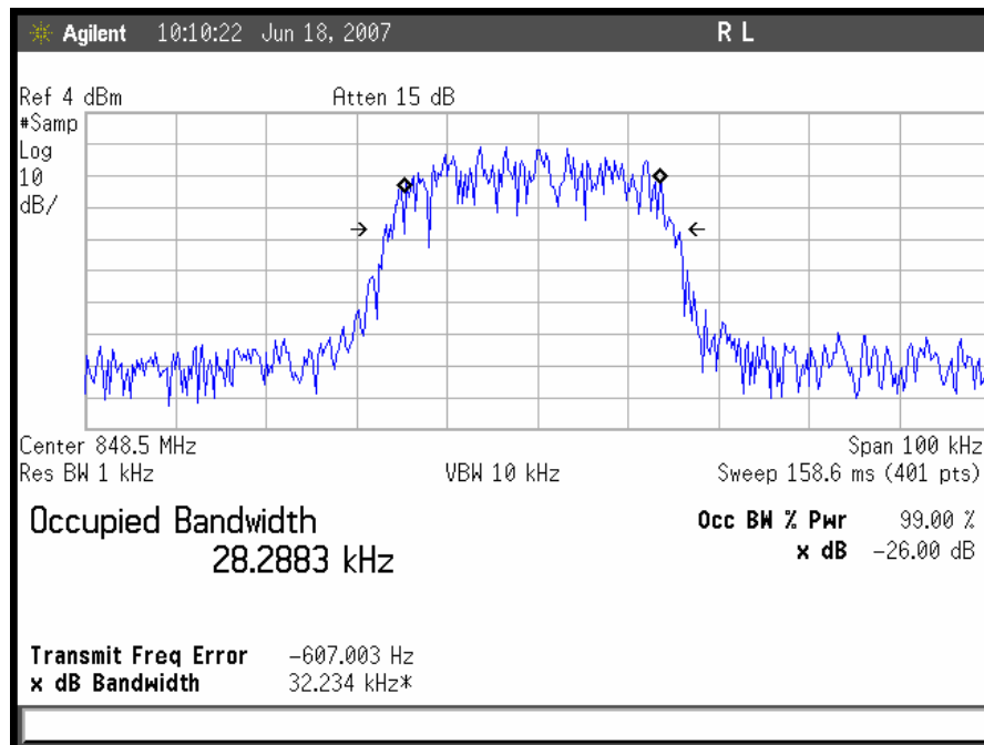
Plot 39. TDMA Uplink High Channel Output
