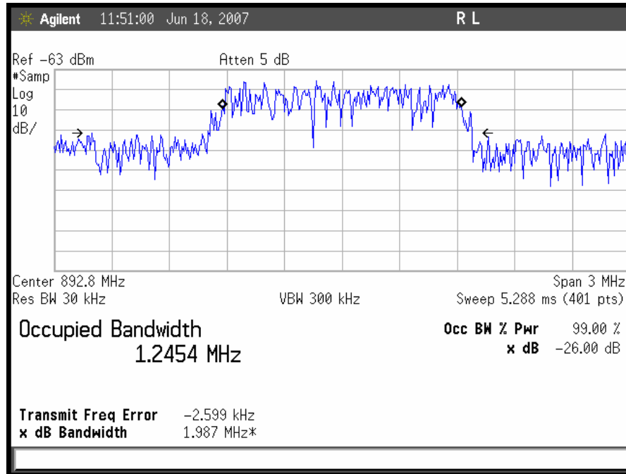
Plot 8. CDMA Downlink High Channel Input
