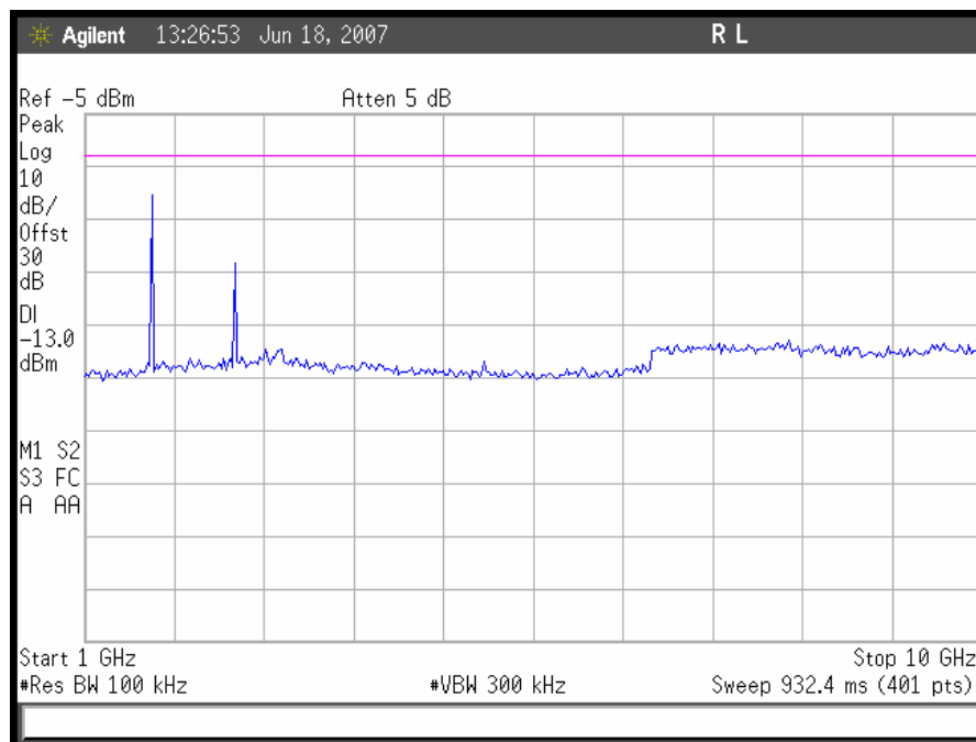
Plot 83. TDMA Uplink Conducted Emissions 1 GHz – 10GHz, Mid Channel
