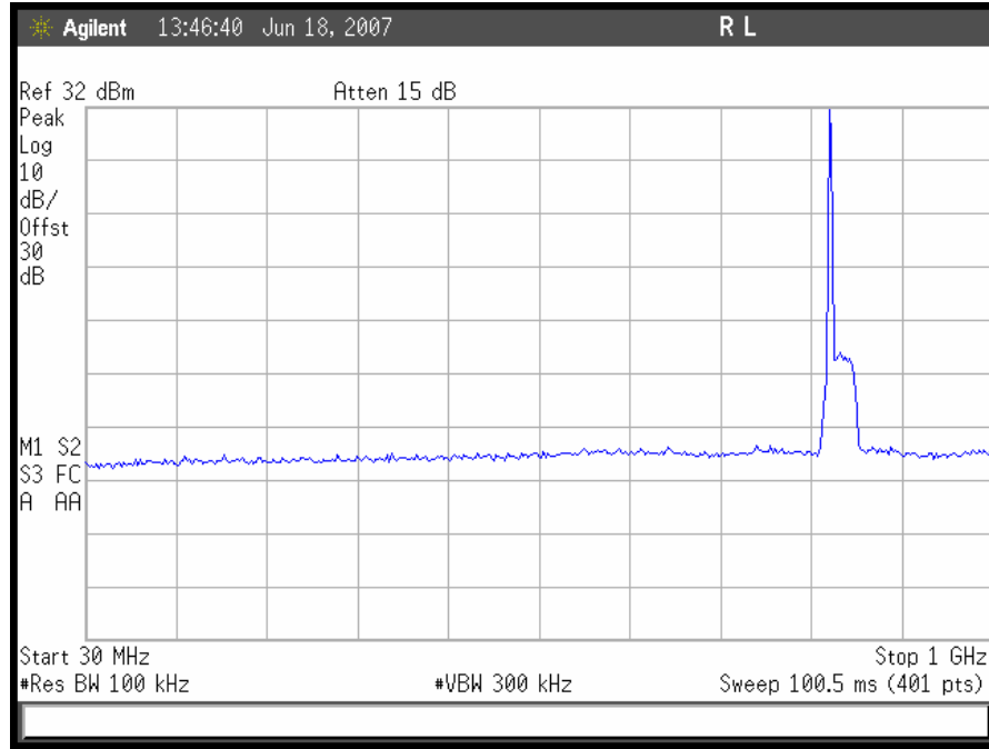
Plot 40. CDMA Downlink Conducted Emissions 30 MHz – 1GHz, Low Channel
