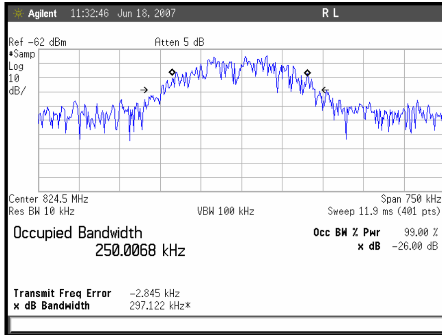
Plot 22. GSM Uplink Low Channel Input
