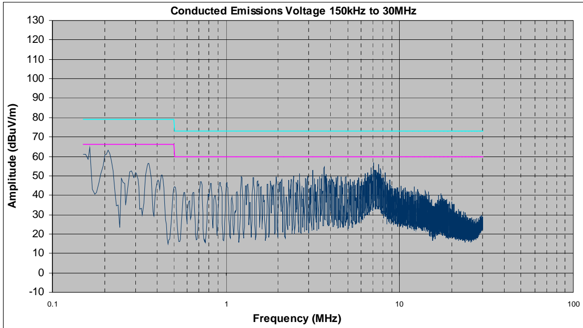
Plot 1. Conducted Emission, Phase Line Plots
