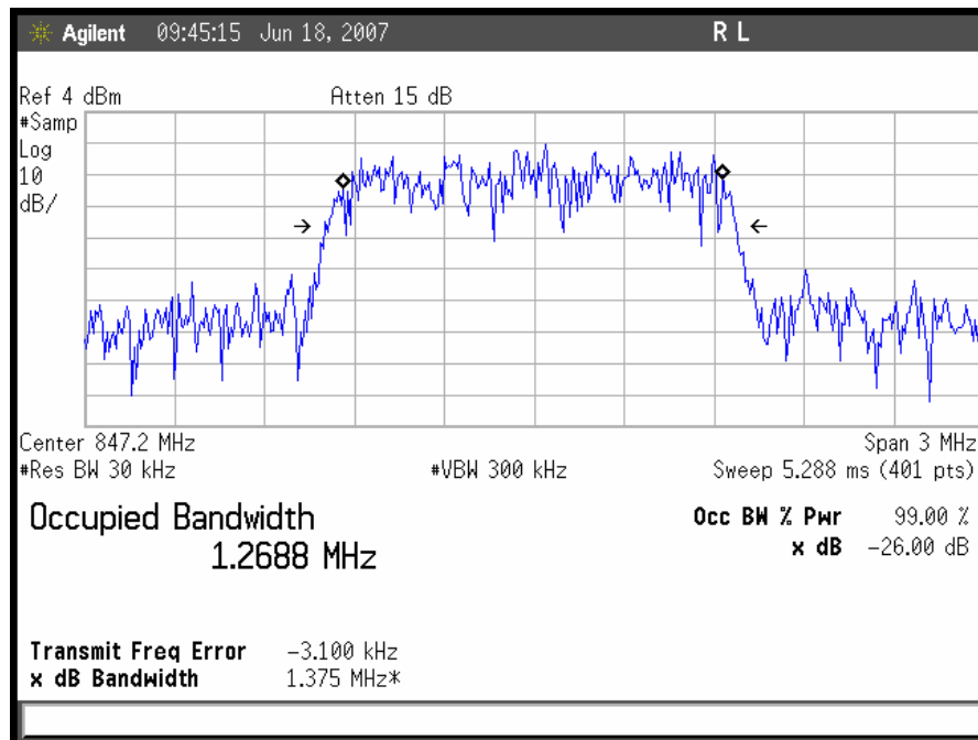
Plot 15. CDMA Uplink High Channel Output
