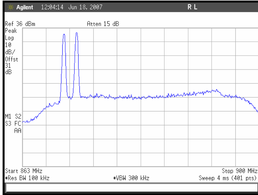
Plot 62. GSM Intermodulation Low End, Downlink
