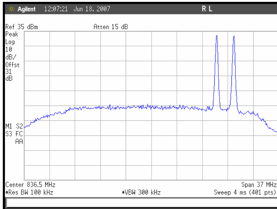
Plot 87. TDMA Intermodulation High End, Uplink
