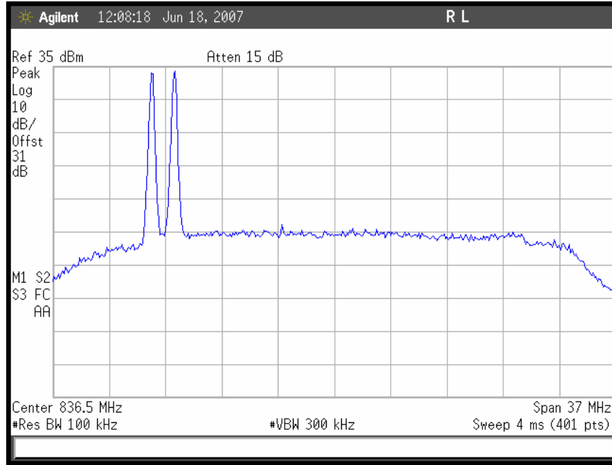
Plot 86. TDMA Intermodulation Low End, Uplink
