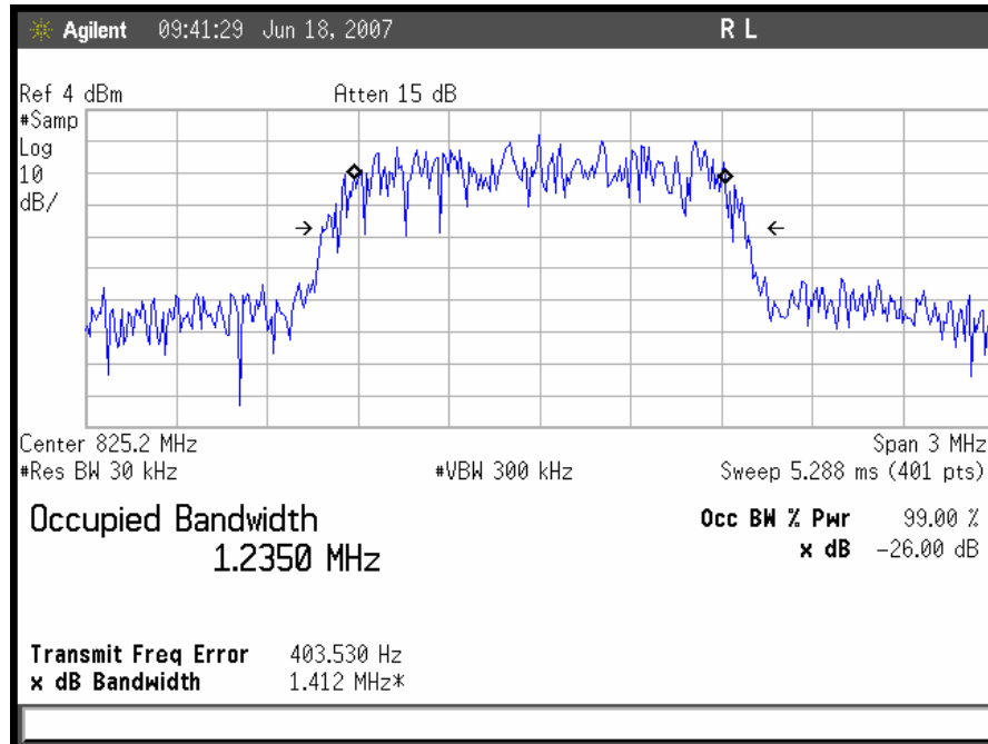
Plot 11. CDMA Uplink Low Channel Output
