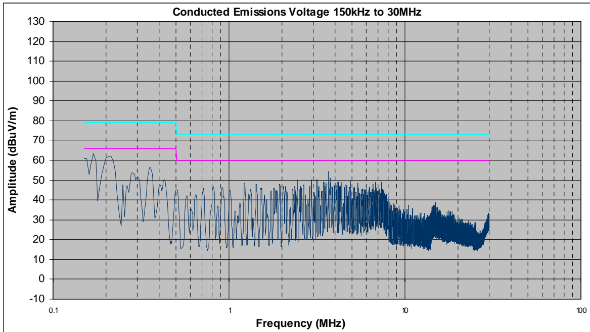
Plot 2. Conducted Emission, Neutral Line Plots
