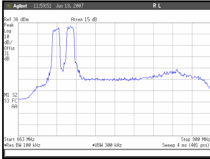
Plot 46. CDMA Intermodulation Low End, Downlink
