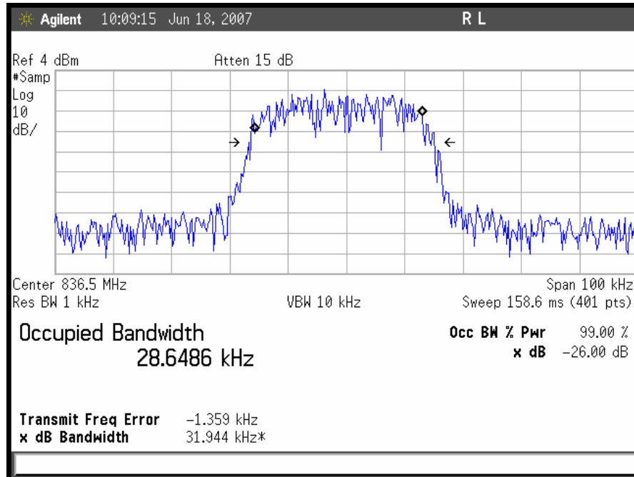
Plot 37. TDMA Uplink Mid Channel Output
