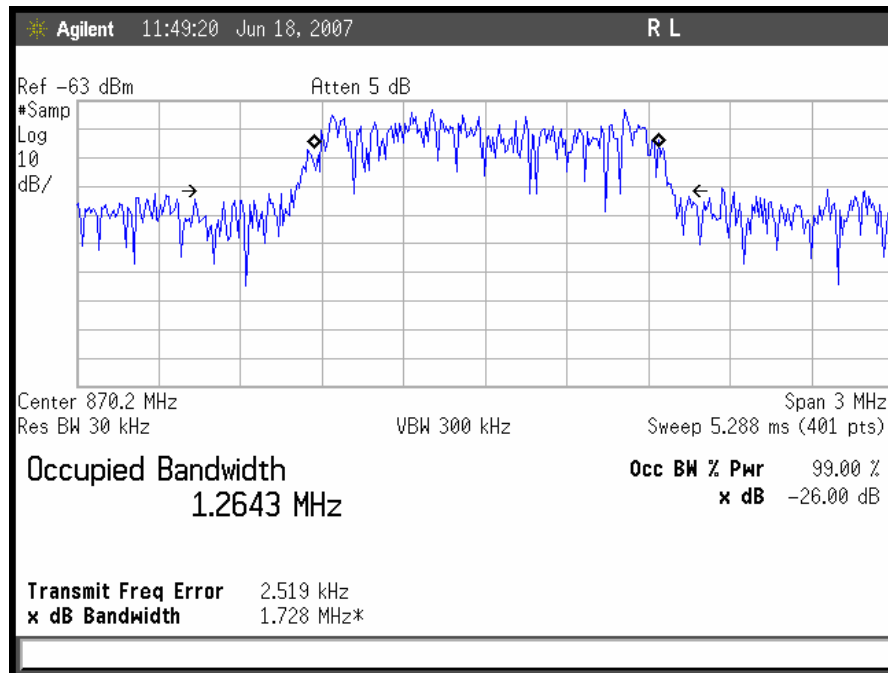
Plot 4. CDMA Downlink Low Channel Input
