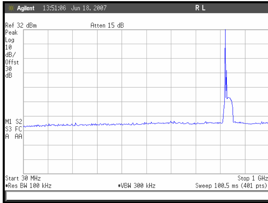
Plot 80. TDMA Uplink Conducted Emissions 30 MHz – 1GHz, Low Channel
