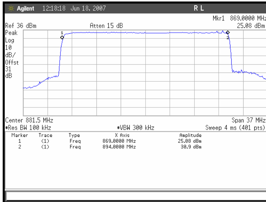
Plot 88. Out of Band Rejection - Downlink
