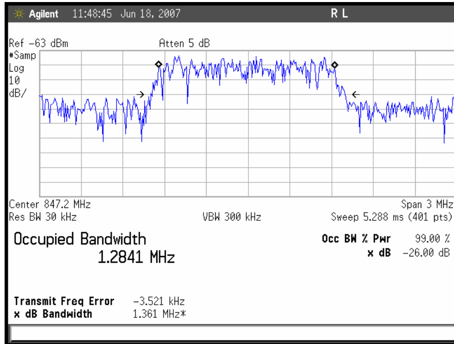
Plot 14. CDMA Uplink High Channel Input
