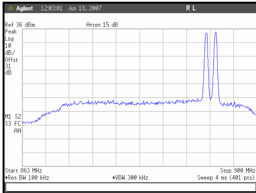
Plot 63. GSM Intermodulation High End, Downlink
