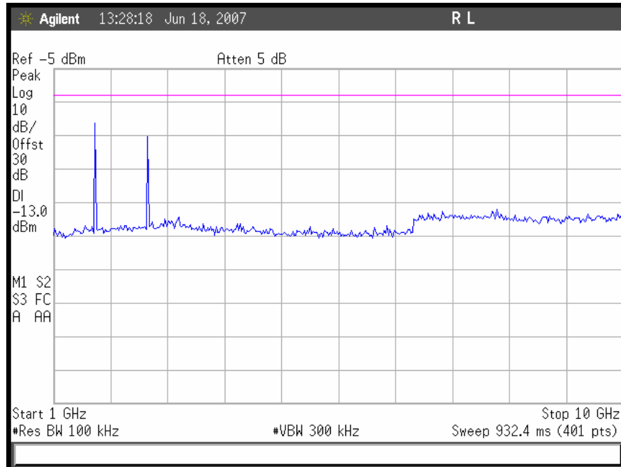
Plot 49. CDMA Uplink Conducted Emissions 1 GHz – 10GHz, Low Channel
