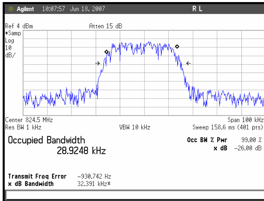
Plot 35. TDMA Uplink Low Channel Output
