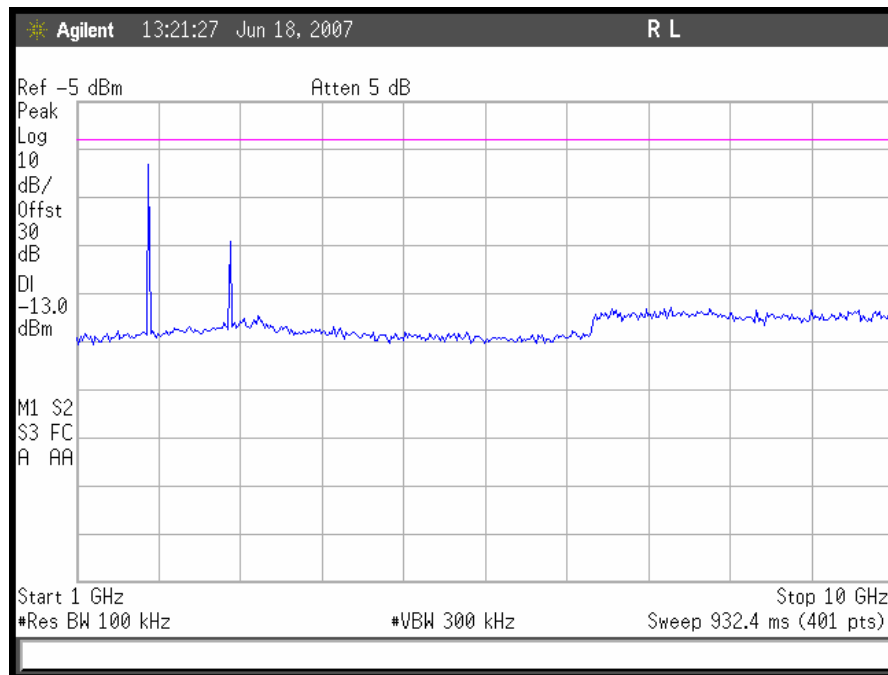
Plot 77. TDMA Downlink Conducted Emissions 1 GHz – 10GHz, High Channel
