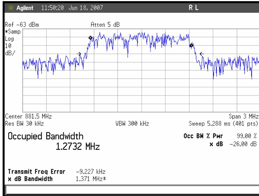
Plot 6. CDMA Downlink Mid Channel Input
