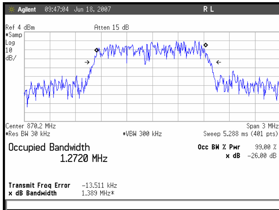
Plot 5. CDMA Downlink Low Channel Output
