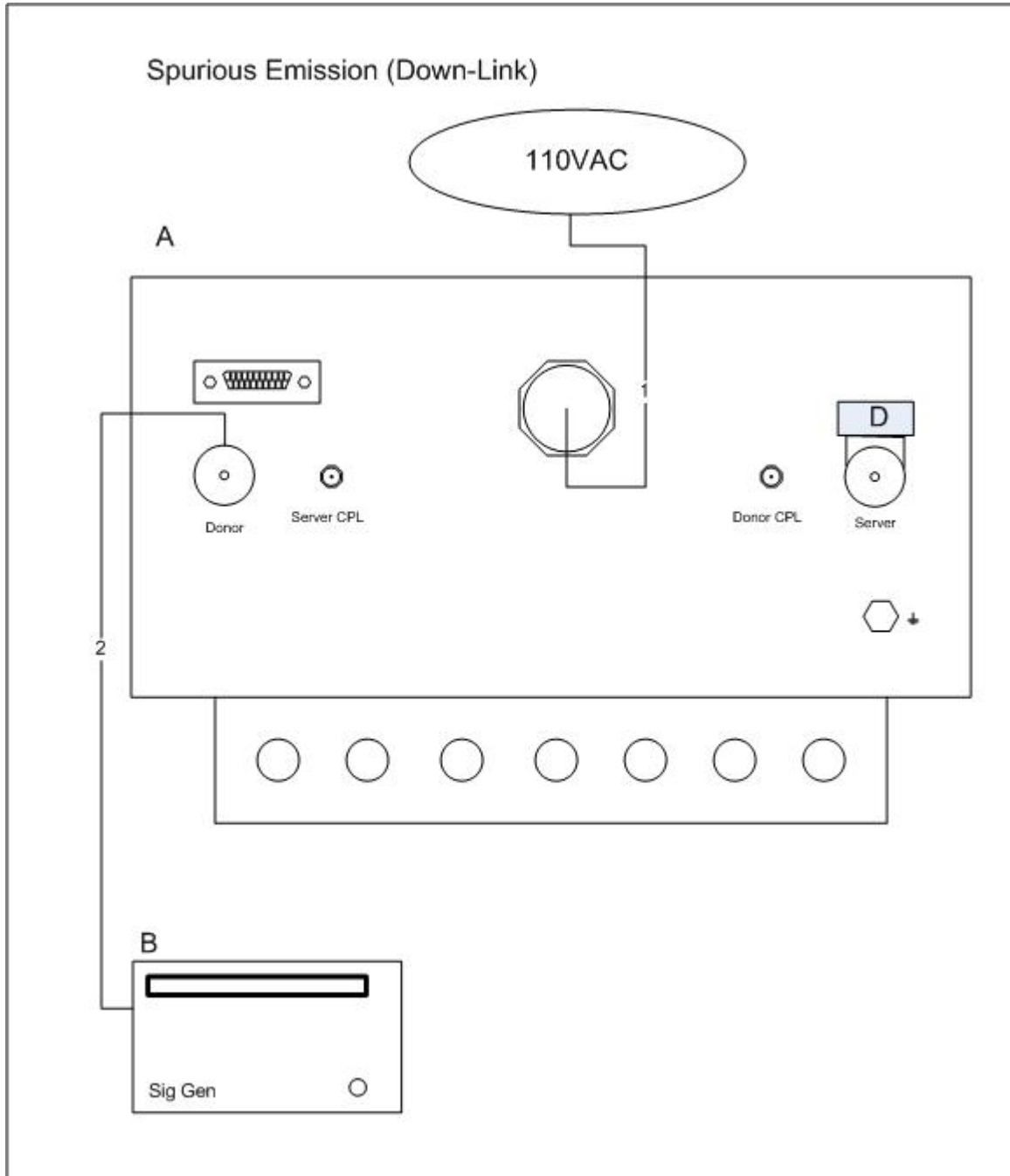
Figure 4. Block Diagram of Test Configuration (Spurious Emission-Downlink)
