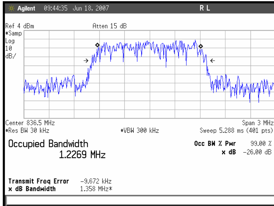
Plot 13. CDMA Uplink Mid Channel Output
