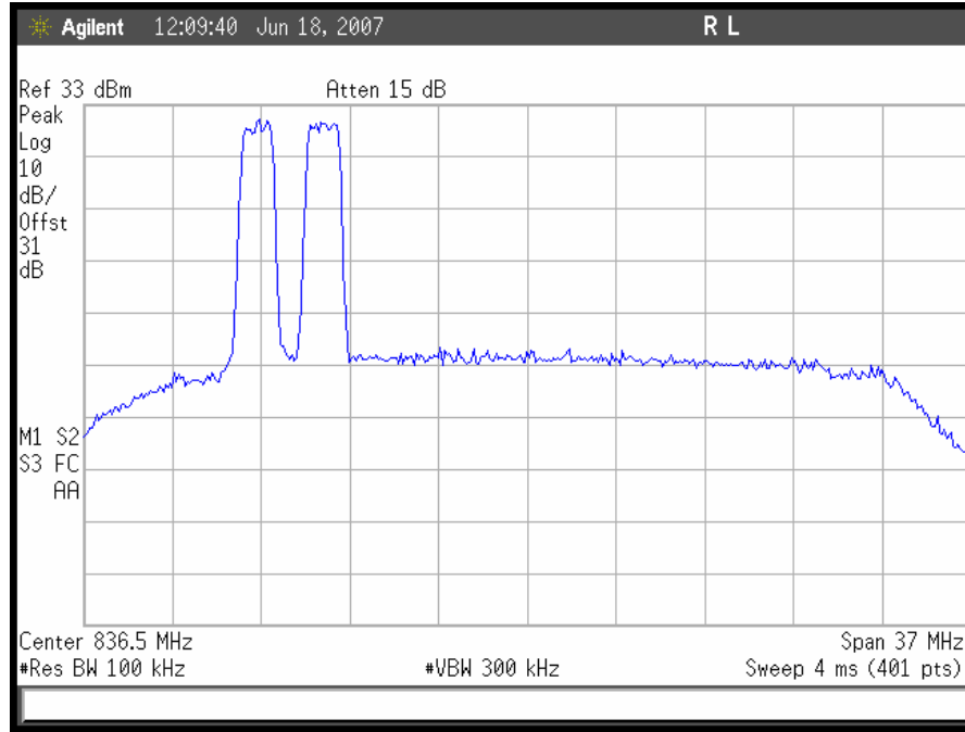
Plot 54. CDMA Intermodulation Low End, Uplink
