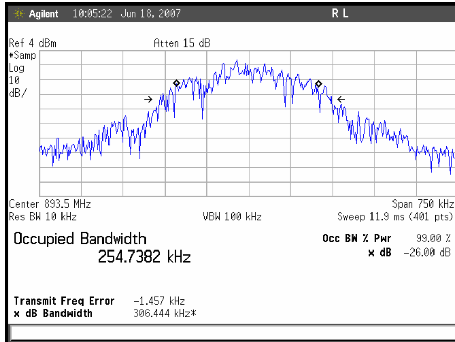
Plot 21. GSM Downlink High Channel Output
