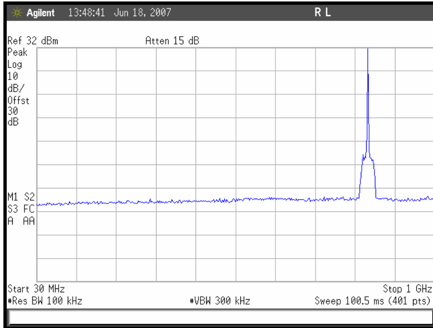
Plot 66. GSM Uplink Conducted Emissions 30 MHz – 1GHz, Mid Channel
