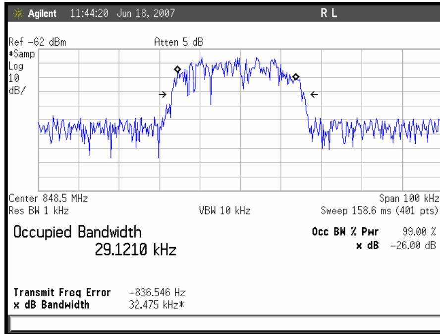
Plot 38. TDMA Uplink High Channel Input
