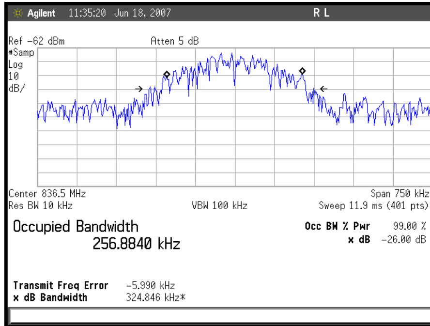
Plot 24. GSM Uplink Mid Channel Input
