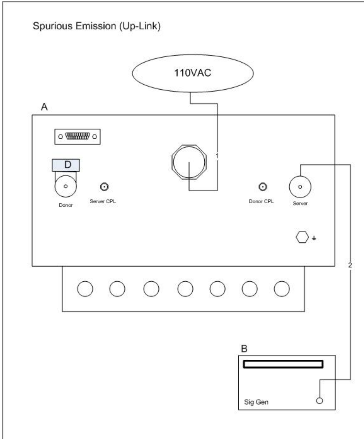
Figure 5. Block Diagram of Test Configuration (Spurious Emission-Uplink)
