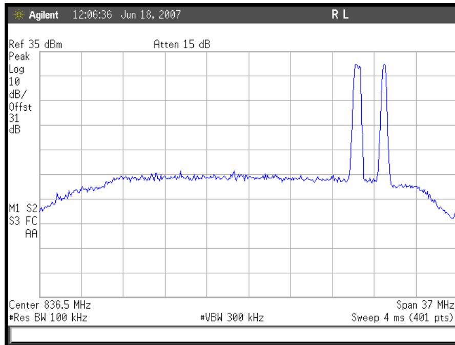
Plot 71. GSM Intermodulation High End, Uplink
