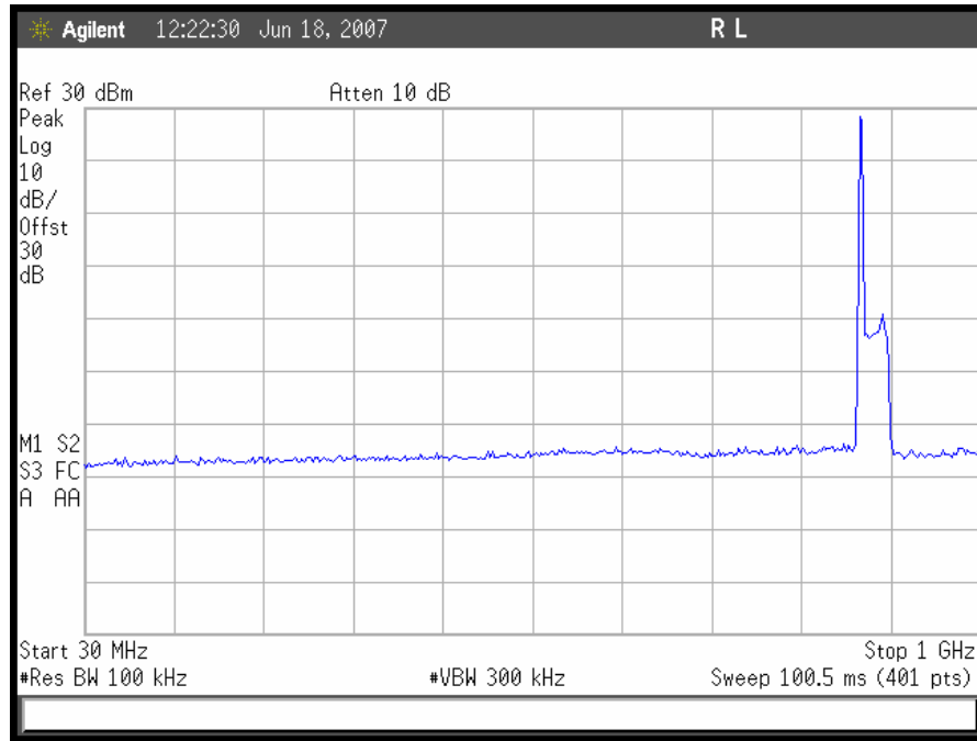
Plot 48. CDMA Uplink Conducted Emissions 30 MHz – 1GHz, Low Channel
