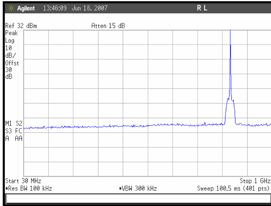
Plot 42. CDMA Downlink Conducted Emissions 30 MHz – 1GHz, Mid Channel
