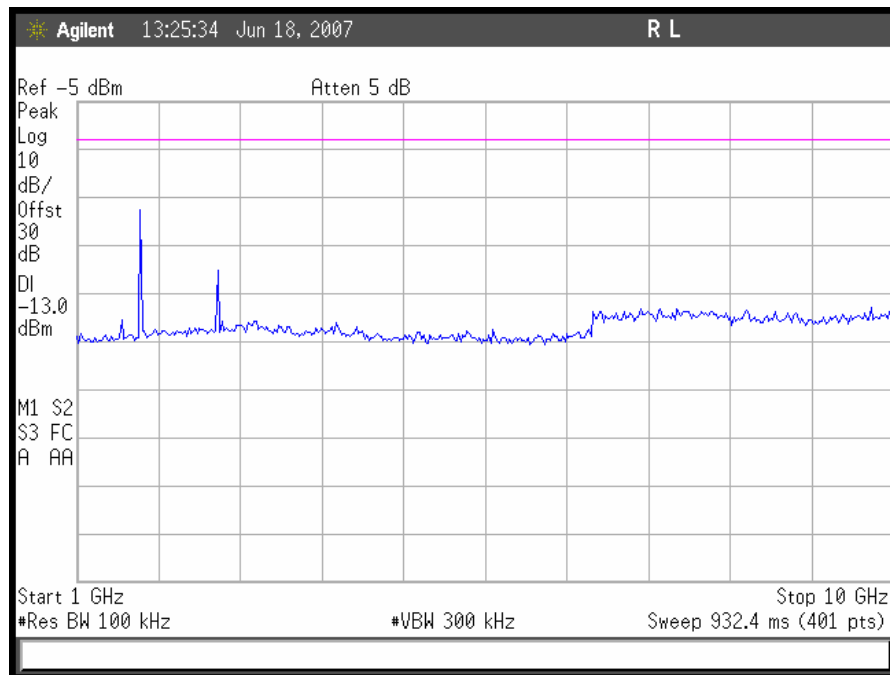
Plot 69. GSM Uplink Conducted Emissions 1 GHz - 10GHz, High Channel
