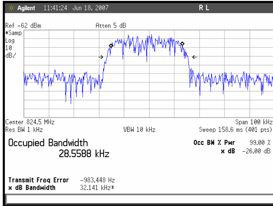
Plot 34. TDMA Uplink Low Channel Input
