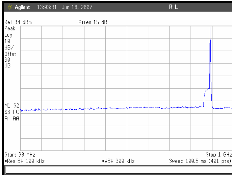
Plot 60. GSM Downlink Conducted Emissions 30 MHz – 1GHz, High Channel
