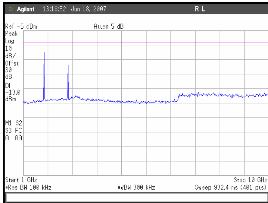
Plot 43. CDMA Downlink Conducted Emissions 1 GHz – 10GHz, Mid Channel
