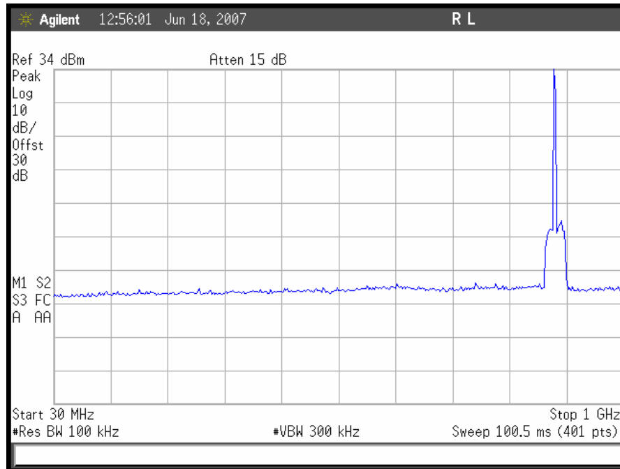
Plot 74. TDMA Downlink Conducted Emissions 30 MHz – 1GHz, Mid Channel
