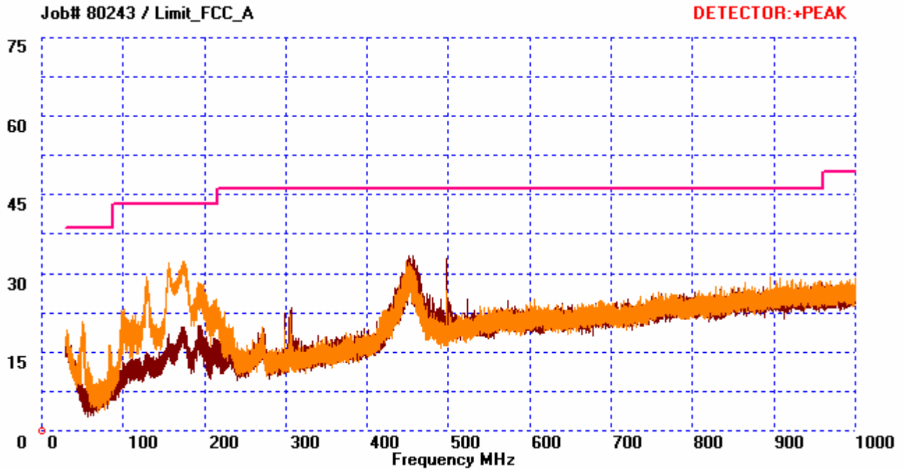
Plot 3. Radiated Emissions Test Results Plot
