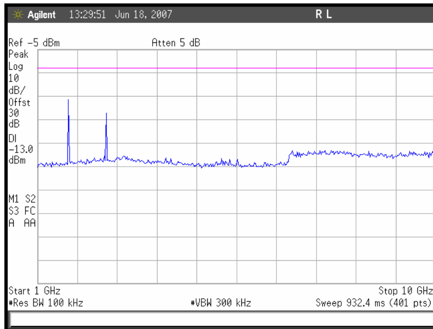
Plot 53. CDMA Uplink Conducted Emissions 1 GHz – 10GHz, High Channel
