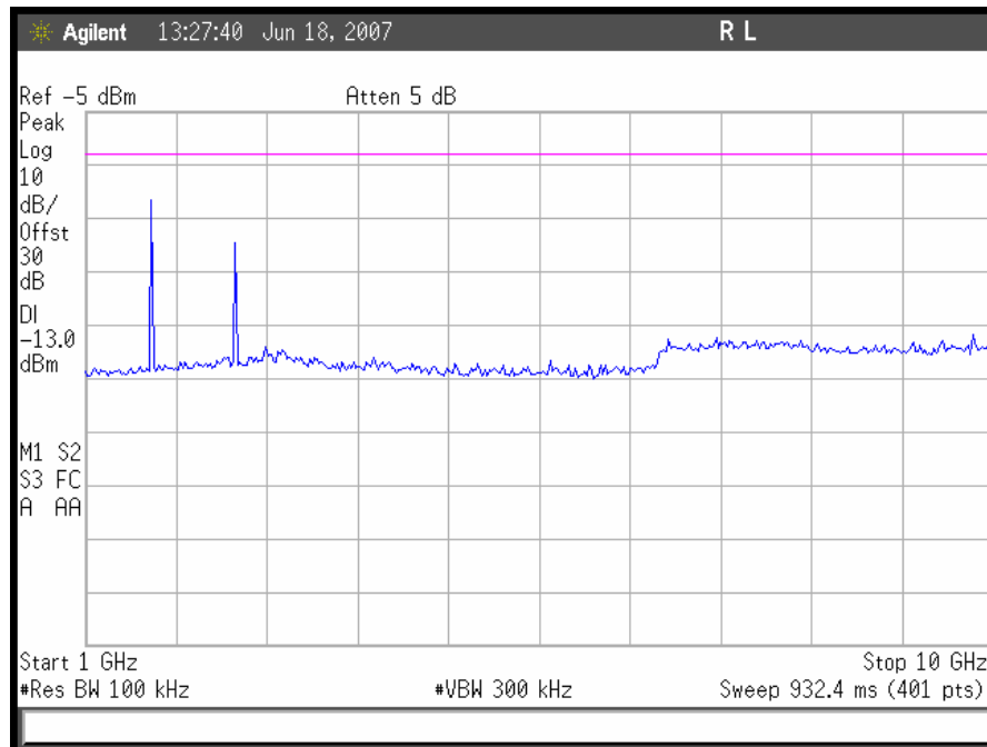
Plot 81. TDMA Uplink Conducted Emissions 1 GHz – 10GHz, Low Channel
