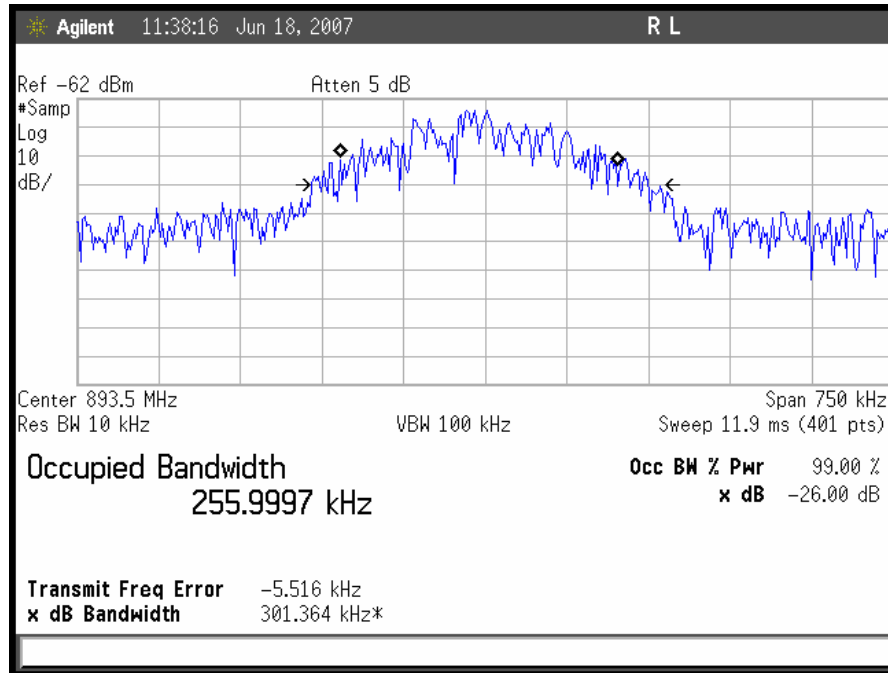
Plot 20. GSM Downlink High Channel Input
