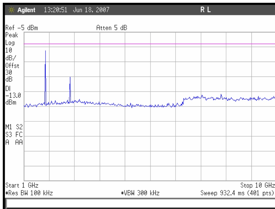
Plot 75. TDMA Downlink Conducted Emissions 1 GHz – 10GHz, Mid Channel
