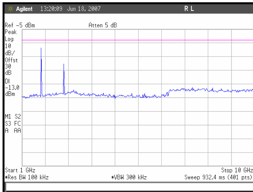
Plot 73. TDMA Downlink Conducted Emissions 1 GHz – 10GHz, Low Channel
