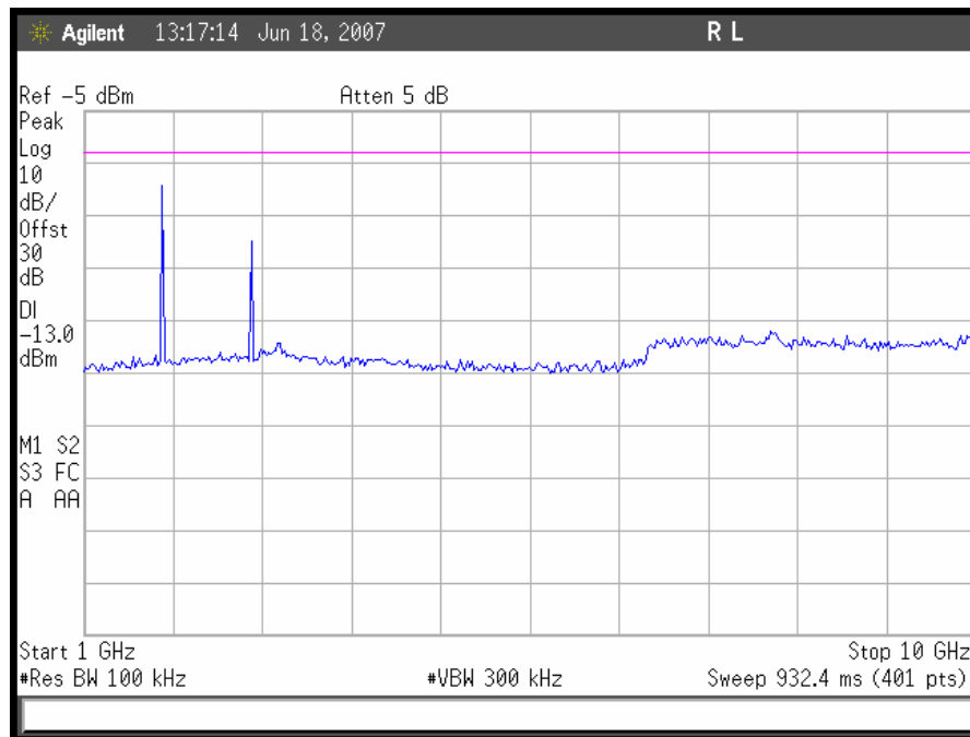
Plot 45. CDMA Downlink Conducted Emissions 1 GHz – 10GHz, High Channel
