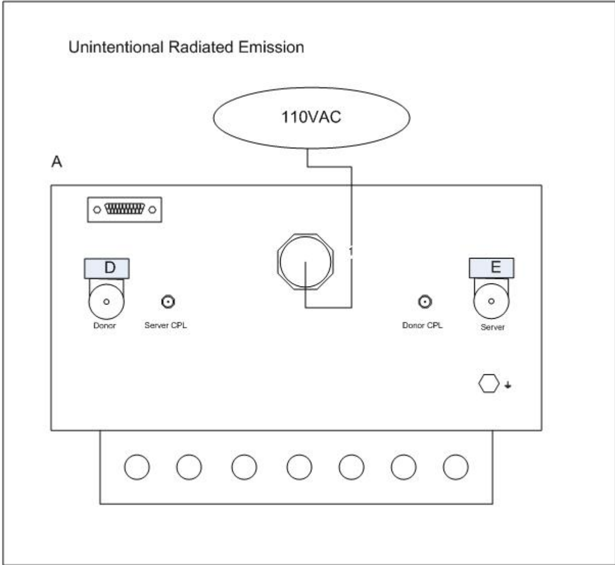
Figure 1. Block Diagram of Test Configuration (Radiated Emissions)
