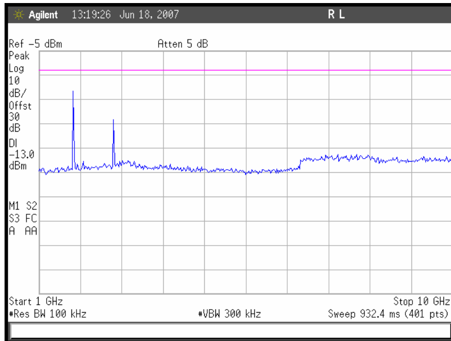
Plot 41. CDMA Downlink Conducted Emissions 1 GHz – 10GHz, Low Channel
