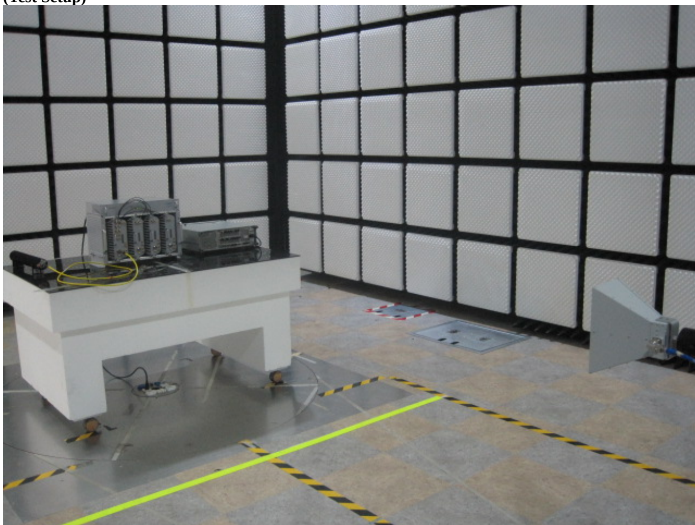
(Test Setup)
