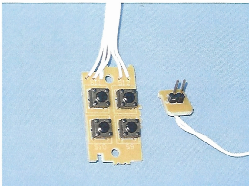
Figure 9 General Appearance of the PCB
