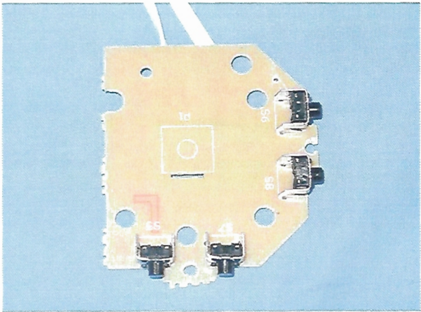
Figure 17 General Appearance of the PCB
