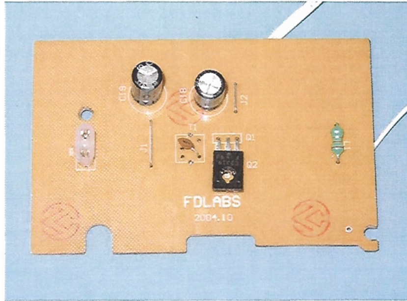
Figure 7 General Appearance of the PCB
