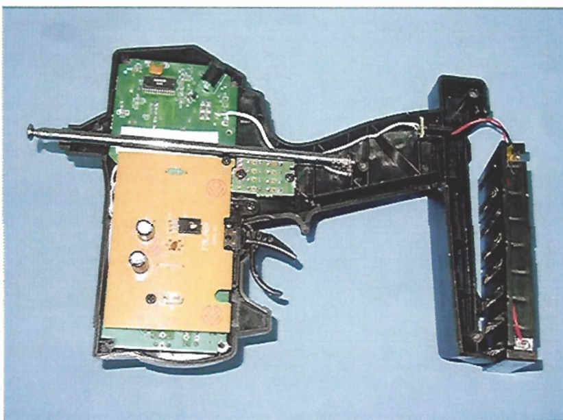
Figure 4 Inside View of the EUT
