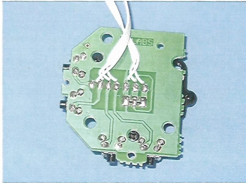
Figure 15 General Appearance of the PCB
