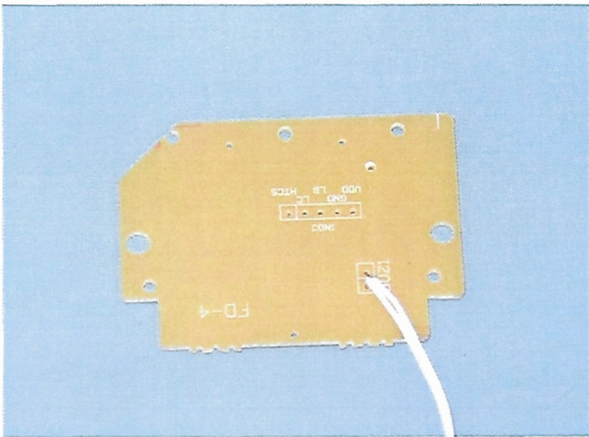
Figure 12 General Appearance of the PCB
