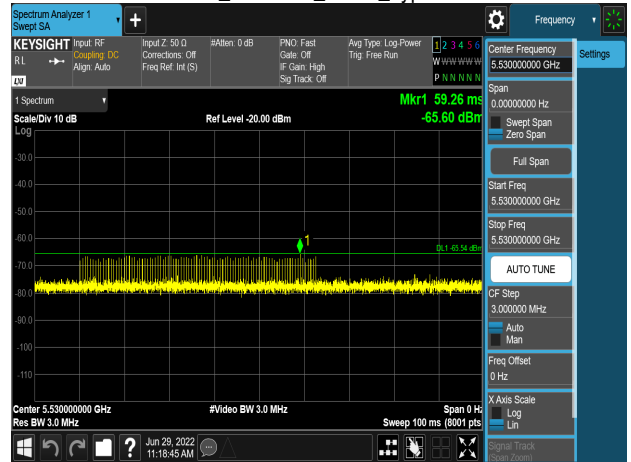
HE80_5530MHz_Radar_Type 1-B
