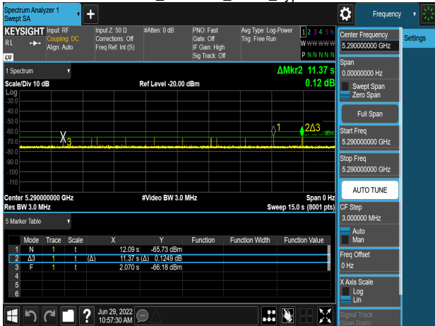
HE80_5290MHz_Radar_Type 6
