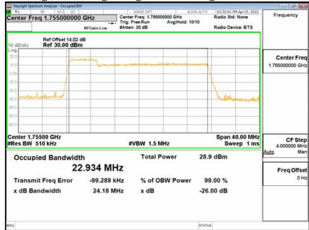
Band66_5MHz+20MHz_64QAM_RB25-0+RB100-0_CH132330+CH132447
