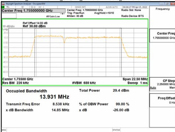
Band66B_5MHz+10MHz_64QAM_RB25-0+RB50-0_CH132375+CH132447
