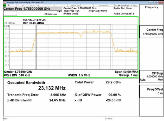
Band66_15MHz+10MHz_64QAM_RB75-0+RB50-0_CH132373+CH132493
