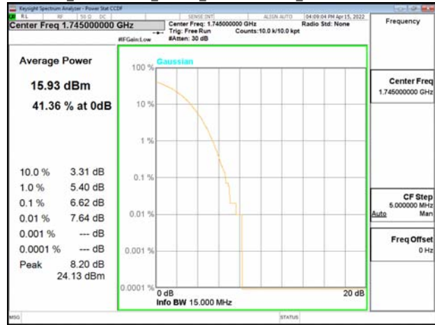
Band66B_5MHz+15MHz_64QAM_RB25-0+RB75-0_CH132353+CH132446
