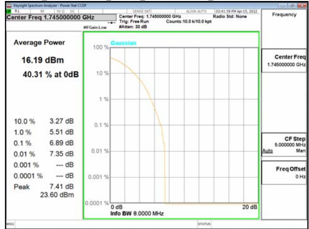
Band66_15MHz+10MHz_64QAM_RB75-0+RB50-0_CH132373+CH132493
