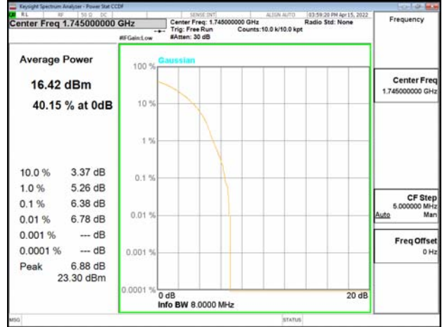
Band66_20MHz+15MHz_64QAM_RB100-0+RB75-0_CH132348+CH132519
