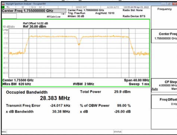
Band66_15MHz+15MHz_16QAM_RB75-0+RB75-0_CH132347+CH132497
