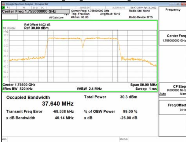
Band66_20MHz+20MHz_16QAM_RB100-0+RB100-0_CH132323+CH132521
