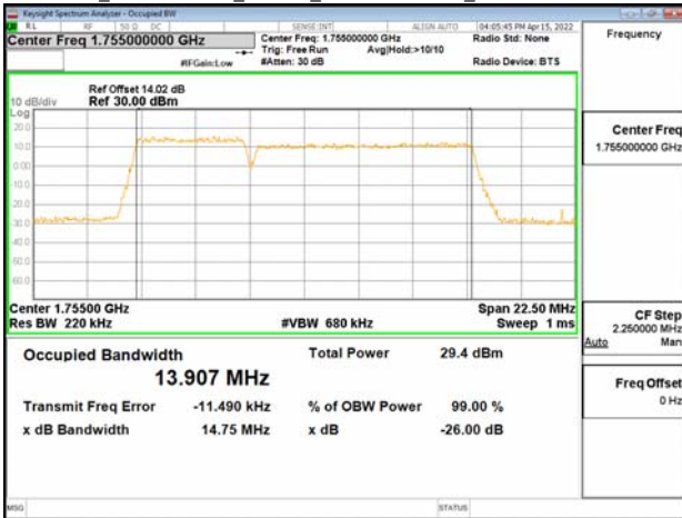
Band66B_5MHz+10MHz_64QAM_RB25-0+RB50-0_CH132375+CH132447
