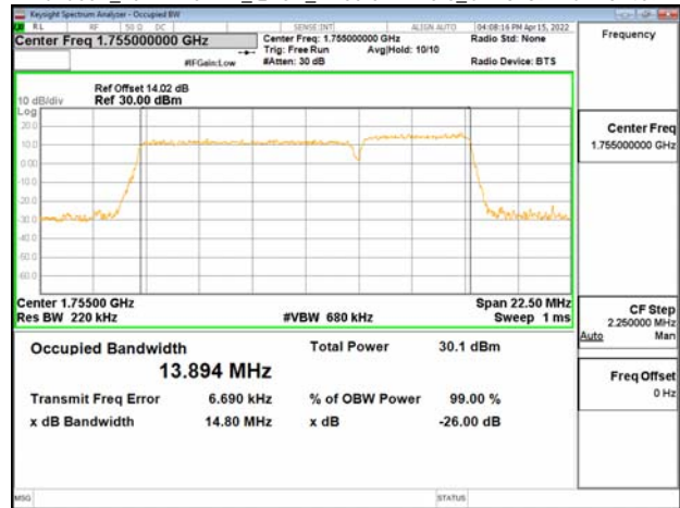
Band66B_10MHz+5MHz_16QAM_RB50-0+RB25-0_CH132397+CH132469
