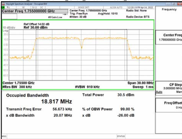
Band66B_10MHz+10MHz_16QAM_RB50-0+RB50-0_CH132373+CH132472
