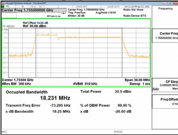
Band66B_5MHz+15MHz_16QAM_RB25-0+RB75-0_CH132353+CH132446
