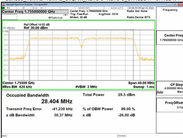
Band66_15MHz+15MHz_64QAM_RB75-0+RB75-0_CH132347+CH132497
