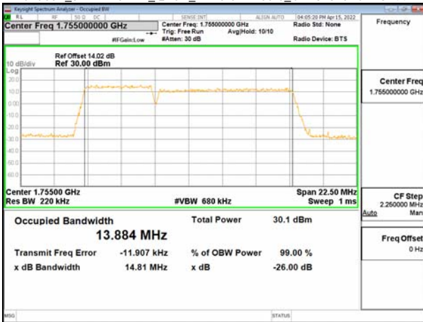
Band66B_5MHz+10MHz_16QAM_RB25-0+RB50-0_CH132375+CH132447
