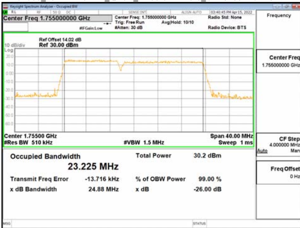
Band66_10MHz+15MHz_16QAM_RB50-0+RB75-0_CH132351+CH132471
