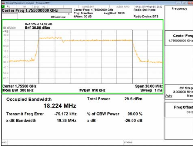
Band66B_5MHz+15MHz_64QAM_RB25-0+RB75-0_CH132353+CH132446
