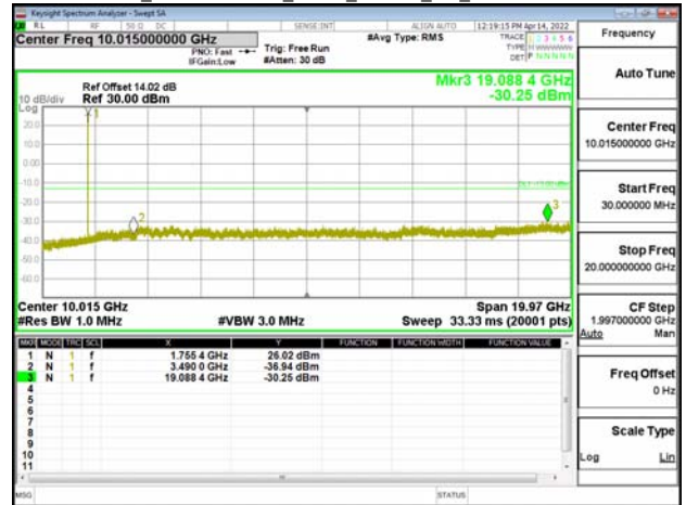
Band66B_10MHz+10MHz_OPSK_RB1-49_1-0_CH132523-132622
