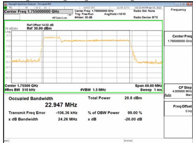
Band66_5MHz+20MHz_64QAM_RB25-0+RB100-0_CH132330+CH132447
