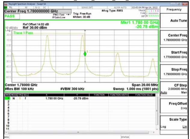
Band66B_5MHz+5MHz_QPSK_RB1-24_1-24_CH132599-132647
