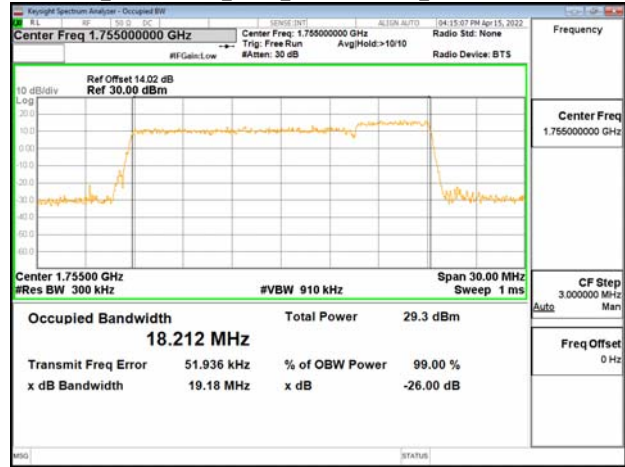
Band66B_15MHz+5MHz_16QAM_RB75-0+RB25-0_CH132398+CH132491
