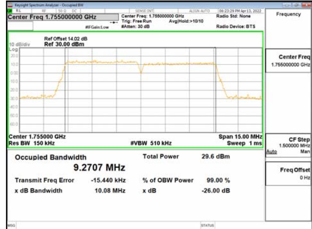
Band66B_5MHz+5MHz_64QAM_RB25-0+RB25-0_CH132398+CH132446
