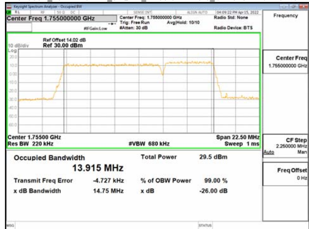
Band66B_10MHz+5MHz_64QAM_RB50-0+RB25-0_CH132397+CH132469
