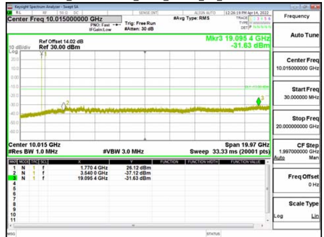
Band66B_10MHz+10MHz_OPSK_RB1-49_1-0_CH132523-132622
