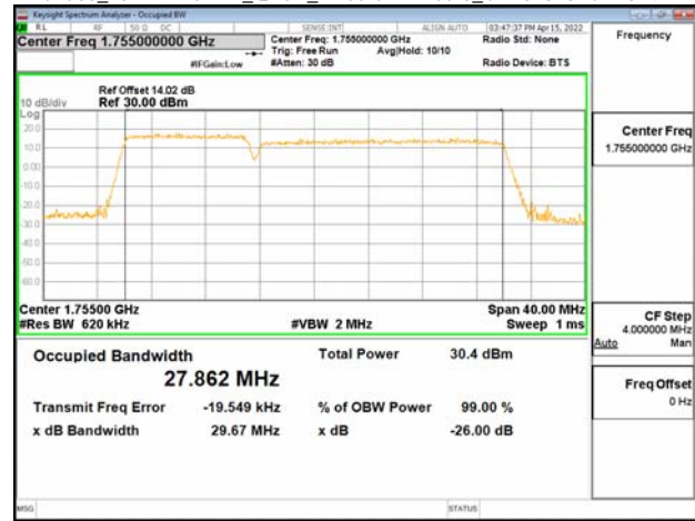
Band66_10MHz+20MHz_16QAM_RB50-0+RB100-0_CH132328+CH132472
