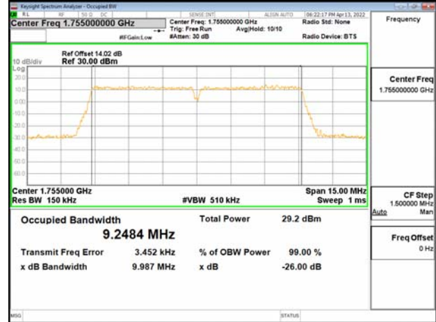
Band66B_5MHz+5MHz_64QAM_RB25-0+RB25-0_CH132398+CH132446
