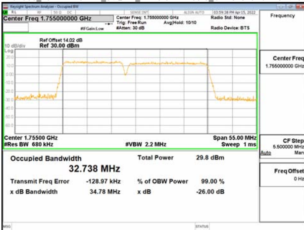
Band66_15MHz+20MHz_64QAM_RB75-0+RB100-0_CH132325+CH132496
