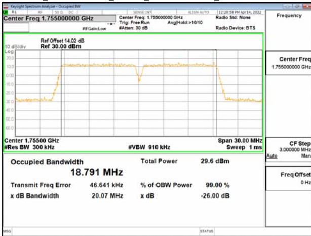
Band66B_10MHz+10MHz_64QAM_RB50-0+RB50-0_CH132373+CH132472
