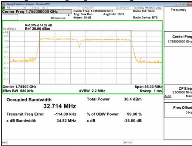
Band66_15MHz+20MHz_16QAM_RB75-0+RB100-0_CH132325+CH132496
