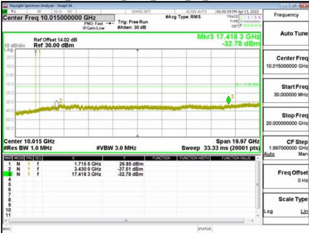
Band66B_5MHz+5MHz_OPSK_RB1-24_1-0_CH132398-132446
