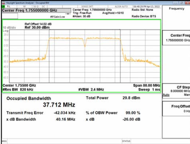
Band66_20MHz+20MHz_64QAM_RB100-0+RB100-0_CH132323+CH132521
