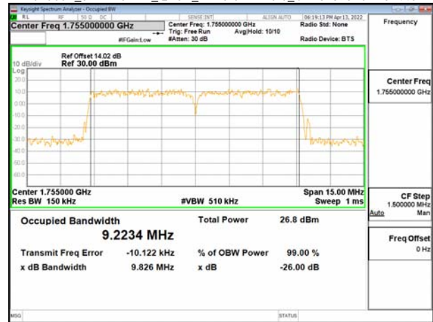
Band66B_5MHz+5MHz_16QAM_RB25-0+RB25-0_CH132398+CH132446
