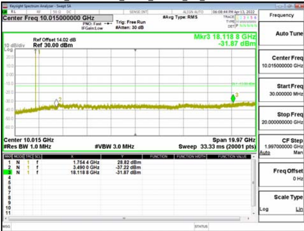
Band66B_5MHz+5MHz_OPSK_RB1-24_1-0_CH132599-132647
