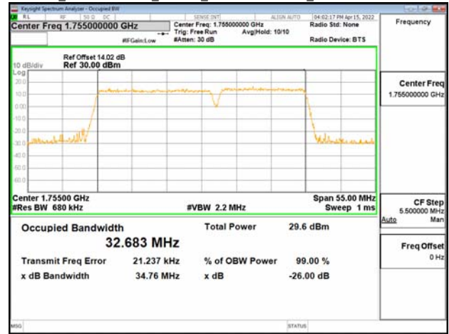
Band66_20MHz+15MHz_64QAM_RB100-0+RB75-0_CH132348+CH132519
