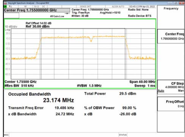
Band66_15MHz+10MHz_64QAM_RB75-0+RB50-0_CH132373+CH132493
