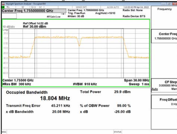
Band66B_10MHz+10MHz_64QAM_RB50-0+RB50-0_CH132373+CH132472
