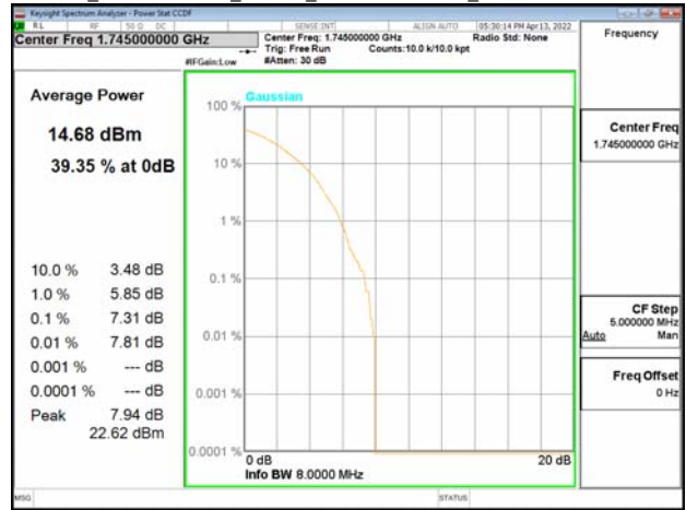
Band66_15MHz+20MHz_64QAM_RB75-0+RB100-0_CH132325+CH132496
