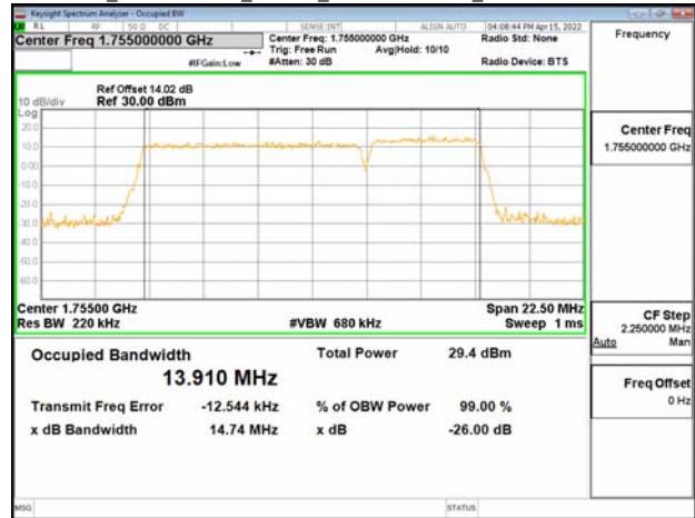
Band66B_10MHz+5MHz_64QAM_RB50-0+RB25-0_CH132397+CH132469
