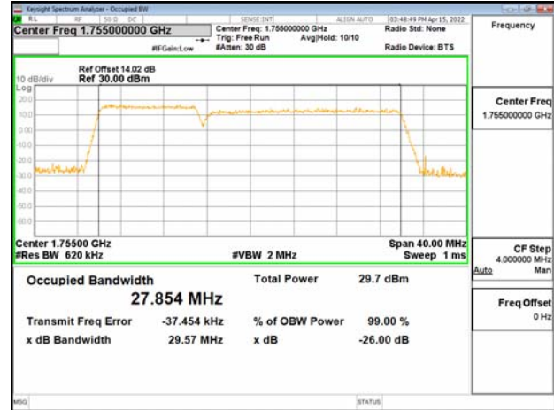
Band66_10MHz+20MHz_64QAM_RB50-0+RB100-0_CH132328+CH132472
