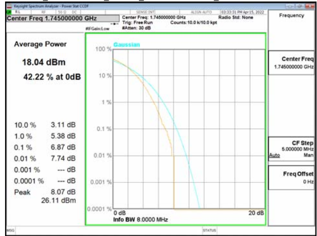
Band66_10MHz+15MHz_64QAM_RB50-0+RB75-0_CH132351+CH132471
