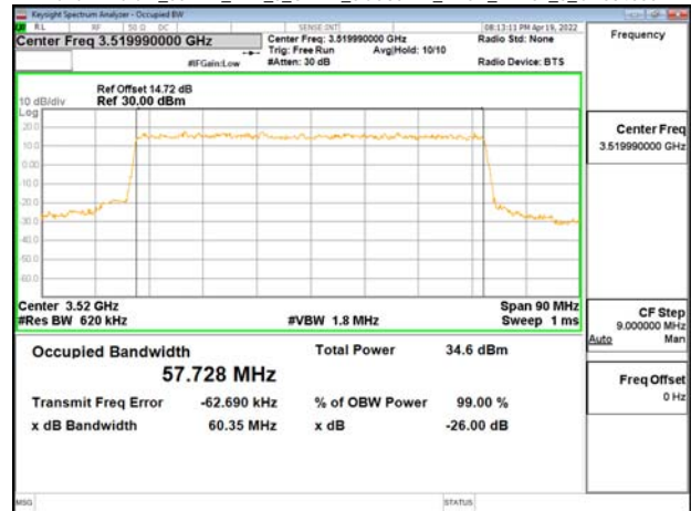
Band77-Part27_60MHz_DFT_s_OFDM_SCS30kHz_BPSK_RB162_0_CH634666
