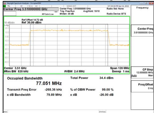
Band77-Part27_80MHz_DFT_s_OFDM_SCS30kHz_64QAM_RB216_0_CH634000
