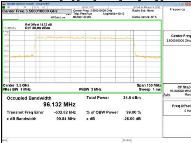
Band77-Part27_100MHz_DFT_s_OFDM_SCS30kHz_256QAM_RB270_0_CH633334
