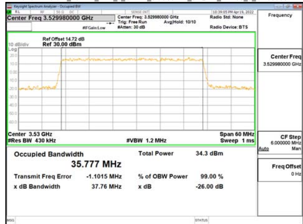
Band77-Part27_40MHz_DFT_s_OFDM_SCS30kHz_64QAM_RB100_0_CH635332
