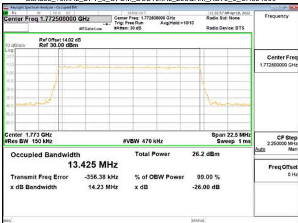
Band66_15MHz_DFT_s_OFDM_SCS15kHz_256QAM_RB75_0_CH354500
