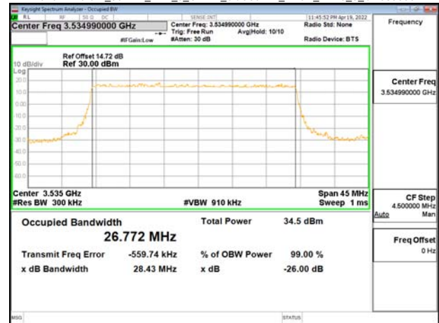
Band77-Part27_30MHz_DFT_s_OFDM_SCS30kHz_BPSK_RB75_0_CH635666
