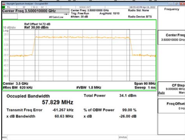
Band77-Part27_60MHz_DFT_s_OFDM_SCS30kHz_64QAM_RB162_0_CH634666
