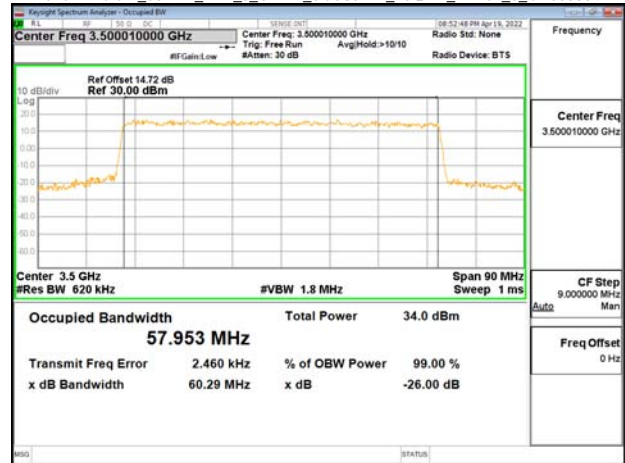
Band77-Part27_60MHz_DFT_s_OFDM_SCS30kHz_16QAM_RB162_0_CH634666
