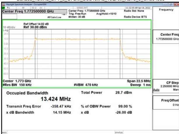
Band66_15MHz_DFT_s_OFDM_SCS15kHz_16QAM_RB75_0_CH354500
