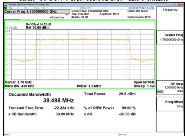
Band66_40MHz_DFT_s_OFDM_SCS15kHz_BPSK_RB216_0_CH352000
