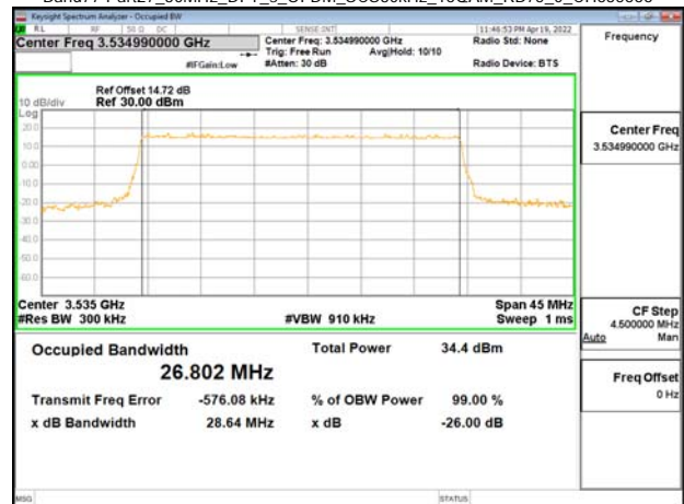
Band77-Part27_30MHz_DFT_s_OFDM_SCS30kHz_16QAM_RB75_0_CH635666
