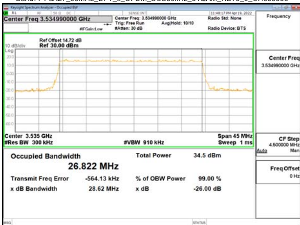
Band77-Part27_30MHz_DFT_s_OFDM_SCS30kHz_64QAM_RB75_0_CH635666
