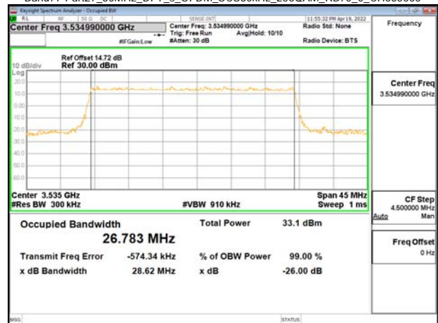
Band77-Part27_30MHz_DFT_s_OFDM_SCS30kHz_256QAM_RB75_0_CH635666
