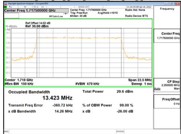
Band66_15MHz_DFT_s_OFDM_SCS15kHz_QPSK_RB75_0_CH349000
