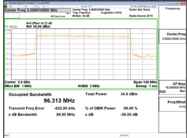
Band77-Part27_100MHz_DFT_s_OFDM_SCS30kHz_QPSK_RB270_0_CH633334
