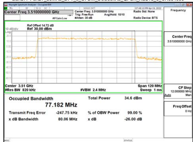
Band77-Part27_80MHz_DFT_s_OFDM_SCS30kHz_QPSK_RB216_0_CH634000
