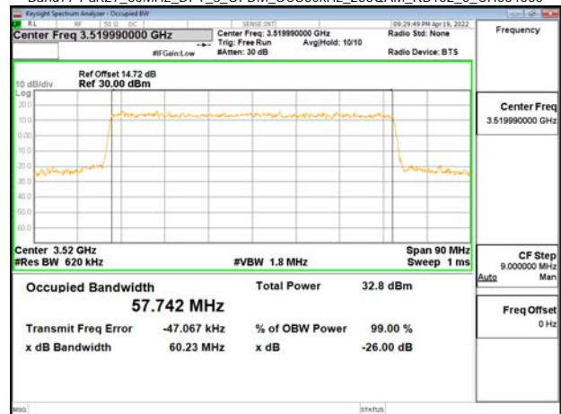
Band77-Part27_60MHz_DFT_s_OFDM_SCS30kHz_256QAM_RB162_0_CH634666
