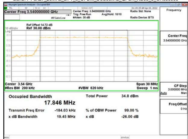
Band77-Part27_20MHz_DFT_s_OFDM_SCS30kHz_QPSK_RB50_0_CH636000
