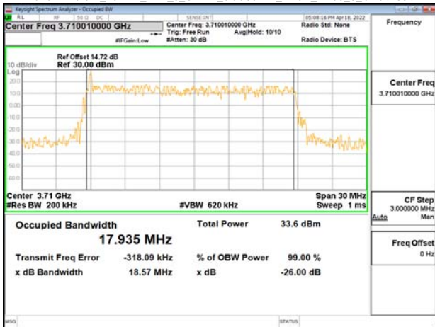
Band77-Part27_20MHz_DFT_s_OFDM_SCS30kHz_BPSK_RB50_0_CH647334
