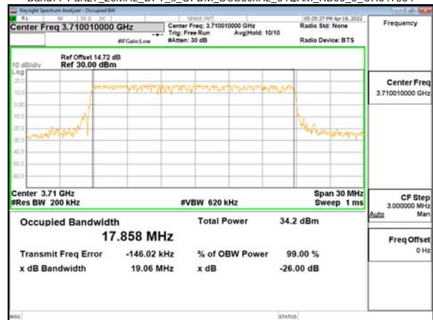
Band77-Part27_20MHz_DFT_s_OFDM_SCS30kHz_64QAM_RB50_0_CH647334
