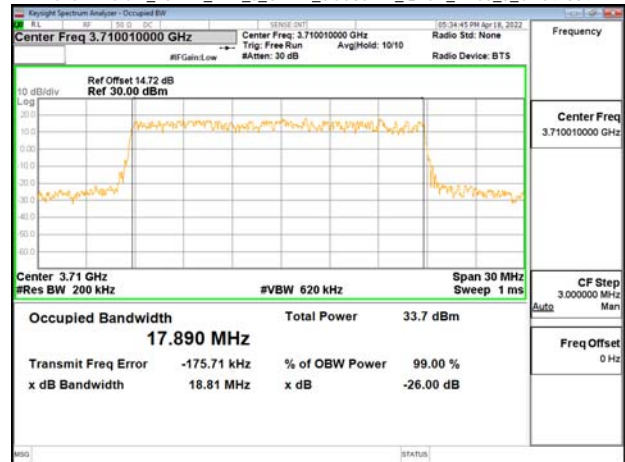
Band77-Part27_20MHz_DFT_s_OFDM_SCS30kHz_OPSK_RB50_0_CH647334
