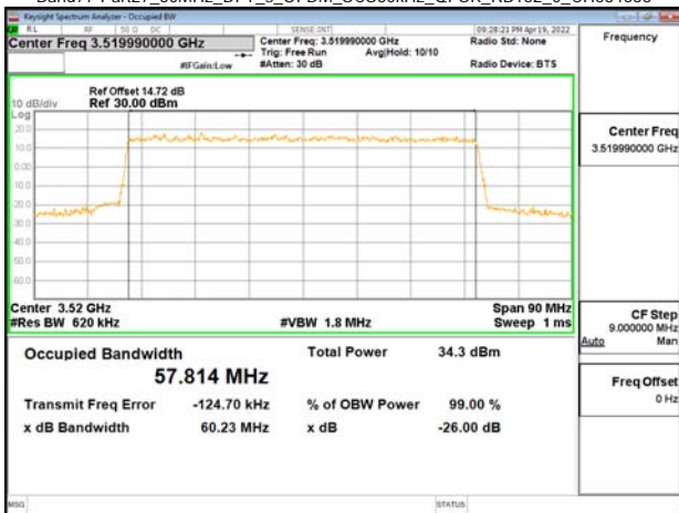
Band77-Part27_60MHz_DFT_s_OFDM_SCS30kHz_QPSK_RB162_0_CH634666
