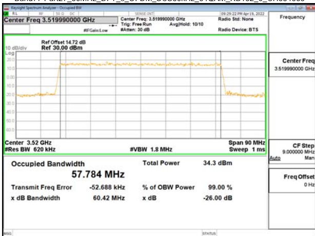
Band77-Part27_60MHz_DFT_s_OFDM_SCS30kHz_64QAM_RB162_0_CH634666
