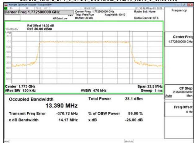
Band66_15MHz_DFT_s_OFDM_SCS15kHz_64QAM_RB75_0_CH354500
