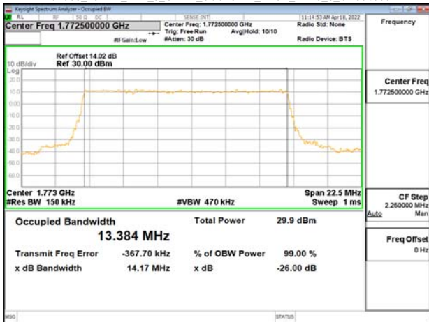
Band66_15MHz_DFT_s_OFDM_SCS15kHz_BPSK_RB75_0_CH354500
