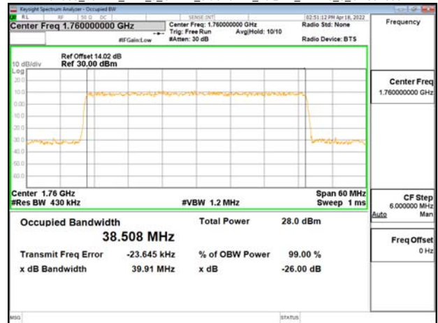
Band66_40MHz_DFT_s_OFDM_SCS15kHz_16QAM_RB216_0_CH352000
