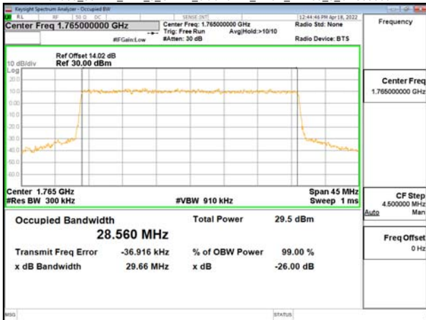
Band66_30MHz_DFT_s_OFDM_SCS15kHz_BPSK_RB160_0_CH353000
