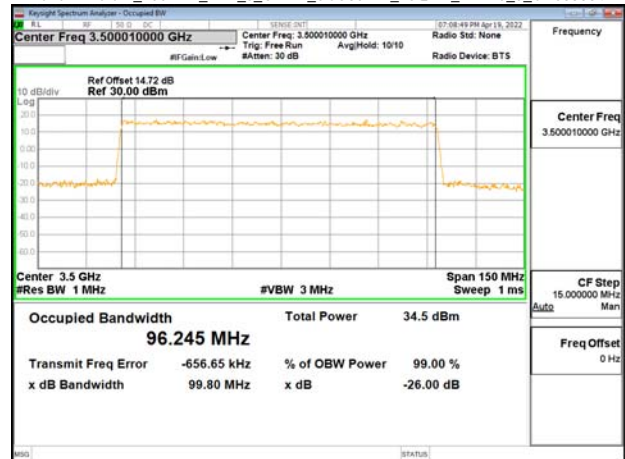
Band77-Part27_100MHz_DFT_s_OFDM_SCS30kHz_16QAM_RB270_0_CH633334
