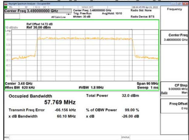
Band77-Part27_60MHz_DFT_s_OFDM_SCS30kHz_256QAM_RB162_0_CH6333334
