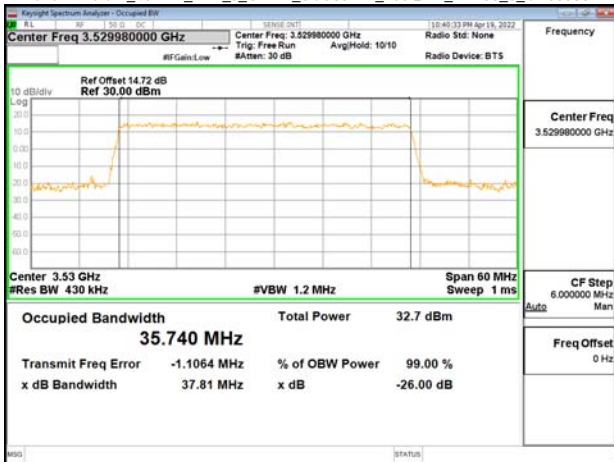
Band77-Part27_40MHz_DFT_s_OFDM_SCS30kHz_256QAM_RB100_0_CH635332
