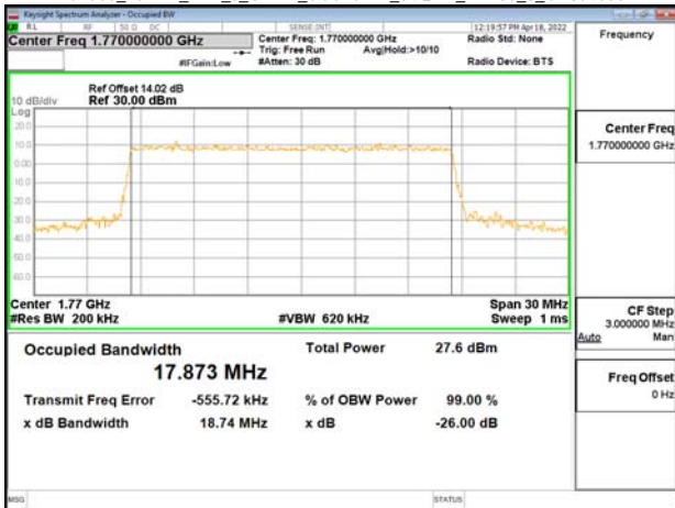
Band66_20MHz_DFT_s_OFDM_SCS15kHz_64QAM_RB100_0_CH354000
