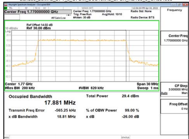
Band66_20MHz_DFT_s_OFDM_SCS15kHz_BPSK_RB100_0_CH354000
