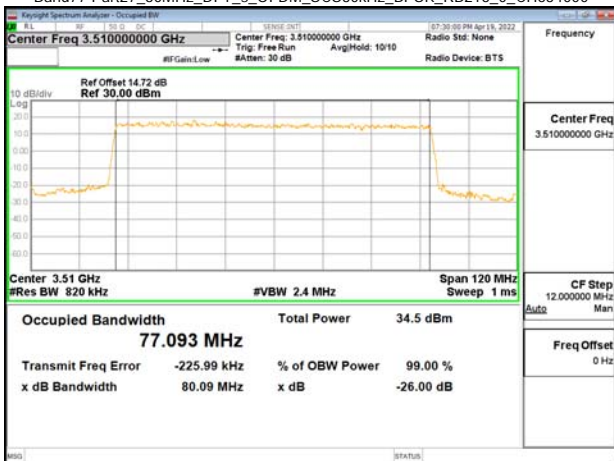
Band77-Part27_80MHz_DFT_s_OFDM_SCS30kHz_BPSK_RB216_0_CH634000
