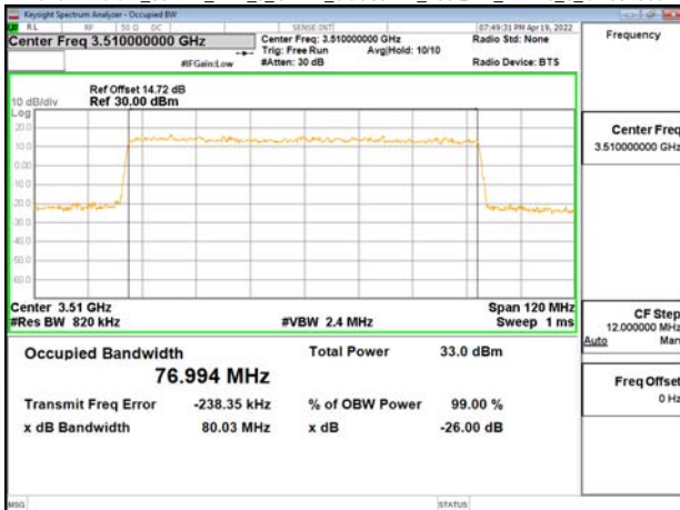
Band77-Part27_80MHz_DFT_s_OFDM_SCS30kHz_256QAM_RB216_0_CH634000
