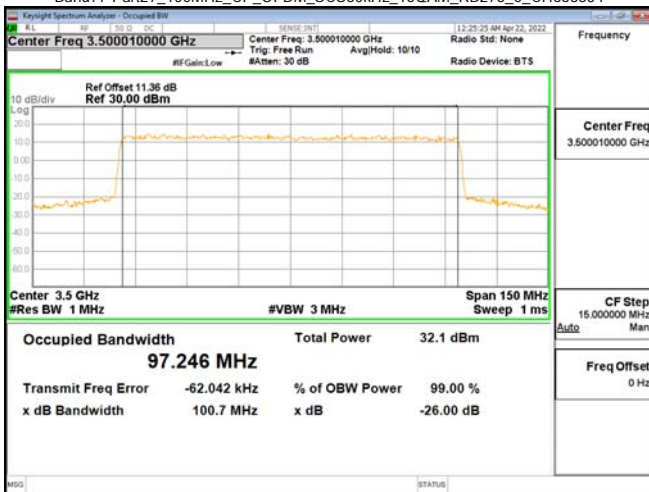
Band77-Part27_100MHz_CP_OFDM_SCS30kHz_64QAM_RB273_0_CH633334
