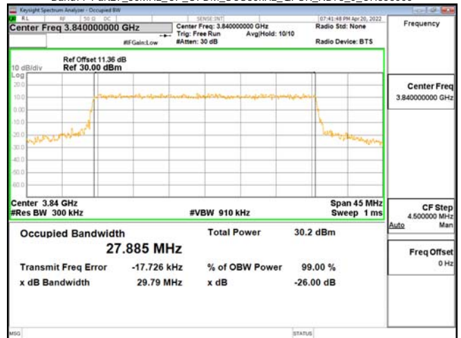
Band77-Part27_30MHz_CP_OFDM_SCS30kHz_QPSK_RB78_0_CH656000
