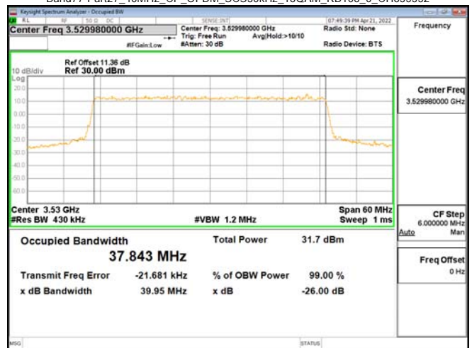
Band77-Part27_40MHz_CP_OFDM_SCS30kHz_16QAM_RB106_0_CH635332
