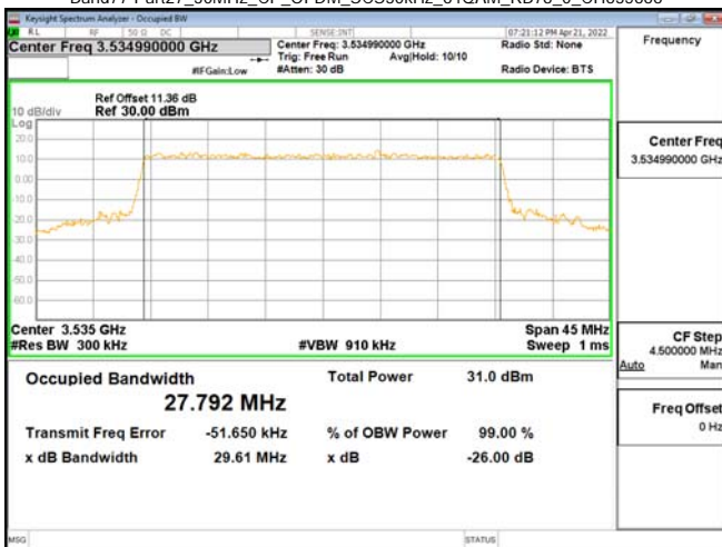
Band77-Part27_30MHz_CP_OFDM_SCS30kHz_64QAM_RB78_0_CH635666
