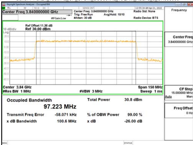
Band77-Part27_100MHz_CP_OFDM_SCS30kHz_16QAM_RB273_0_CH656000
