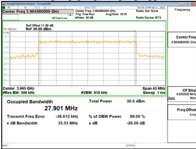
Band77-Part27_30MHz_CP_OFDM_SCS30kHz_16QAM_RB78_0_CH647668
