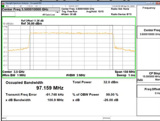
Band77-Part27_100MHz_CP_OFDM_SCS30kHz_16QAM_RB273_0_CH633334
