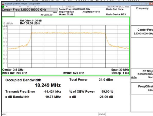
Band77-Part27_20MHz_CP_OFDM_SCS30kHz_QPSK_RB51_0_CH636000
