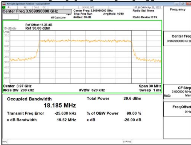
Band77-Part27_20MHz_CP_OFDM_SCS30kHz_256QAM_RB51_0_CH647334
