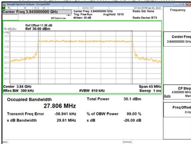
Band77-Part27_30MHz_CP_OFDM_SCS30kHz_16QAM_RB78_0_CH656000
