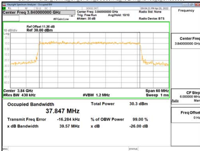
Band77-Part27_40MHz_CP_OFDM_SCS30kHz_16QAM_RB106_0_CH656000
