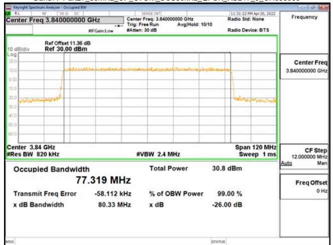
Band77-Part27_80MHz_CP_OFDM_SCS30kHz_QPSK_RB217_0_CH656000
