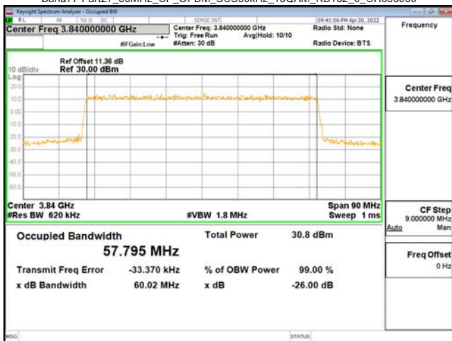
Band77-Part27_60MHz_CP_OFDM_SCS30kHz_16QAM_RB162_0_CH656000
