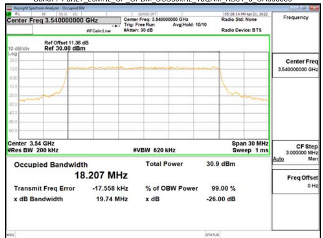
Band77-Part27_20MHz_CP_OFDM_SCS30kHz_16QAM_RB51_0_CH636000
