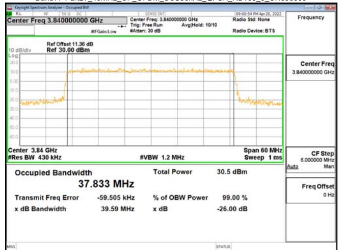
Band77-Part27_40MHz_CP_OFDM_SCS30kHz_QPSK_RB106_0_CH656000
