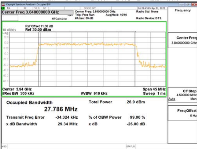
Band77-Part27_30MHz_CP_OFDM_SCS30kHz_256QAM_RB78_0_CH656000
