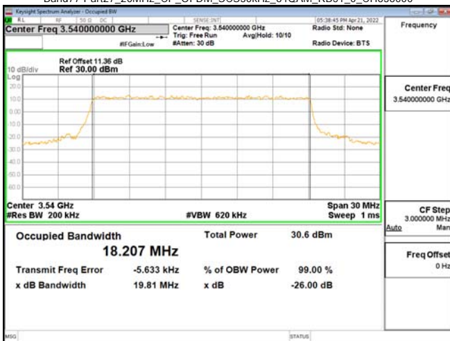
Band77-Part27_20MHz_CP_OFDM_SCS30kHz_64QAM_RB51_0_CH636000
