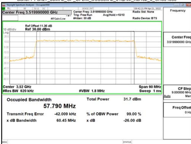
Band77-Part27_60MHz_CP_OFDM_SCS30kHz_64QAM_RB162_0_CH634666
