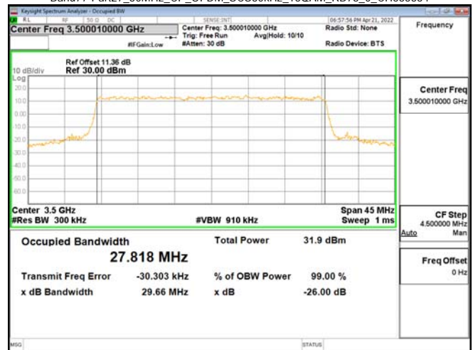
Band77-Part27_30MHz_CP_OFDM_SCS30kHz_16QAM_RB78_0_CH635666
