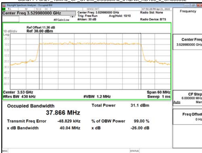
Band77-Part27_40MHz_CP_OFDM_SCS30kHz_64QAM_RB106_0_CH635332
