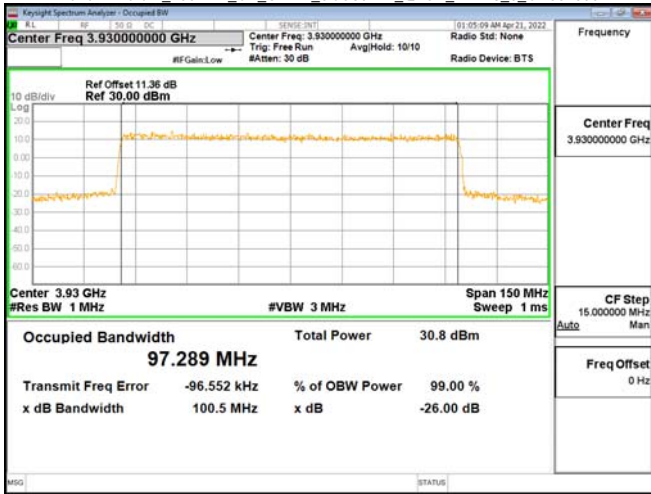
Band77-Part27_100MHz_CP_OFDM_SCS30kHz_16QAM_RB273_0_CH650000
