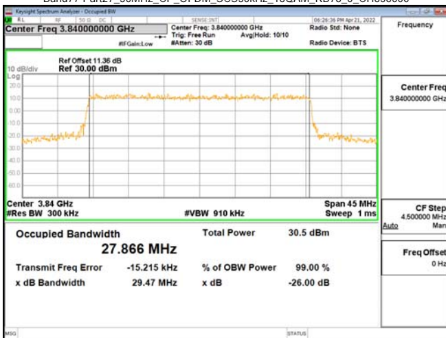
Band77-Part27_30MHz_CP_OFDM_SCS30kHz_16QAM_RB78_0_CH656000
