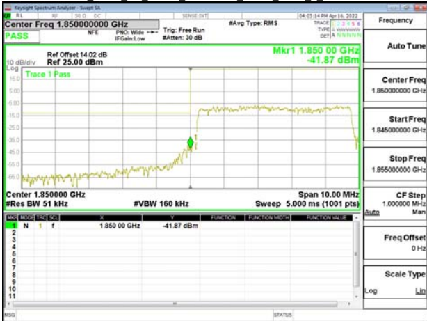
Band2_5MHz_CP_OFDM_SCS15kHz_QPSK_RB25_0_CH381500
