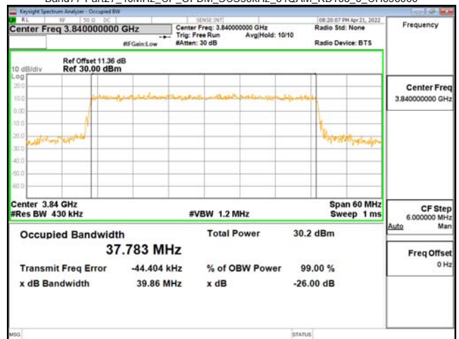
Band77-Part27_40MHz_CP_OFDM_SCS30kHz_64QAM_RB106_0_CH656000
