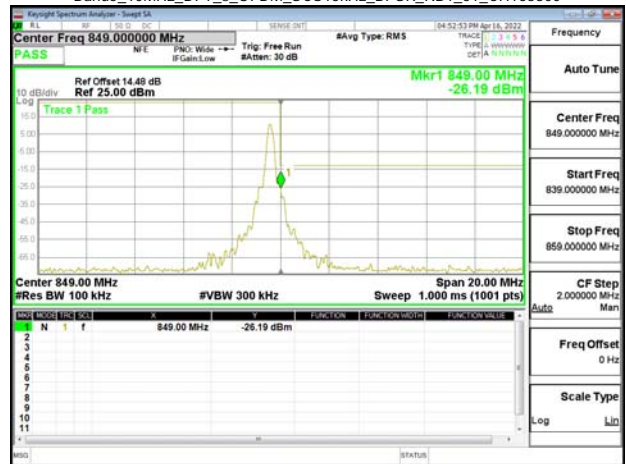
Band5_10MHz_DFT_s_OFDM_SCS15kHz_BPSK_RB1_51_CH168800
