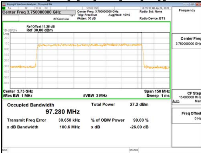
Band77-Part27_100MHz_CP_OFDM_SCS30kHz_256QAM_RB273_0_CH656000
