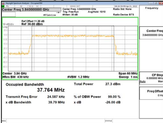
Band77-Part27_40MHz_CP_OFDM_SCS30kHz_256QAM_RB106_0_CH656000
