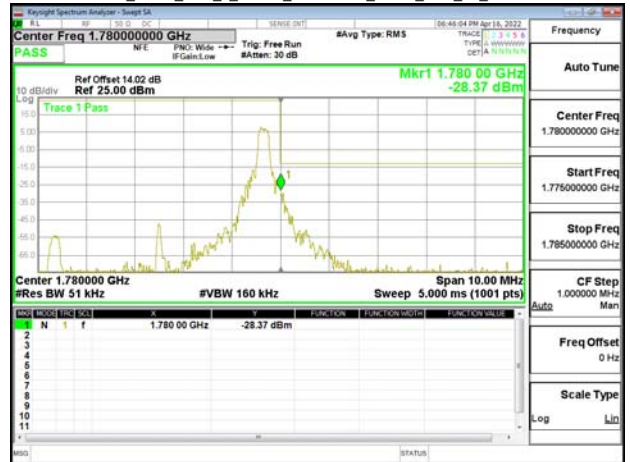
Band66_5MHz_DFT_s_OFDM_SCS15kHz_BPSK_RB1_24_CH355500
