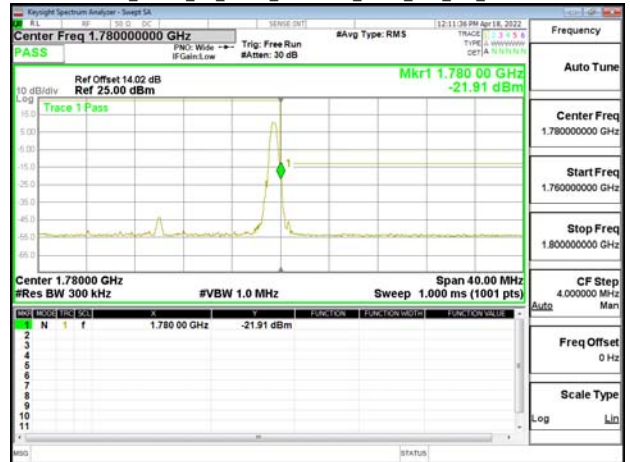
Band66_20MHz_CP_OFDM_SCS15kHz_QPSK_RB1_105_CH354000
