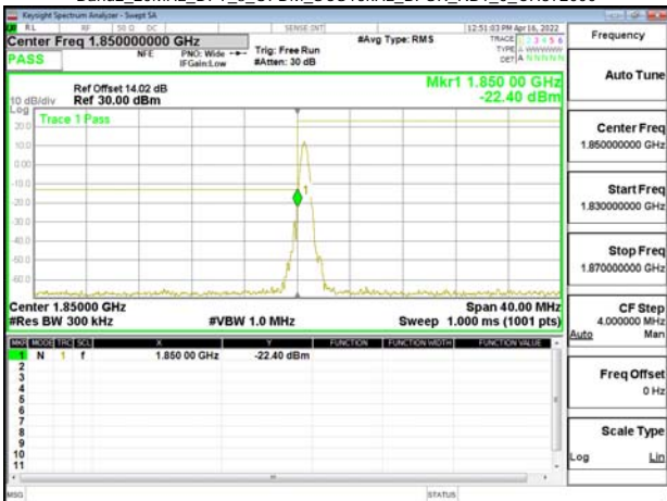
Band2_20MHz_DFT_s_OFDM_SCS15kHz_BPSK_RB1_0_CH372000
