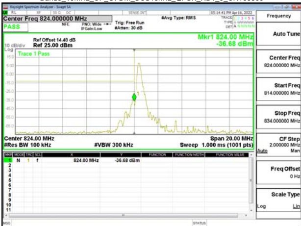
Band5_10MHz_CP_OFDM_SCS15kHz_OPK_RB1_0_CH165800
