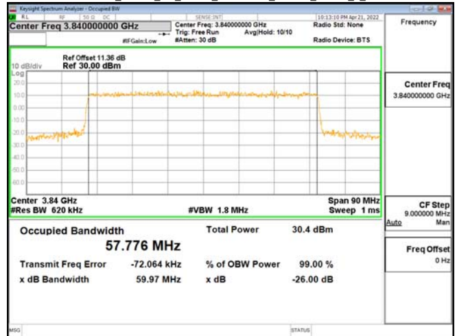
Band77-Part27_60MHz_CP_OFDM_SCS30kHz_64QAM_RB162_0_CH656000
