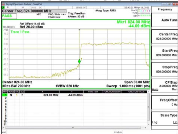
Band5_15MHz_DFT_s_OFDM_SCS15kHz_BPSK_RB75_0_CH166300
