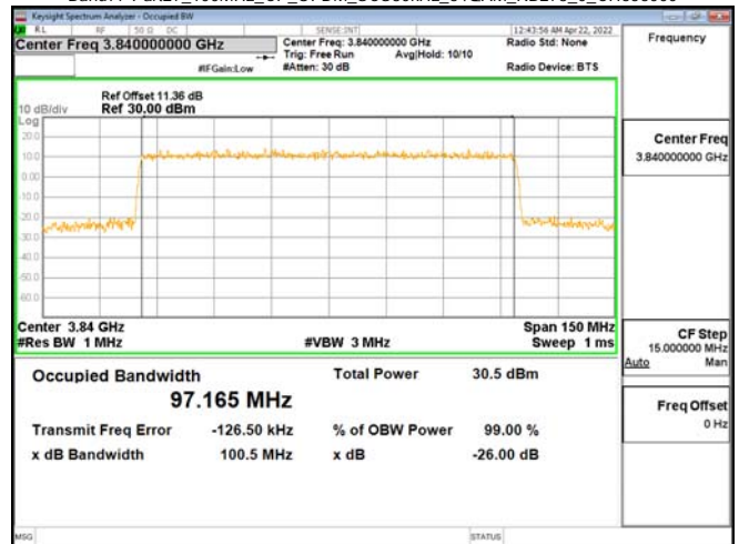
Band77-Part27_100MHz_CP_OFDM_SCS30kHz_64QAM_RB273_0_CH656000
