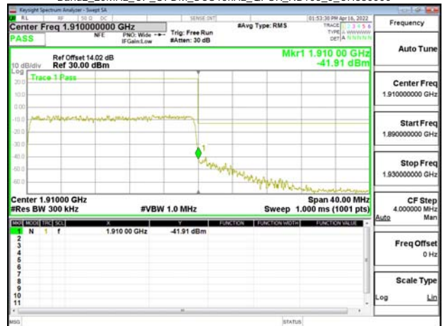
Band2_20MHz_CP_OFDM_SCS15kHz_QPSK_RB106_0_CH380000
