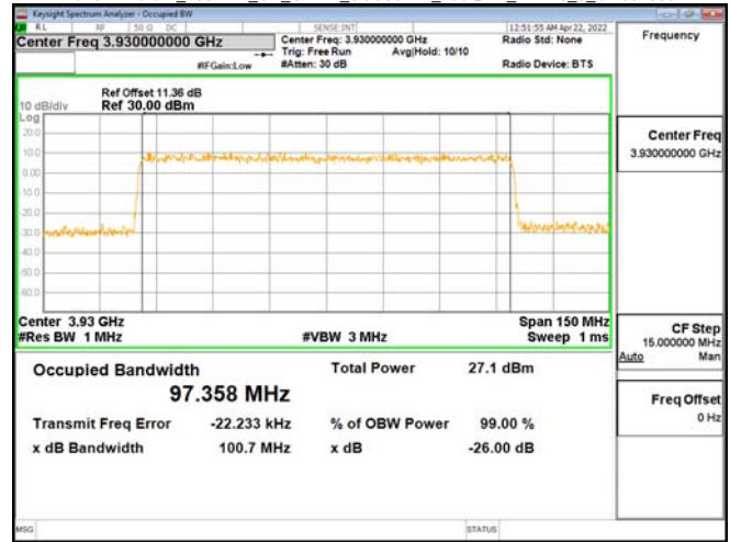
Band77-Part27_100MHz_CP_OFDM_SCS30kHz_256QAM_RB273_0_CH662000
