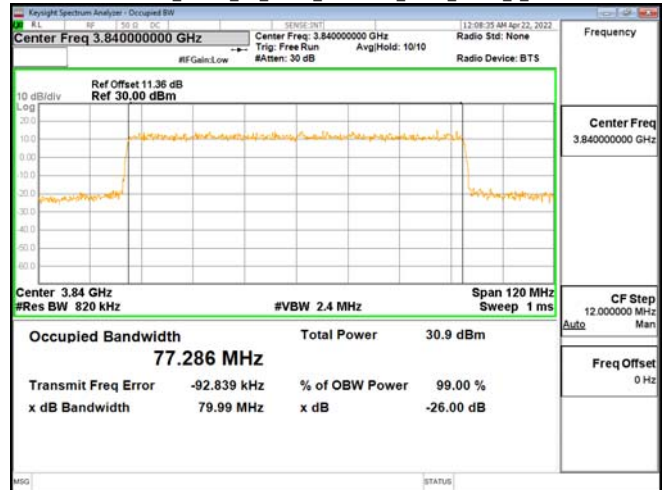
Band77-Part27_80MHz_CP_OFDM_SCS30kHz_QPSK_RB217_0_CH656000
