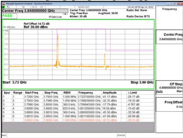
Band77-Part27_80MHz_CP_OFDM_SCS30kHz_OPSK_RB1_0_CH656000
