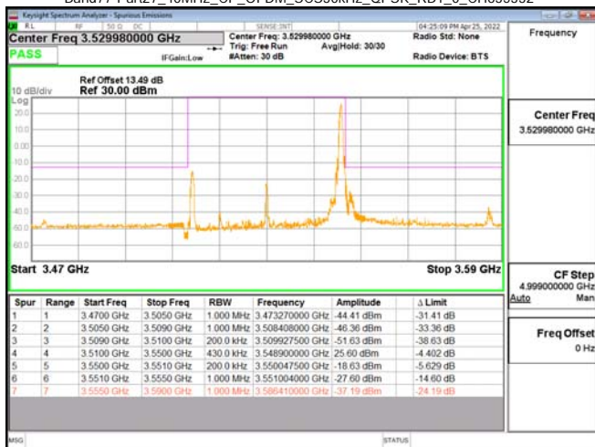
Band77-Part27_40MHz_CP_OFDM_SCS30kHz_OPSK_RB1_0_CH635332
