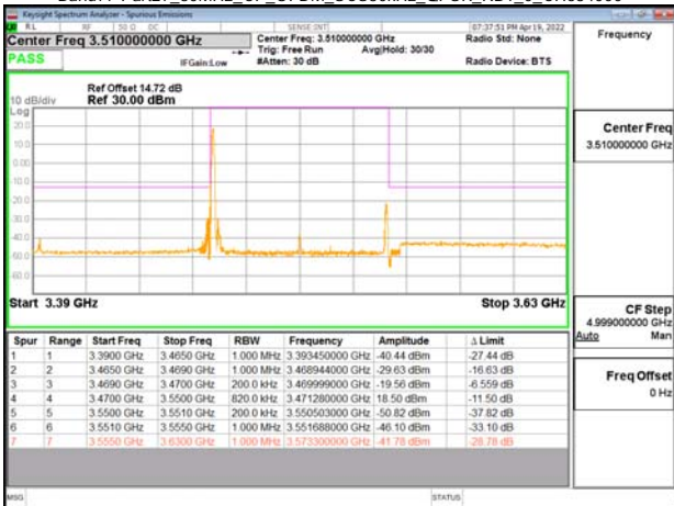
Band77-Part27_80MHz_CP_OFDM_SCS30kHz_OPSK_RB1_0_CH649334
