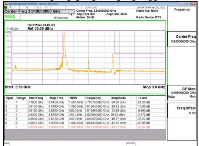
Band77-Part27_40MHz_CP_OFDM_SCS30kHz_OPSK_RB100_0_CH664000
