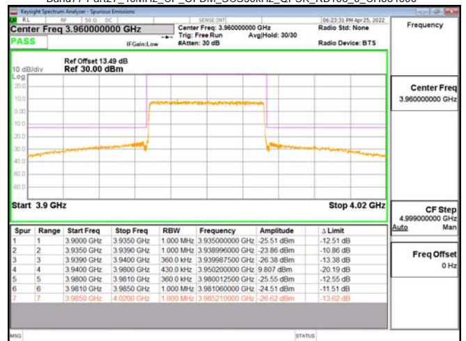
Band77-Part27_40MHz_CP_OFDM_SCS30kHz_OPSK_RB106_0_CH664000
