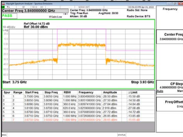
Band77-Part27_60MHz_CP_OFDM_SCS30kHz_OPSK_RB162_0_CH656000
