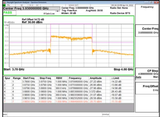
Band77-Part27_100MHz_CP_OFDM_SCS30kHz_QPSK_RB273_0_CH662000
