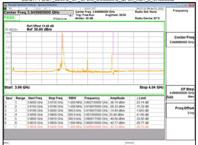
Band77-Part27_60MHz_CP_OFDM_SCS30kHz_OPSK_RB1_0_CH663332
