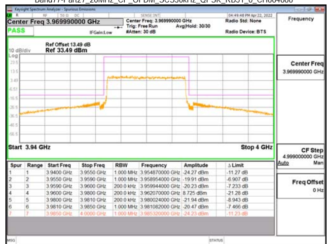
Band77-Part27_20MHz_CP_OFDM_SCS30kHz_QPSK_RB51_0_CH664666
