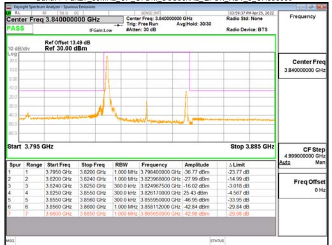
Band77-Part27_30MHz_CP_OFDM_SCS30kHz_OPSK_RB1_0_CH664332
