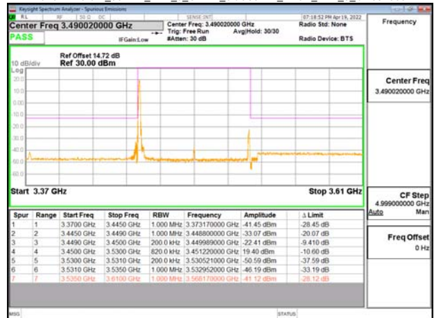
Band77-Part27_80MHz_DFT_s_OFDM_SCS30kHz_BPSK_RB1_0_CH633334
