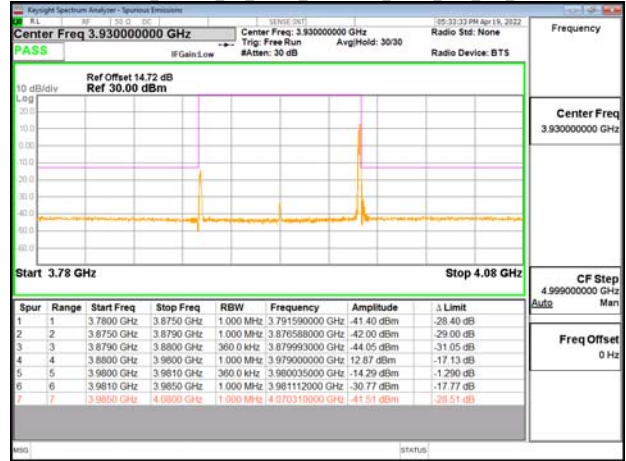
Band77-Part27_100MHz_CP_OFDM_SCS30kHz_OPK_RB1_272_CH662000
