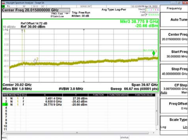
Band77-Part27_30MHz_DFT_s_OFDM_SCS30kHz_BPSK_RB1_1_CH633334
