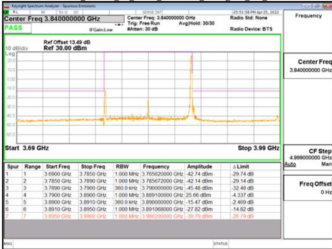
Band77-Part27_100MHz_CP_OFDM_SCS30kHz_OPK RB1_272_CH662000
