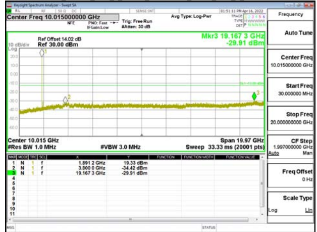
Band2_20MHz_DFT_s_OFDM_SCS15kHz_BPSK_RB1_1_CH380000
