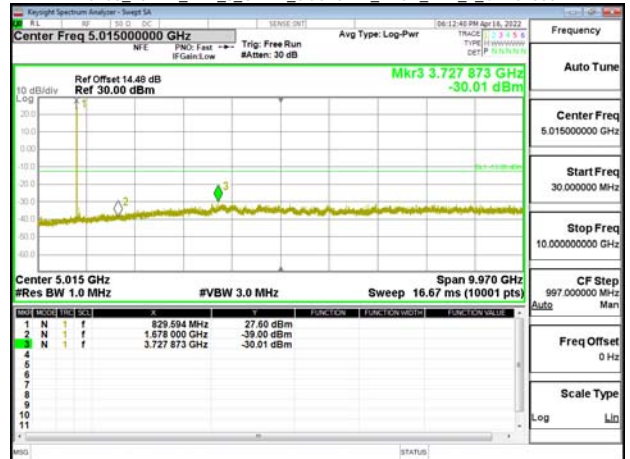
Band5_20MHz_DFT_s_OFDM_SCS15kHz_BPSK_RB1_1_CH167800
