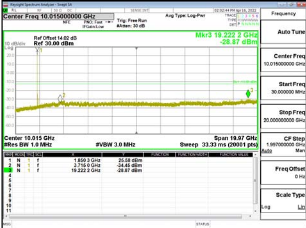
Band2_15MHz_DFT_s_OFDM_SCS15kHz_BPSK_RB1_1_CH376000
