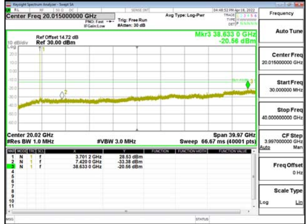
Band77-Part27_20MHz_DFT_s_OFDM_SCS30kHz_BPSK_RB1_1_CH656000
