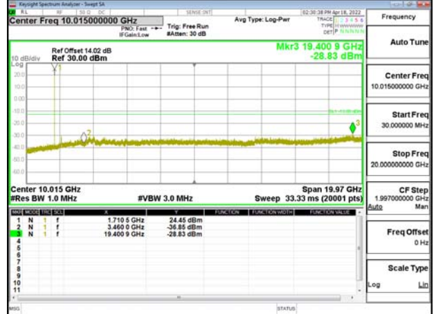
Band66_40MHz_DFT_s_OFDM_SCS15kHz_BPSK_RB1_1_CH349000
