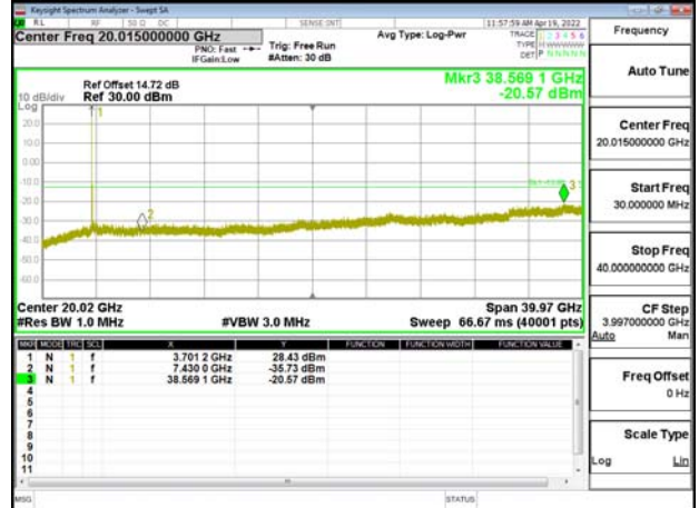
Band77-Part27_30MHz_DFT_s_OFDM_SCS30kHz_BPSK_RB1_1_CH656000
