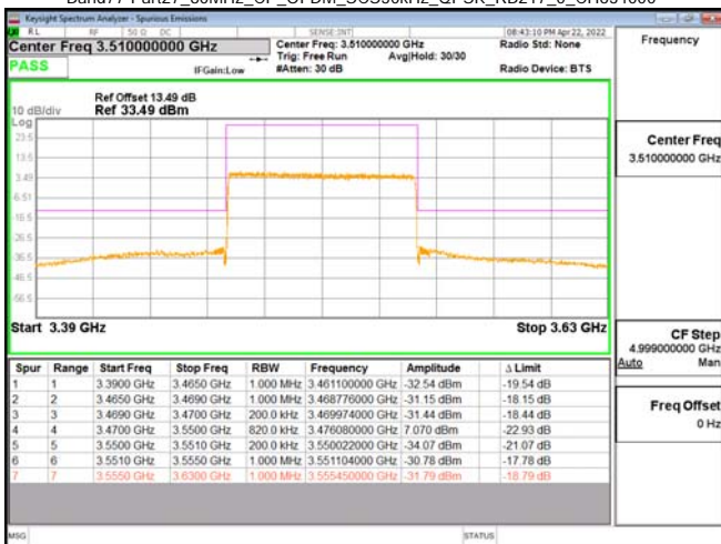
Band77-Part27_80MHz_CP_OFDM_SCS30kHz_OPSK_RB217_0_CH634000
