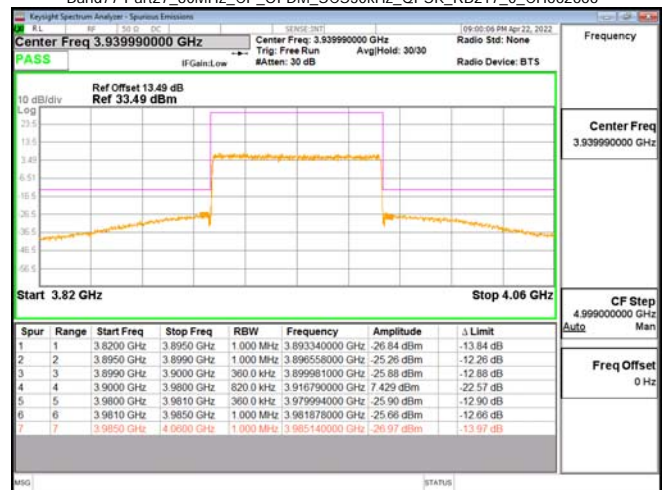
Band77-Part27_80MHz_CP_OFDM_SCS30kHz_OPSK_RB217_0_CH662666
