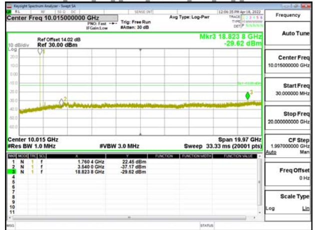
Band66_20MHz_DFT_s_OFDM_SCS15kHz_BPSK_RB1_1_CH354000
