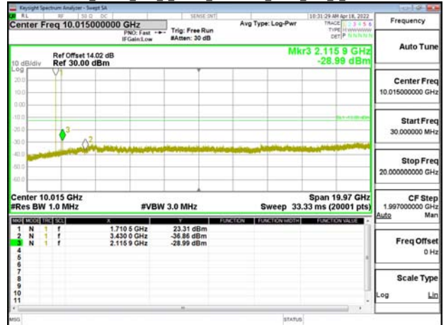
Band66_10MHz_DFT_s_OFDM_SCS15kHz_BPSK_RB1_1_CH349000
