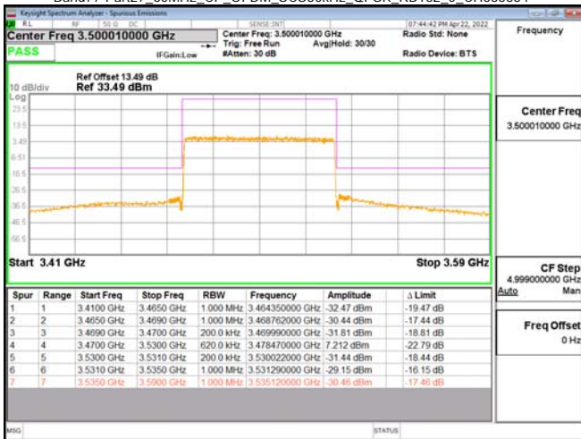
Band77-Part27_60MHz_CP_OFDM_SCS30kHz_OPSK_RB162_0_CH634666
