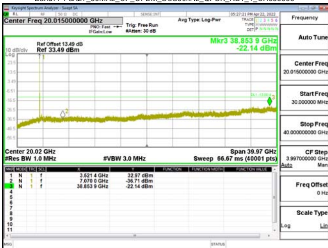
Band77-Part27_30MHz_CP_OFDM_SCS30kHz_OPSK_RB1_1_CH635666
