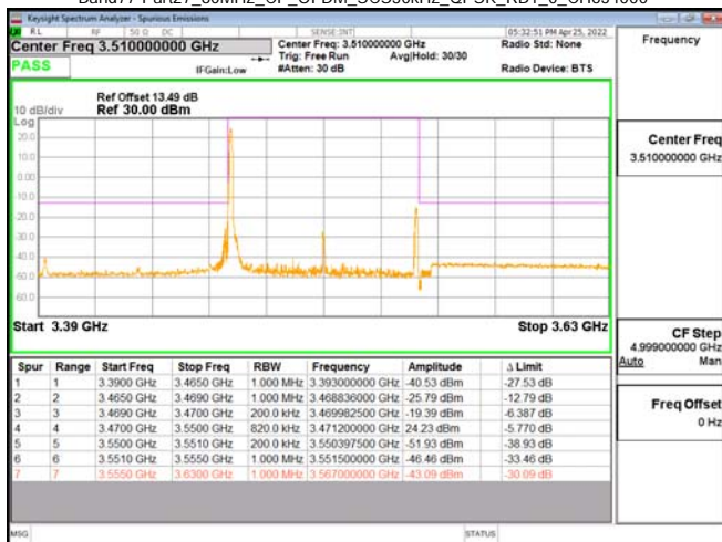
Band77-Part27_80MHz_CP_OFDM_SCS30kHz_OPSK_RB1_0_CH634000
