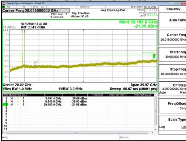
Band77-Part27_40MHz_CP_OFDM_SCS30kHz_OPSK_RB1_1_CH633334
