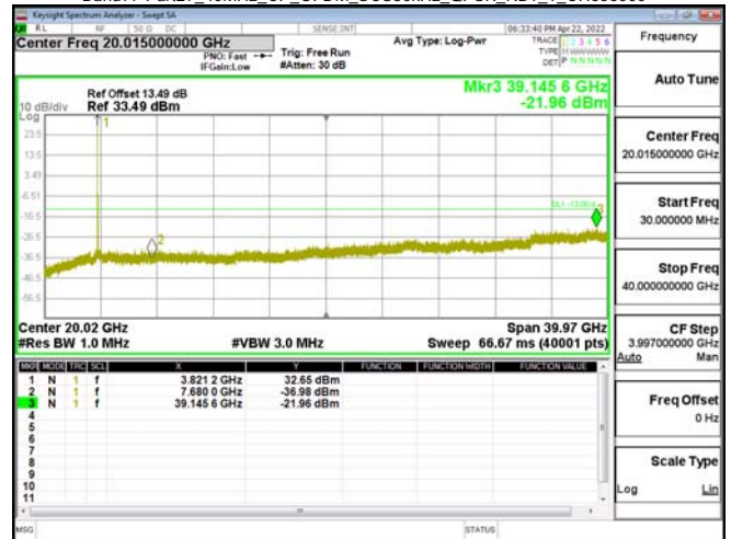
Band77-Part27_40MHz_CP_OFDM_SCS30kHz_OPSK_RB1_1_CH664000
