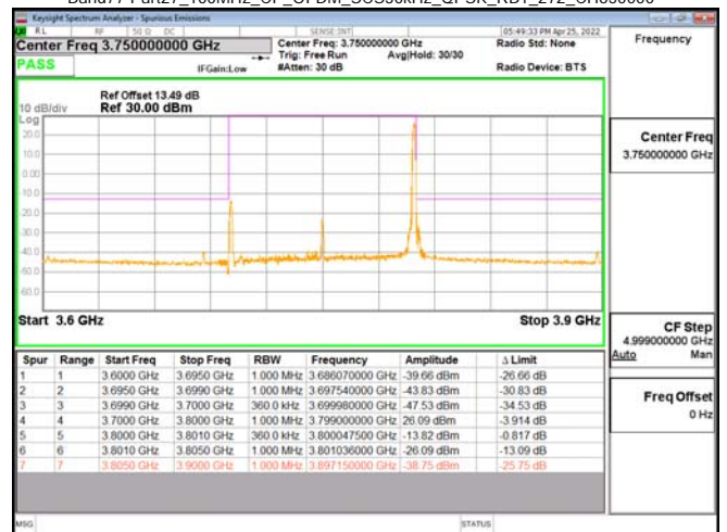
Band77-Part27_100MHz_CP_OFDM_SCS30kHz_OPK_RB1_272_CH650000
