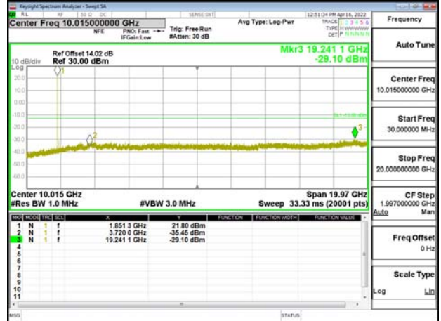
Band2_20MHz_DFT_s_OFDM_SCS15kHz_BPSK_RB1_1_CH376000
