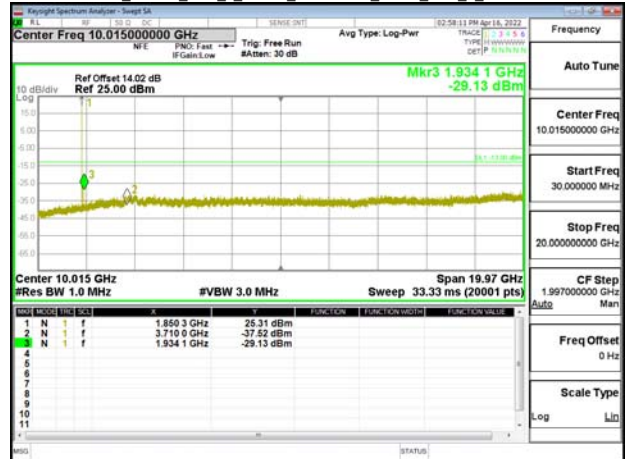
Band2_10MHz_DFT_s_OFDM_SCS15kHz_BPSK_RB1_1_CH376000
