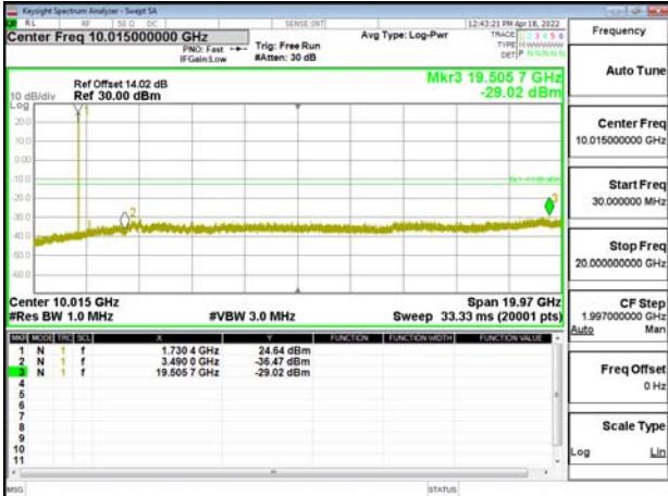
Band66_30MHz_DFT_s_OFDM_SCS15kHz_BPSK_RB1_1_CH353000
