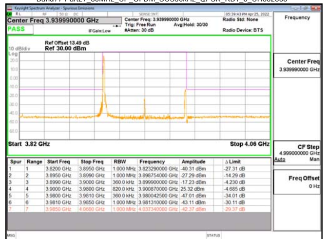
Band77-Part27_80MHz_CP_OFDM_SCS30kHz_OPSK_RB1_0_CH662666
