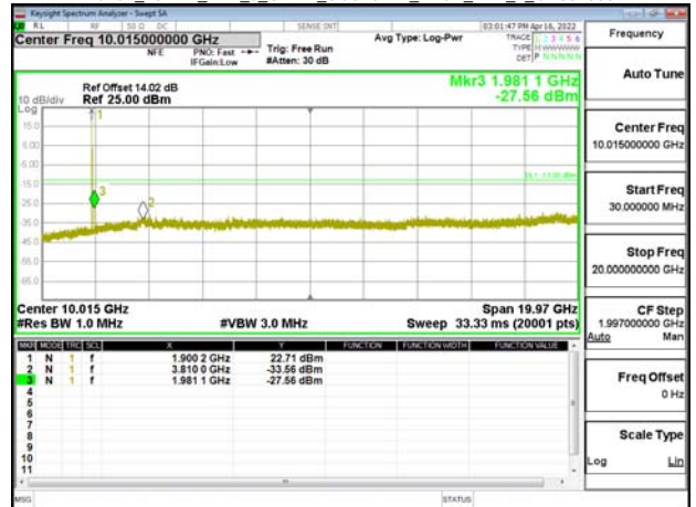
Band2_10MHz_DFT_s_OFDM_SCS15kHz_BPSK_RB1_1_CH381000
