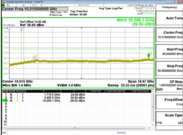
Band66_30MHz_DFT_s_OFDM_SCS15kHz_BPSK_RB1_1_CH349000
