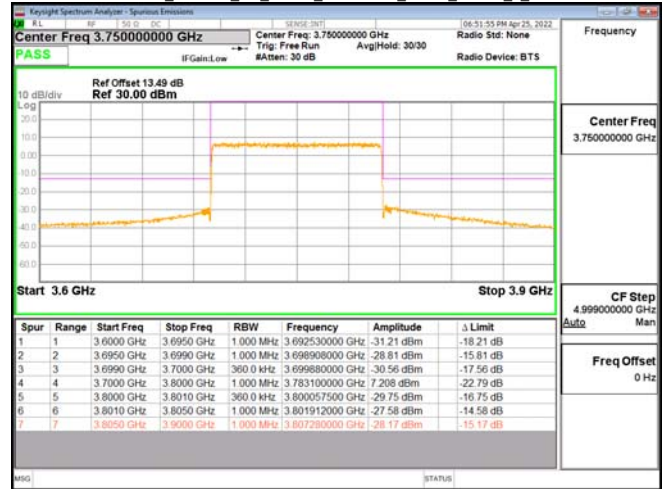
Band77-Part27_100MHz_CP_OFDM_SCS30kHz_OPK RB273_0_CH650000
