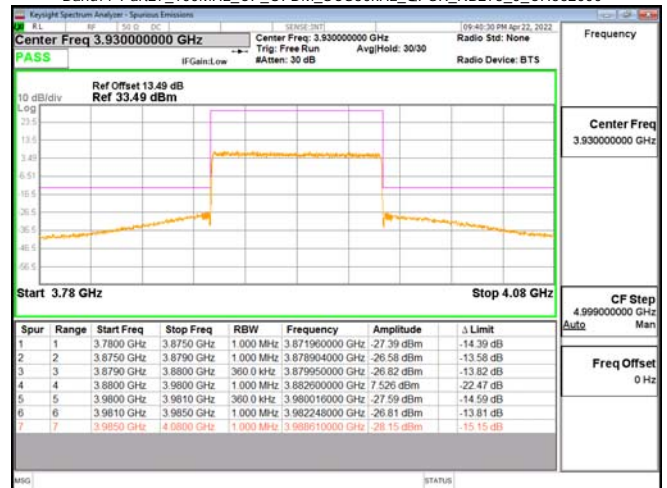
Band77-Part27_100MHz_CP_OFDM_SCS30kHz_OPK RB273_0_CH662000
