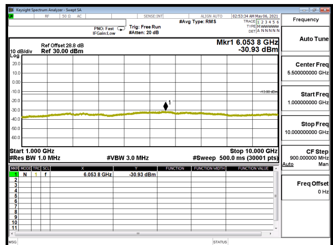
CSE-B12_10M-CH23095-64QAM(1,49)-1G-10G
