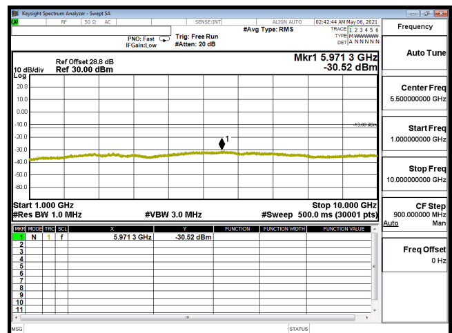
CSE-B12_5M-CH23035-64QAM(1,24)-1G-10G
