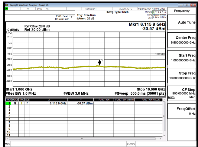
CSE-B12_10M-CH23130-QPSK(1,25)-1G-10G
