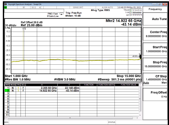
CSE-B30_5M-CH27685-QPSK(1,0)-1G-15G
