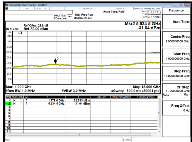
CSE-B66_3M-CH132657-QPSK(1,7)-1G-18G
