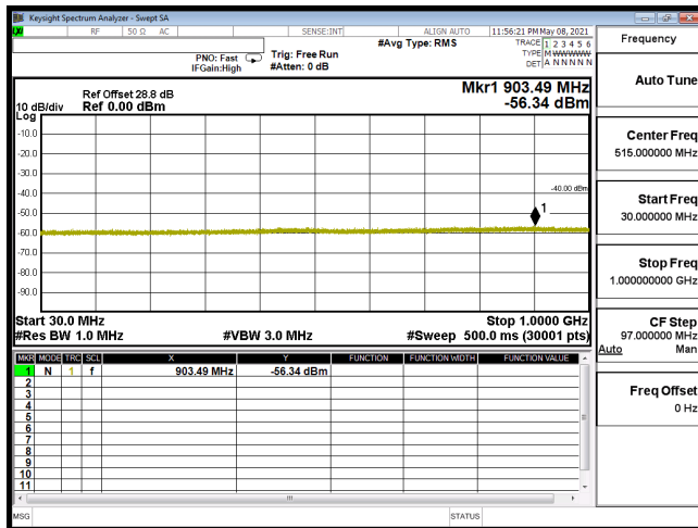
CSE-B30_5M-CH27735-QPSK(1,12)-30M-1G
