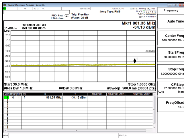
CSE-B66_1.4M-CH131979-16QAM(1,0)-30M-1G
