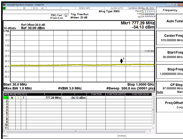
CSE-B66_1.4M-CH132665-QPSK(3,2)-30M-1G
