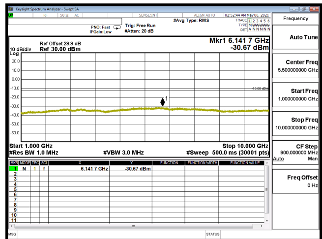
CSE-B12_10M-CH23060-16QAM(1,25)-1G-10G
