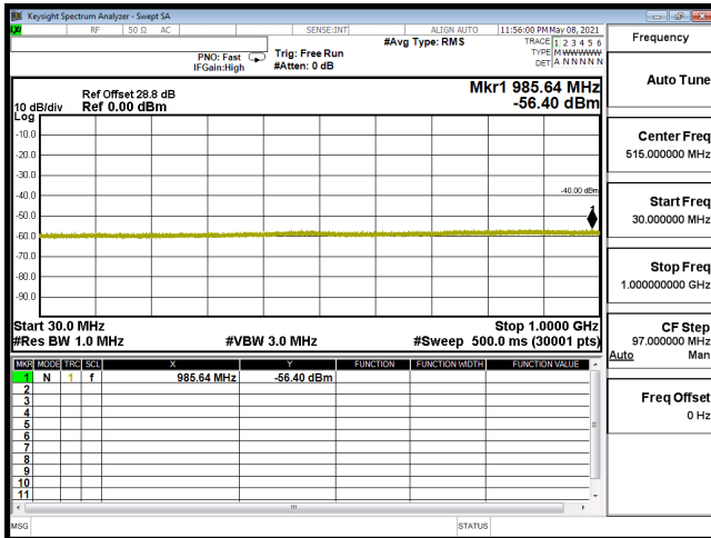
CSE-B30_5M-CH27710-16QAM(1,12)-30M-1G
