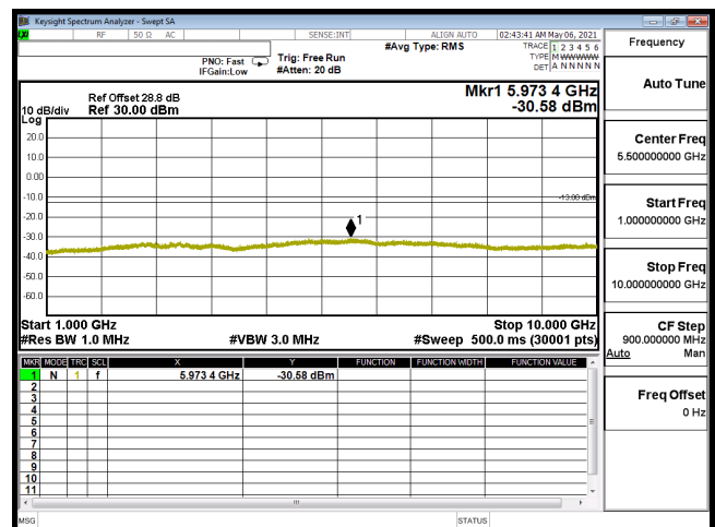
CSE-B12_5M-CH23095-64QAM(1,12)-1G-10G
