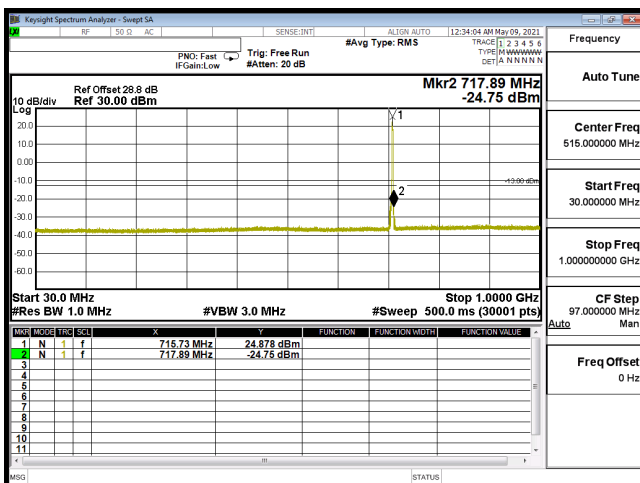
CSE-B12_3M-CH23165-64QAM(1,14)-30M-1G
