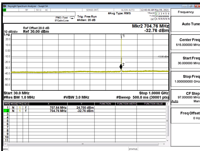
CSE-B12_5M-CH23095-64QAM(1,12)-30M-1G
