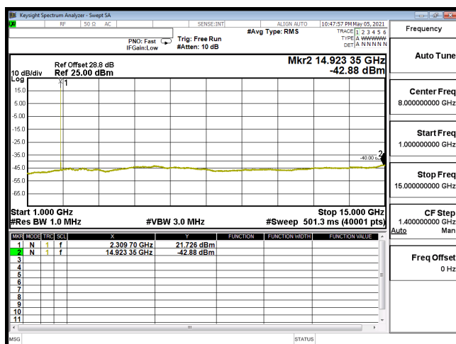
CSE-B30_5M-CH27685-16QAM(1,24)-1G-15G
