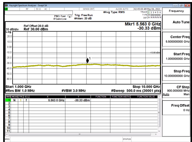
CSE-B12_5M-CH23155-16QAM(1,24)-1G-10G
