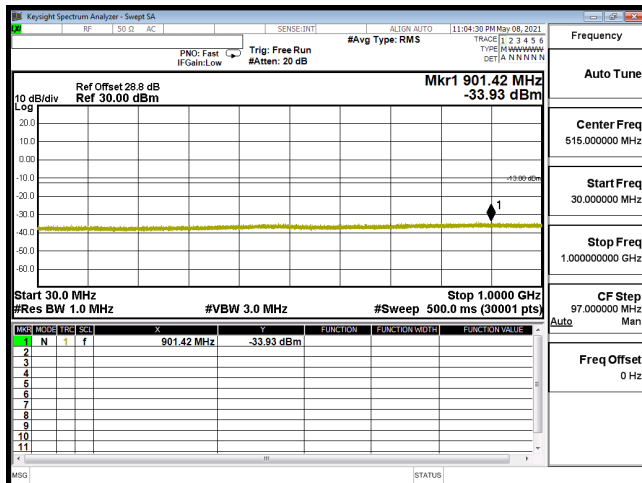
CSE-B66_3M-CH132657-QPSK(1,7)-30M-1G
