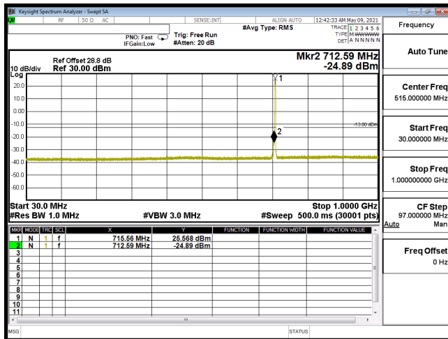
CSE-B12_5M-CH23155-QPSK(1,24)-30M-1G
