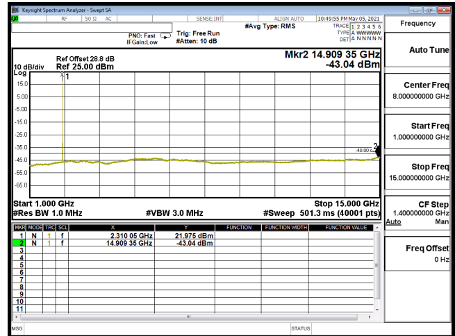
CSE-B30_5M-CH27710-16QAM(1,12)-1G-15G
