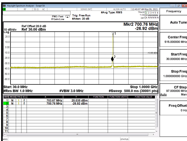
CSE-B12_5M-CH23035-64QAM(1,24)-30M-1G
