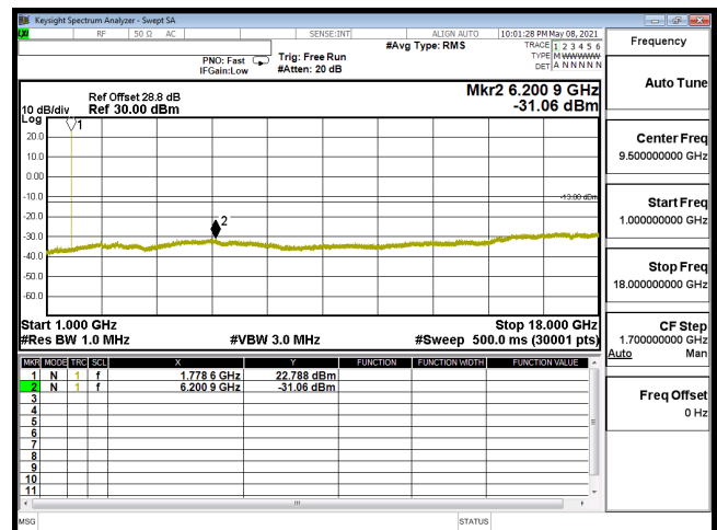
CSE-B66_3M-CH132657-16QAM(1,7)-1G-18G
