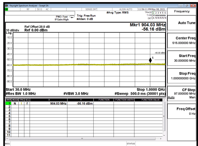
CSE-B30_5M-CH27710-64QAM(1,0)-30M-1G
