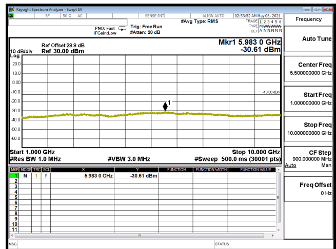
CSE-B12_10M-CH23095-16QAM(1,49)-1G-10G
