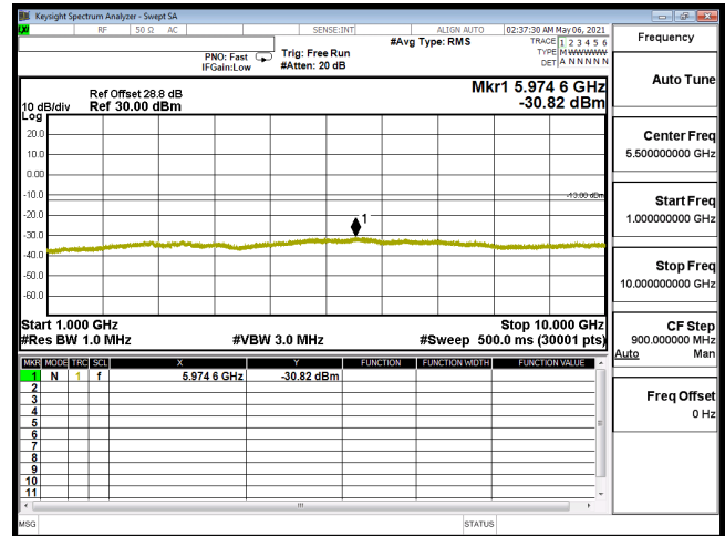
CSE-B12_3M-CH23165-QPSK(1,14)-1G-10G
