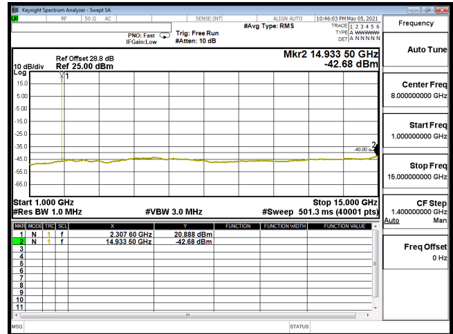
CSE-B30_5M-CH27685-64QAM(1,12)-1G-15G
