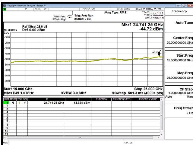
CSE-B30_5M-CH27710-16QAM(1,12)-15G-25G
