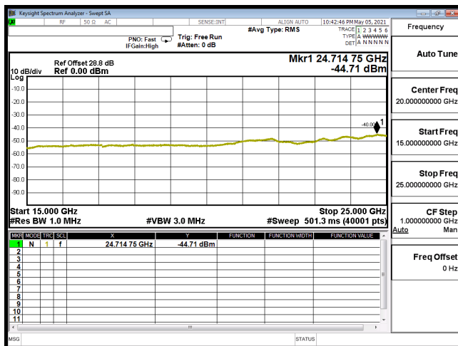
CSE-B30_5M-CH27735-QPSK(1,12)-15G-25G
