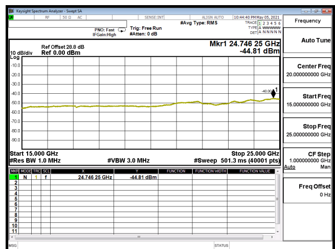
CSE-B30_5M-CH27685-16QAM(1,24)-15G-25G
