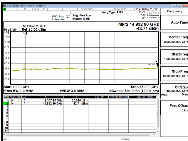
CSE-B30_5M-CH27710-64QAM(1,0)-1G-15G
