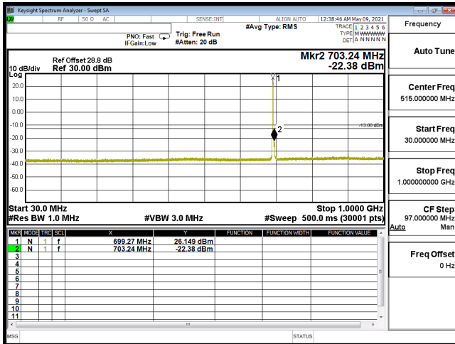
CSE-B12_5M-CH23035-QPSK(1,0)-30M-1G
