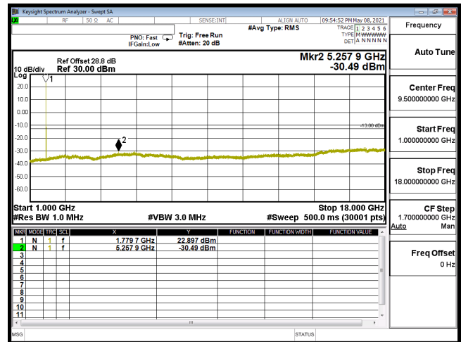
CSE-B66_1.4M-CH132665-QPSK(3,2)-1G-18G
