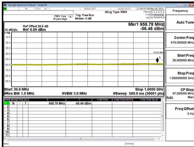
CSE-B30_5M-CH27735-64QAM(1,12)-30M-1G
