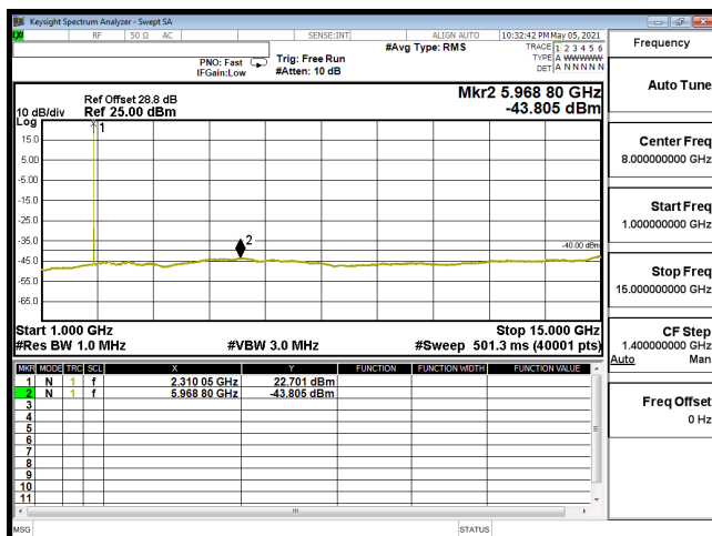
CSE-B30_10M-CH27710-QPSK(1,25)-1G-15G
