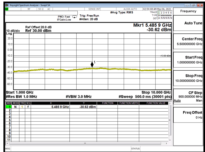
CSE-B12_10M-CH23095-QPSK(1,49)-1G-10G
