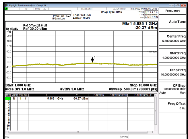
CSE-B12_3M-CH23165-16QAM(1,7)-1G-10G
