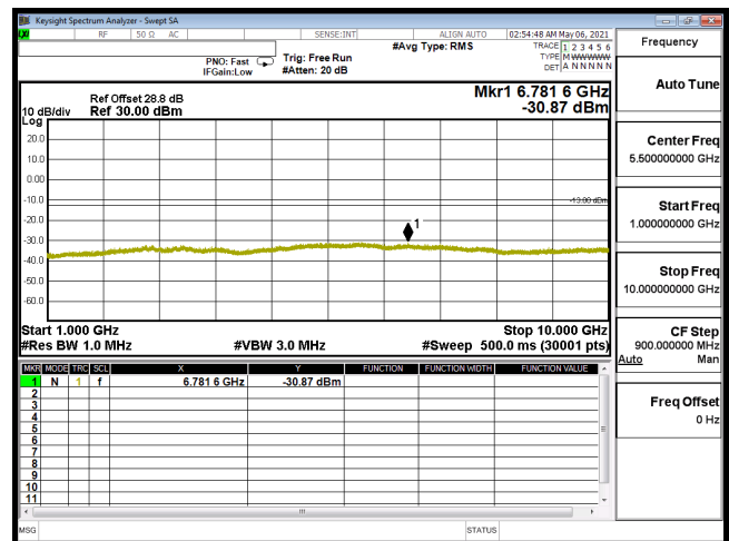
CSE-B12_10M-CH23130-16QAM(1,25)-1G-10G
