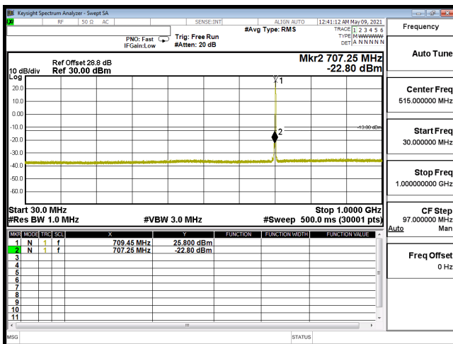
CSE-B12_5M-CH23095-16QAM(1,24)-30M-1G
