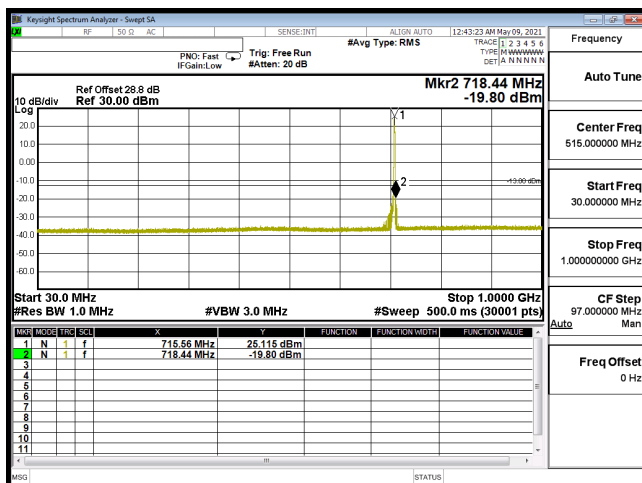
CSE-B12_5M-CH23155-64QAM(1,24)-30M-1G
