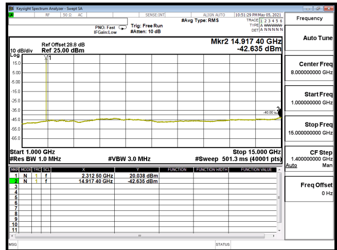
CSE-B30_5M-CH27735-64QAM(1,12)-1G-15G
