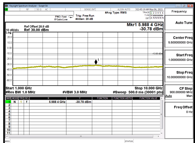
CSE-B12_5M-CH23155-64QAM(1,24)-1G-10G
