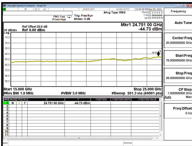
CSE-B30_5M-CH27685-64QAM(1,12)-15G-25G
