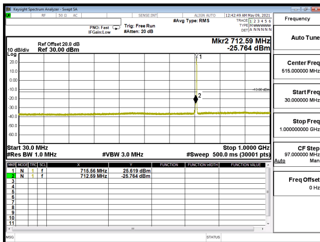
CSE-B12_5M-CH23155-16QAM(1,24)-30M-1G
