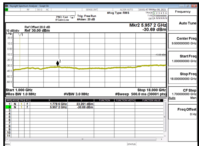
CSE-B66_3M-CH132657-64QAM(1,7)-1G-18G
