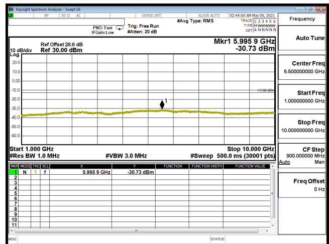
CSE-B12_5M-CH23095-16QAM(1,24)-1G-10G
