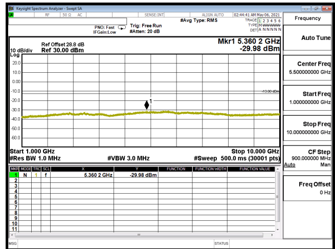
CSE-B12_5M-CH23155-QPSK(1,24)-1G-10G
