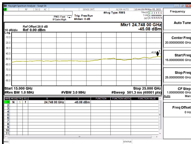
CSE-B30_5M-CH27685-QPSK(1,0)-15G-25G
