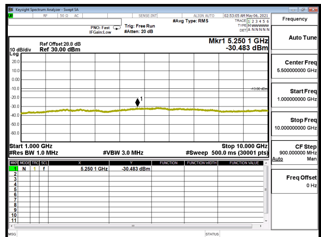
CSE-B12_10M-CH23060-64QAM(1,25)-1G-10G
