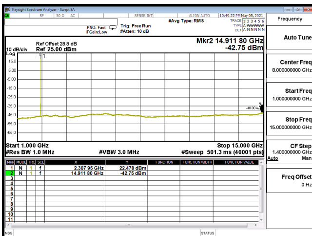
CSE-B30_5M-CH27710-QPSK(1,0)-1G-15G
