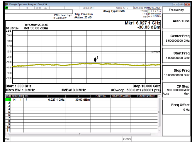
CSE-B12_10M-CH23060-QPSK(1,25)-1G-10G
