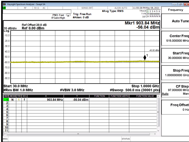
CSE-B30_5M-CH27685-64QAM(1,12)-30M-1G
