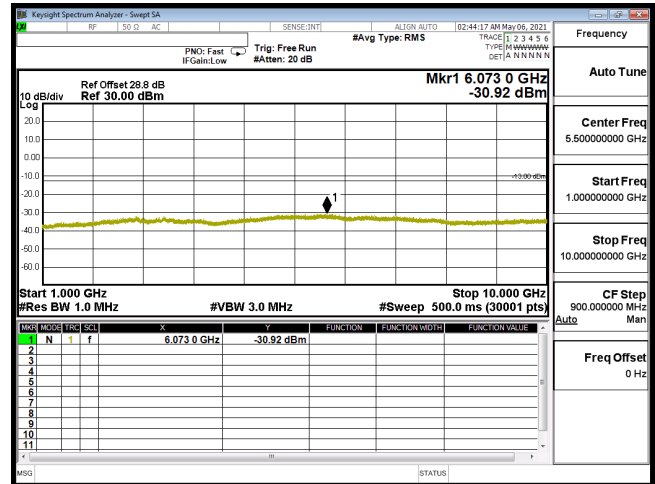
CSE-B12_5M-CH23095-QPSK(1,24)-1G-10G
