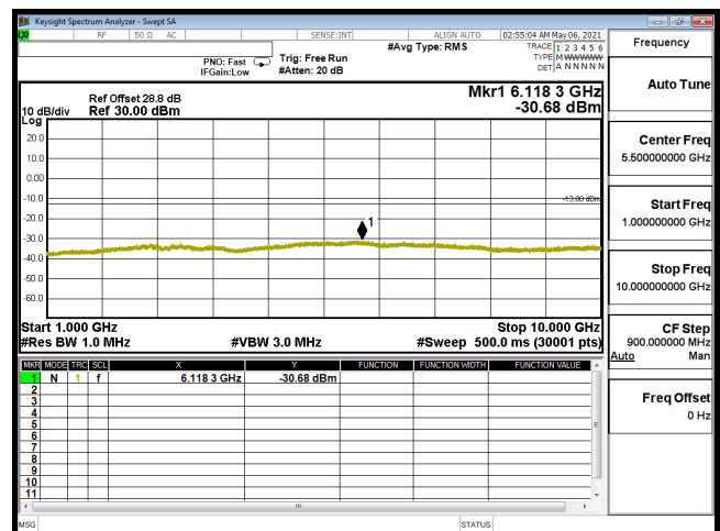
CSE-B12_10M-CH23130-64QAM(1,25)-1G-10G
