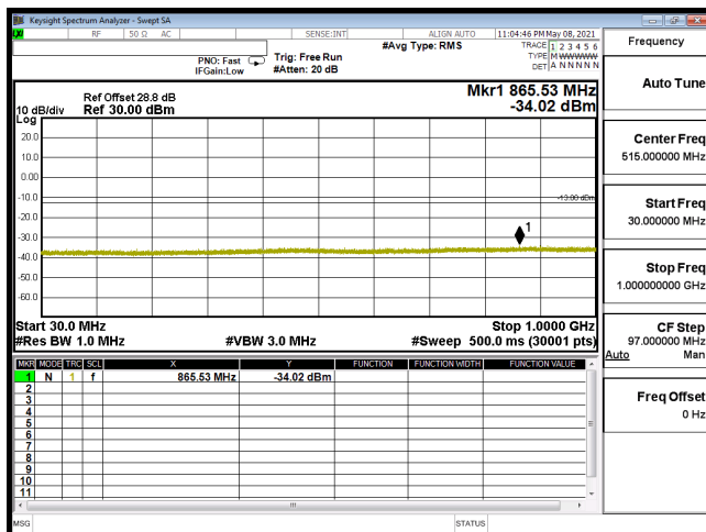
CSE-B66_3M-CH132657-16QAM(1,7)-30M-1G
