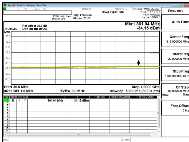
CSE-B66_1.4M-CH131979-64QAM(1,0)-30M-1G
