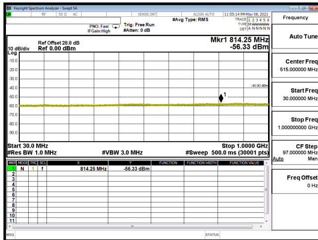
CSE-B30_5M-CH27685-QPSK(1,0)-30M-1G
