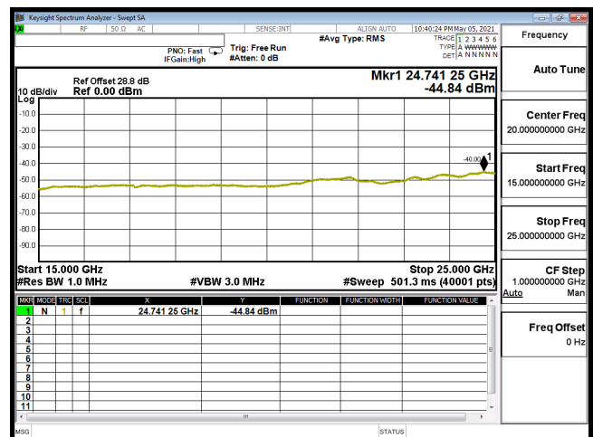
CSE-B30_5M-CH27710-QPSK(1,0)-15G-25G
