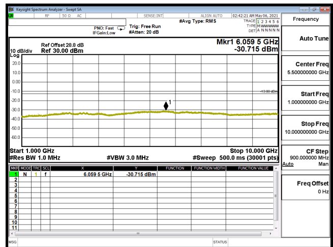
CSE-B12_5M-CH23035-16QAM(1,24)-1G-10G
