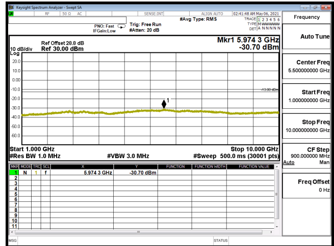
CSE-B12_5M-CH23035-QPSK(1,0)-1G-10G
