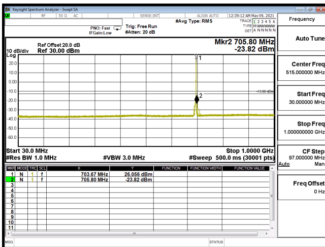
CSE-B12_5M-CH23035-16QAM(1,24)-30M-1G
