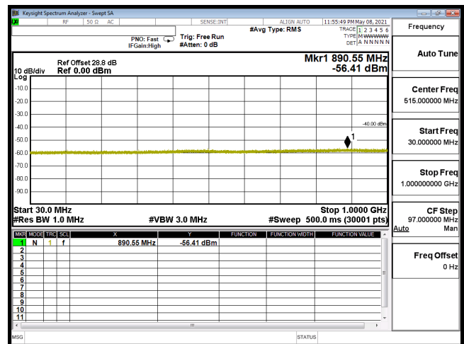
CSE-B30_5M-CH27710-QPSK(1,0)-30M-1G
