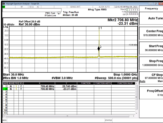
CSE-B12_5M-CH23095-QPSK(1,24)-30M-1G
