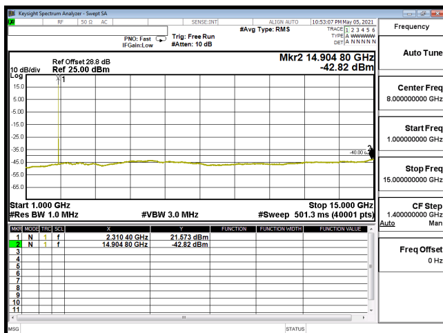
CSE-B30_5M-CH27735-16QAM(1,0)-1G-15G
