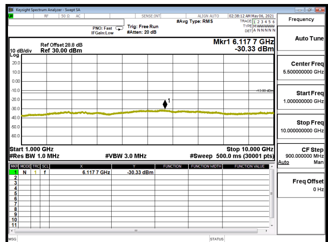
CSE-B12_3M-CH23165-64QAM(1,14)-1G-10G
