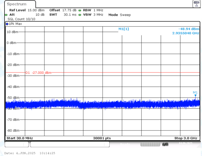
11AX80MIMO-Ant2-6465-30~3000-PASS
