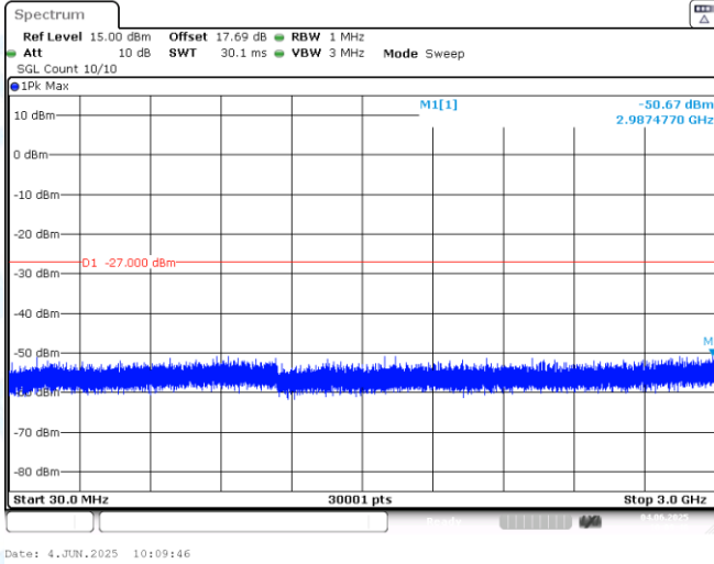
11AX80MIMO-Ant1-6465-30~3000-PASS
