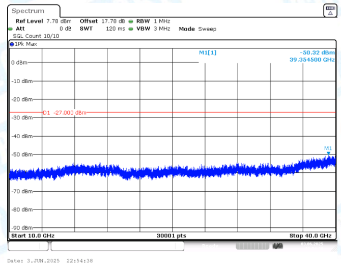
11AX40MIMO-Ant2-6525-10000~40000-PASS
