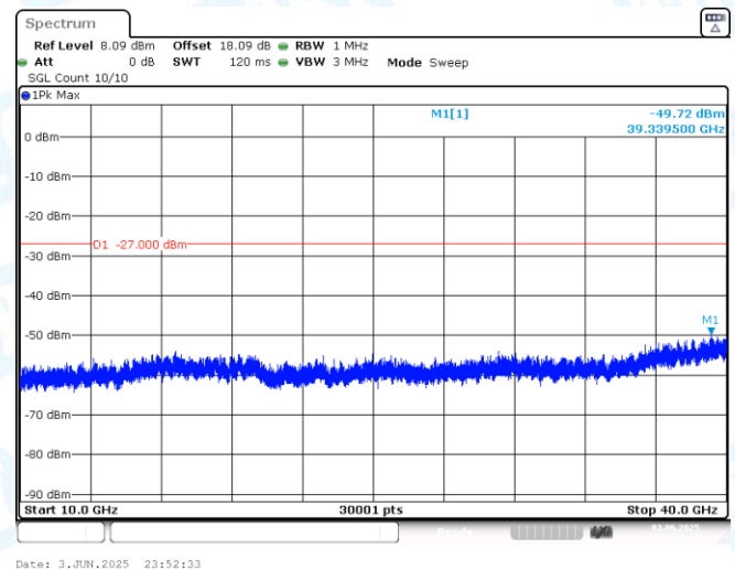
11AX40MIMO-Ant2-6925-10000~40000-PASS
