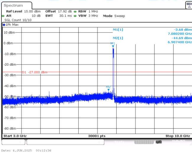
11AX40MIMO-Ant1-7085-3000~10000-PASS
