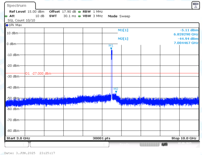
11AX40MIMO-Ant2-6845-3000~10000-PASS
