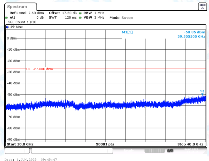
11AX80MIMO-Ant2-6145-10000~40000-PASS
