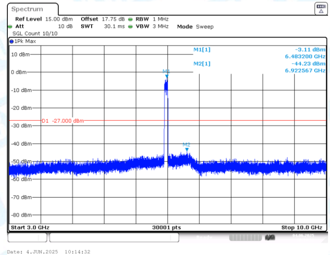
11AX80MIMO-Ant2-6465-3000~10000-PASS
