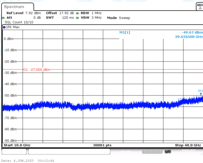
11AX40MIMO-Ant1-7085-10000~40000-PASS
