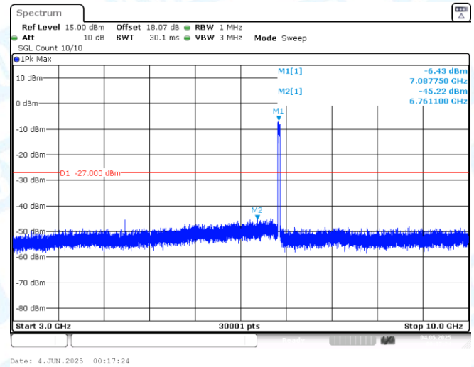
11AX40MIMO-Ant2-7085-3000~10000-PASS
