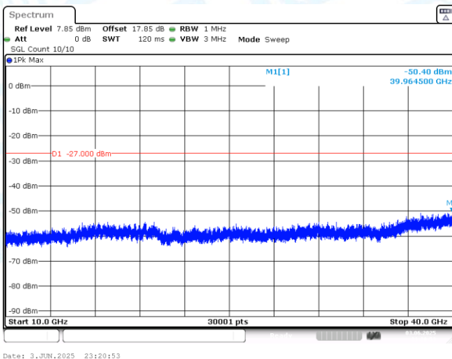
11AX40MIMO-Ant1-6845-10000~40000-PASS
