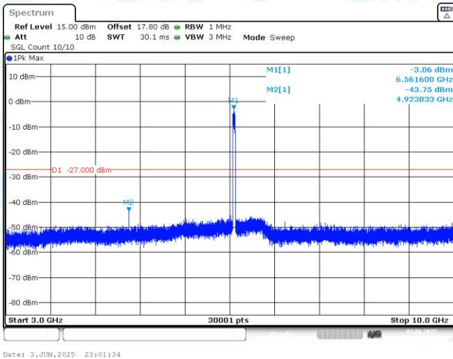
11AX40MIMO-Ant1-6565-3000~10000-PASS
