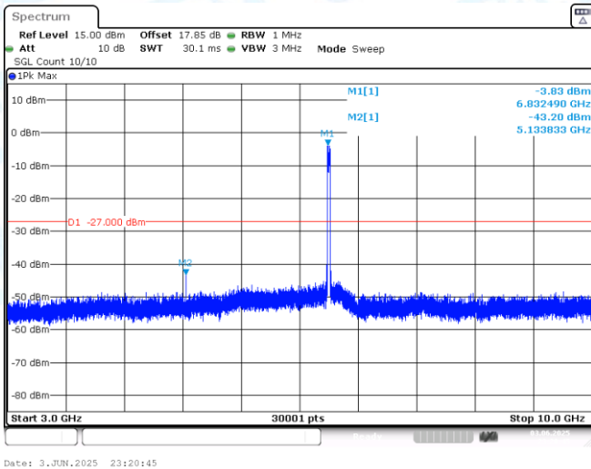
11AX40MIMO-Ant1-6845-3000~10000-PASS
