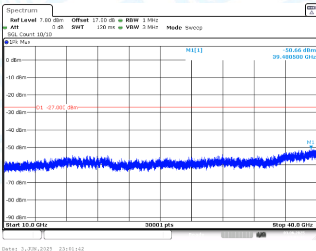
11AX40MIMO-Ant1-6565-10000~40000-PASS
