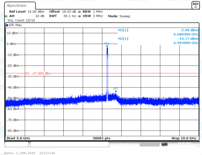
11AX40MIMO-Ant2-6685-3000~10000-PASS
