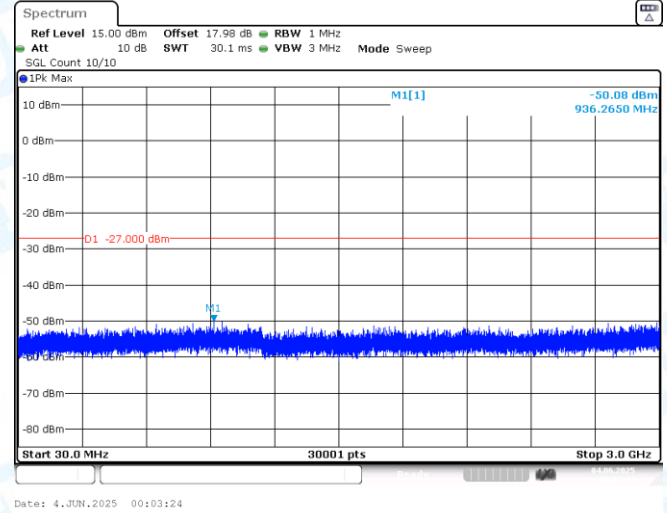
11AX40MIMO-Ant2-6965-30~3000-PASS
