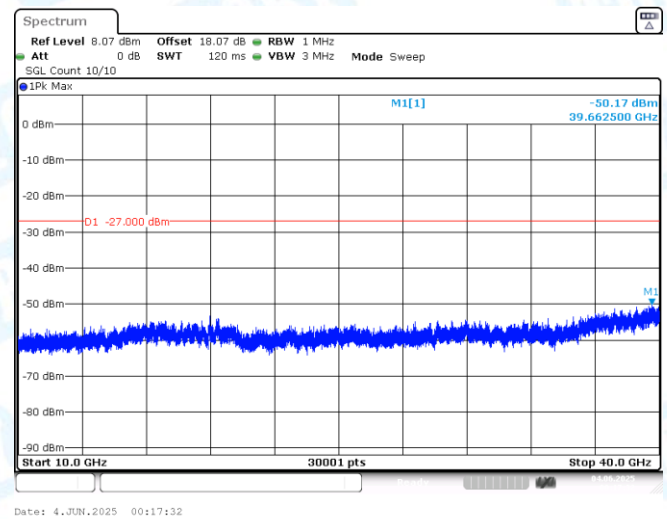
11AX40MIMO-Ant2-7085-10000~40000-PASS
