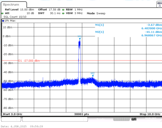
11AX80MIMO-Ant1-6385-3000~10000-PASS
