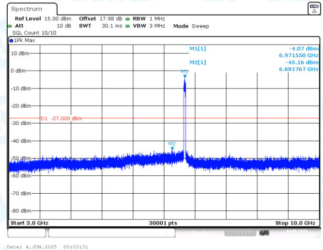
11AX40MIMO-Ant2-6965-3000~10000-PASS
