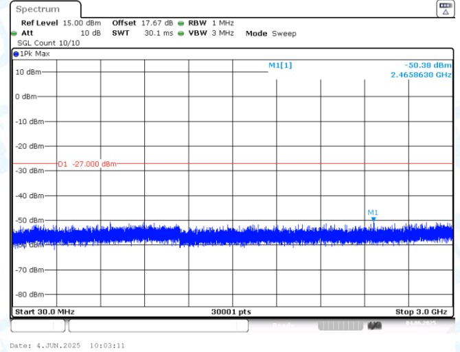
11AX80MIMO-Ant2-6385-30~3000-PASS
