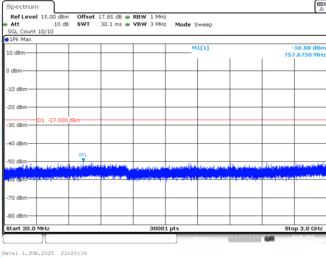
11AX40MIMO-Ant1-6845-30~3000-PASS
