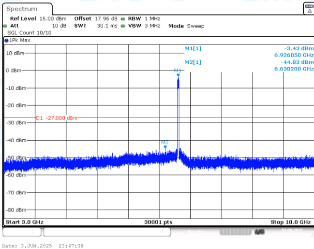
11AX40MIMO-Ant1-6925-3000~10000-PASS
