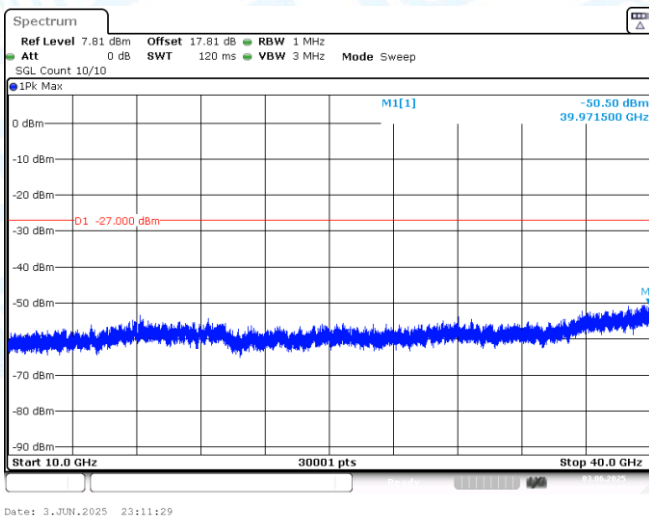
11AX40MIMO-Ant1-6685-10000~40000-PASS
