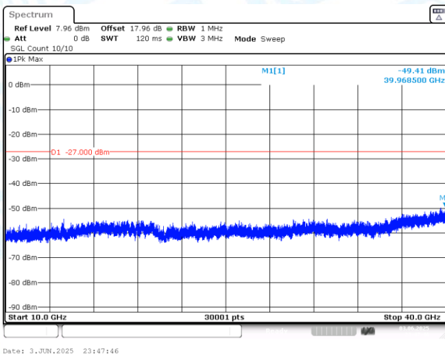
11AX40MIMO-Ant1-6925-10000~40000-PASS
