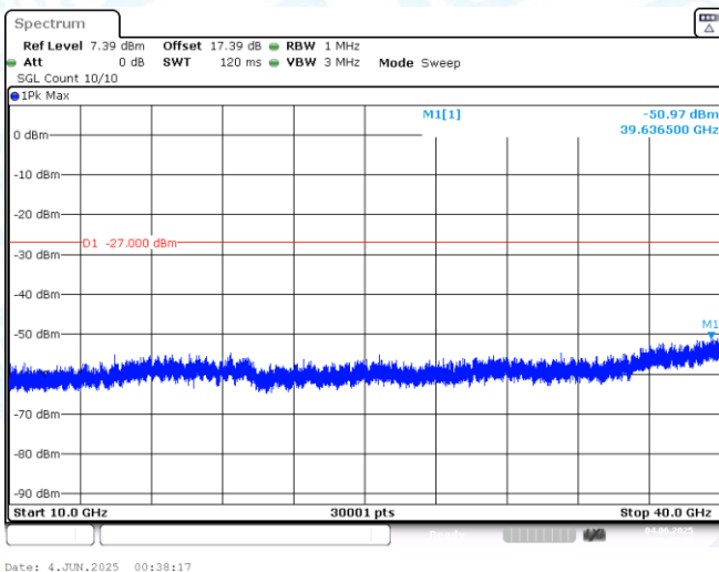
11AX80MIMO-Ant1-5985-10000~40000-PASS
