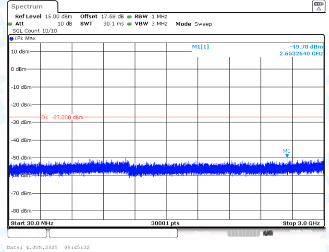
11AX80MIMO-Ant2-6145-30~3000-PASS
