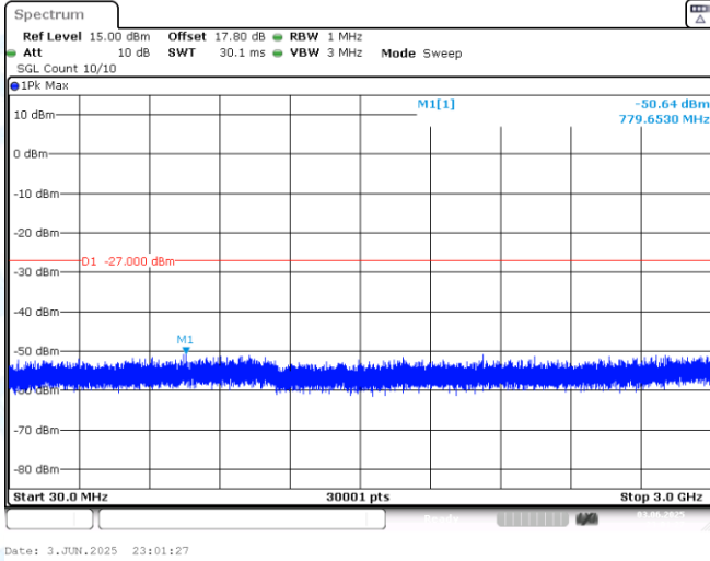
11AX40MIMO-Ant1-6565-30~3000-PASS
