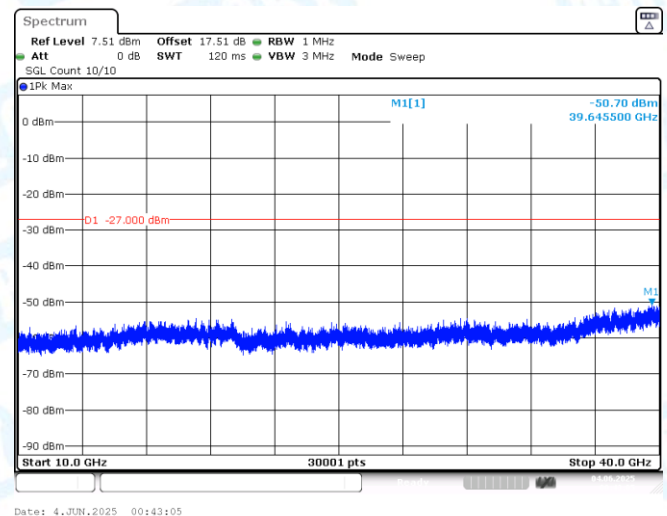
11AX80MIMO-Ant2-5985-10000~40000-PASS
