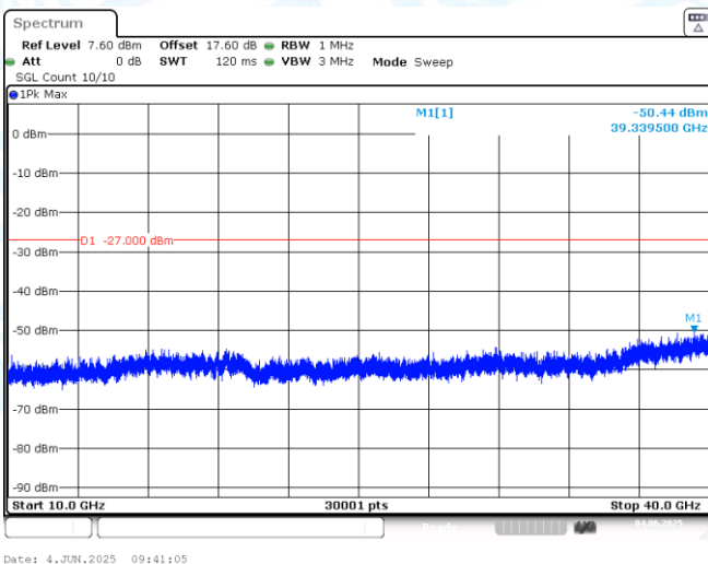
11AX80MIMO-Ant1-6145-10000~40000-PASS
