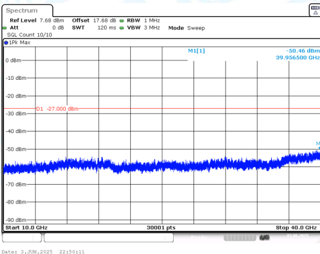
11AX40MIMO-Ant1-6525-10000~40000-PASS
