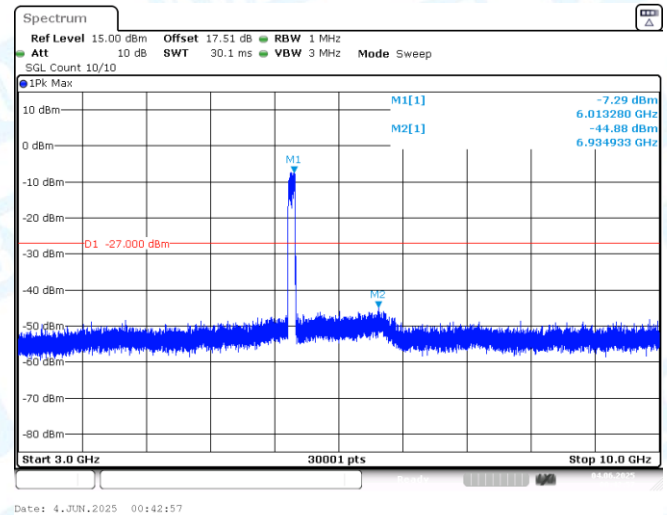
11AX80MIMO-Ant2-5985-3000~10000-PASS
