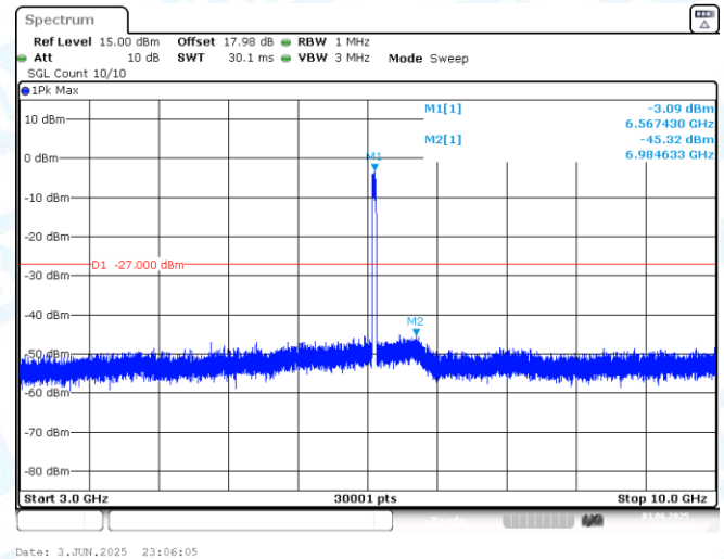
11AX40MIMO-Ant2-6565-3000~10000-PASS
