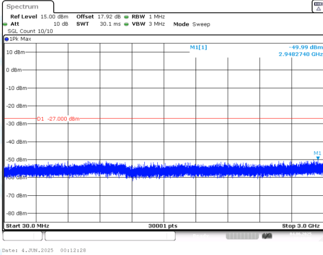
11AX40MIMO-Ant1-7085-30~3000-PASS
