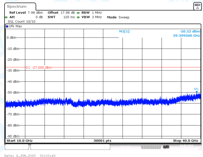
11AX40MIMO-Ant2-6965-10000~40000-PASS
