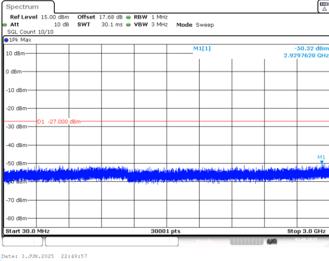
11AX40MIMO-Ant1-6525-30~3000-PASS
