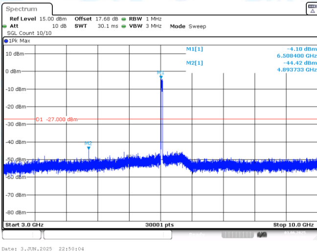
11AX40MIMO-Ant1-6525-3000~10000-PASS
