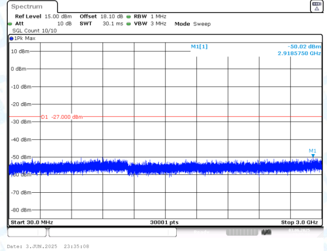
11AX40MIMO-Ant2-6885-30~3000-PASS
