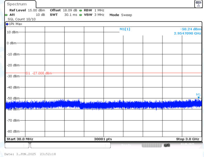
11AX40MIMO-Ant2-6925-30~3000-PASS
