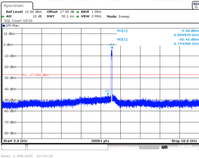
11AX40MIMO-Ant1-6885-3000~10000-PASS
