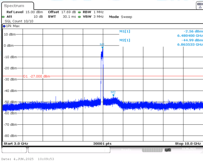
11AX80MIMO-Ant1-6465-3000~10000-PASS
