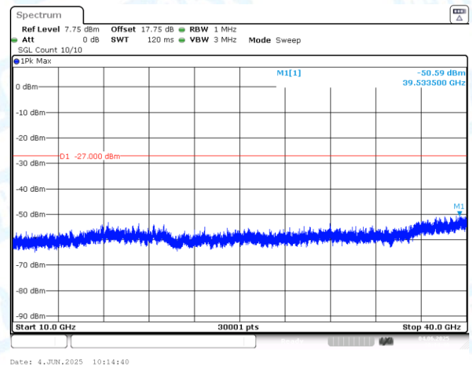
11AX80MIMO-Ant2-6465-10000~40000-PASS
