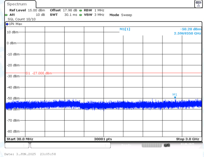
11AX40MIMO-Ant2-6565-30~3000-PASS
