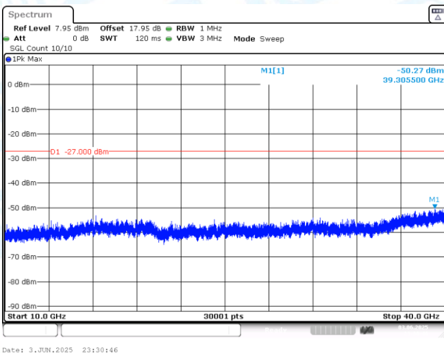
11AX40MIMO-Ant1-6885-10000~40000-PASS
