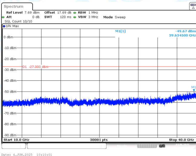
11AX80MIMO-Ant1-6465-10000~40000-PASS
