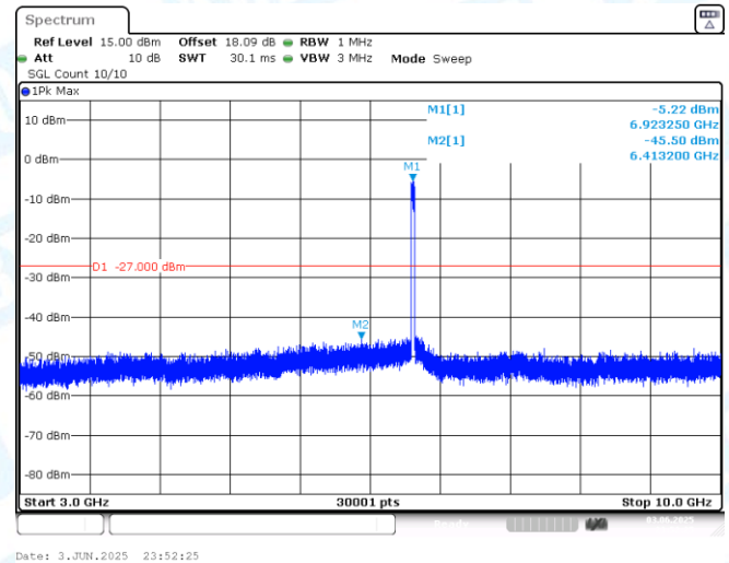
11AX40MIMO-Ant2-6925-3000~10000-PASS
