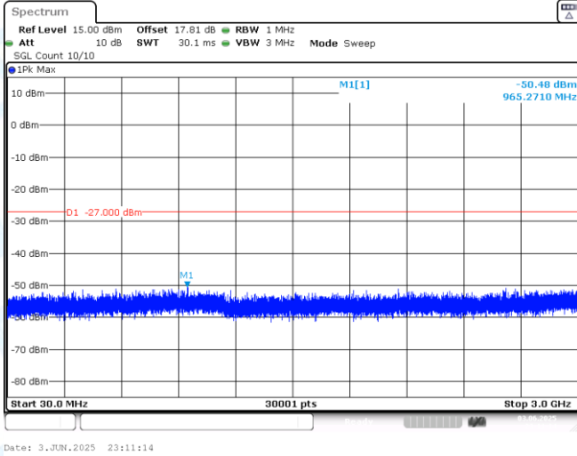
11AX40MIMO-Ant1-6685-30~3000-PASS
