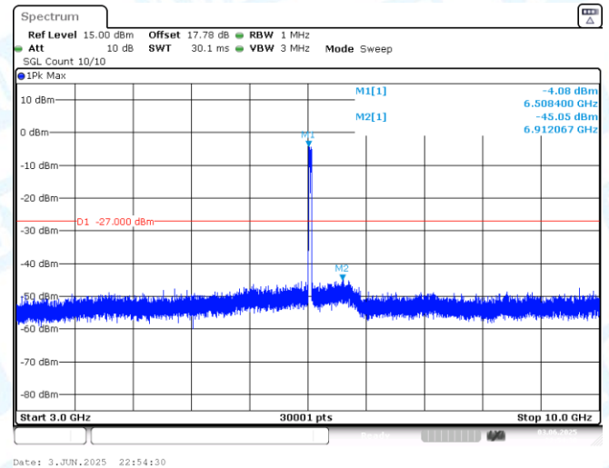
11AX40MIMO-Ant2-6525-3000~10000-PASS
