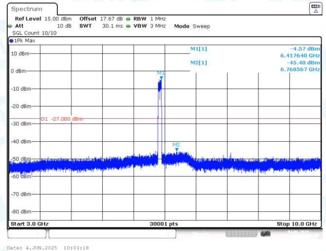
11AX80MIMO-Ant2-6385-3000~10000-PASS
