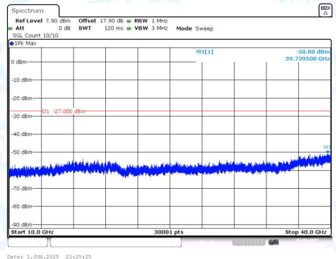
11AX40MIMO-Ant2-6845-10000~40000-PASS
