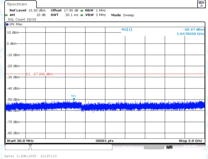
11AX40MIMO-Ant2-6845-30~3000-PASS
