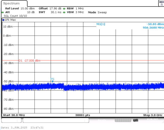
11AX40MIMO-Ant1-6925-30~3000-PASS
