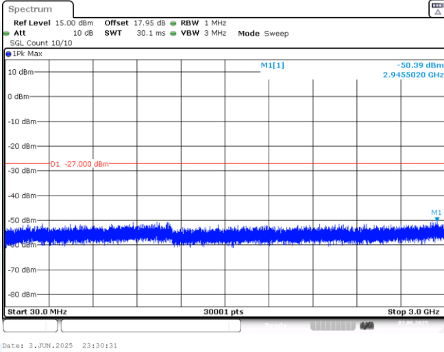
11AX40MIMO-Ant1-6885-30~3000-PASS
