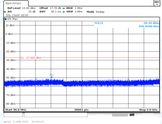
11AX40MIMO-Ant2-6525-30~3000-PASS
