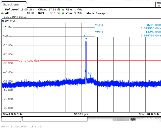
11AX40MIMO-Ant1-6685-3000~10000-PASS
