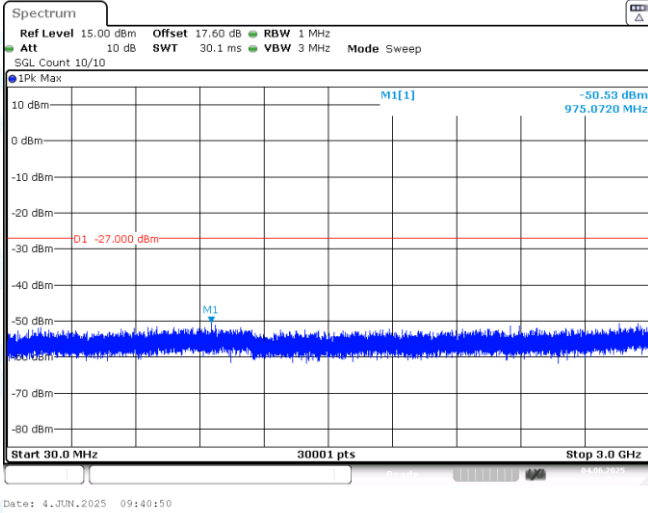
11AX80MIMO-Ant1-6145-30~3000-PASS
