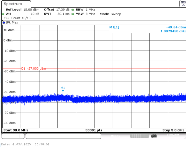
11AX80MIMO-Ant1-5985-30~3000-PASS
