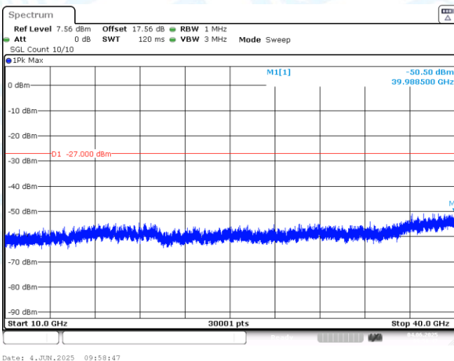
11AX80MIMO-Ant1-6385-10000~40000-PASS
