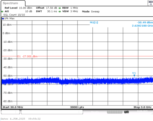
11AX80MIMO-Ant1-6385-30~3000-PASS
