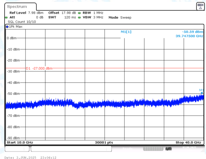
11AX40MIMO-Ant2-6565-10000~40000-PASS
