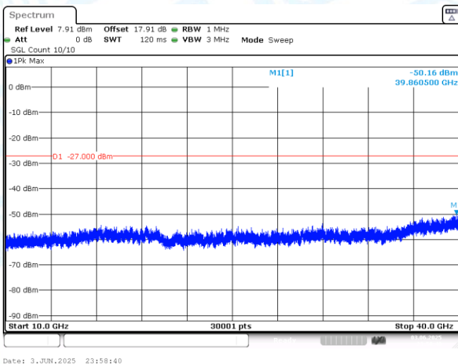
11AX40MIMO-Ant1-6965-10000~40000-PASS
