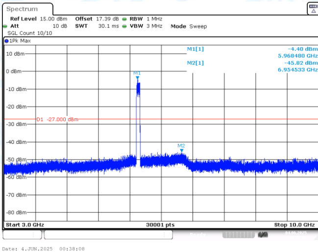
11AX80MIMO-Ant1-5985-3000~10000-PASS
