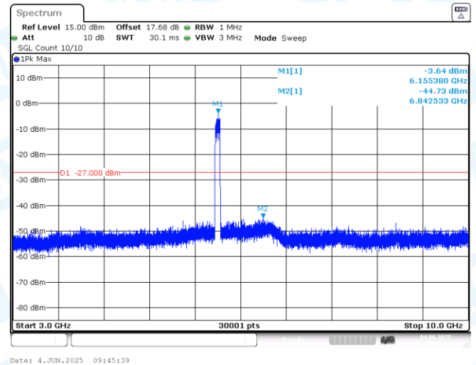
11AX80MIMO-Ant2-6145-3000~10000-PASS
