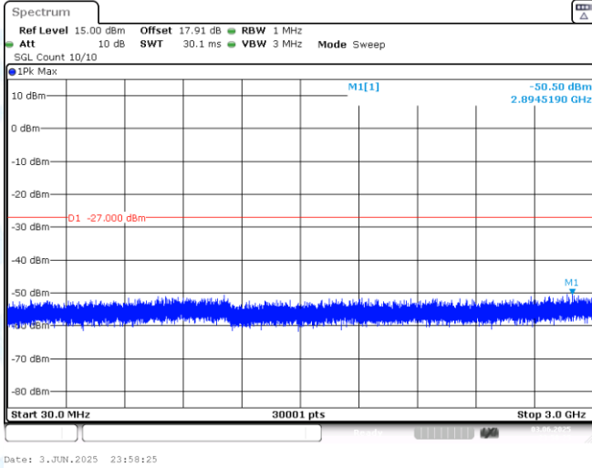
11AX40MIMO-Ant1-6965-30~3000-PASS
