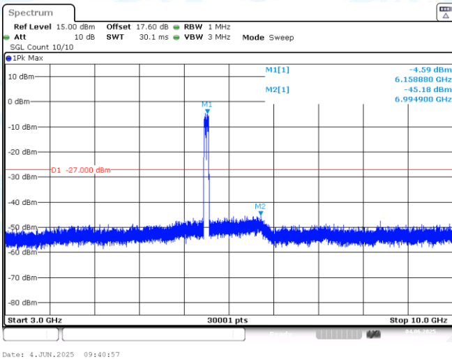
11AX80MIMO-Ant1-6145-3000~10000-PASS
