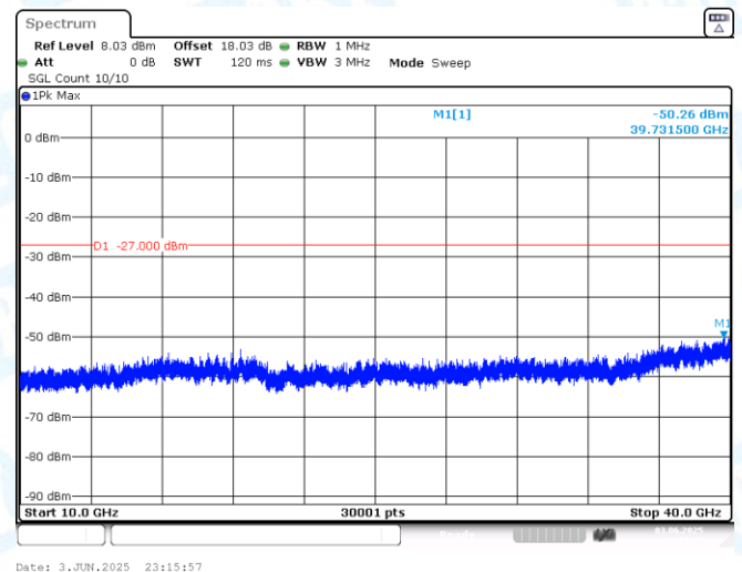
11AX40MIMO-Ant2-6685-10000~40000-PASS
