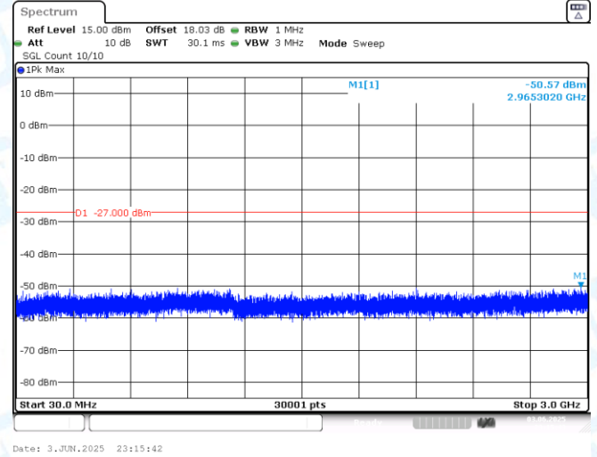
11AX40MIMO-Ant2-6685-30~3000-PASS
