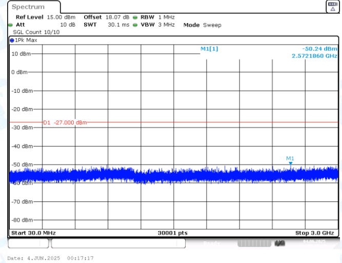
11AX40MIMO-Ant2-7085-30~3000-PASS
