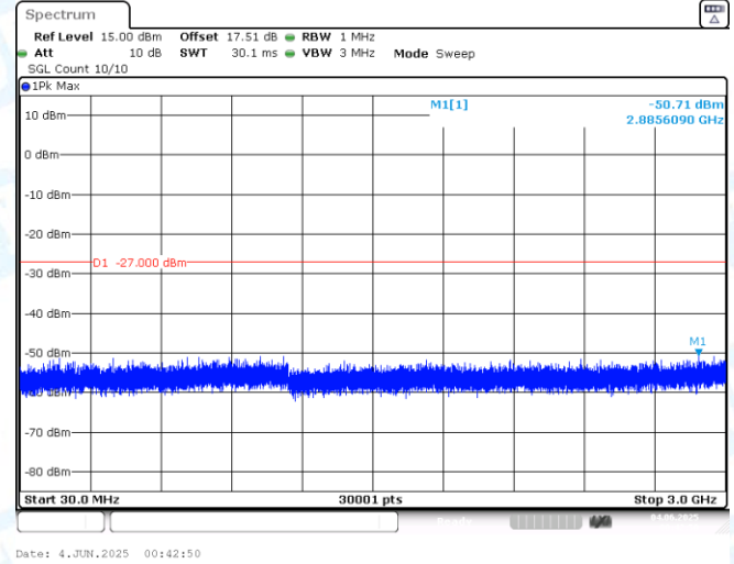
11AX80MIMO-Ant2-5985-30~3000-PASS
