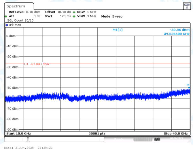
11AX40MIMO-Ant2-6885-10000~40000-PASS
