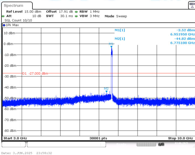
11AX40MIMO-Ant1-6965-3000~10000-PASS
