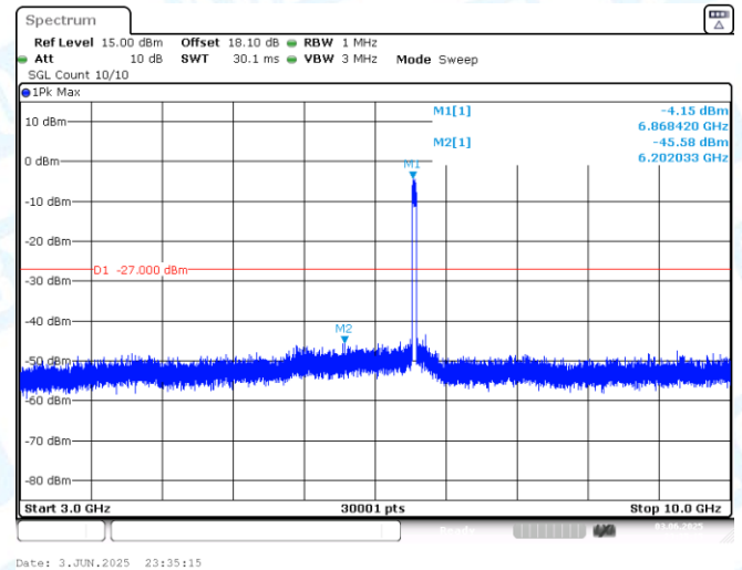
11AX40MIMO-Ant2-6885-3000~10000-PASS
