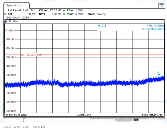
11AX80MIMO-Ant2-6385-10000~40000-PASS
