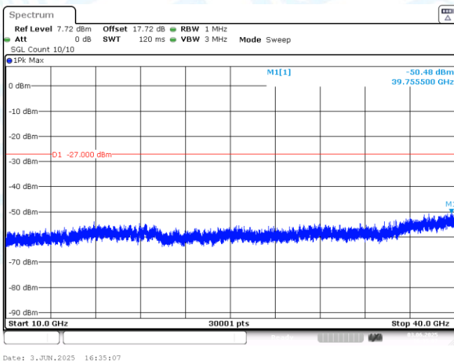
11AX20MIMO-Ant1-6535-10000~40000-PASS
