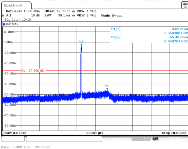
11AX40MIMO-Ant1-5965-3000~10000-PASS
