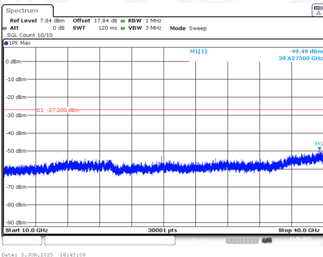
11AX20MIMO-Ant1-6695-10000~40000-PASS
