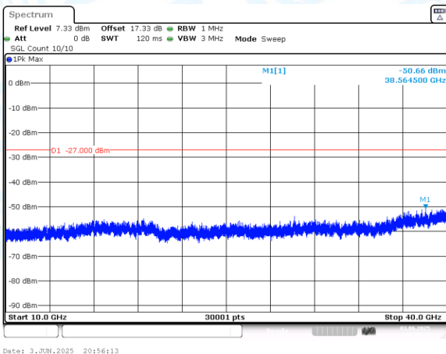
11AX40MIMO-Ant1-5965-10000~40000-PASS
