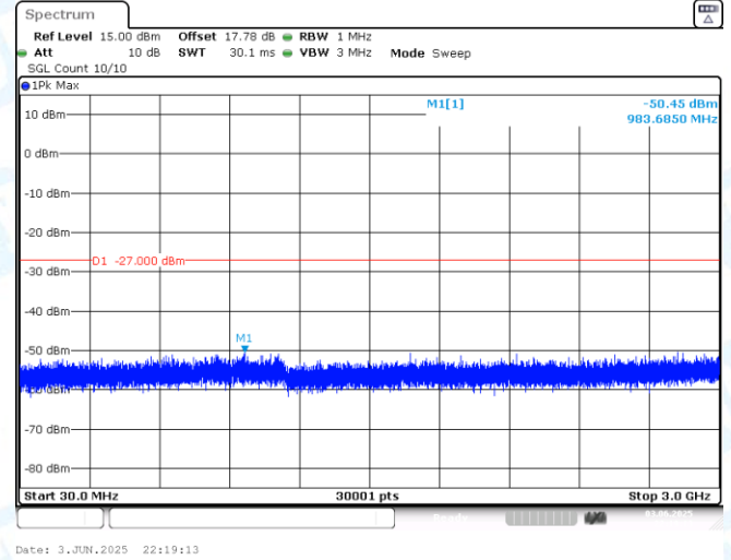
11AX40MIMO-Ant2-6445-30~3000-PASS
