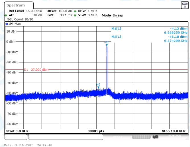
11AX20MIMO-Ant2-6895-3000~10000-PASS
