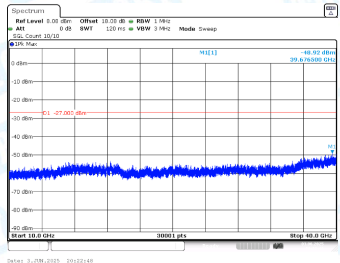
11AX20MIMO-Ant2-6895-10000~40000-PASS
