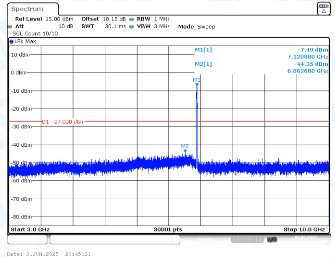
11AX20MIMO-Ant2-7115-3000~10000-PASS
