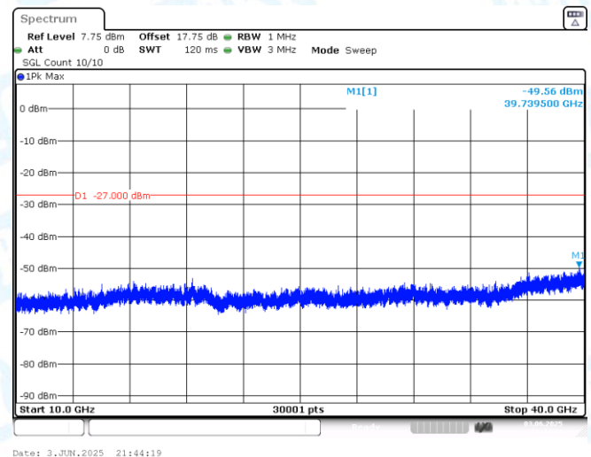
11AX40MIMO-Ant2-6405-10000~40000-PASS
