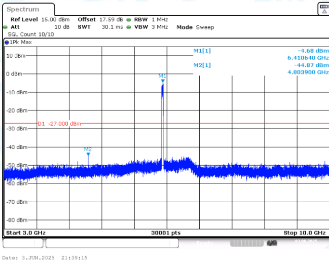
11AX40MIMO-Ant1-6405-3000~10000-PASS
