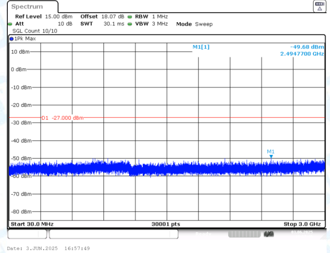
11AX20MIMO-Ant2-6695-30~3000-PASS
