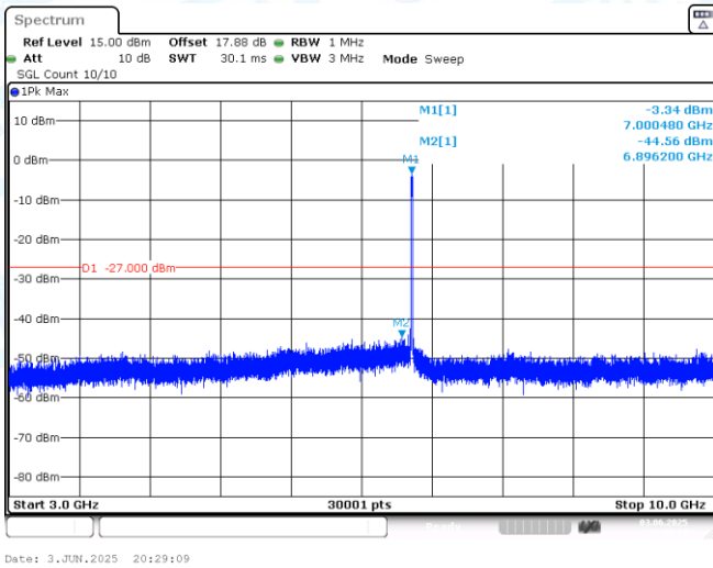
11AX20MIMO-Ant1-6995-3000~10000-PASS
