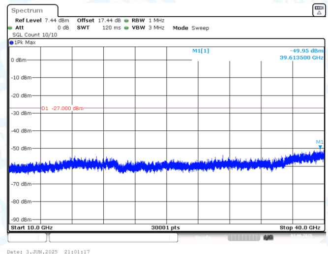
11AX40MIMO-Ant2-5965-10000~40000-PASS
