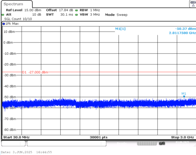
11AX20MIMO-Ant1-6695-30~3000-PASS
