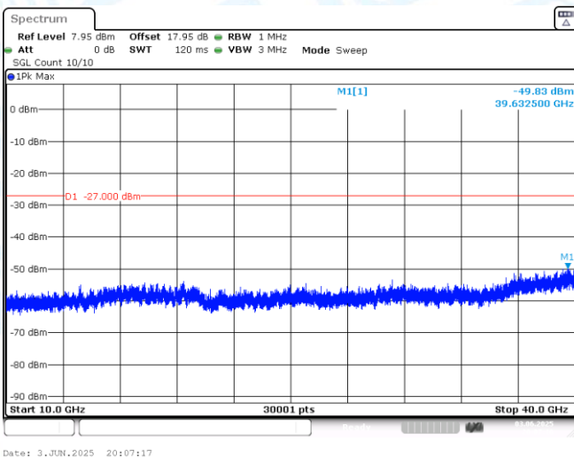
11AX20MIMO-Ant1-6875-10000~40000-PASS
