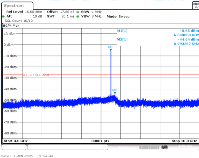
11AX20MIMO-Ant1-6855-3000~10000-PASS
