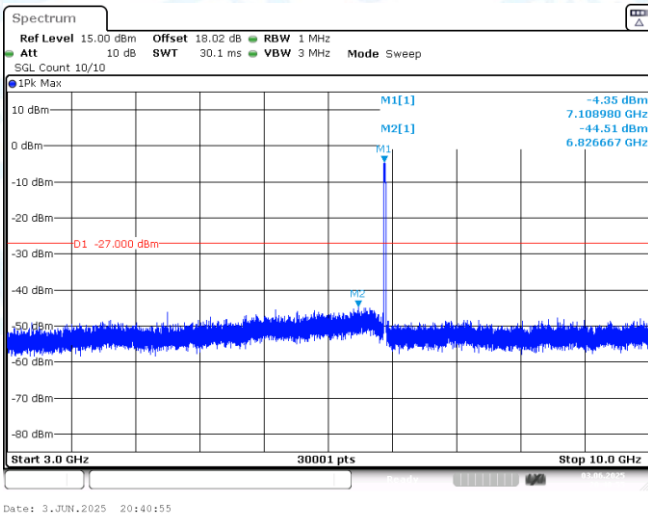
11AX20MIMO-Ant1-7115-3000~10000-PASS
