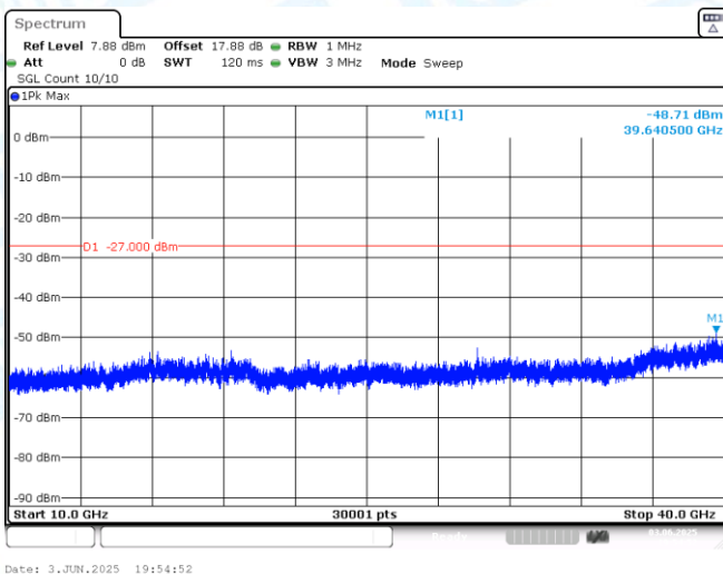
11AX20MIMO-Ant1-6855-10000~40000-PASS
