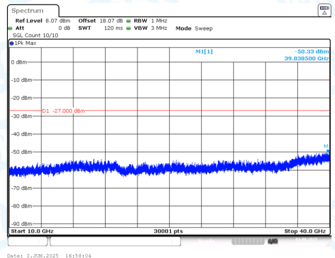
11AX20MIMO-Ant2-6695-10000~40000-PASS
