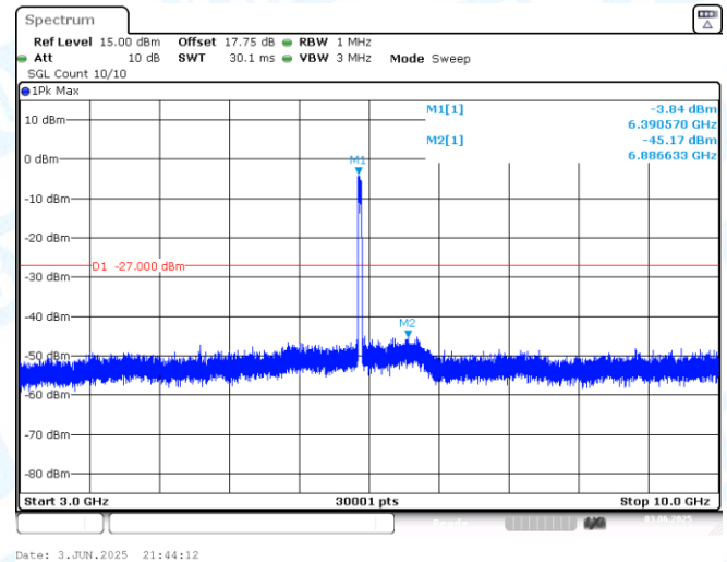
11AX40MIMO-Ant2-6405-3000~10000-PASS
