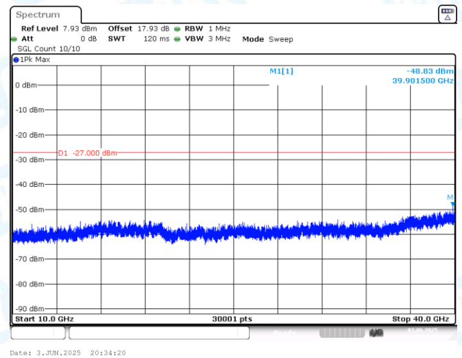
11AX20MIMO-Ant2-6995-10000~40000-PASS
