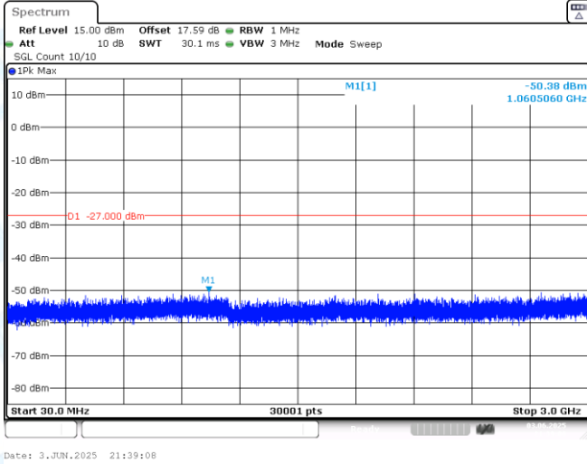
11AX40MIMO-Ant1-6405-30~3000-PASS
