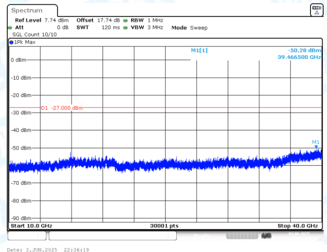
11AX40MIMO-Ant2-6485-10000~40000-PASS
