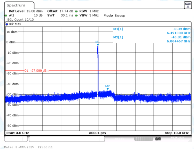
11AX40MIMO-Ant2-6485-3000~10000-PASS
