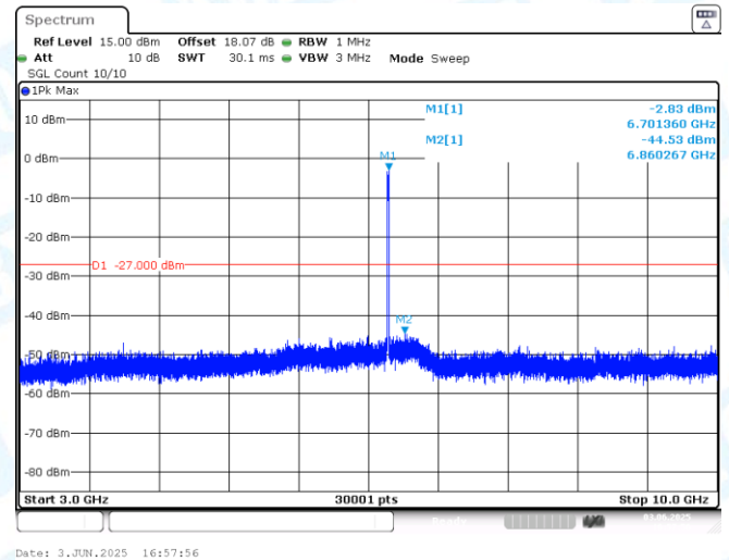
11AX20MIMO-Ant2-6695-3000~10000-PASS
