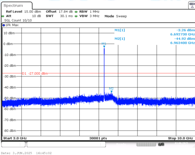
11AX20MIMO-Ant1-6695-3000~10000-PASS
