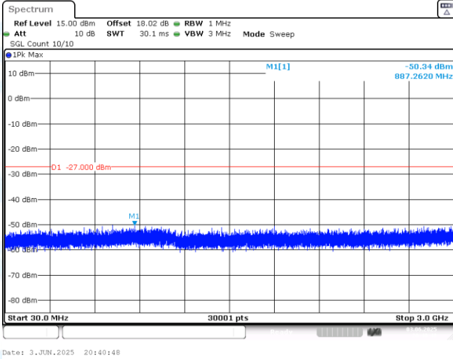
11AX20MIMO-Ant1-7115-30~3000-PASS
