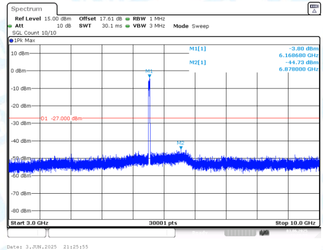
11AX40MIMO-Ant2-6165-3000~10000-PASS
