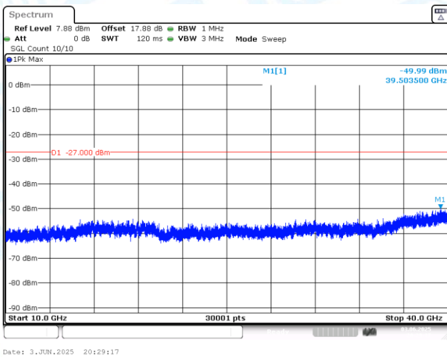
11AX20MIMO-Ant1-6995-10000~40000-PASS
