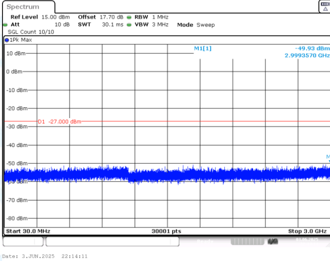
11AX40MIMO-Ant1-6445-30~3000-PASS
