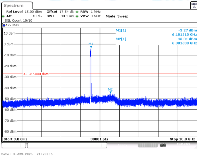
11AX40MIMO-Ant1-6165-3000~10000-PASS
