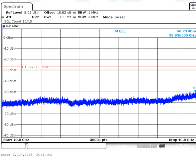
11AX20MIMO-Ant1-7115-10000~40000-PASS
