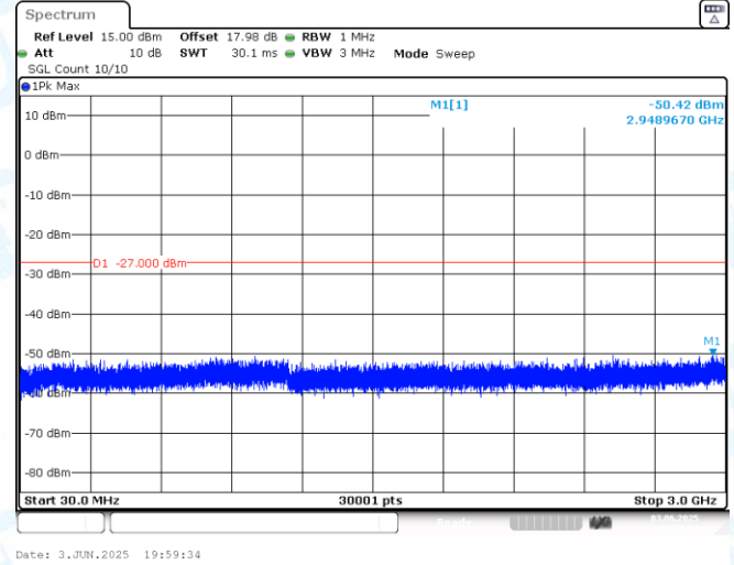
11AX20MIMO-Ant2-6855-30~3000-PASS
