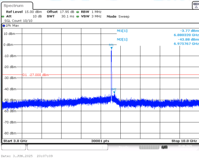
11AX20MIMO-Ant1-6875-3000~10000-PASS
