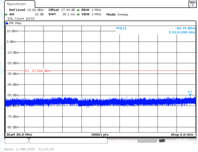
11AX40MIMO-Ant2-5965-30~3000-PASS
