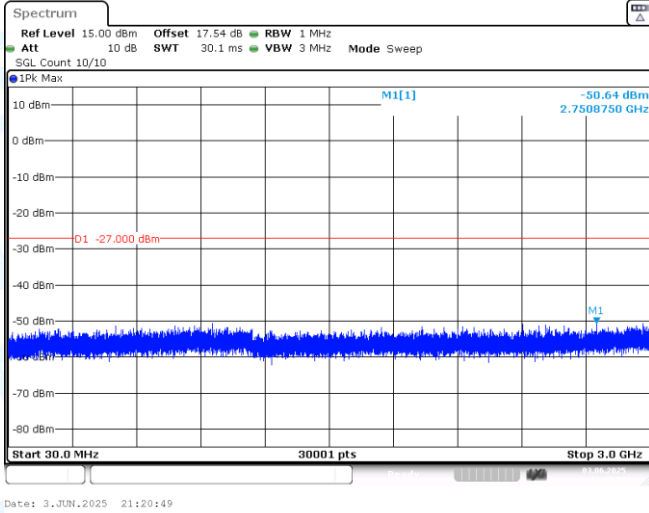
11AX40MIMO-Ant1-6165-30~3000-PASS
