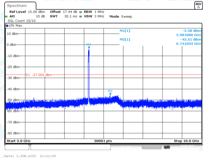
11AX40MIMO-Ant2-5965-3000~10000-PASS
