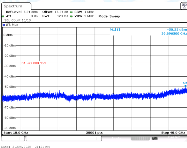
11AX40MIMO-Ant1-6165-10000~40000-PASS
