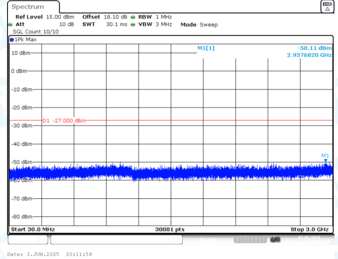
11AX20MIMO-Ant2-6875-30~3000-PASS
