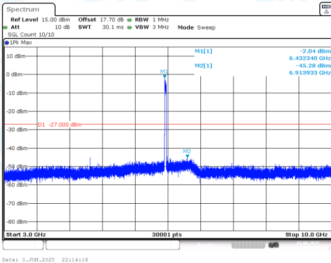
11AX40MIMO-Ant1-6445-3000~10000-PASS
