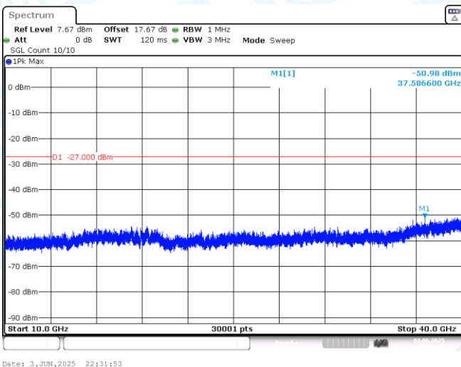
11AX40MIMO-Ant1-6485-10000~40000-PASS
