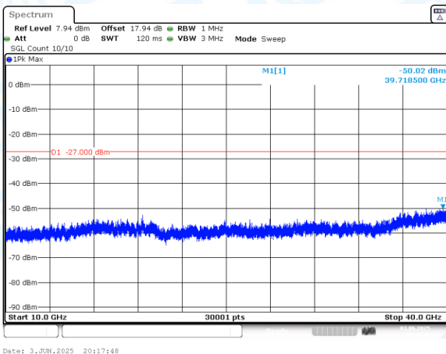
11AX20MIMO-Ant1-6895-10000~40000-PASS
