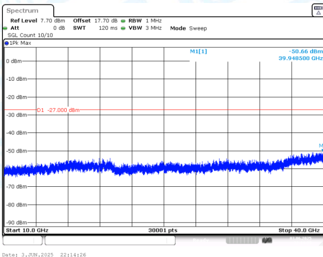
11AX40MIMO-Ant1-6445-10000~40000-PASS
