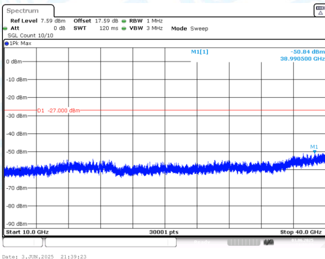
11AX40MIMO-Ant1-6405-10000~40000-PASS
