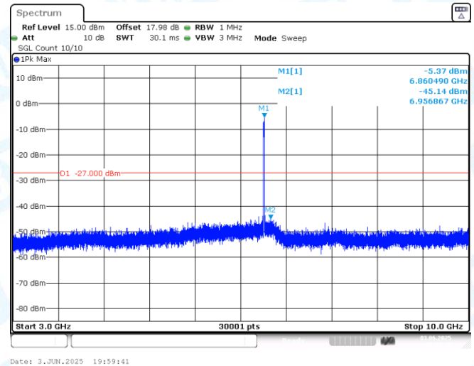
11AX20MIMO-Ant2-6855-3000~10000-PASS
