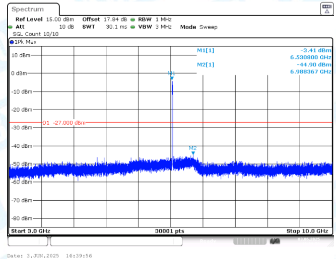
11AX20MIMO-Ant2-6535-3000~10000-PASS
