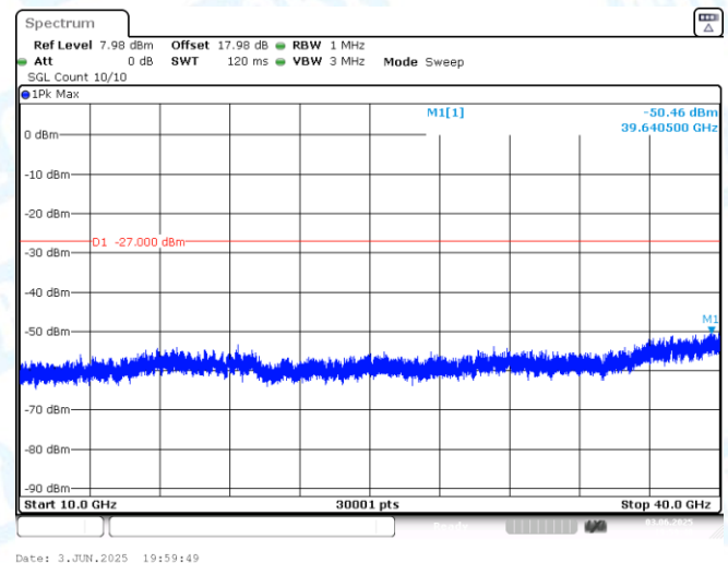
11AX20MIMO-Ant2-6855-10000~40000-PASS
