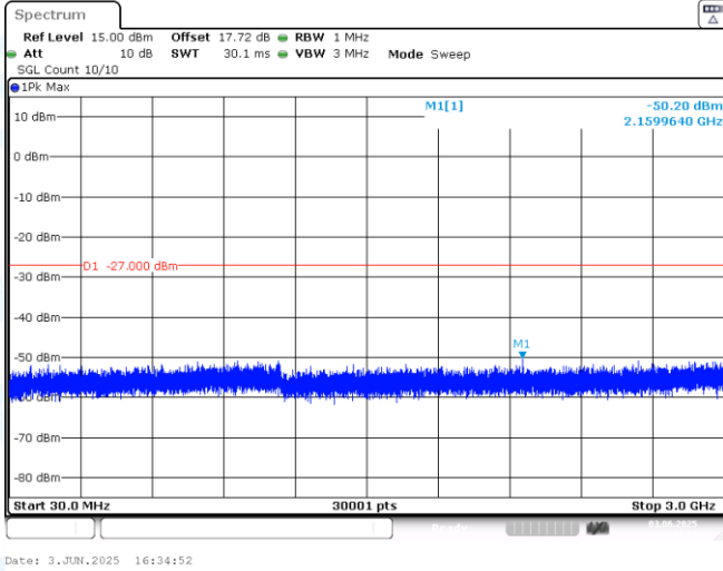
11AX20MIMO-Ant1-6535-30~3000-PASS
