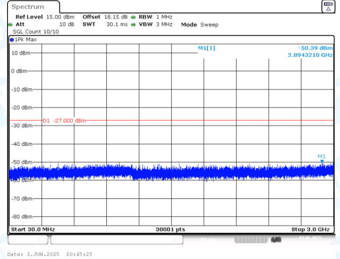
11AX20MIMO-Ant2-7115-30~3000-PASS
