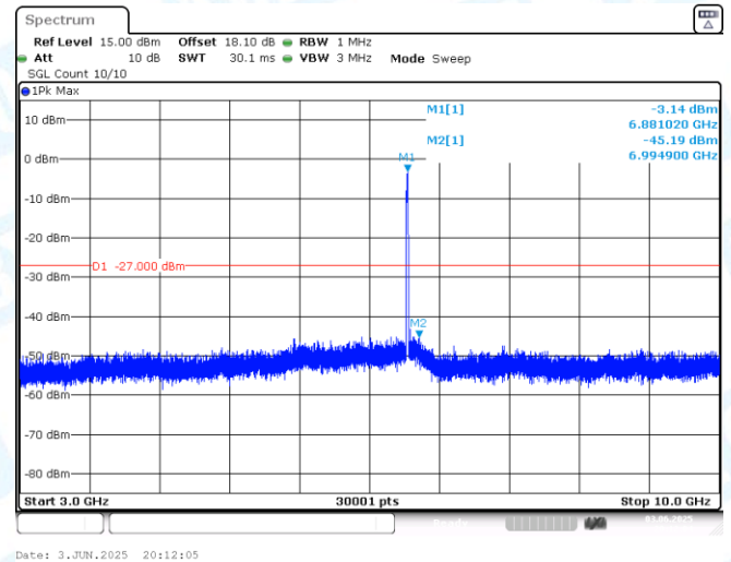
11AX20MIMO-Ant2-6875-3000~10000-PASS
