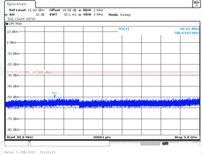
11AX20MIMO-Ant2-6895-30~3000-PASS
