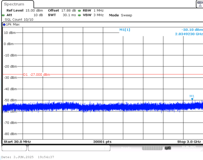
11AX20MIMO-Ant1-6855-30~3000-PASS
