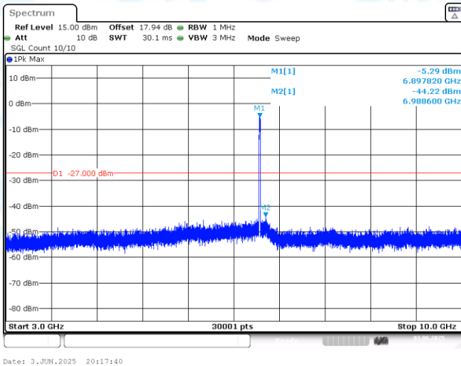
11AX20MIMO-Ant1-6895-3000~10000-PASS
