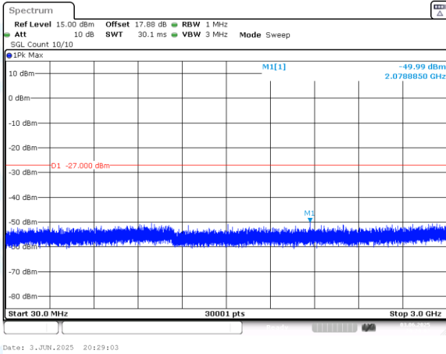
11AX20MIMO-Ant1-6995-30~3000-PASS
