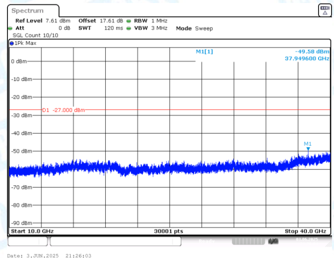
11AX40MIMO-Ant2-6165-10000~40000-PASS
