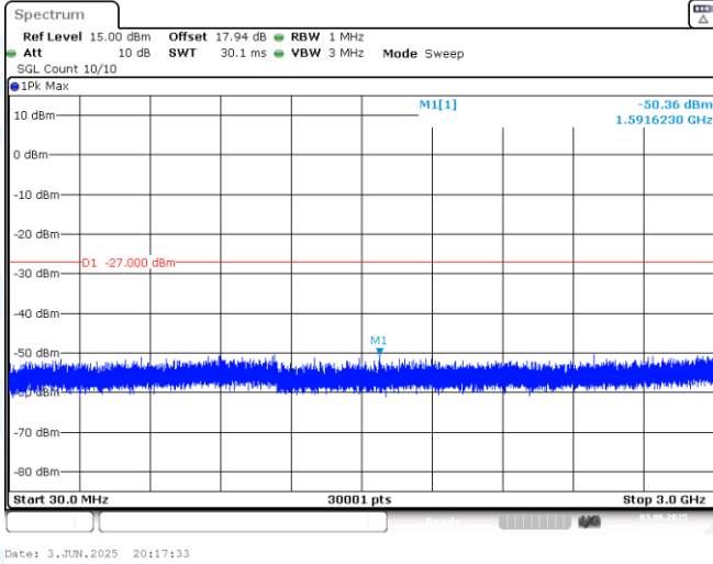
11AX20MIMO-Ant1-6895-30~3000-PASS
