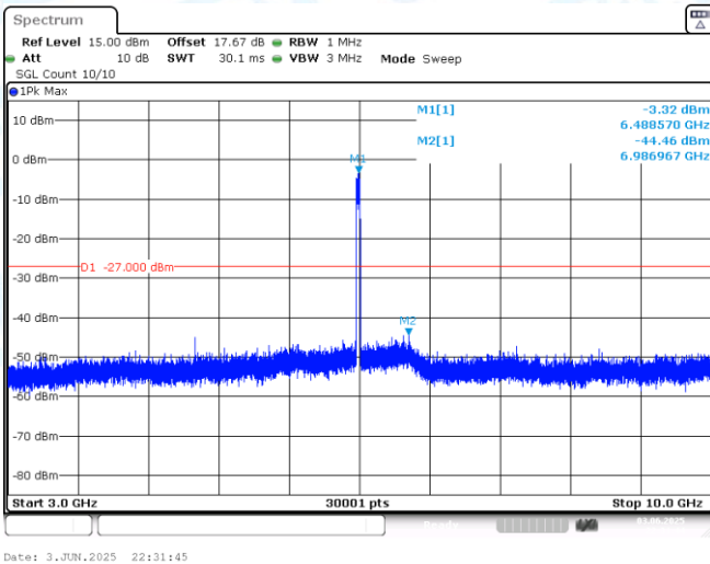
11AX40MIMO-Ant1-6485-3000~10000-PASS
