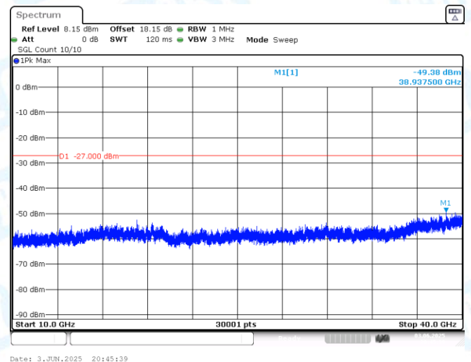
11AX20MIMO-Ant2-7115-10000~40000-PASS
