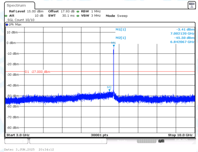
11AX20MIMO-Ant2-6995-3000~10000-PASS
