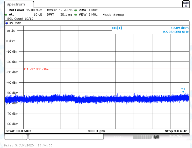
11AX20MIMO-Ant2-6995-30~3000-PASS
