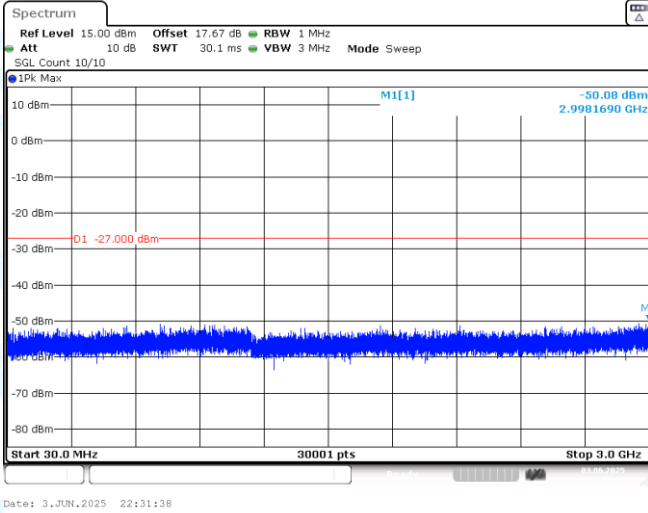
11AX40MIMO-Ant1-6485-30~3000-PASS
