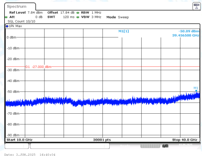
11AX20MIMO-Ant2-6535-10000~40000-PASS
