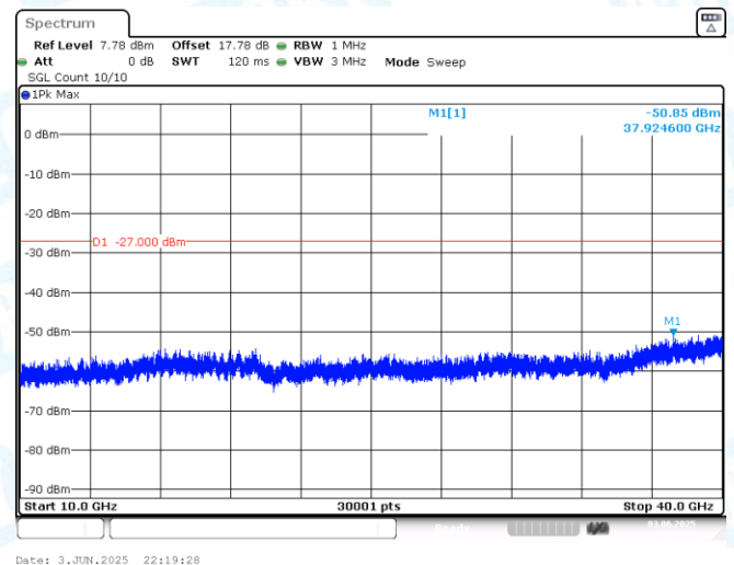
11AX40MIMO-Ant2-6445-10000~40000-PASS
