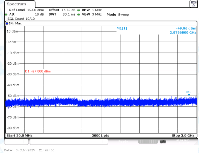
11AX40MIMO-Ant2-6405-30~3000-PASS
