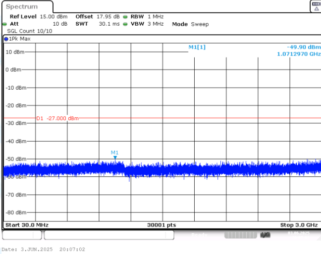
11AX20MIMO-Ant1-6875-30~3000-PASS
