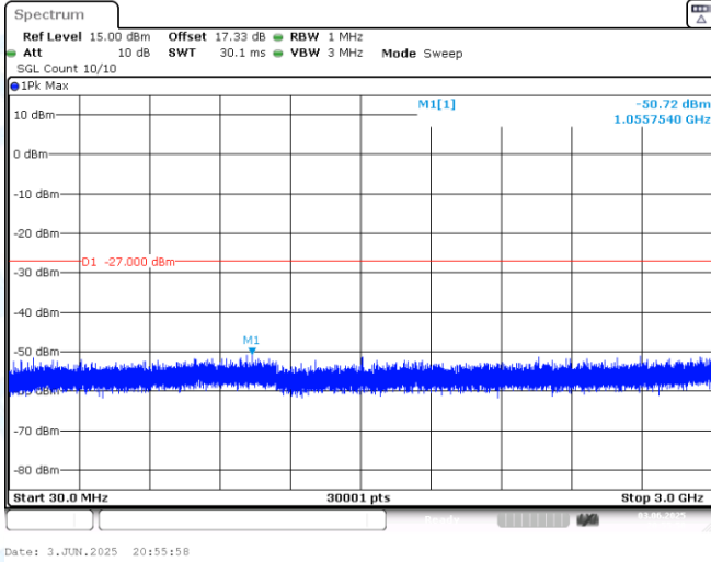
11AX40MIMO-Ant1-5965-30~3000-PASS
