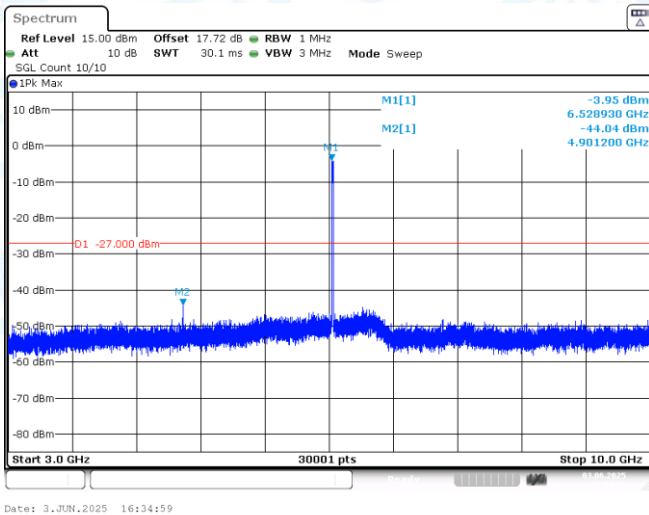
11AX20MIMO-Ant1-6535-3000~10000-PASS
