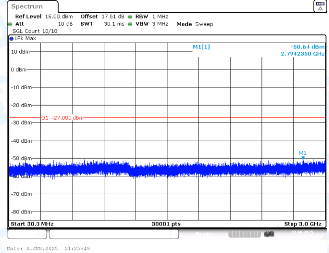
11AX40MIMO-Ant2-6165-30~3000-PASS
