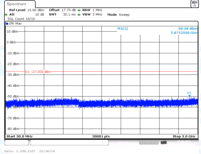
11AX40MIMO-Ant2-6485-30~3000-PASS
