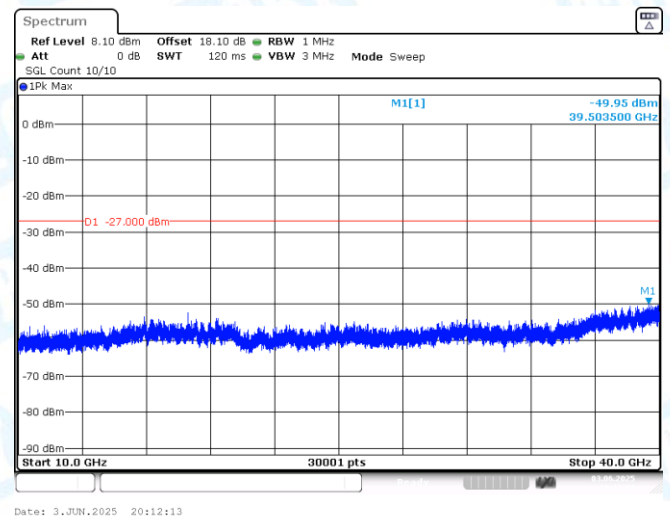
11AX20MIMO-Ant2-6875-10000~40000-PASS
