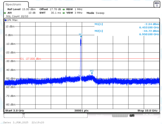
11AX40MIMO-Ant2-6445-3000~10000-PASS
