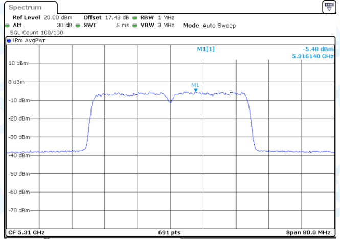
11AX40MIMO-Ant1-5310-PASS
