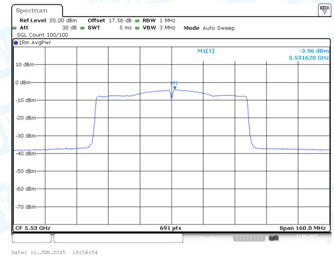
11AC80MIMO-Ant1-5530-PASS
