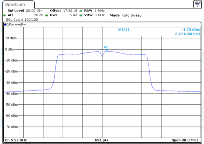
11AC40MIMO-Ant1-5270-PASS
