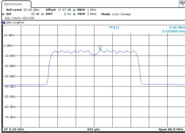
11AX40MIMO-Ant2-5550-PASS
