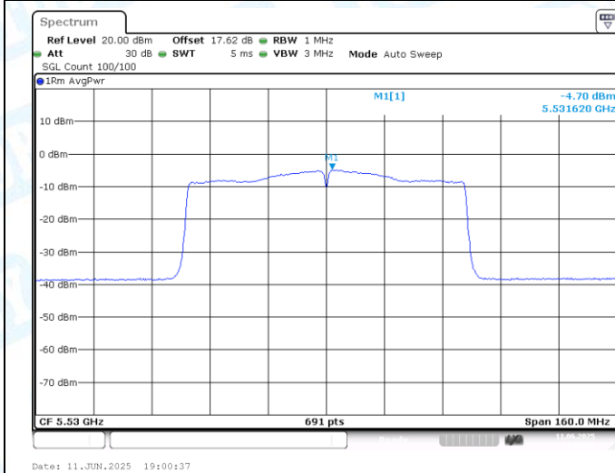
11AC80MIMO-Ant2-5530-PASS
