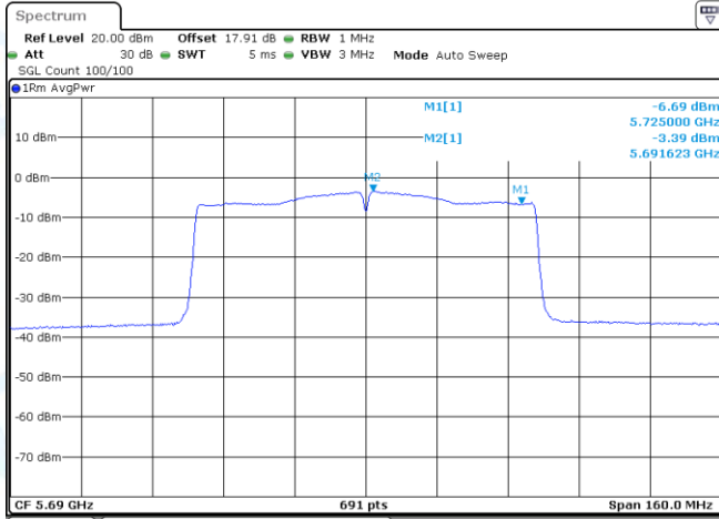
11AC80MIMO-Ant2-5690_UNII-2C-PASS
