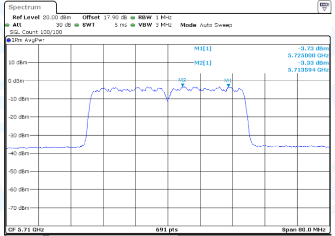
11AX40MIMO-Ant1-5710_UNII-2C-PASS
