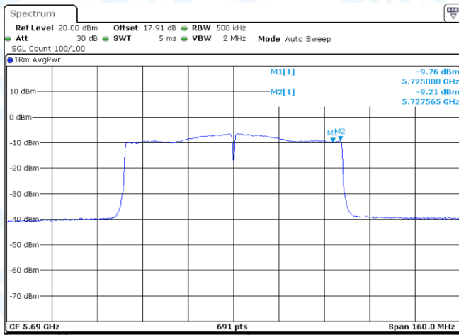
11AC80MIMO-Ant2-5690_UNII-2C-PASS
