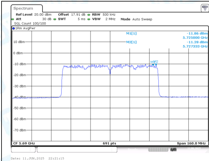
11AX80MIMO-Ant2-5690_UNII-3-PASS
