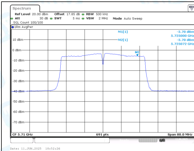
11AC40MIMO-Ant2-5710_UNII-3-PASS
