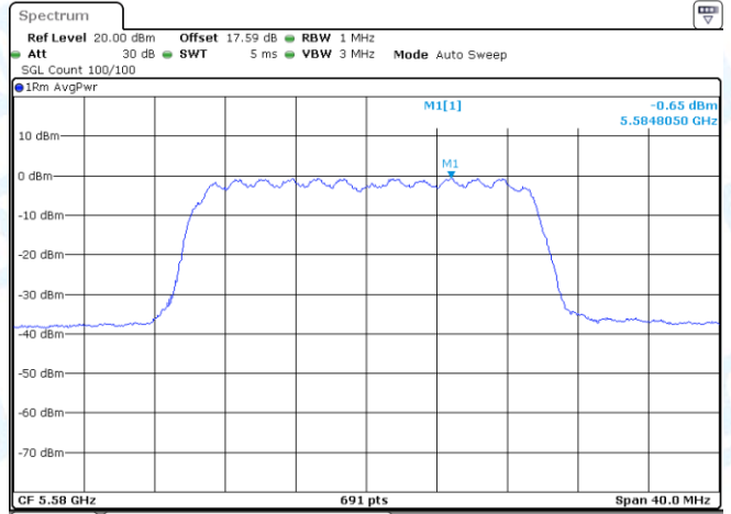
11AX20MIMO-Ant1-5580-PASS
