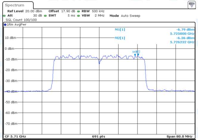
11AX40MIMO-Ant1-5710_UNII-2C-PASS
