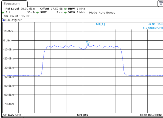
11AX40MIMO-Ant2-5270-PASS
