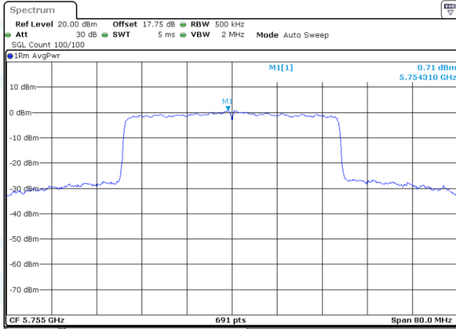
11AX40MIMO-Ant2-5755-PASS
