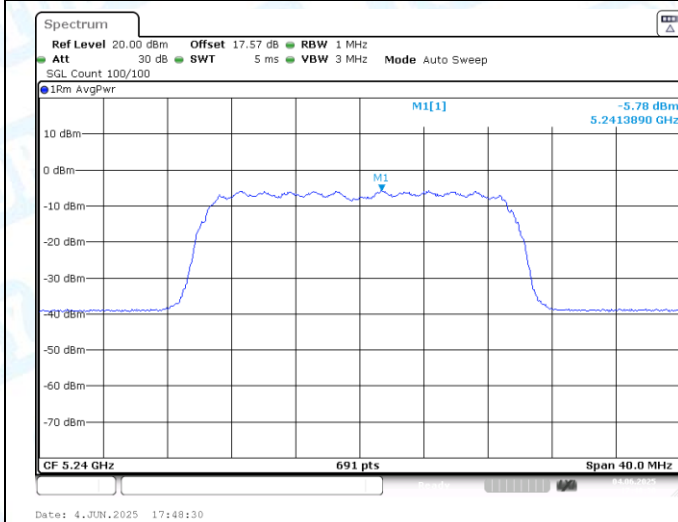
11AX20MIMO-Ant2-5240-PASS
