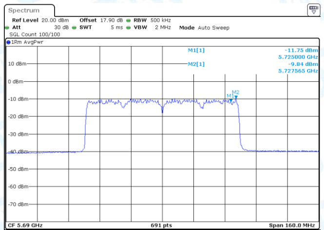
11AX80MIMO-Ant1-5690_UNII-2C-PASS
