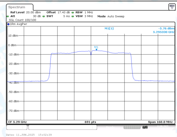
11AC80MIMO-Ant1-5290-PASS
