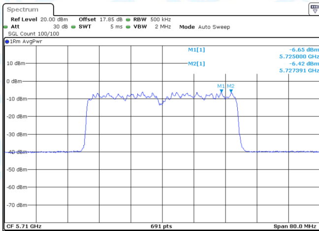
11AX40MIMO-Ant2-5710_UNII-2C-PASS
