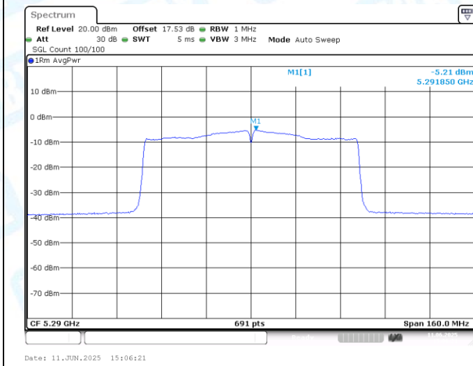
11AC80MIMO-Ant2-5290-PASS
