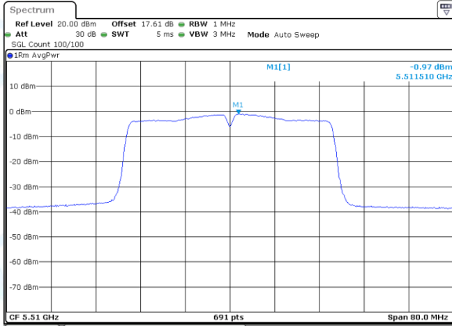
11AC40MIMO-Ant2-5510-PASS
