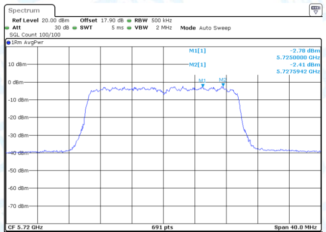
11AX20MIMO-Ant1-5720_UNII-2C-PASS
