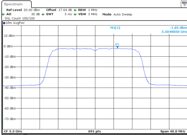
11AX20MIMO-Ant2-5500-PASS
