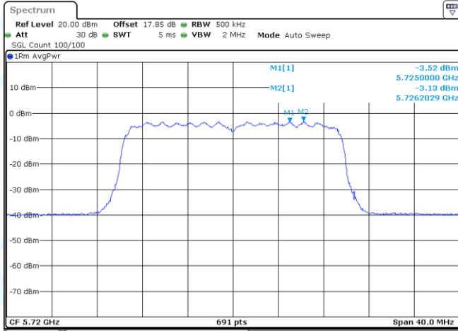
11AX20MIMO-Ant2-5720_UNII-3-PASS
