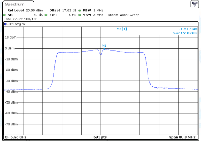
11AC40MIMO-Ant1-5550-PASS
