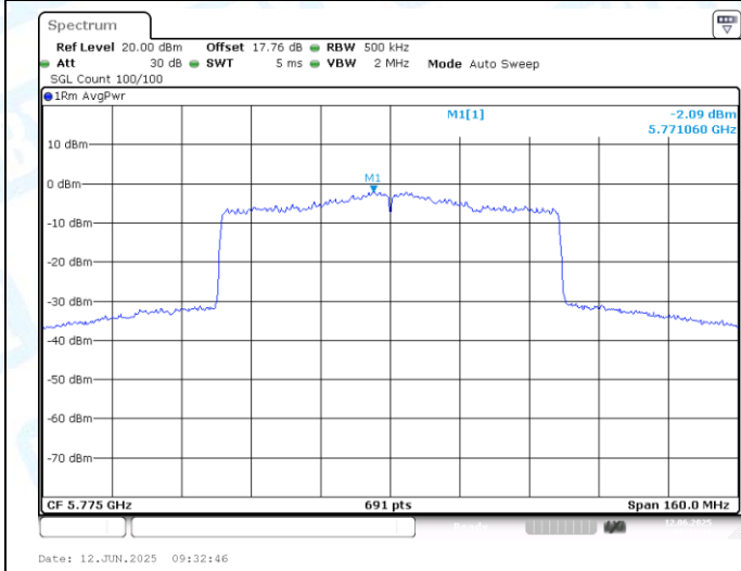
11AX80MIMO-Ant2-5775-PASS
