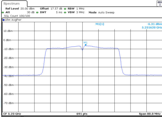
11AC40MIMO-Ant2-5230-PASS
