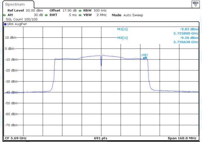
11AC80MIMO-Ant1-5690_UNII-3-PASS
