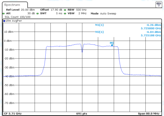
11AC40MIMO-Ant1-5710_UNII-2C-PASS
