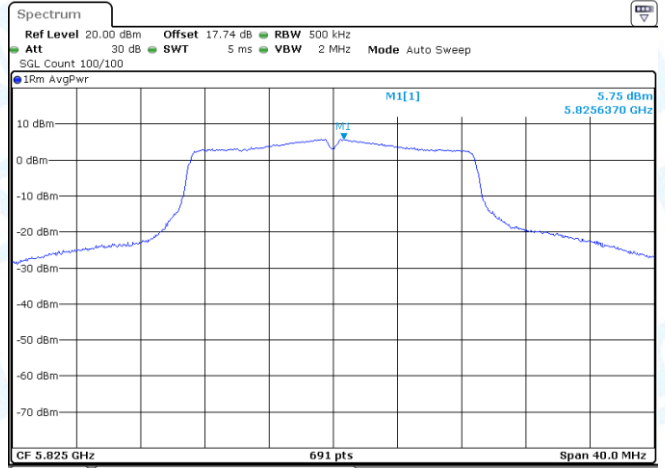
11AC20MIMO-Ant1-5825-PASS
