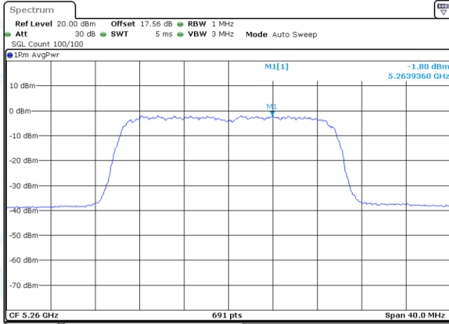
11AX20MIMO-Ant2-5260-PASS
