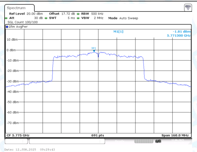
11AX80MIMO-Ant1-5775-PASS
