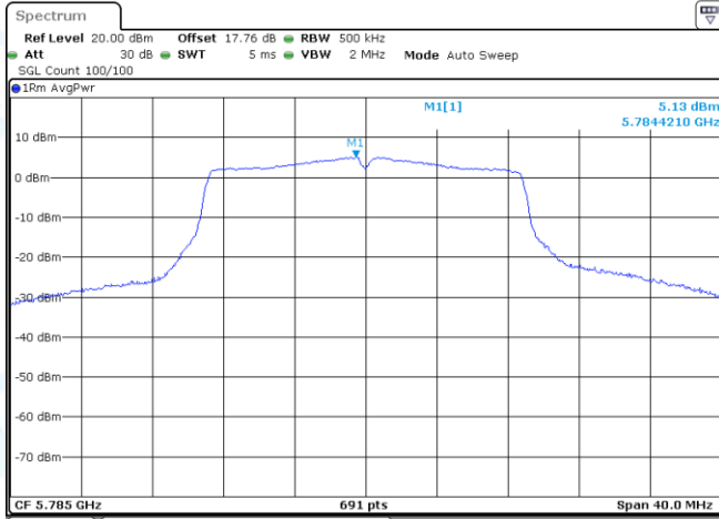
11AC20MIMO-Ant2-5785-PASS
