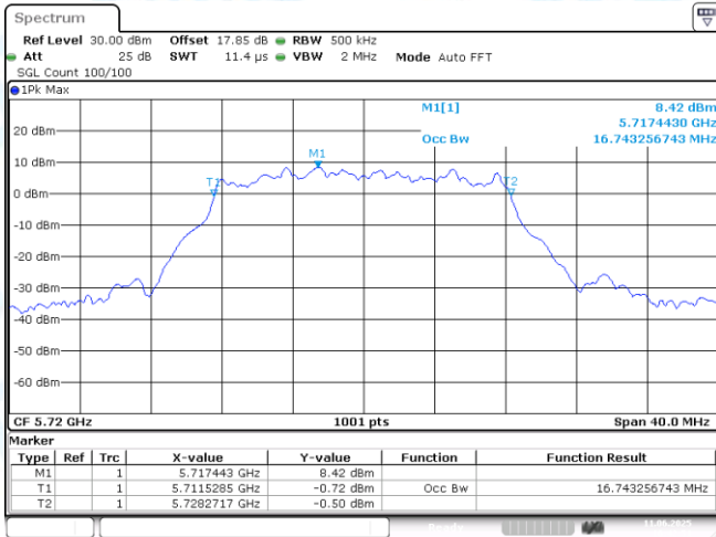
11A-CDD-Ant2-5720
