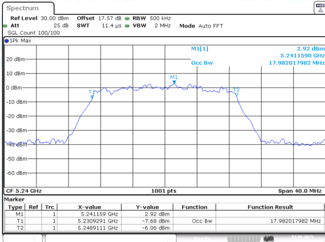
11N20MIMO-Ant2-5240
