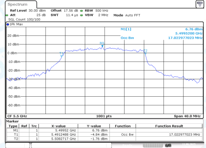
11A-CDD-Ant1-5500
