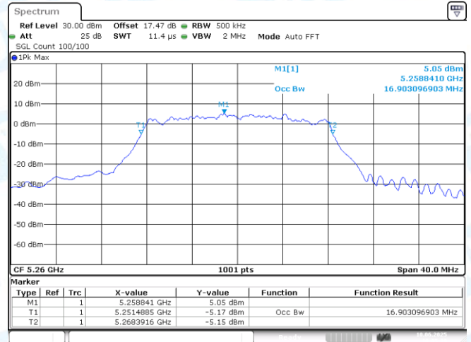
11A-CDD-Ant1-5260
