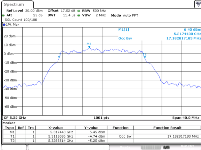
11A-CDD-Ant2-5320
