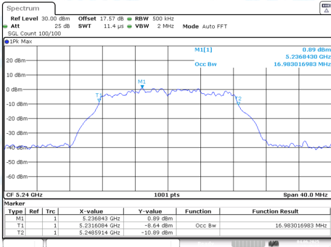
11A-CDD-Ant2-5240
