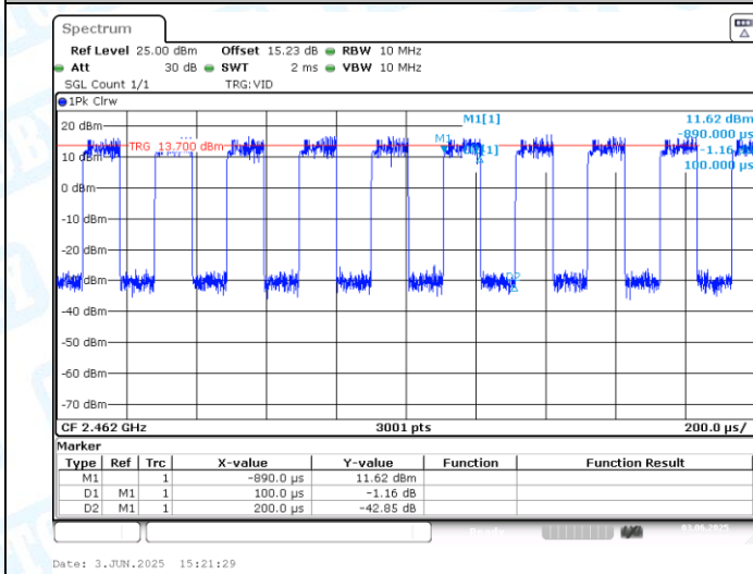
NTNV-11AX20MIMO-Ant2-2462
