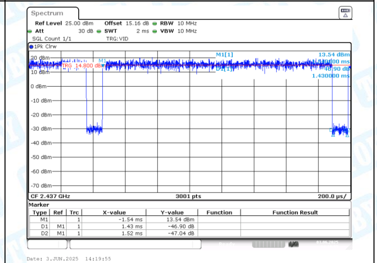
NTNV-11G-CDD-Ant1-2437
