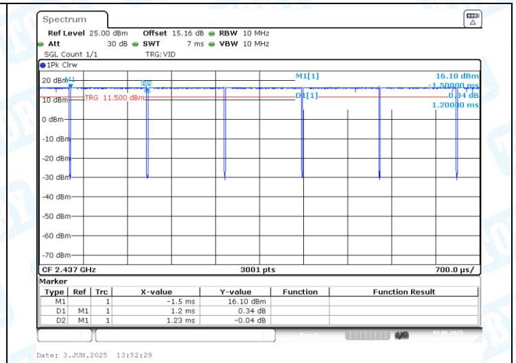
NTNV-11B-Ant1-2437
