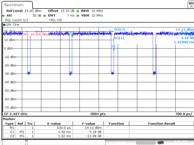
NTNV-11G-CDD-Ant2-2437
