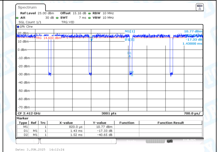
NTNV-11G-CDD-Ant1-2412
