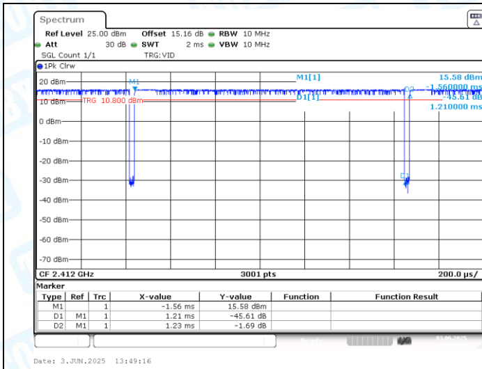
NTNV-11B-Ant1-2412
